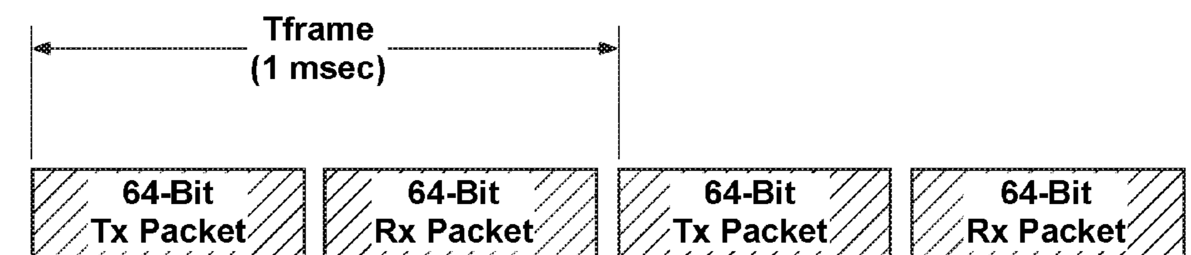
TDD Packet Structure
