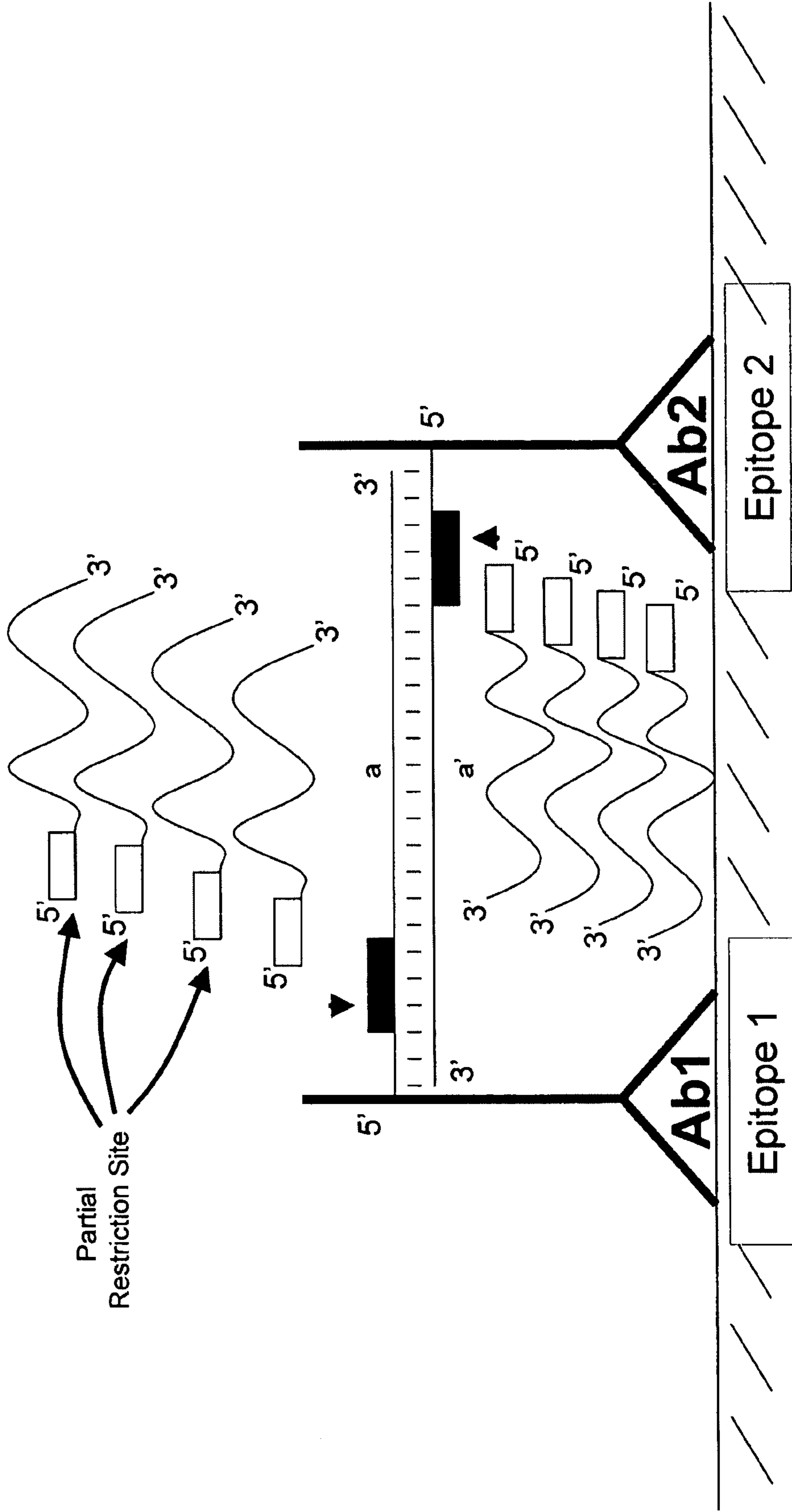
FIGURE 1D Extension, displacement and linear amplification
