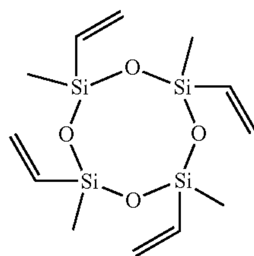
divinyl cyclotetrasiloxane,
