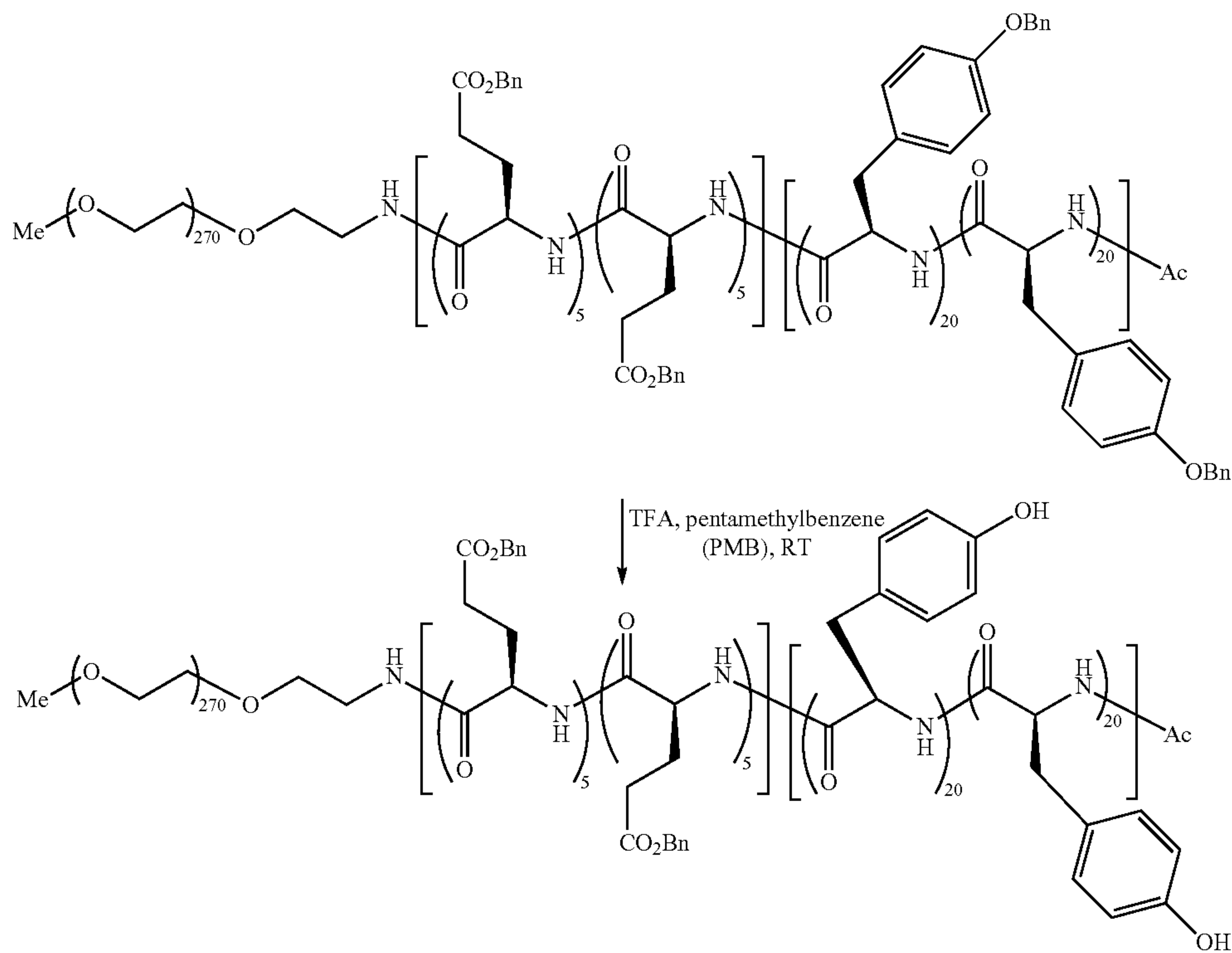
mPEG12K-b-Poly-(d-Glu(OBn) 5 -co-Glu(OBn) 5 )-b-Poly-(d-Tyr(OH) 20 -co-Tyr(OH) 20 )-Ac
