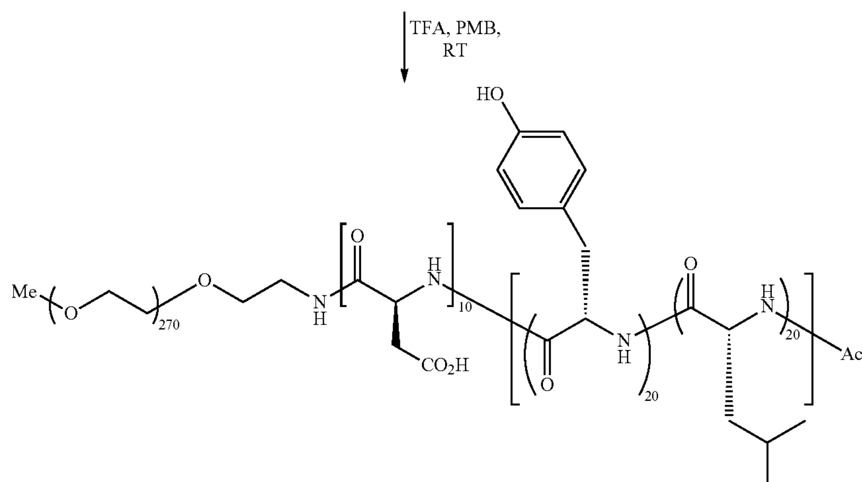
mPEG12K-b-Poly-(Asp(OH) 10 )-b-Poly-(d-Leu 20 -co-Tyr(OH) 20 )-Ac
