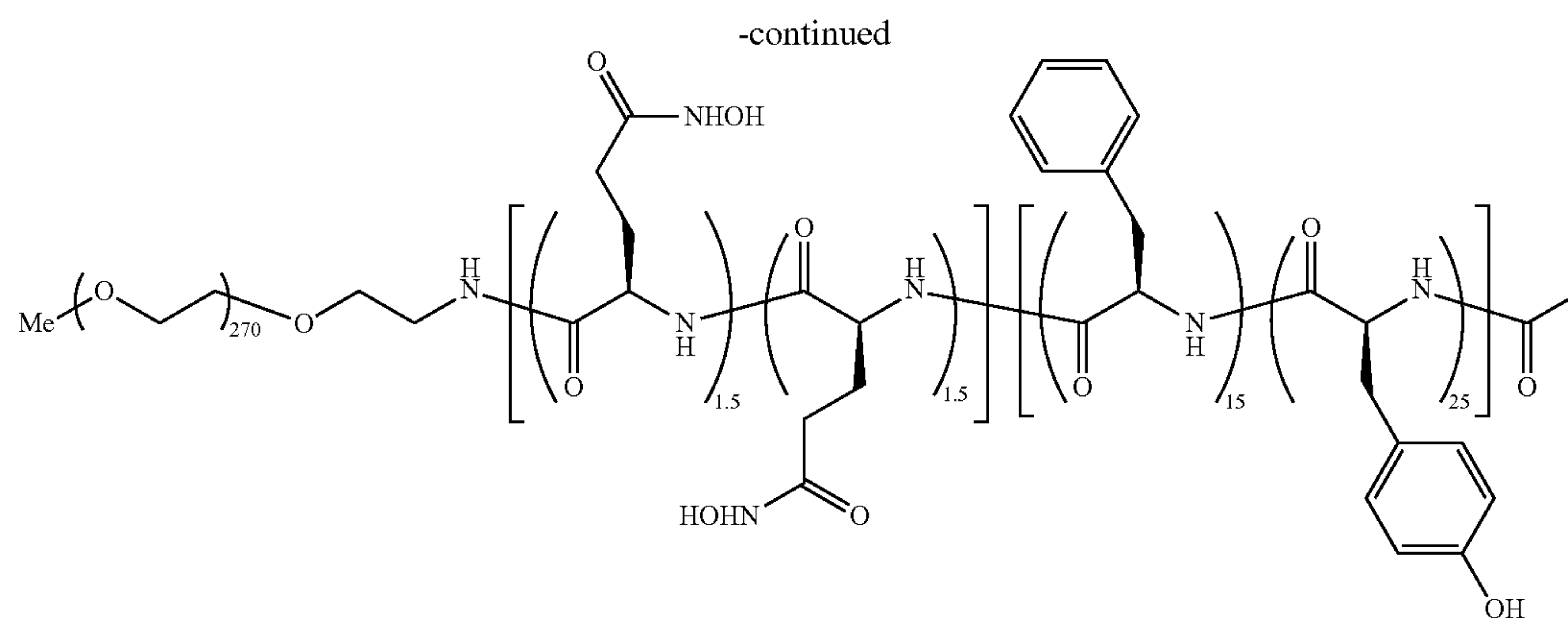
mPEG12K-b-Poly-(d-Glu(NHOH) 1.5 -co-Glu(NHOH) 1.5 )-b-Poly (Tyr(OH) 25 -co-d-Phe 15 )-Ac
