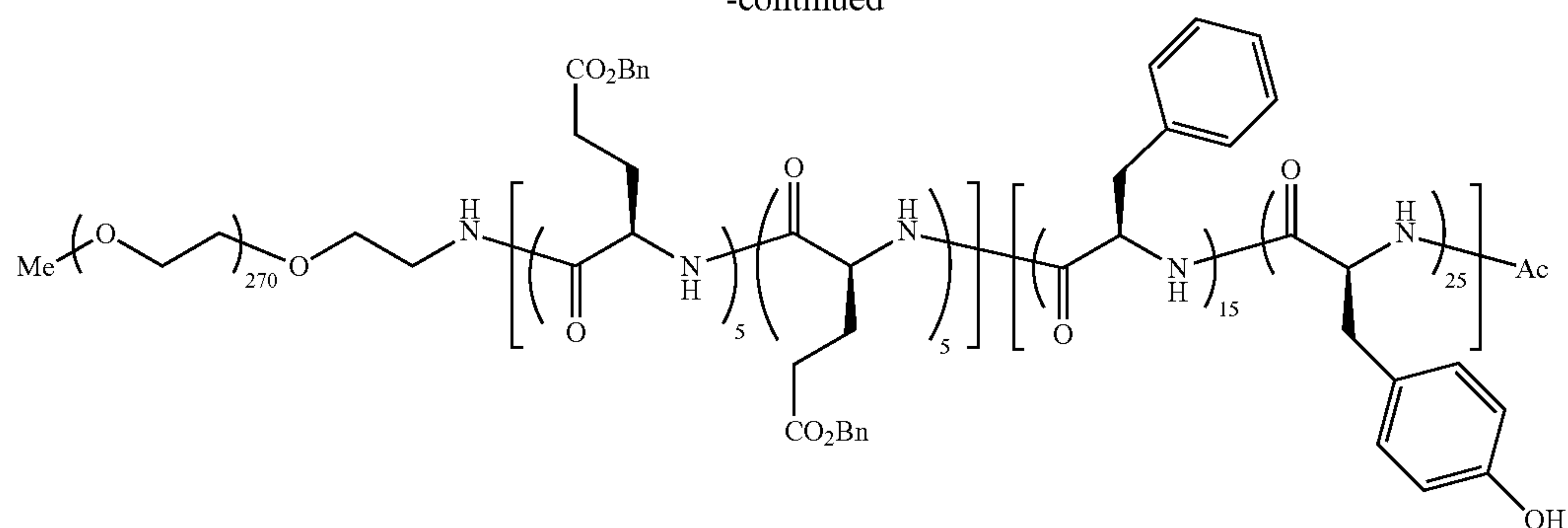
mPEG12K-b-Poly-[d-Glu(OBn) 5 -co-Glu(OBn) 5 ]-b-Poly-(Tyr(OH) 25 -co-d-Phe 15 )-Ac
