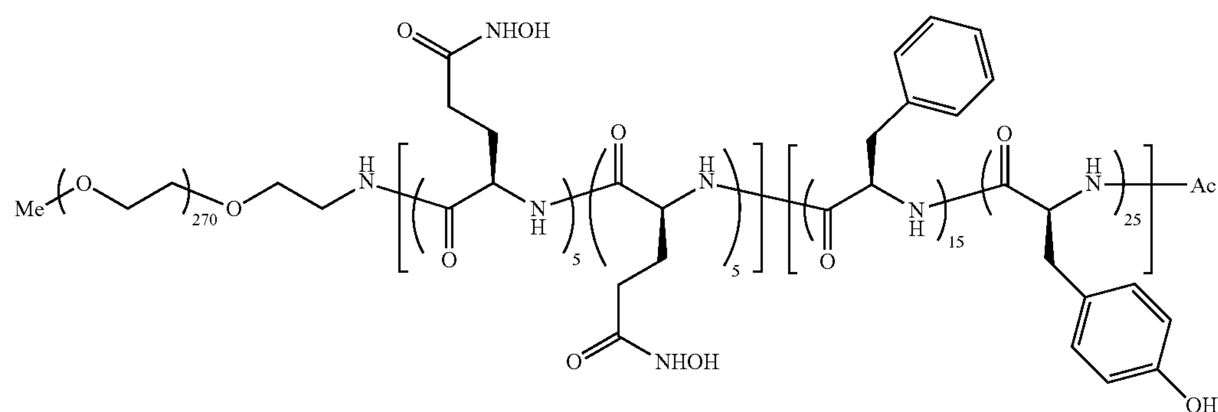
mPEG12K-b-Poly-[d-Glu(NHOH) 5 -co-Glu(NHOH) 5 ]-b-Poly-(Tyr(OH) 25 -co-d-Phe 15 )-Ac
