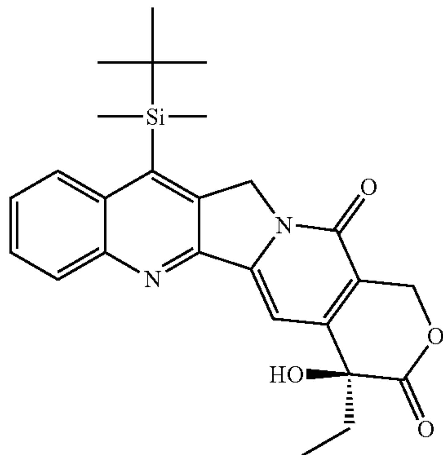
Silatecan
