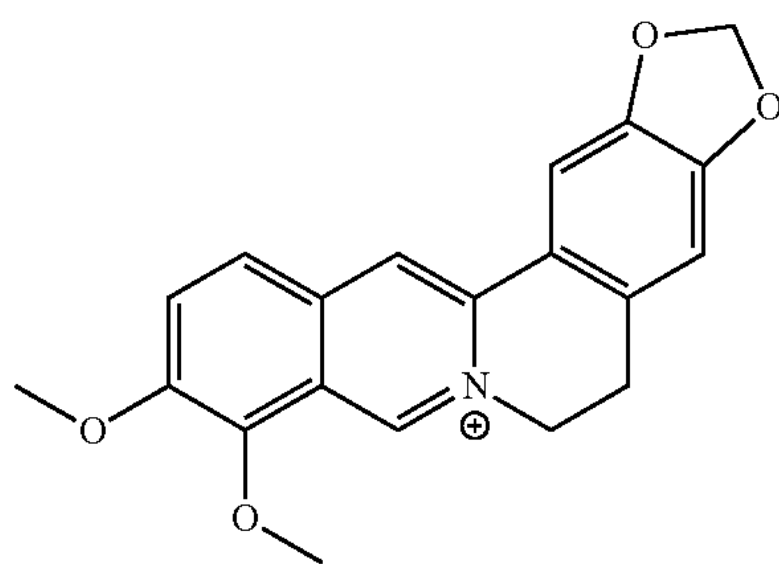
Berberine
