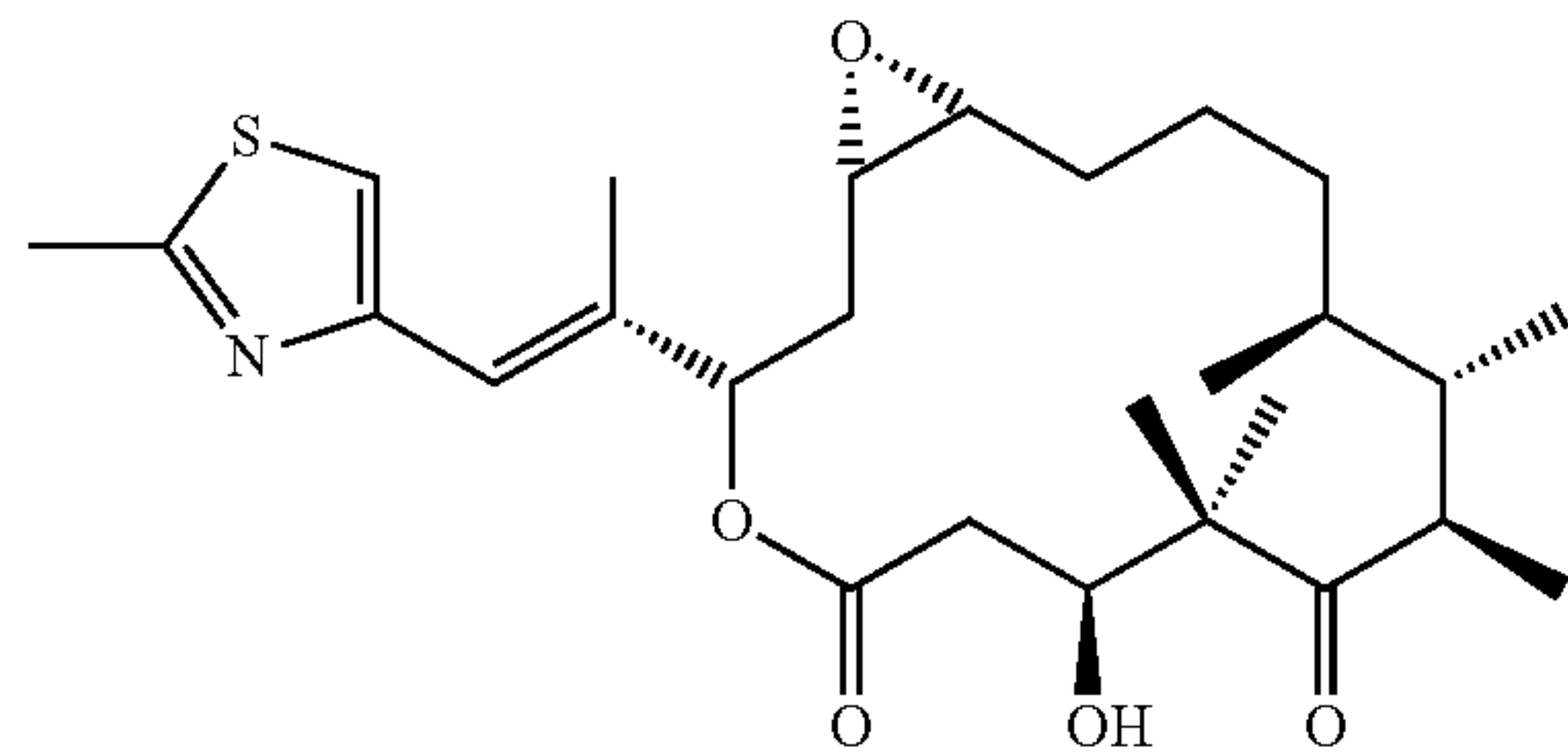
Epothilone A
