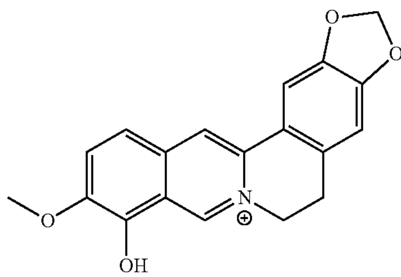
Berberrubine
