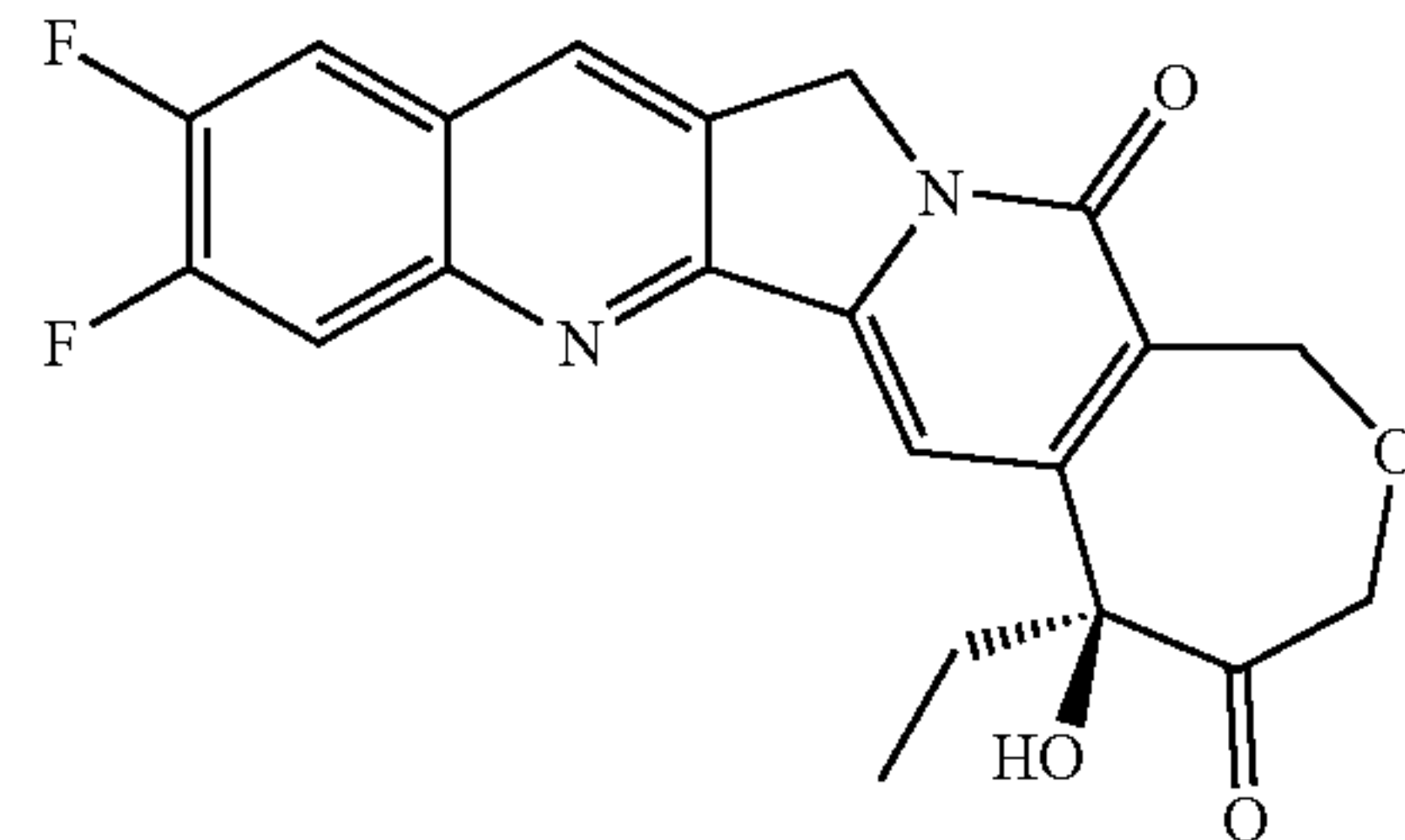
Diflomotecan
