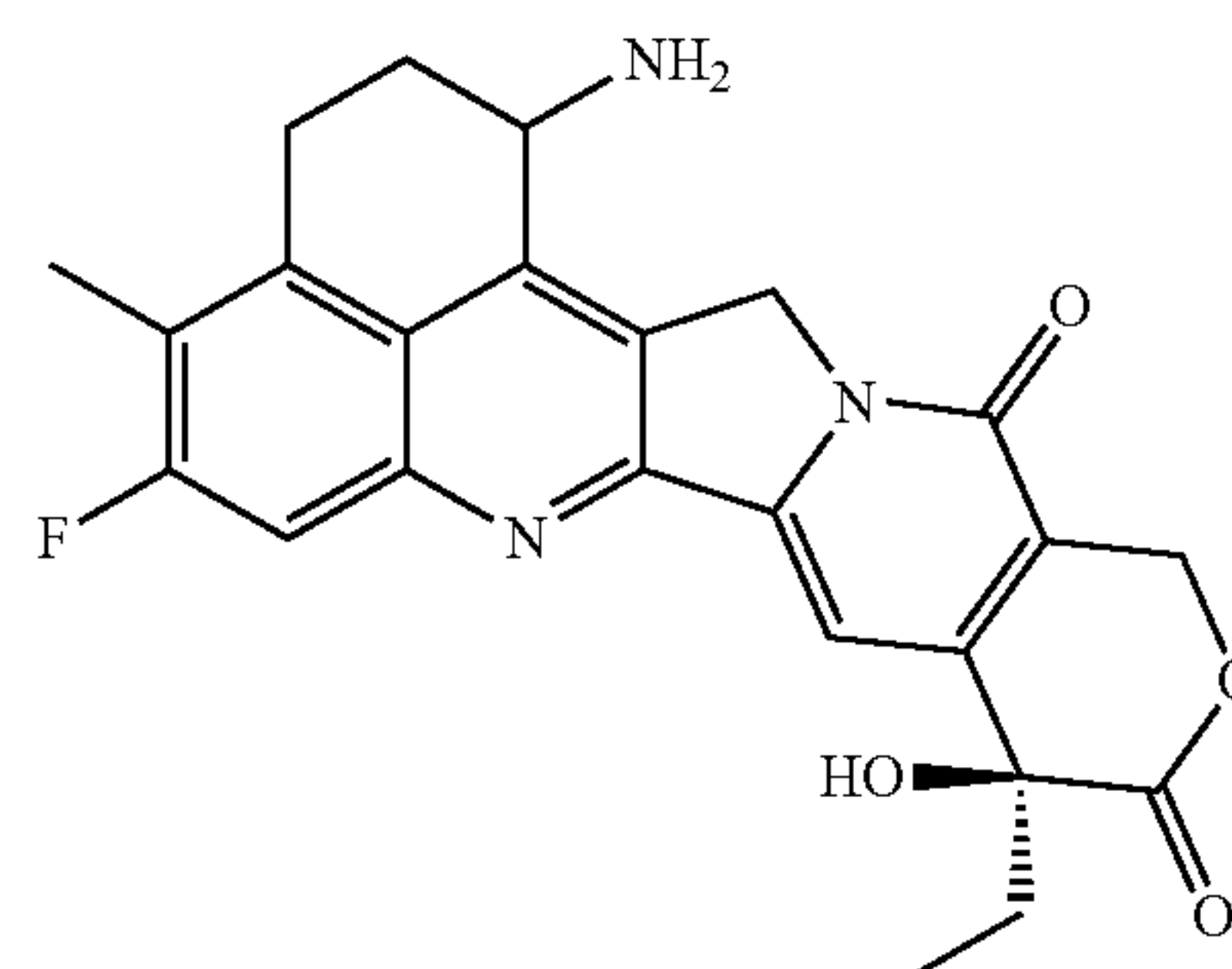
Exatecan
