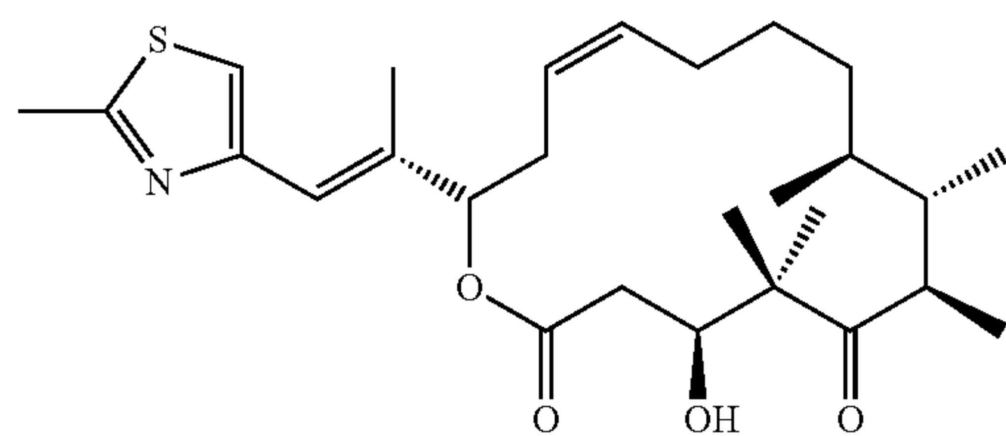
Epothilone C
