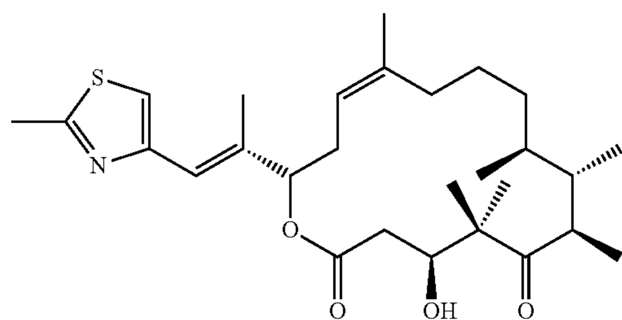
Epothilone D
