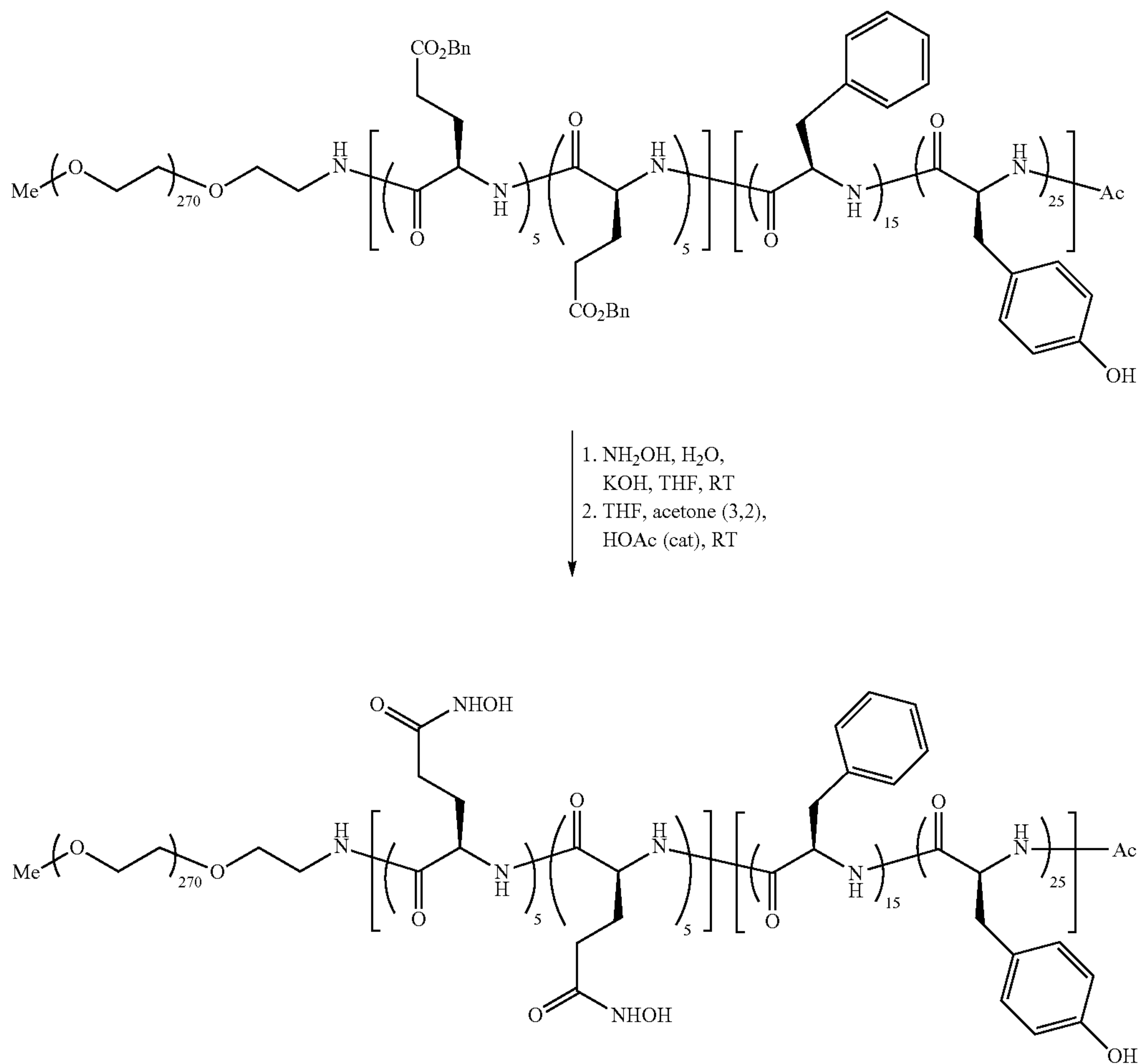
mPEG12K-b-Poly-[d-Glu(NHOH) 5 -co-Glu(NHOH) 5 ]-b-Poly-(Tyr(OH) 25 -co-d-Phe 15 )-Ac
