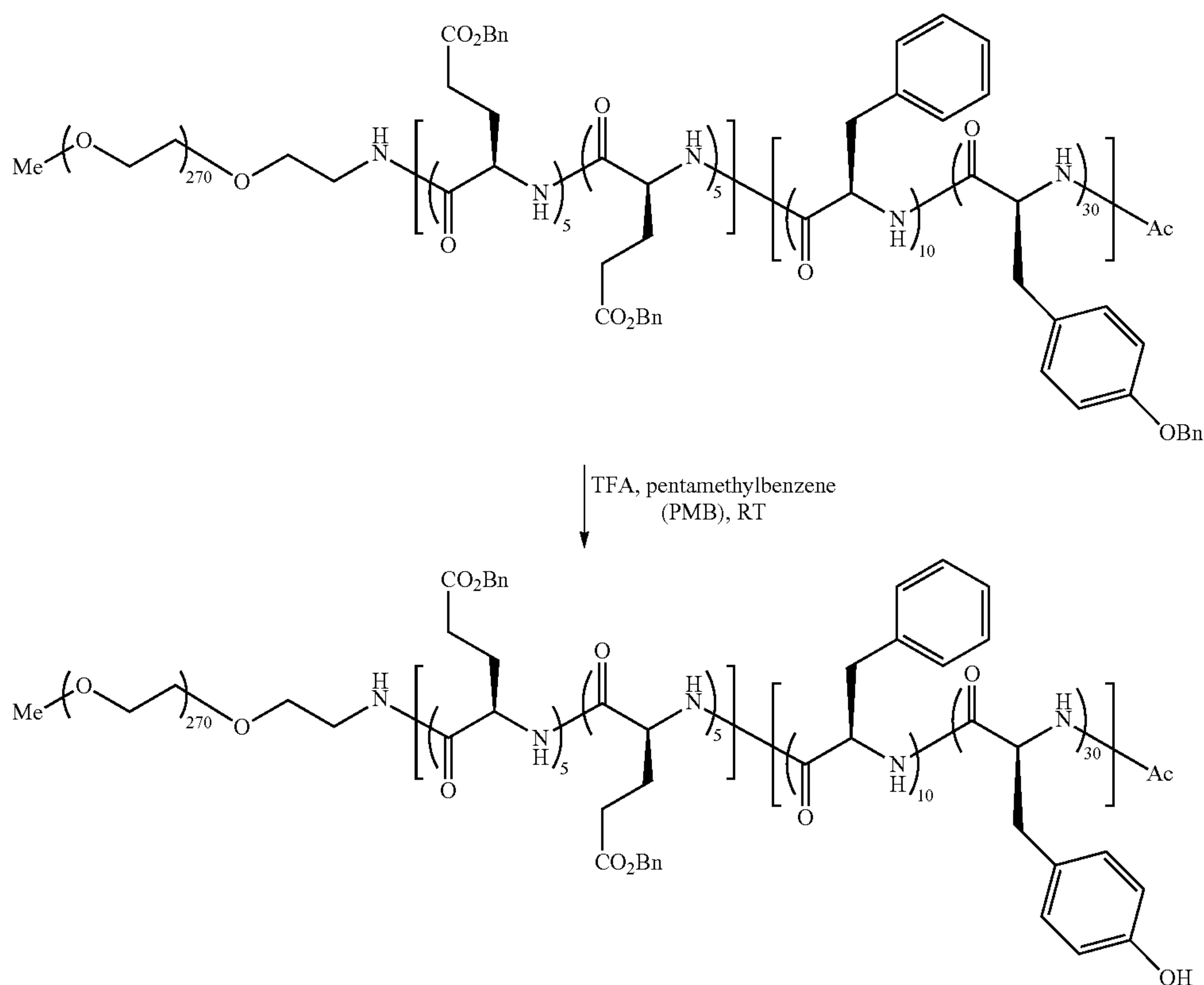
mPEG12K-b-Poly-[d-Glu(OBn) 5 -co-Glu(OBn) 5 ]-b-Poly-(Tyr(OH) 30 -co-d-Phe 10 )-Ac
