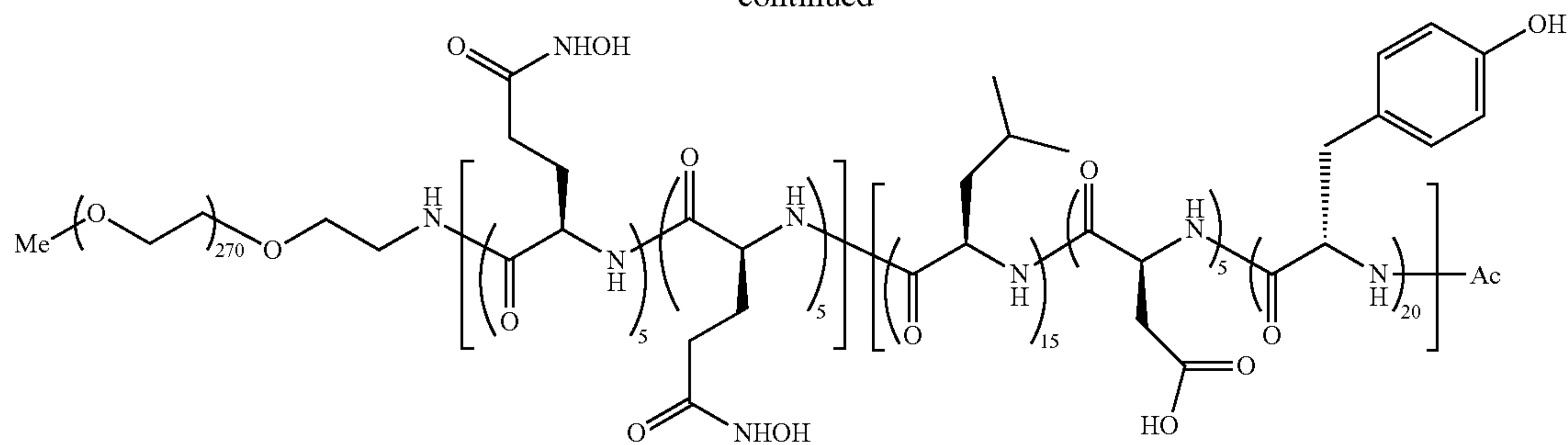
mPEG12K-b-Poly-(d-Glu(NHOH) 5 -co-Glu(NHOH) 5 )-b-Poly-(d-Leu 15 -co-Asp(OH) 5 -co-Tyr(OH) 20 )-Ac
