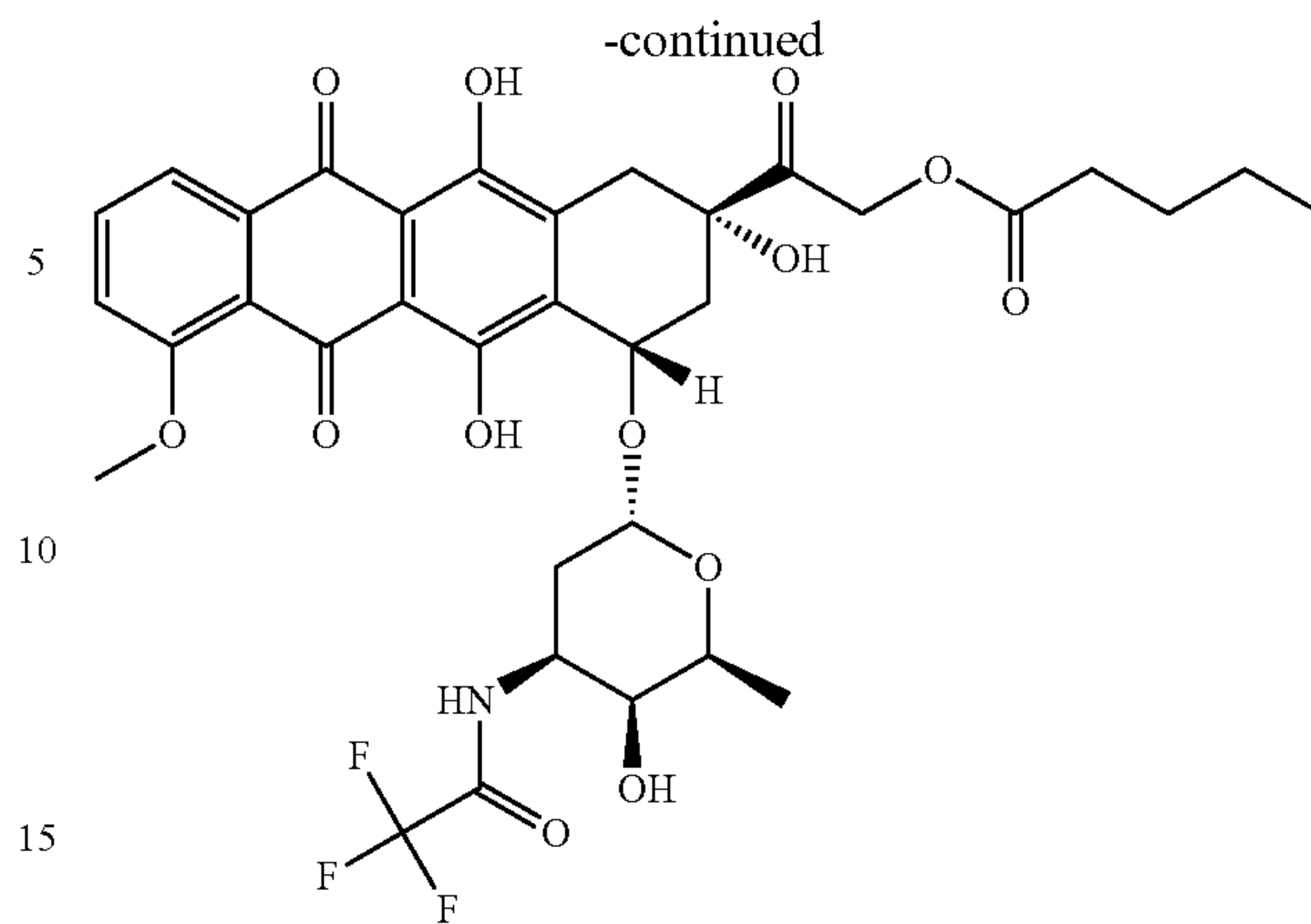
valrubicin
