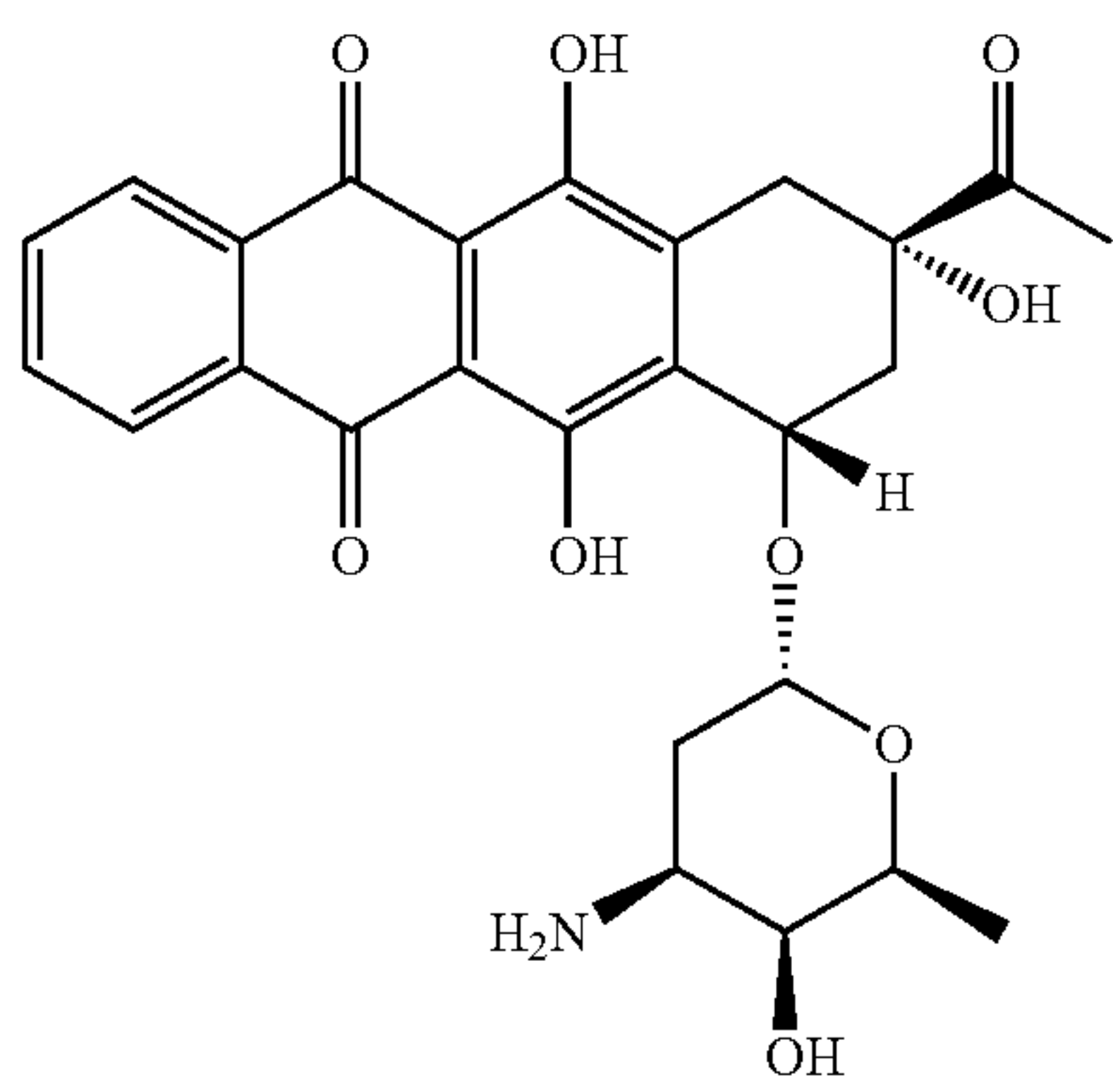
idarubicin
