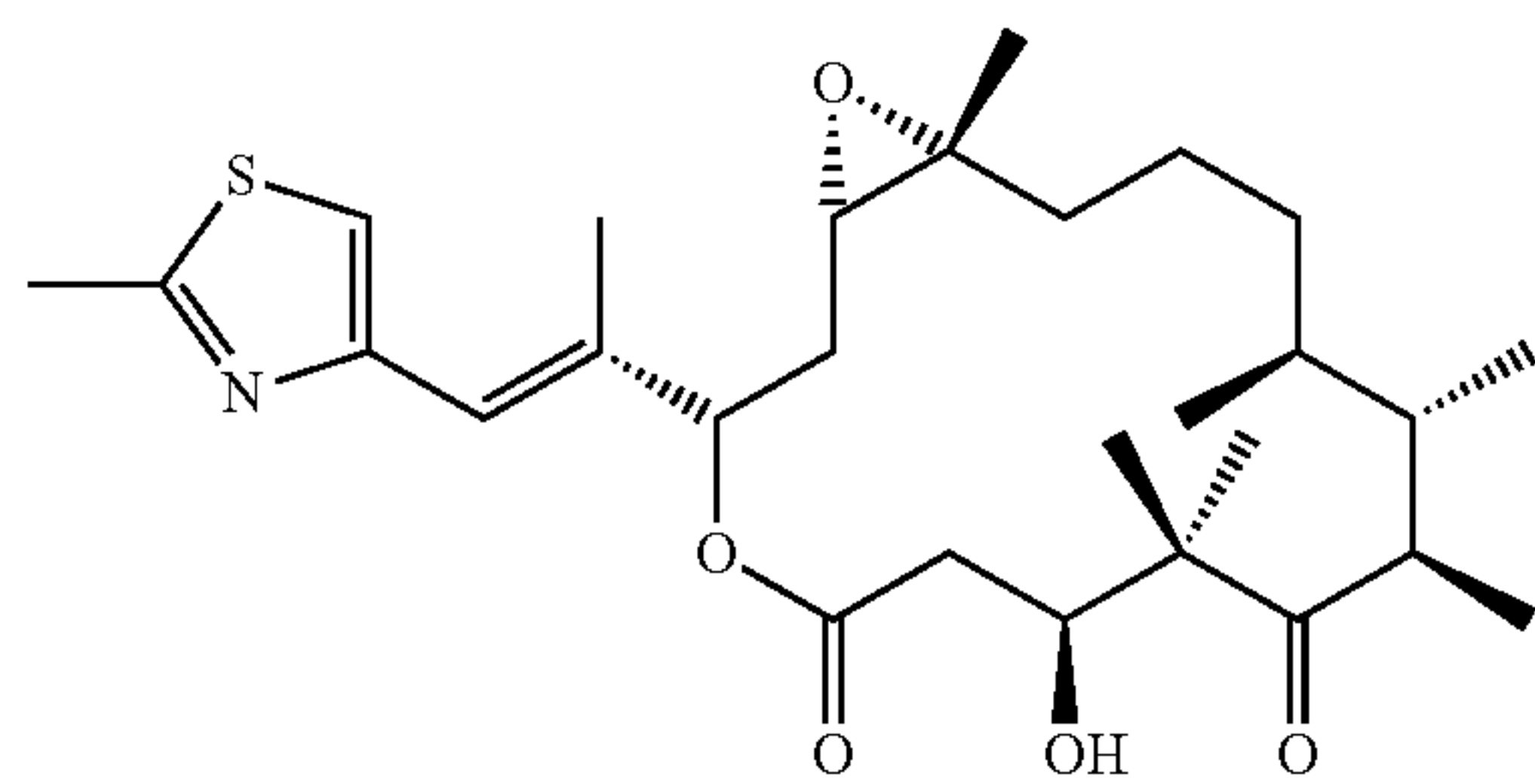
Epothilone B
