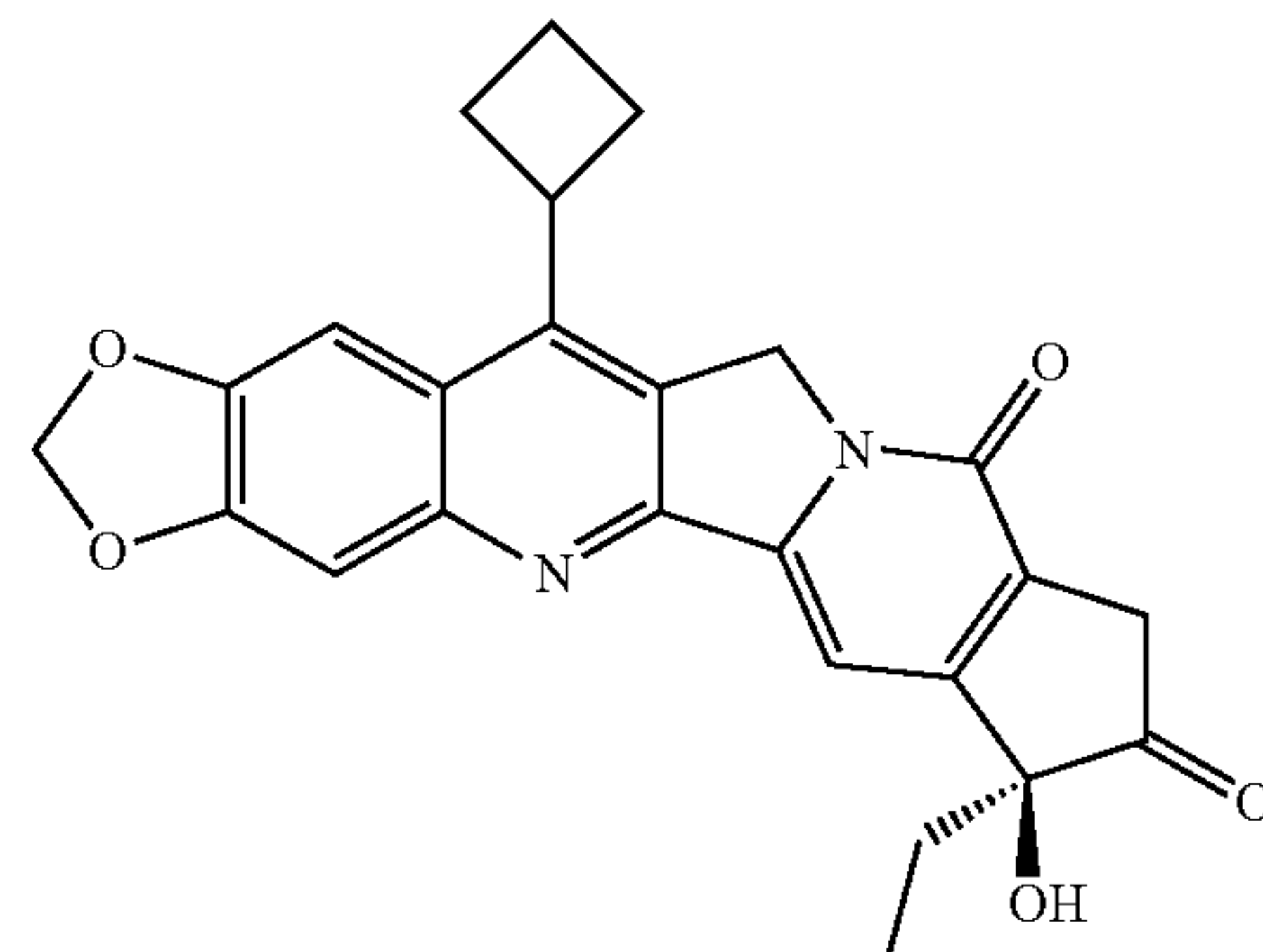
S39625
