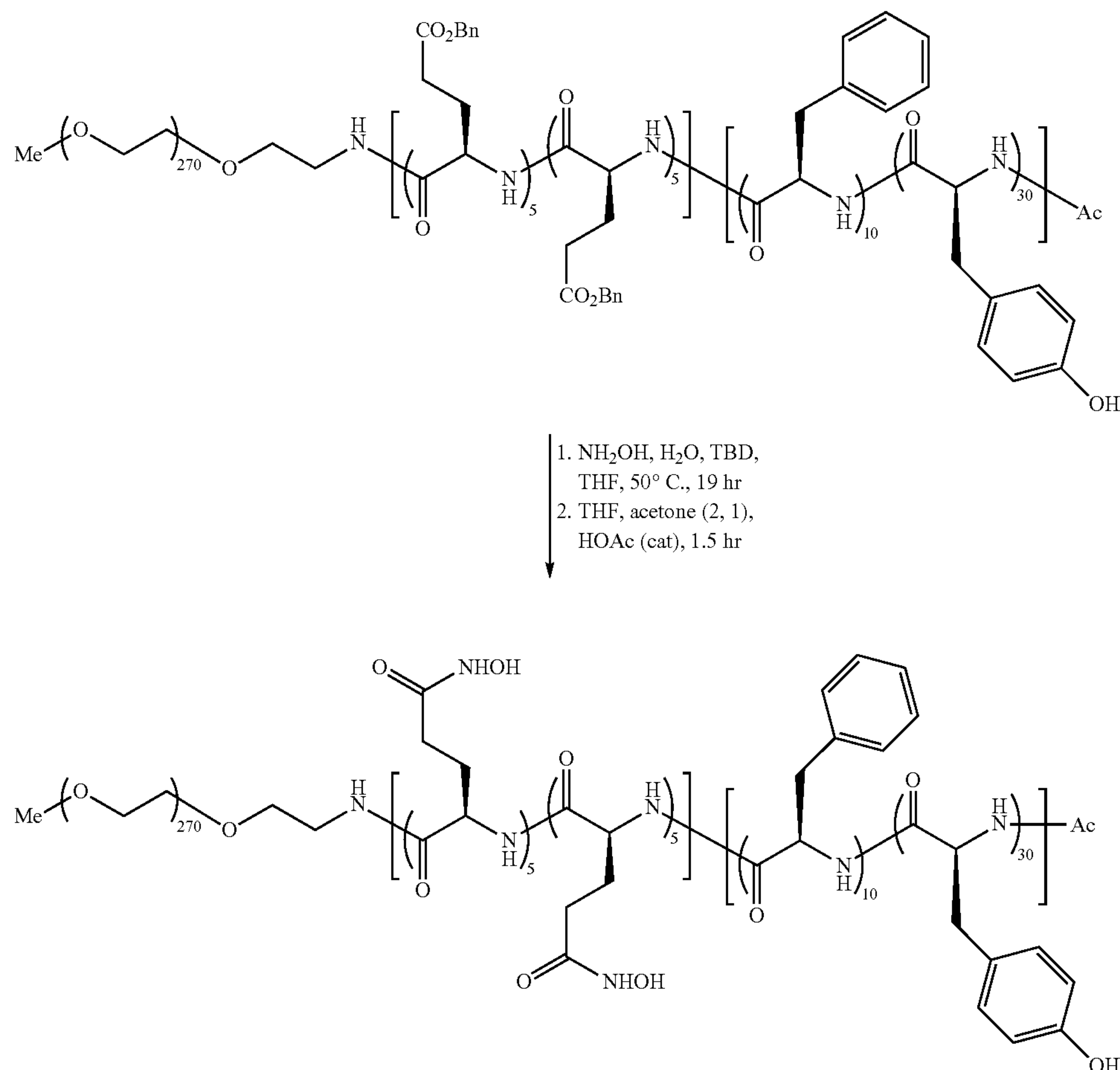
mPEG12K-b-Poly-[d-Glu(NHOH) 5 -co-Glu(NHOH) 5 ]-b-Poly-(Tyr(OH) 30 -co-d-Phe 10 )-Ac
