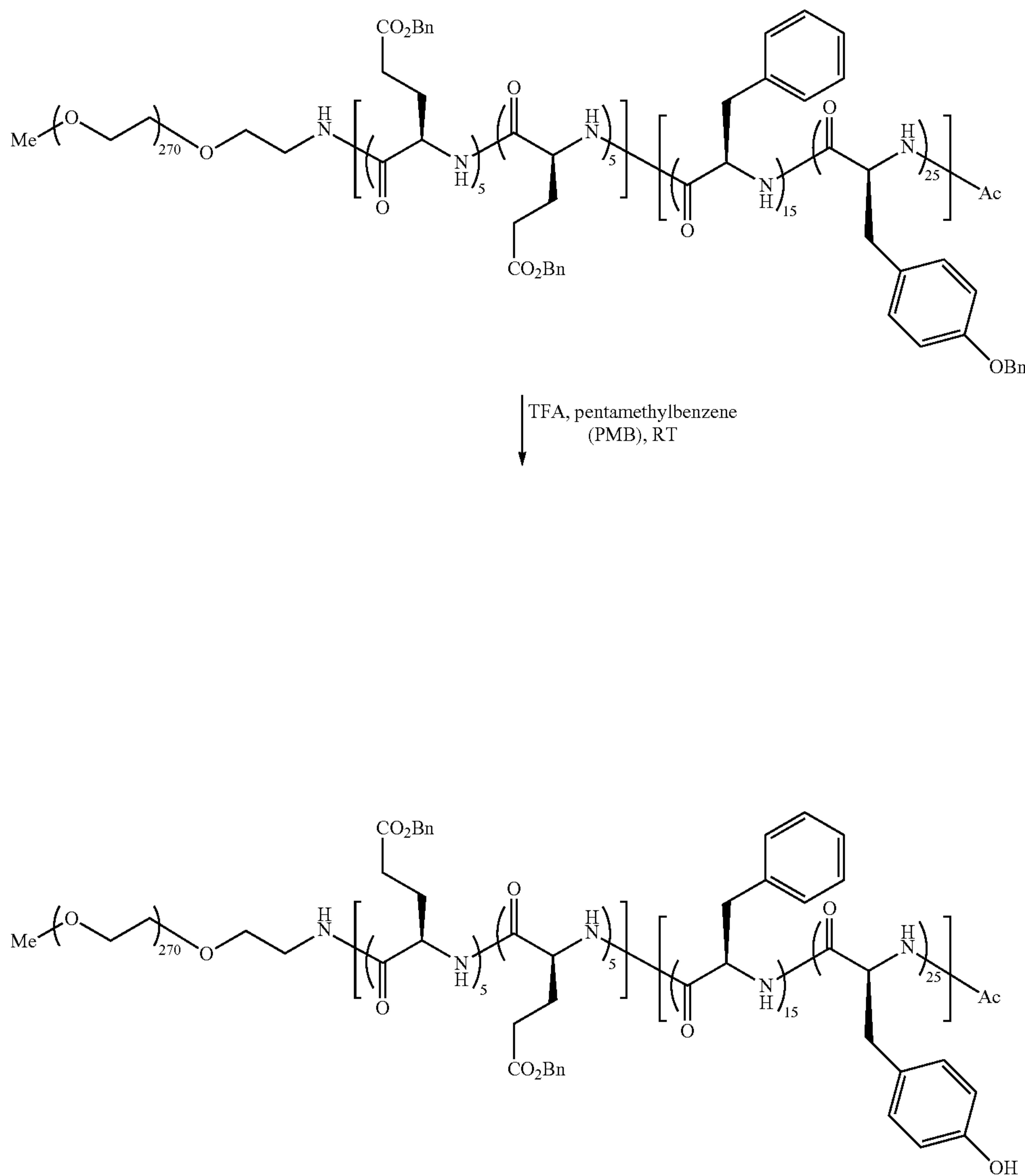
mPEG12K-b-Poly-[d-Glu(OBn) 5 -co-Glu(OBn) 5 ]-b-Poly-(Tyr(OH) 25 -co-d-Phe 15 )-Ac
