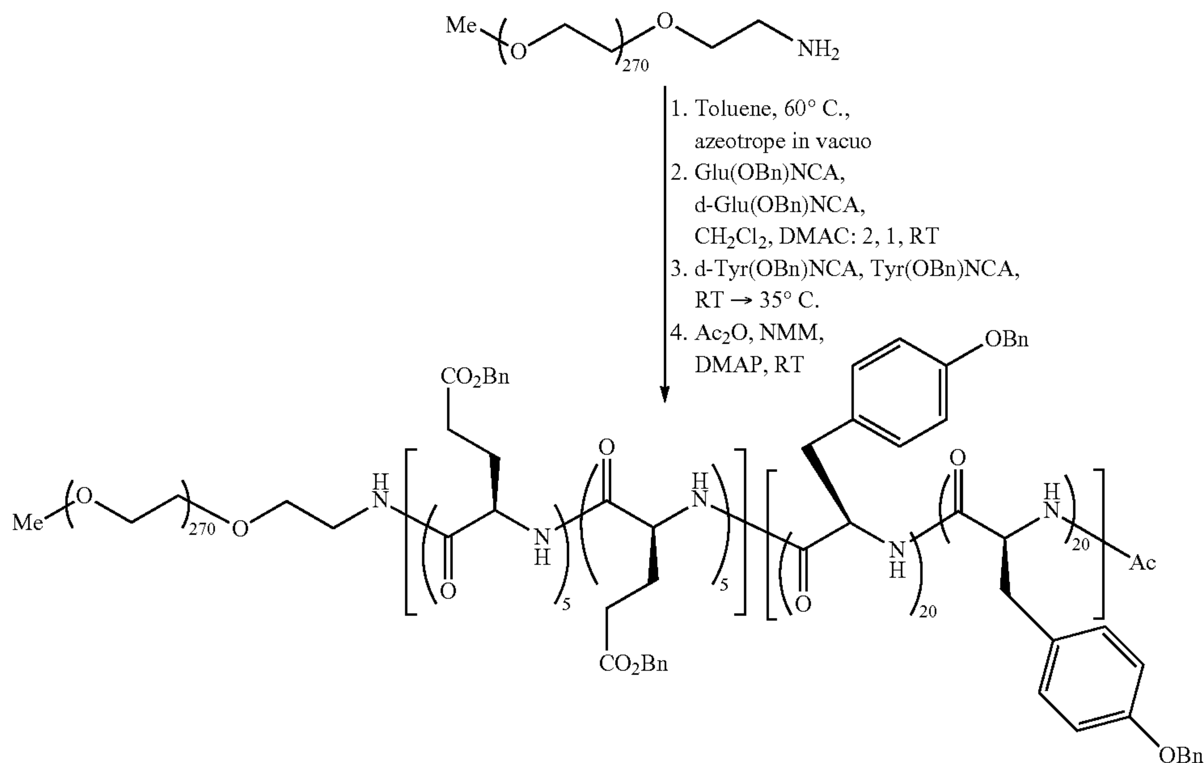
mPEG12K-b-Poly-(d-Glu(OBn) 5 -co-Glu(OBn) 5 )-b-Poly-(d-Tyr(OBn) 20 -co-Tyr(OBn) 20 )-Ac
