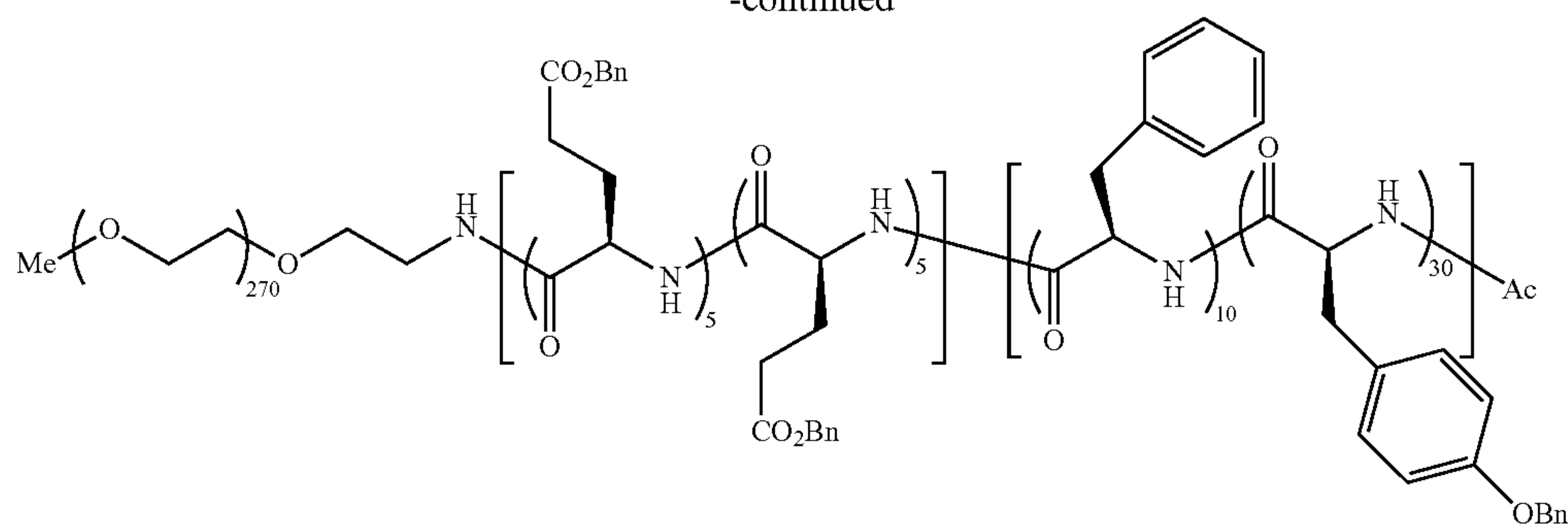
mPEG12K-b-Poly-(d-Glu(OBn) 5 -co-Glu(OBn) 5 -b-Poly (Tyr(OBn) 30 -co-d-Phe 10 )-Ac
