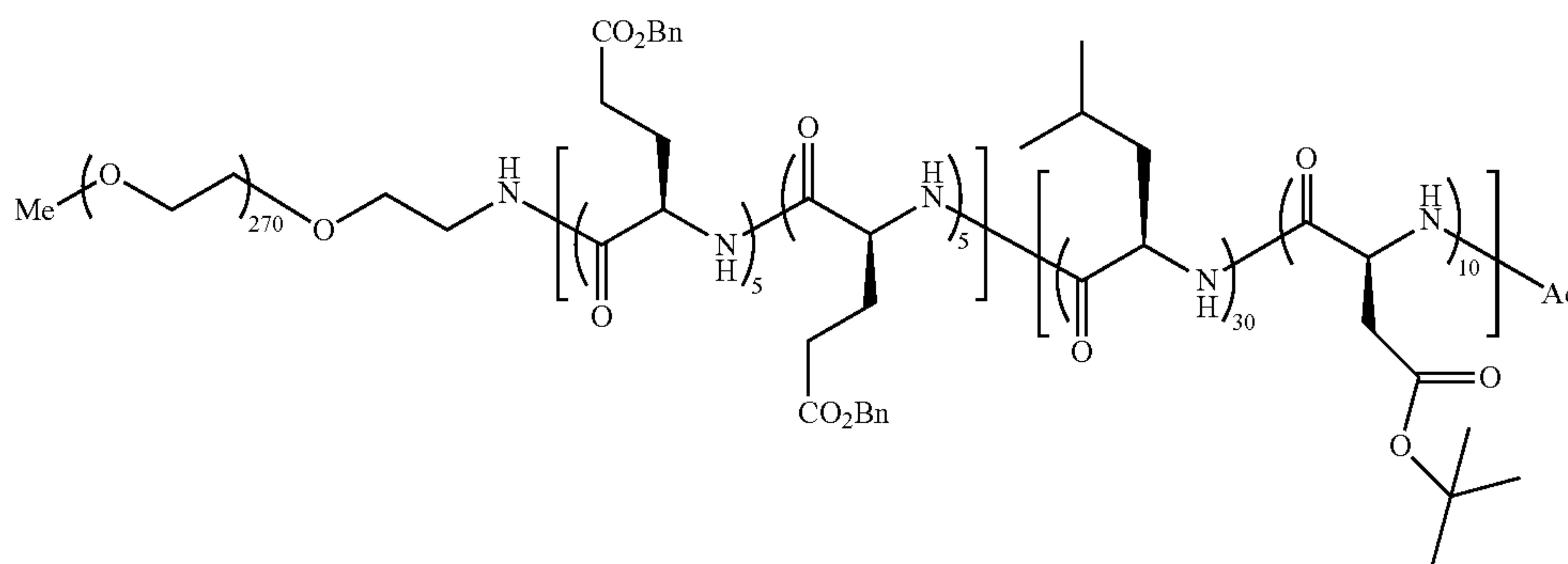
mPEG12K-b-Poly-(d-Glu(OBn) 5 -co-Glu(OBn) 5 )-b-Poly(d-Leu 30 -co-Asp(OtBu) 10 )-Ac
