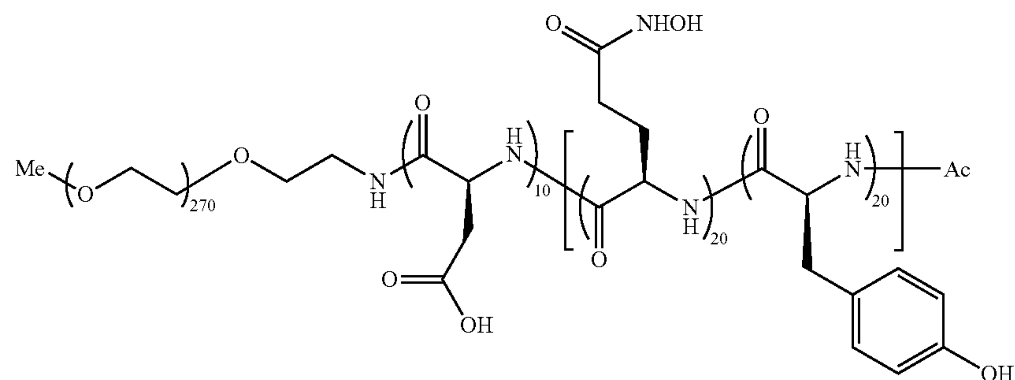
mPEG12K-b-Poly-(Asp(OH) 10 -b-Poly-(Tyr(OH) 20 -co-d-Glu(NHOH) 20 -Ac
