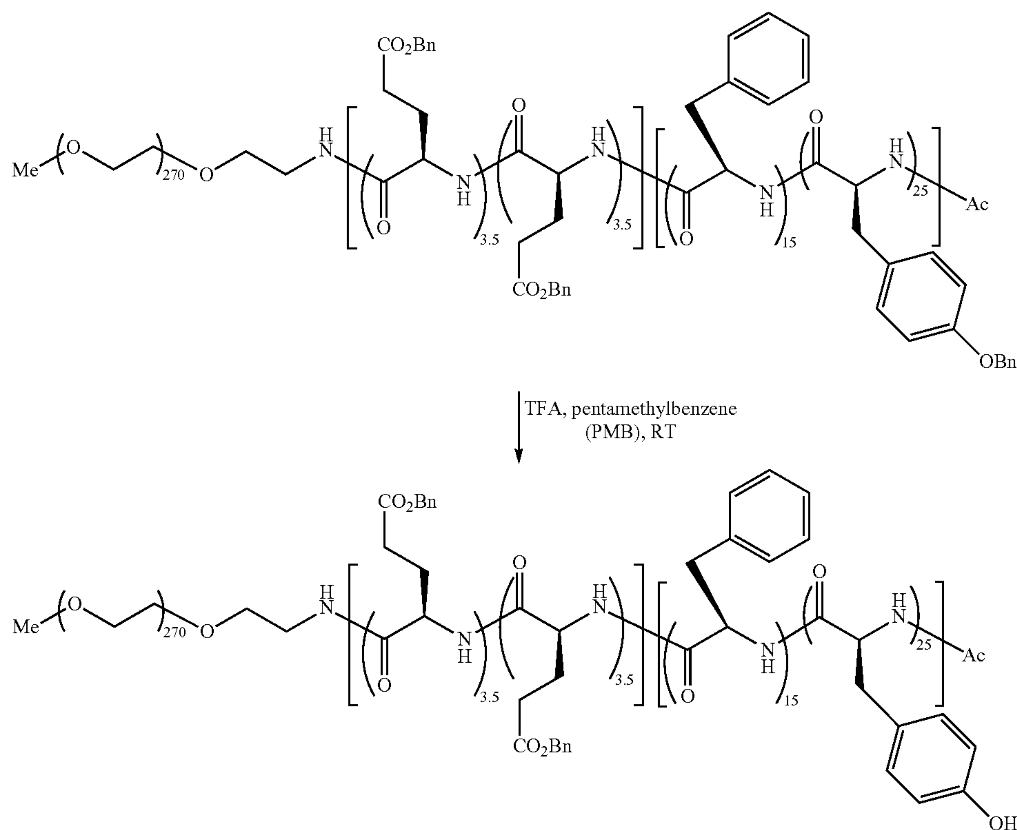
mPEG12K-b-Poly-[d-Glu(OBn) 3.5 -co-Glu(OBn) 3.5 ]-b-Poly-(Tyr(OH) 25 -co-d-Phe 15 )-Ac
