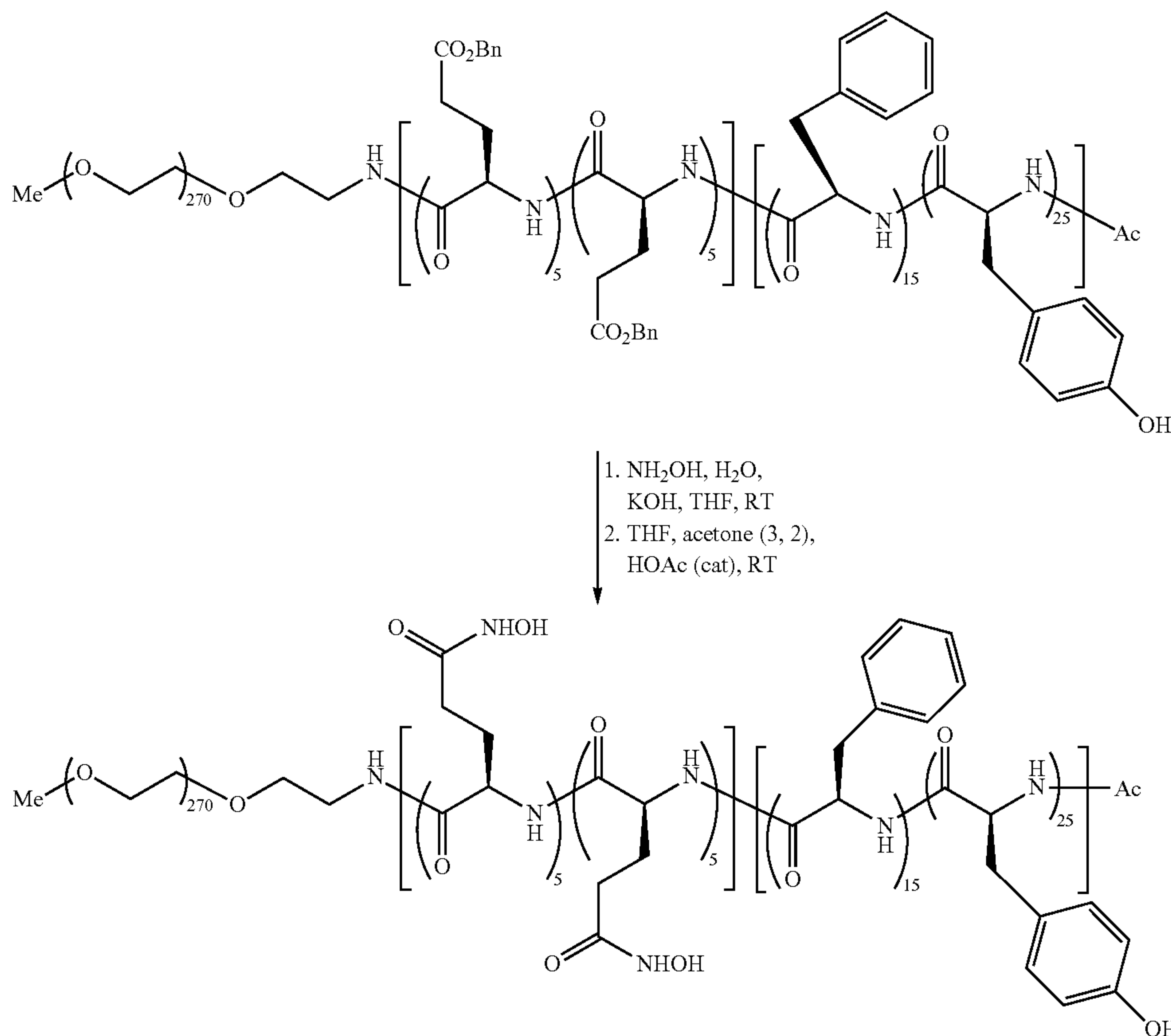
mPEG12K-b-Poly-[d-Glu(NHOH) 5 -co-Glu(NHOH) 5 ]-b-Poly-(Tyr(OH) 25 -co-d-Phe 15 )-Ac
