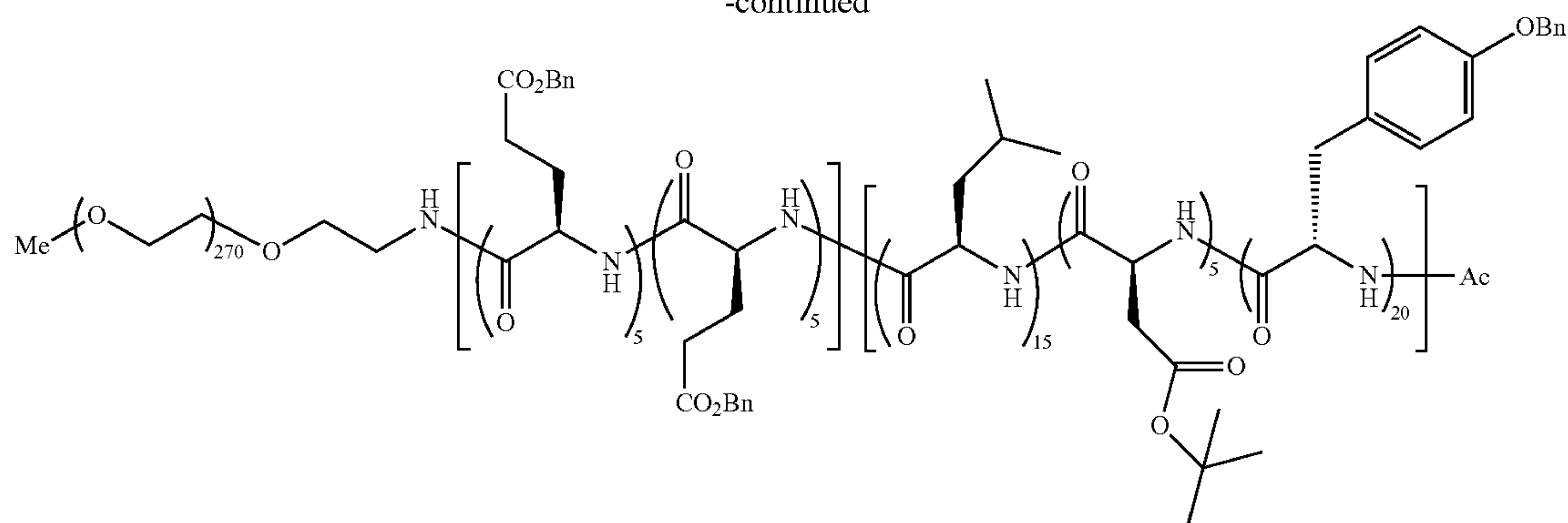
mPEG12K-b-Poly-(d-Glu(OBn) 5 -co-Glu(OBn) 5 )-b-Poly(d-Leu 15 -co-Asp(OtBu) 5 -co-Tyr(OBn) 20 )-Ac
