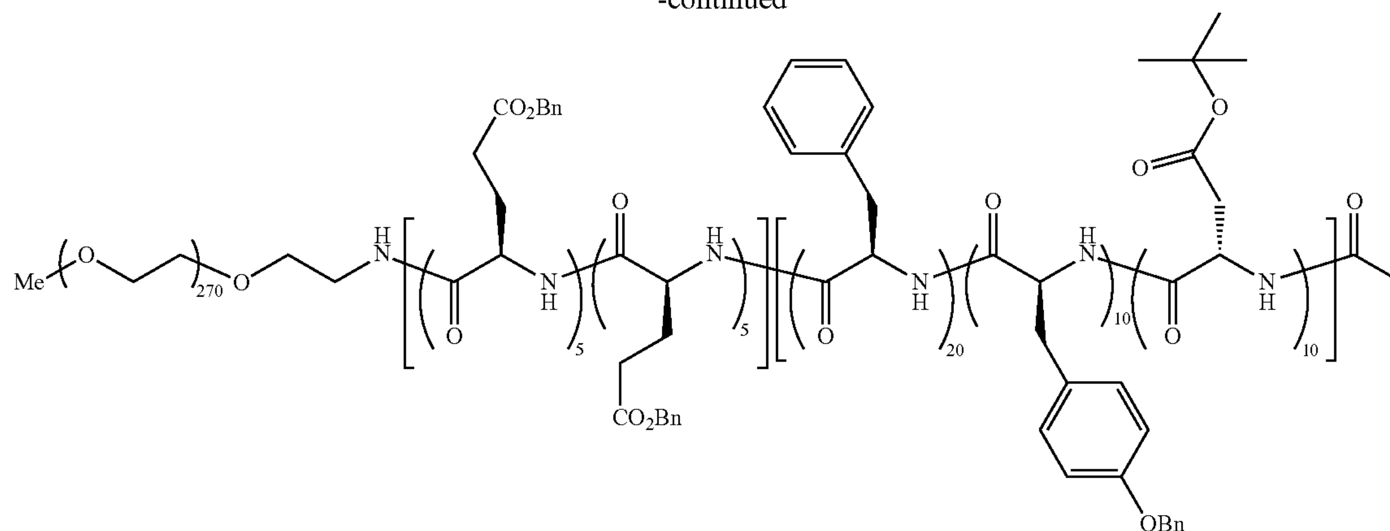
mPEG12K-b-Poly-(d-Glu(OBn) 5 -co-Glu(OBn) 5 )-b-Poly (Tyr(OBn) 10 -co-d-Phe 20 -co-Asp(oTbu) 10 -Ac
