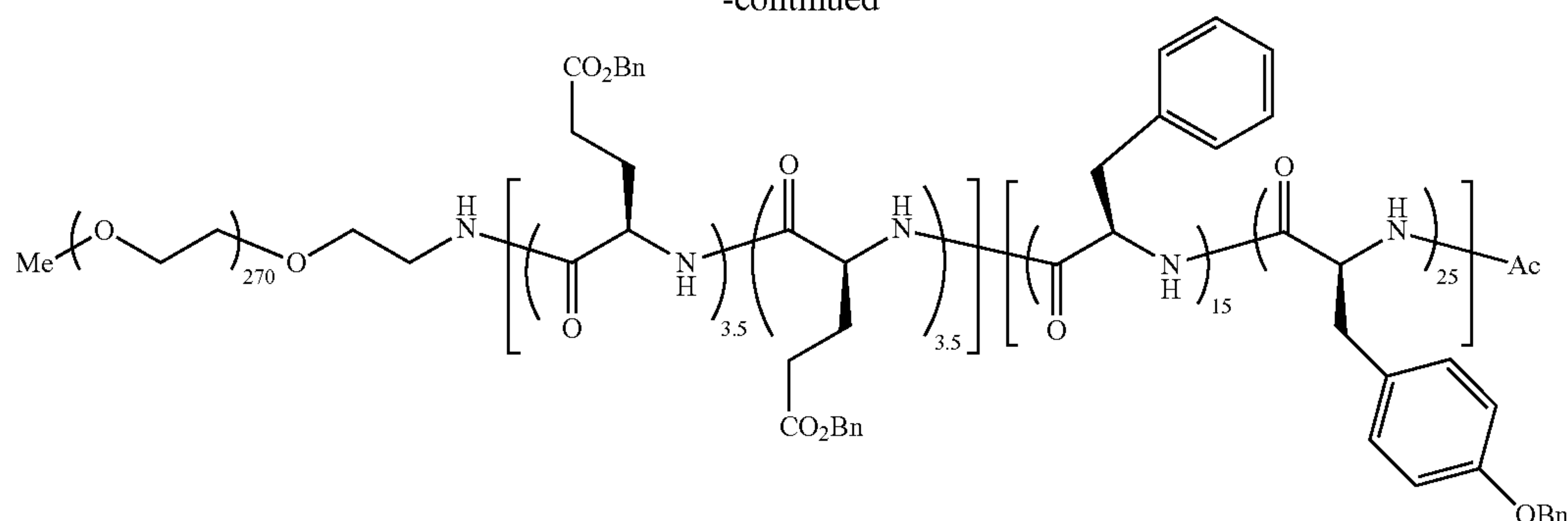
mPEG12K-b-Poly-(d-Glu(OBn) 3.5 -co-Glu(OBn) 3.5 )-b-Poly-(Tyr(OBn) 25 -co-d-Phe 15 )-Ac
