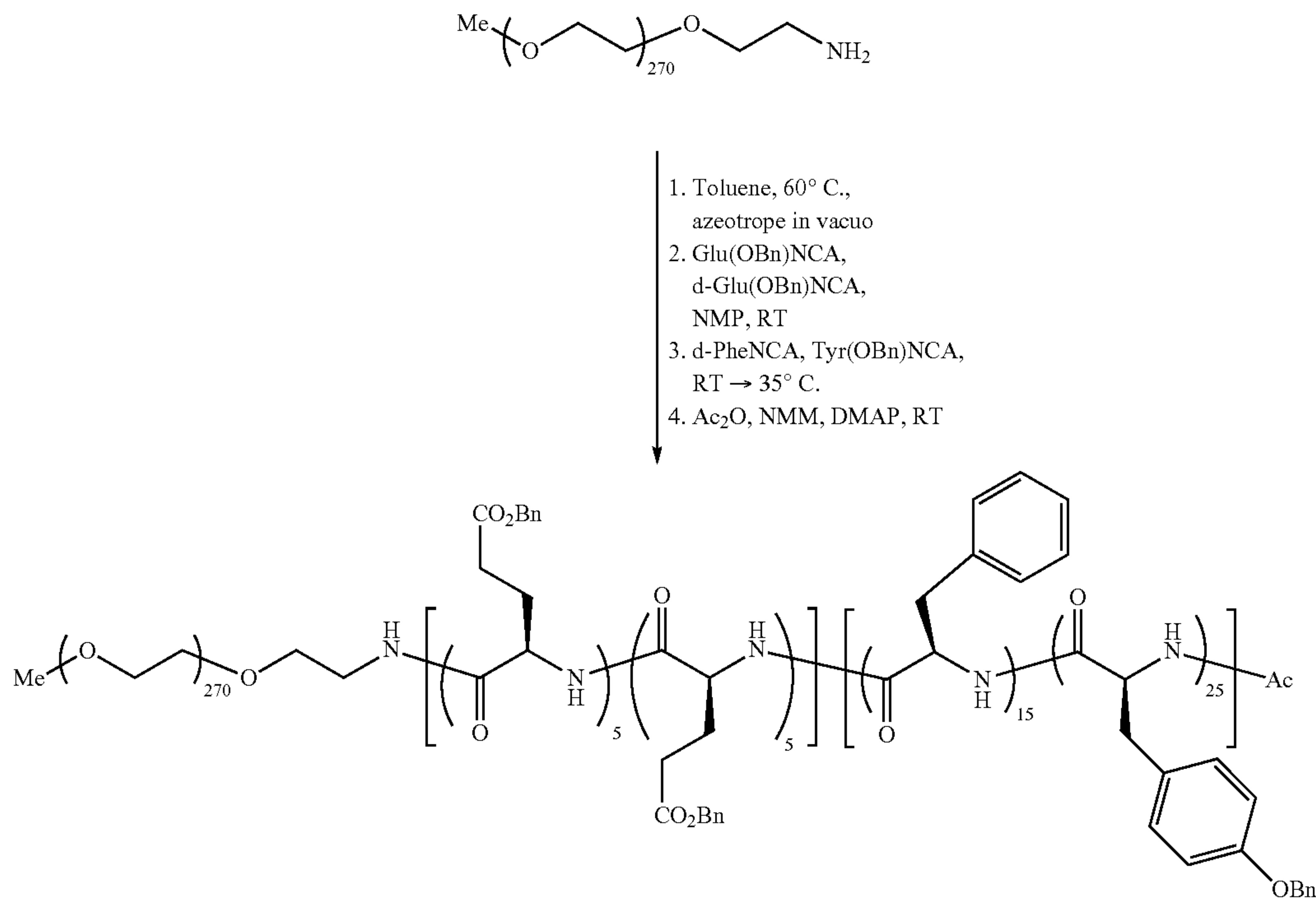
mPEG12K-b-Poly-(d-Glu(OBn) 5 -co-Glu(OBn) 5 )-b-Poly-(Tyr(OBn) 25 -co-d-Phe 15 )-Ac
