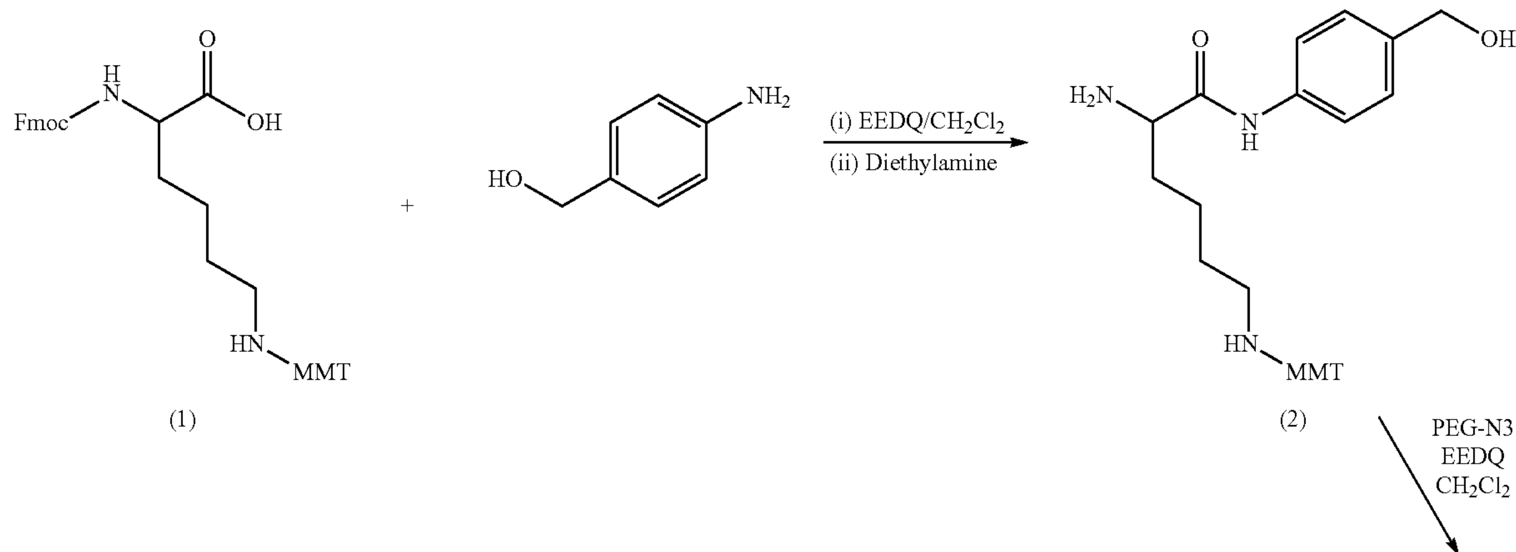
Scheme-3: Preparation of CL2A-SN-38
