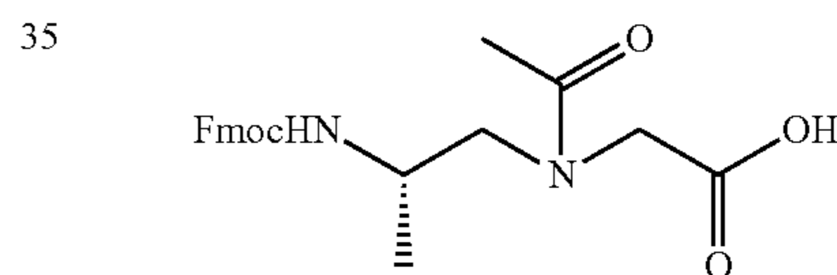
Compound B2:
