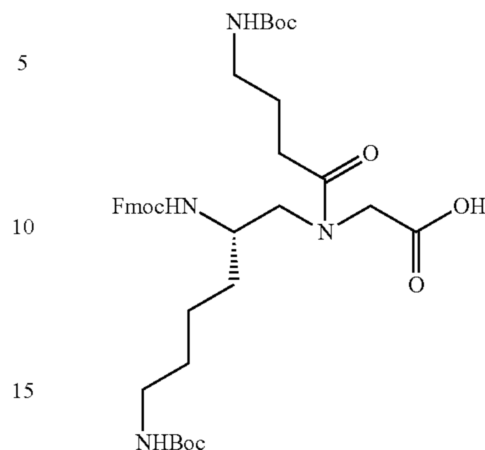
Compound B1:
