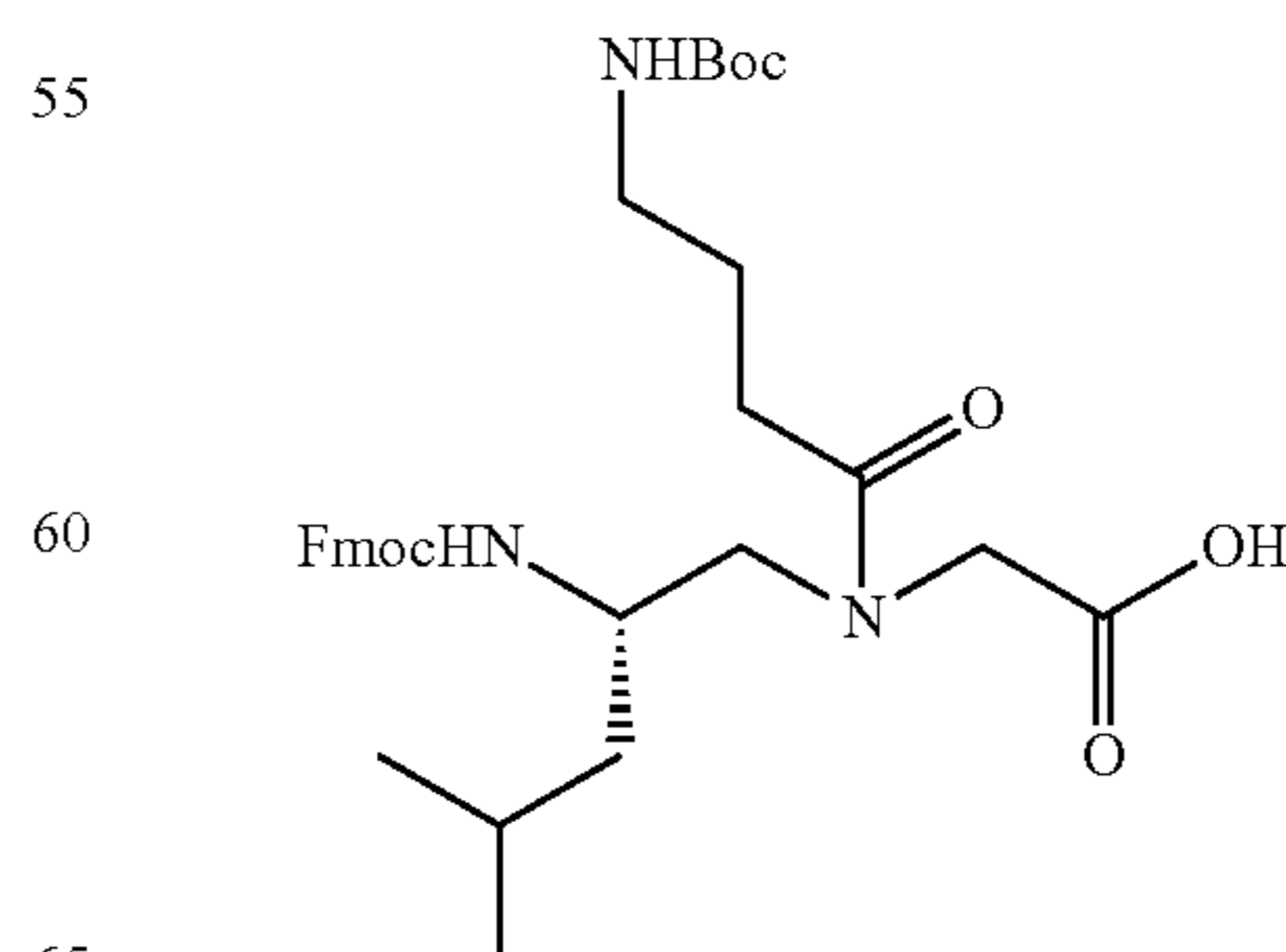
Compound B3:
