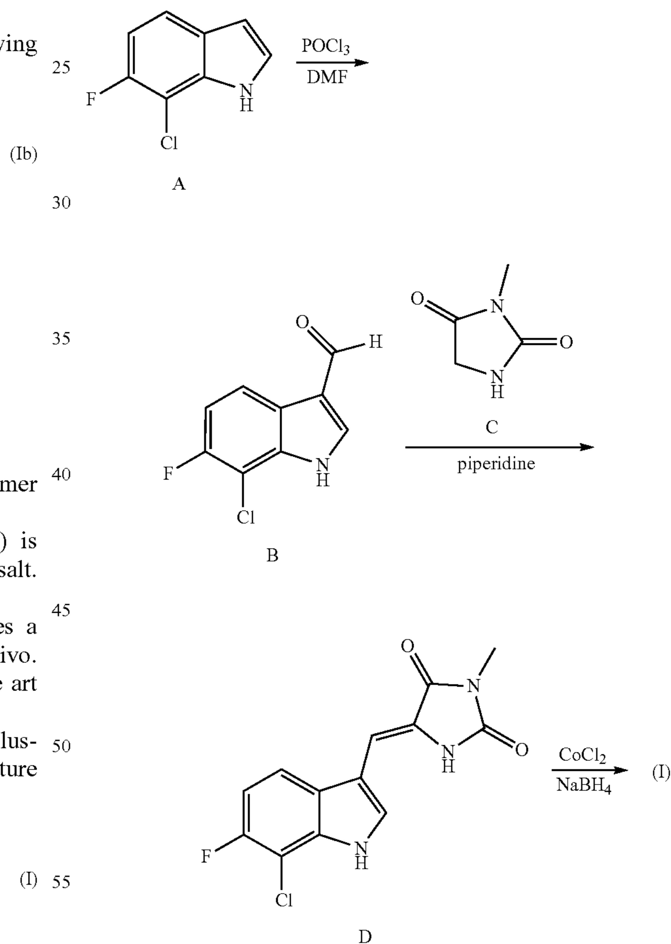
General Reaction Scheme I
