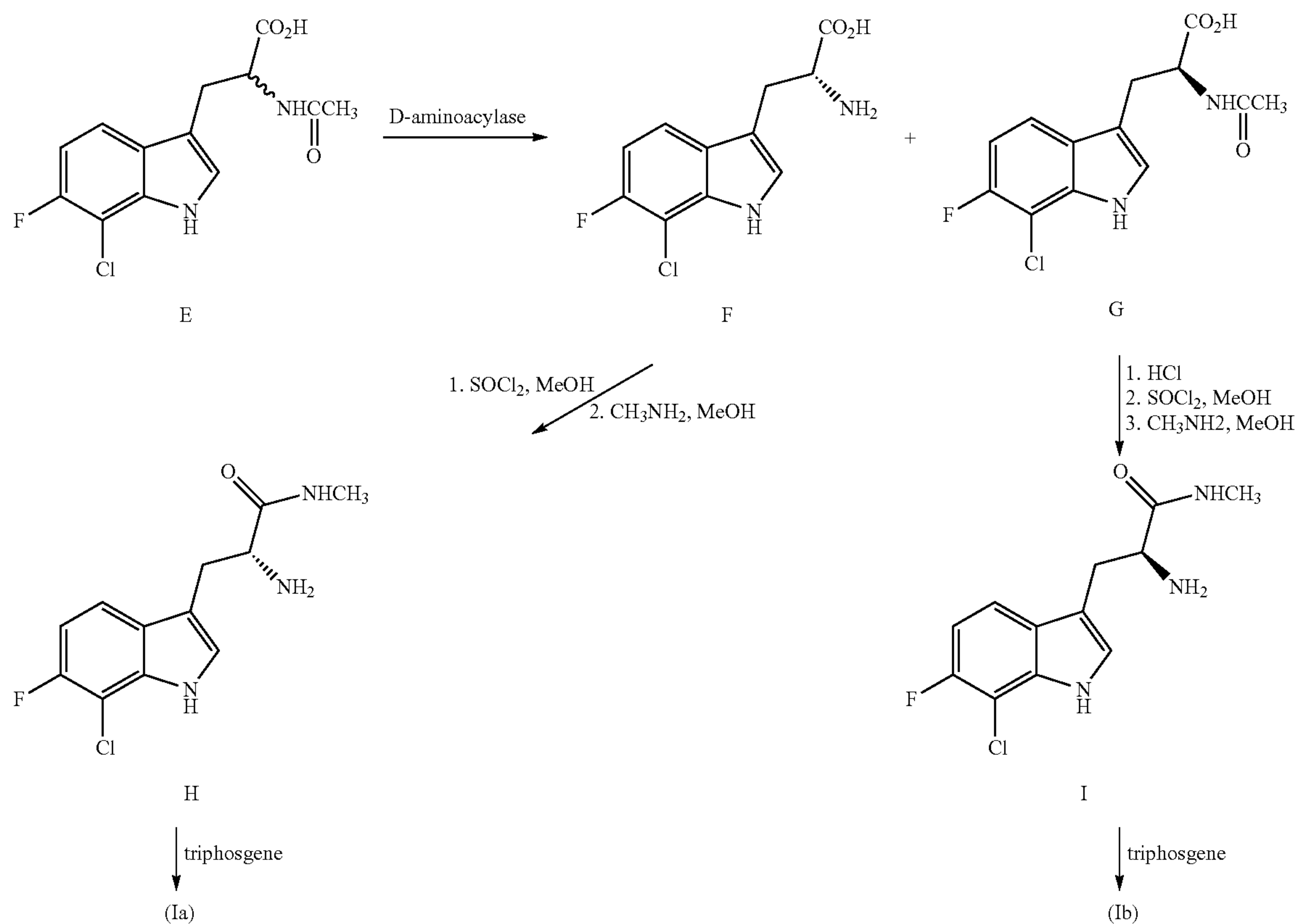
General Reaction Scheme II
