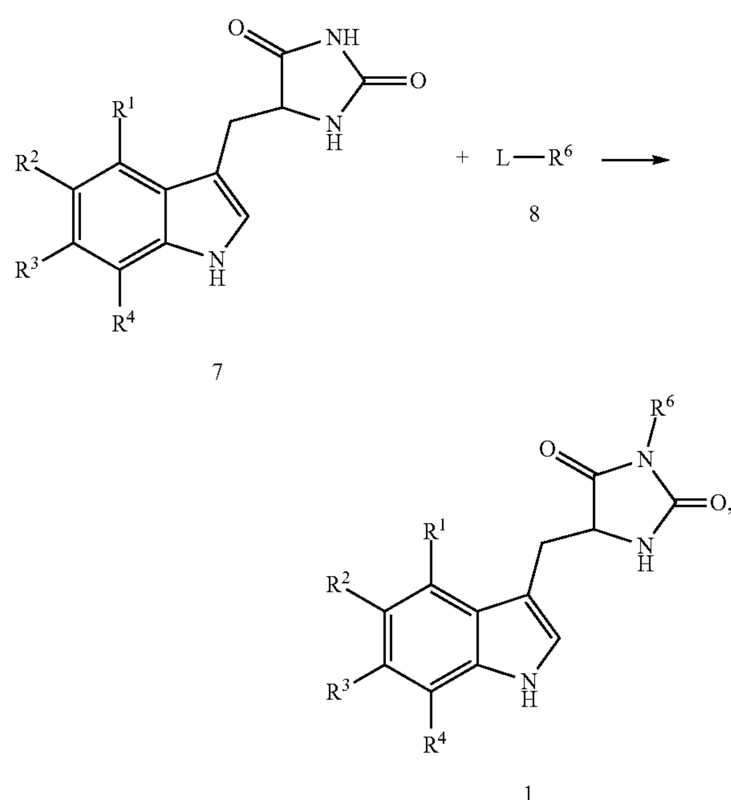
Reaction Scheme 2
