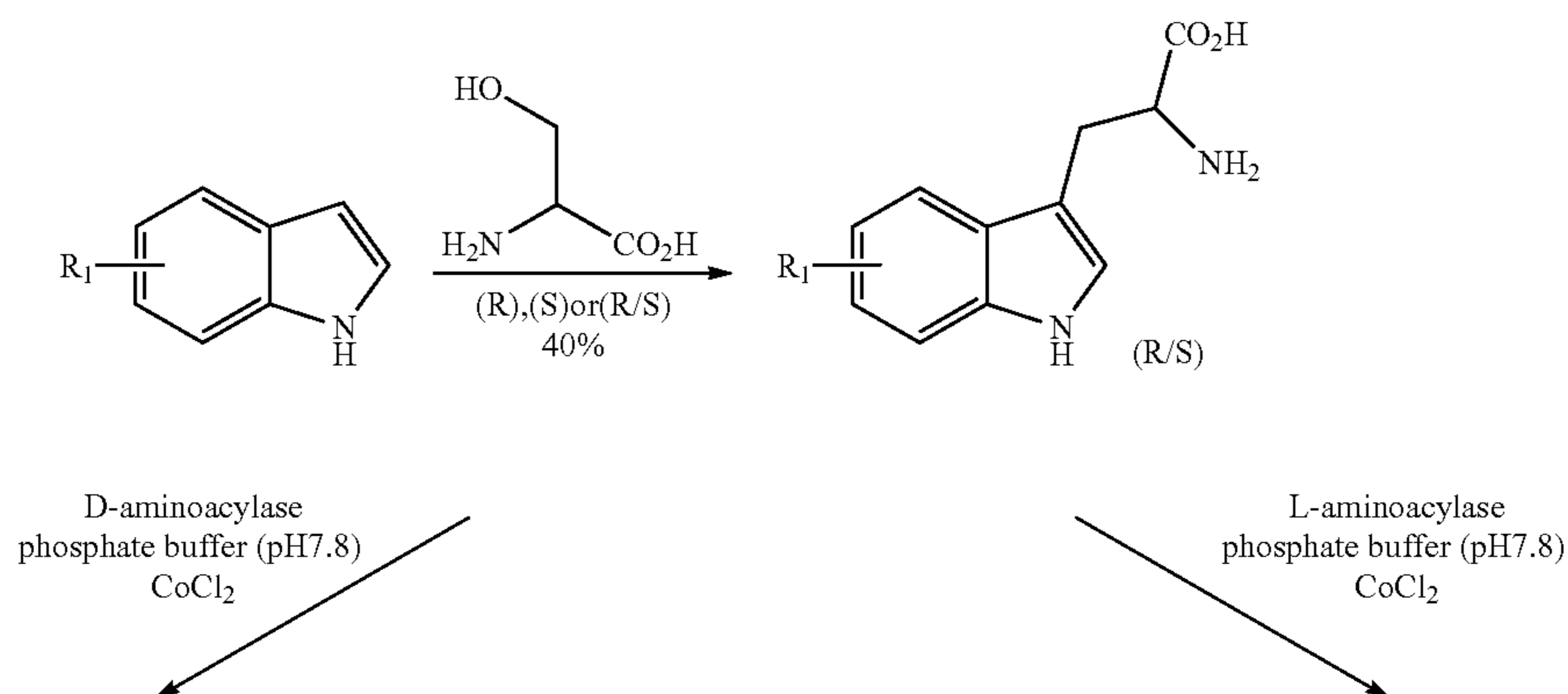
Comparative Reaction Scheme 3
