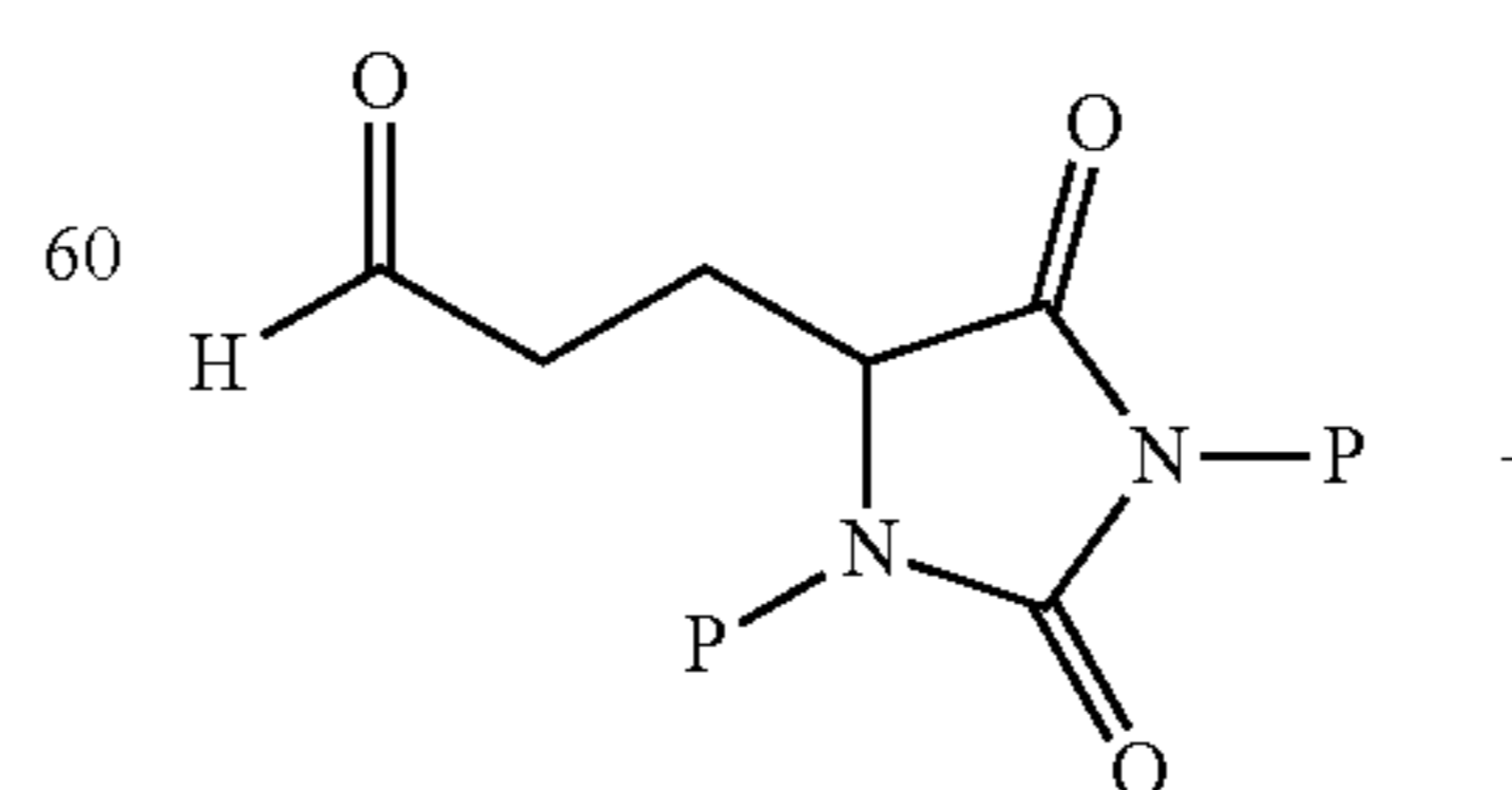
Reaction Scheme 1
