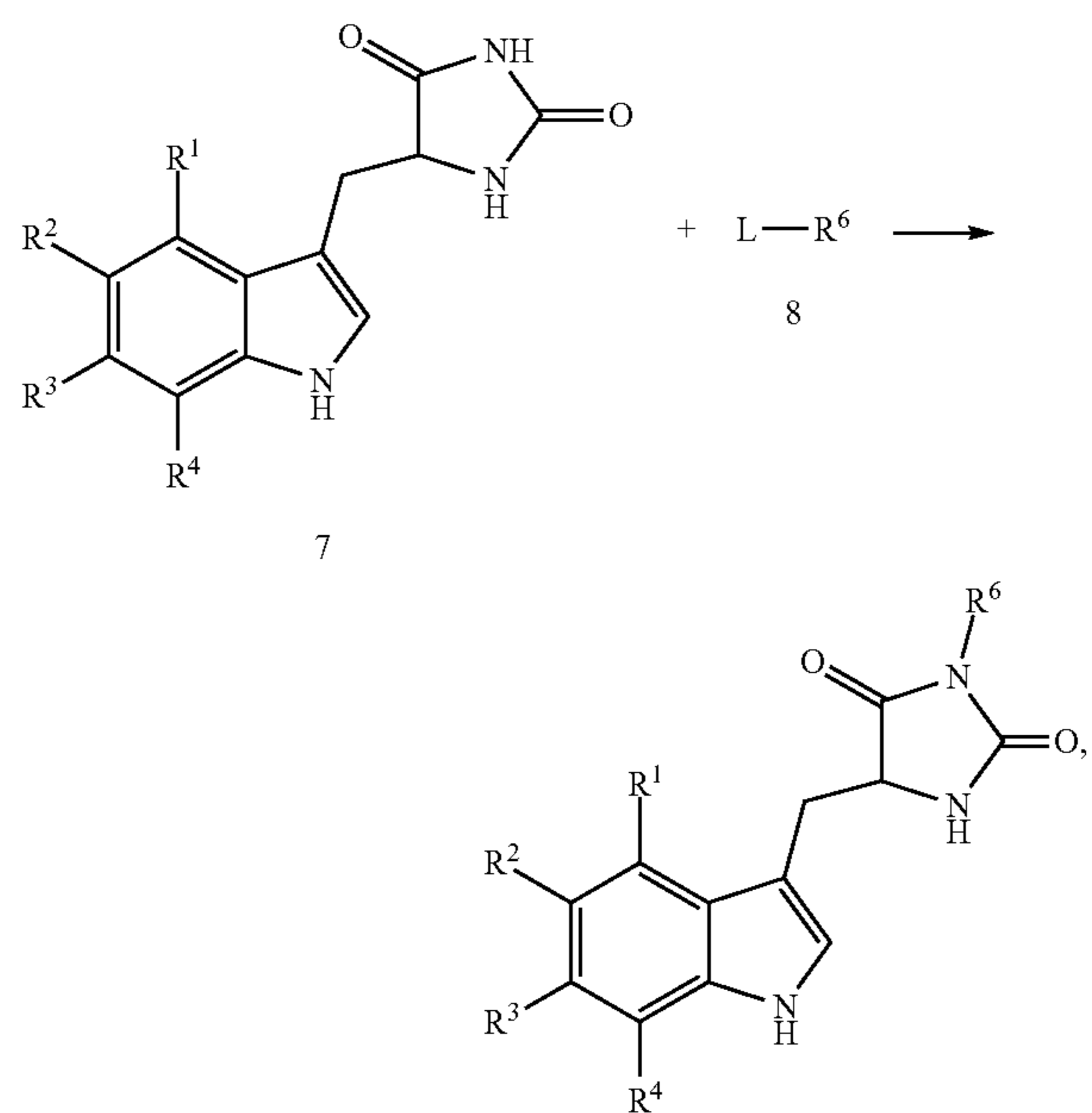
Reaction Scheme 2
