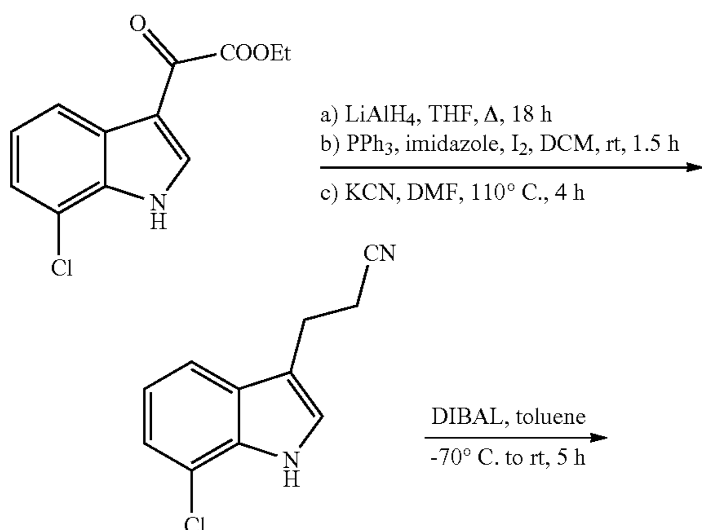
Comparative Reaction Scheme 2
