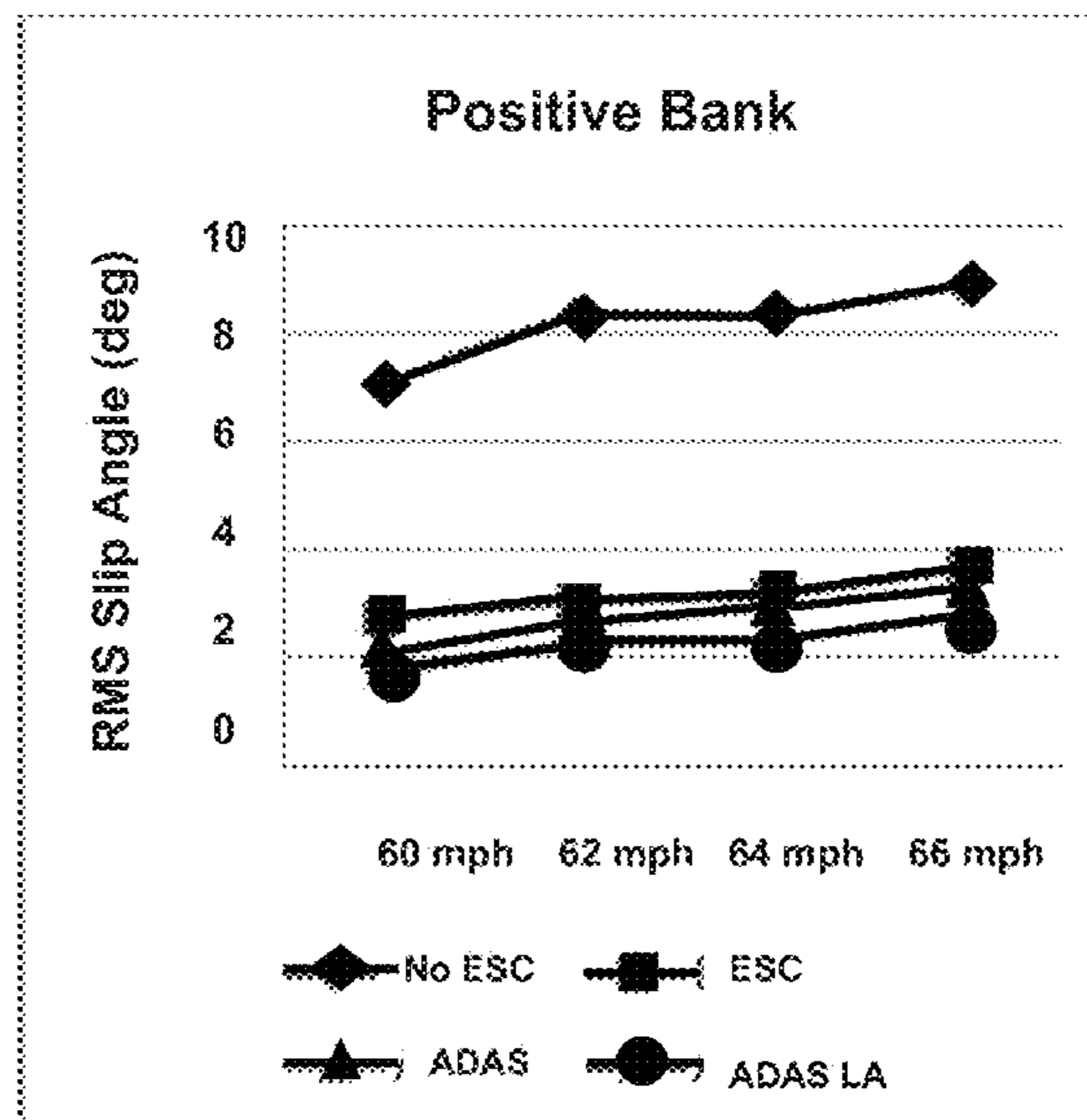
RMS SLIP ANGLE, POSITIVE BANK
