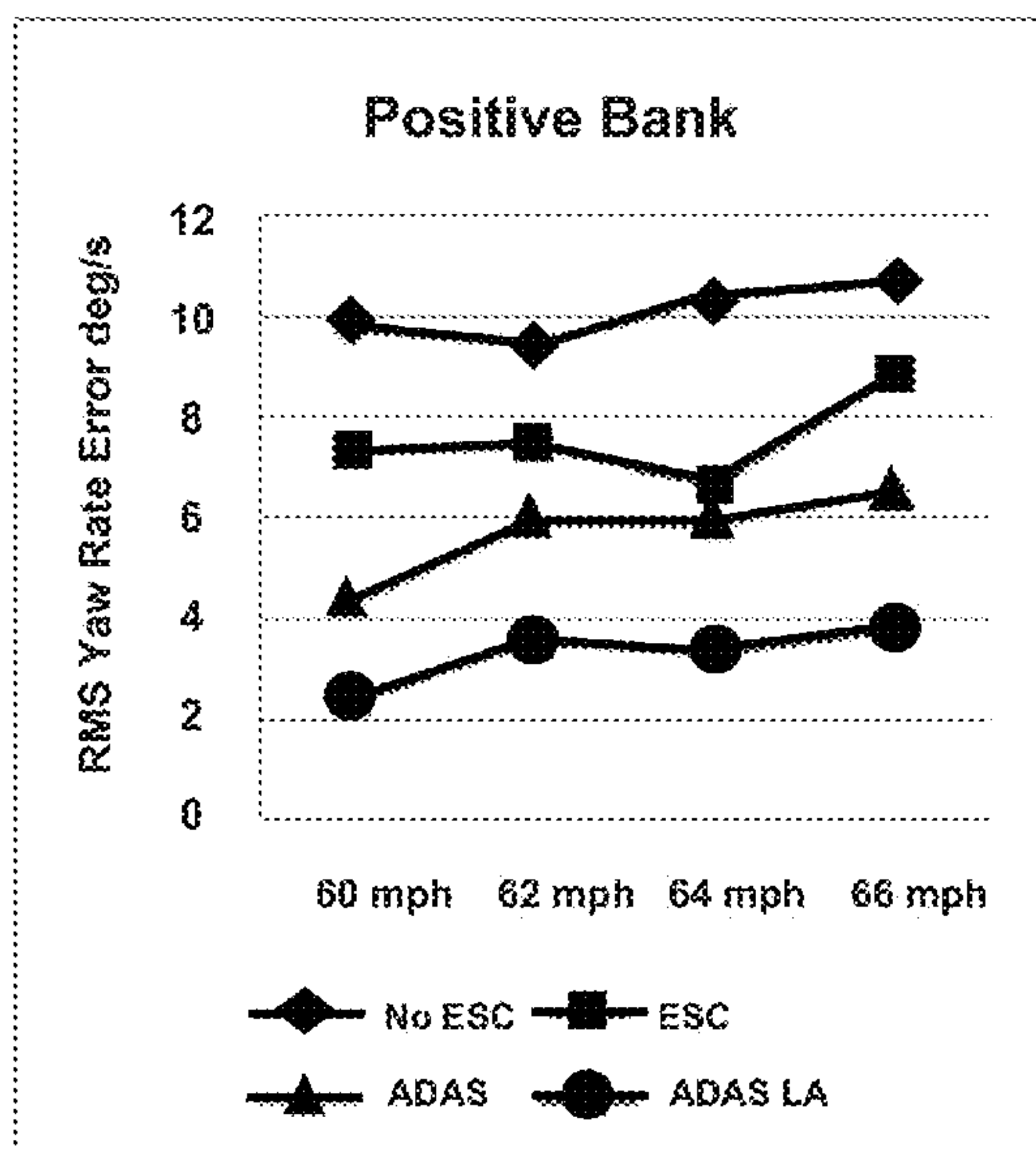
RMS YAW RATE ERROR, POSITIVE BANK
