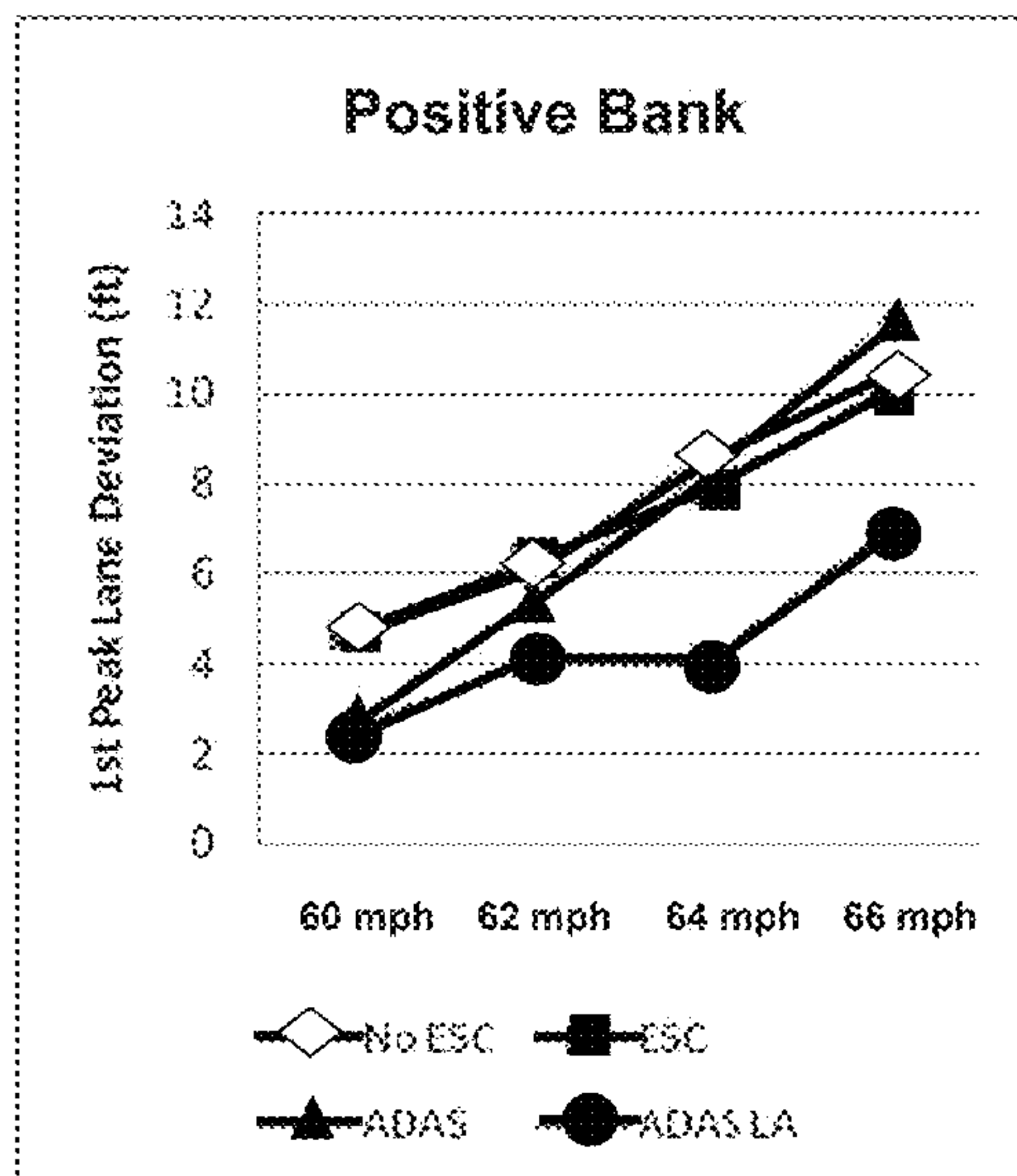
PRIMARY LANE DEVIATION PEAK, POSITIVE BANK
