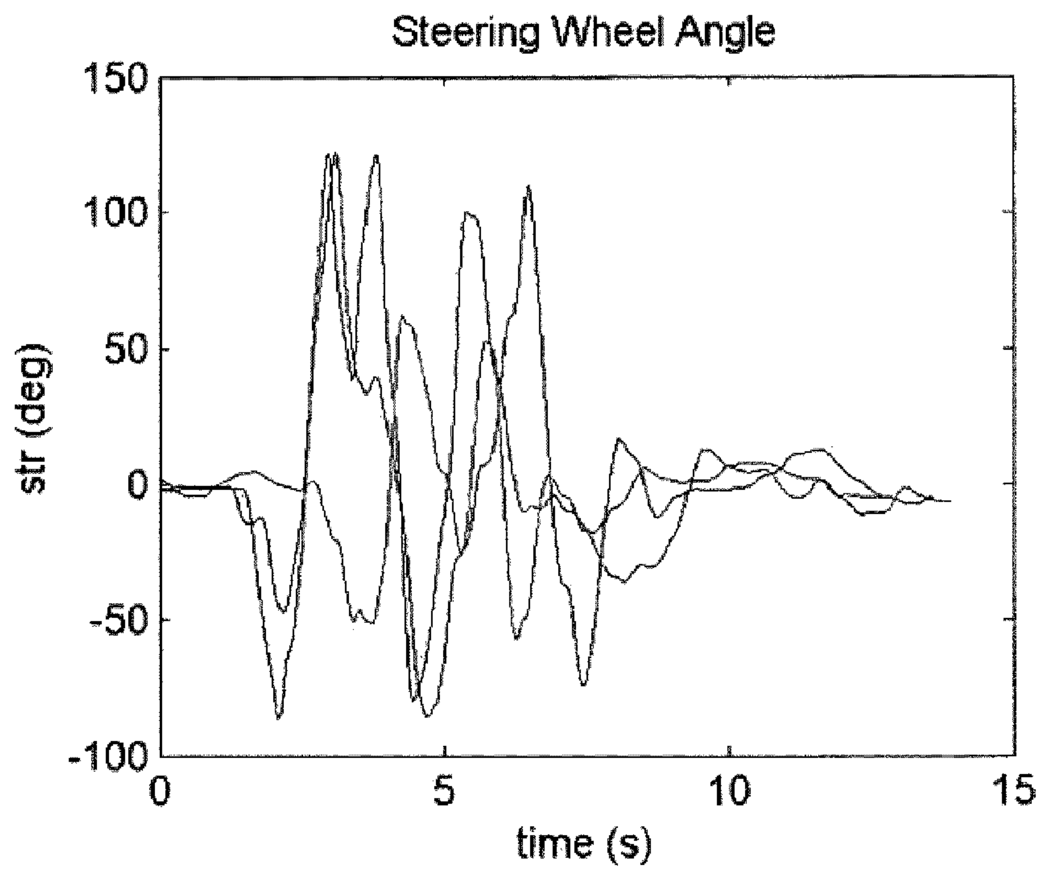
THREE SAMPLE STEERING INPUTS
