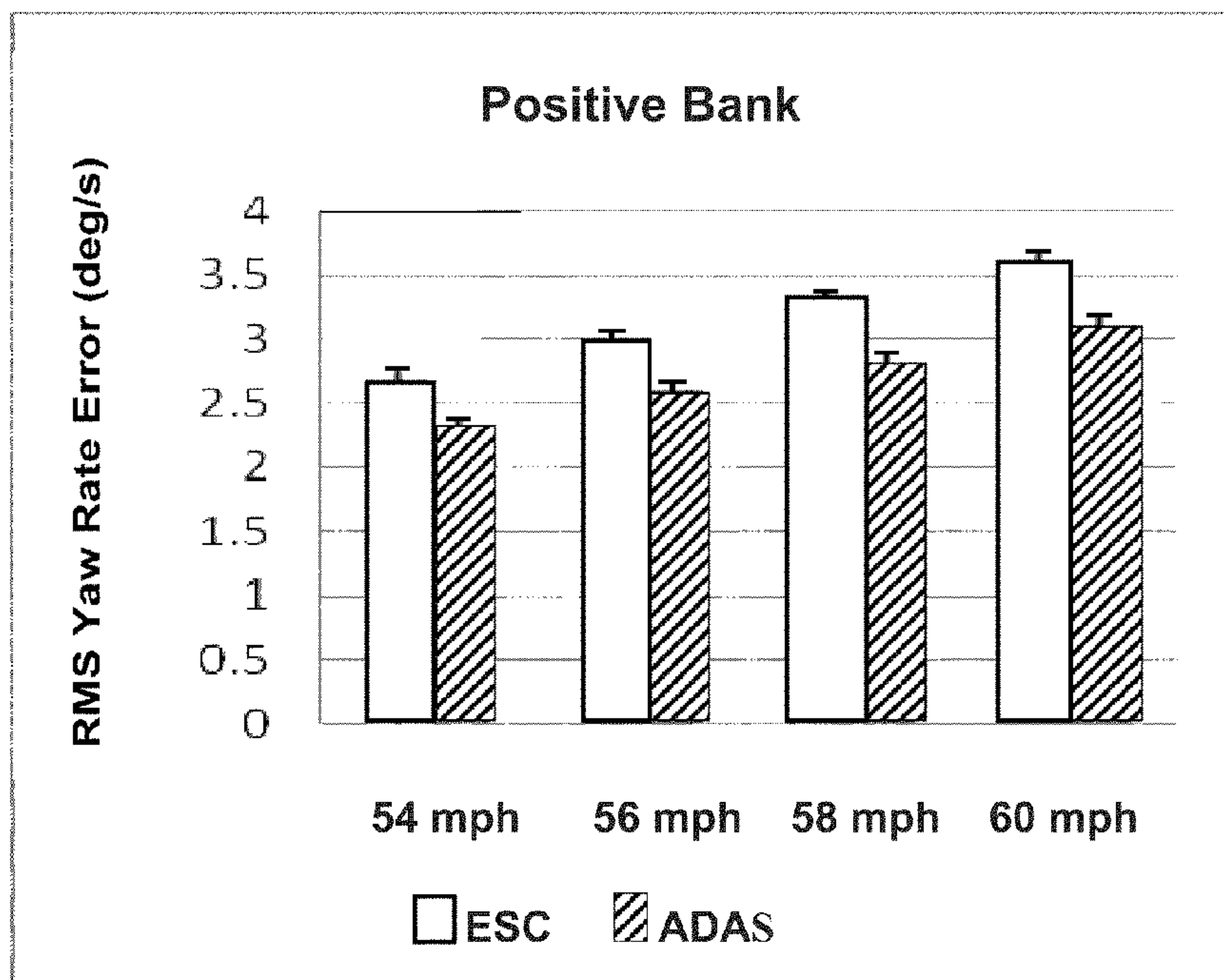
YAW RATE ERROR REDUCTION WITH ADAS ON BANKED CURVE
