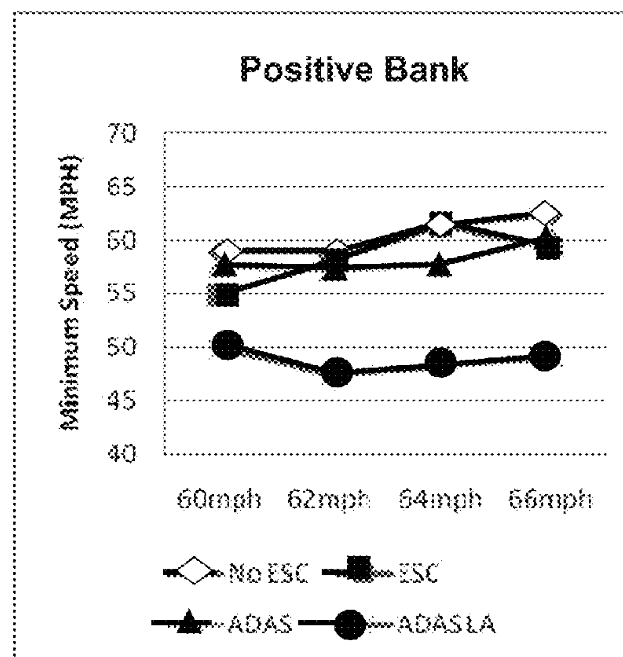
MINIMUM EVENT VELOCITY, POSITIVE BANK
