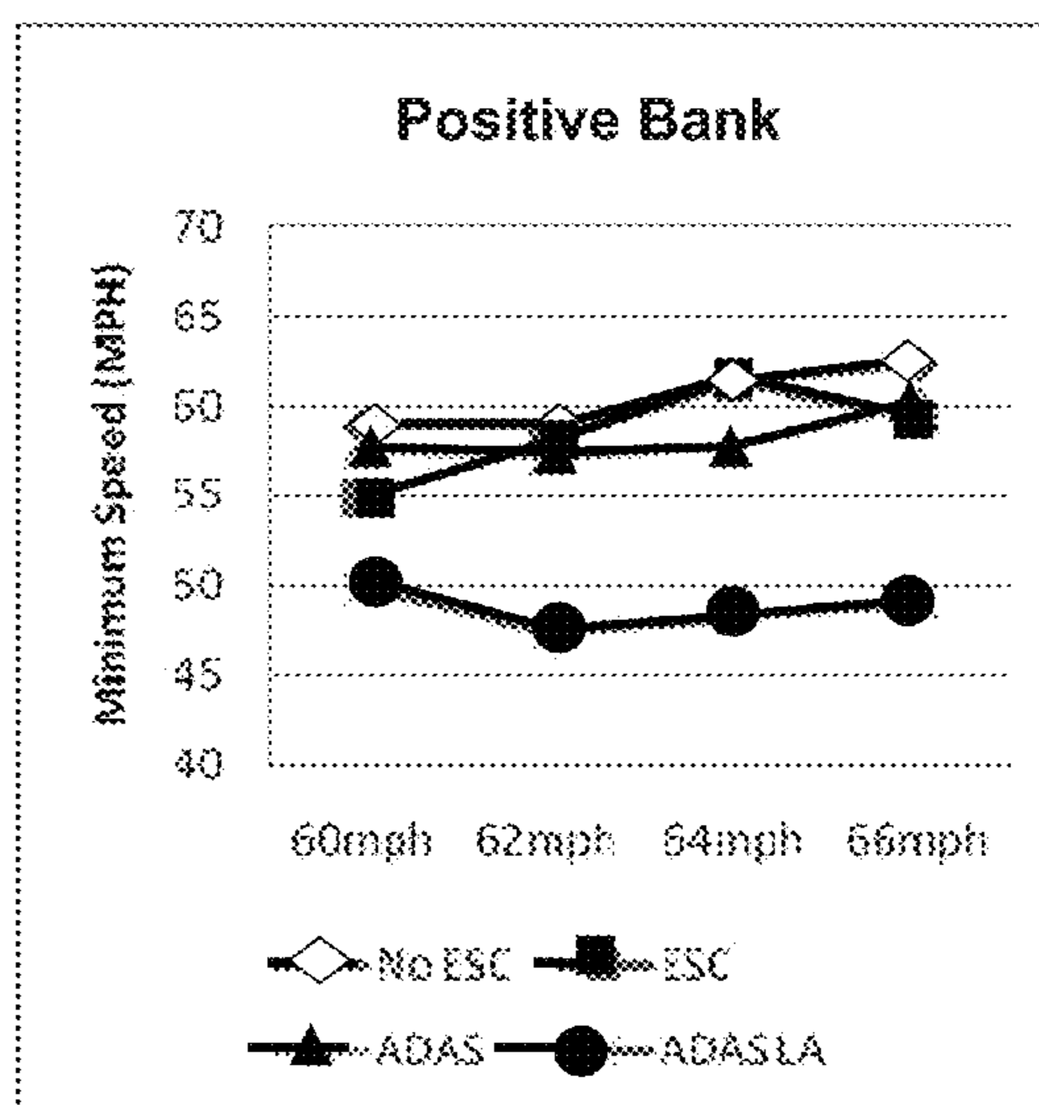
MINIMUM EVENT VELOCITY, POSITIVE BANK
