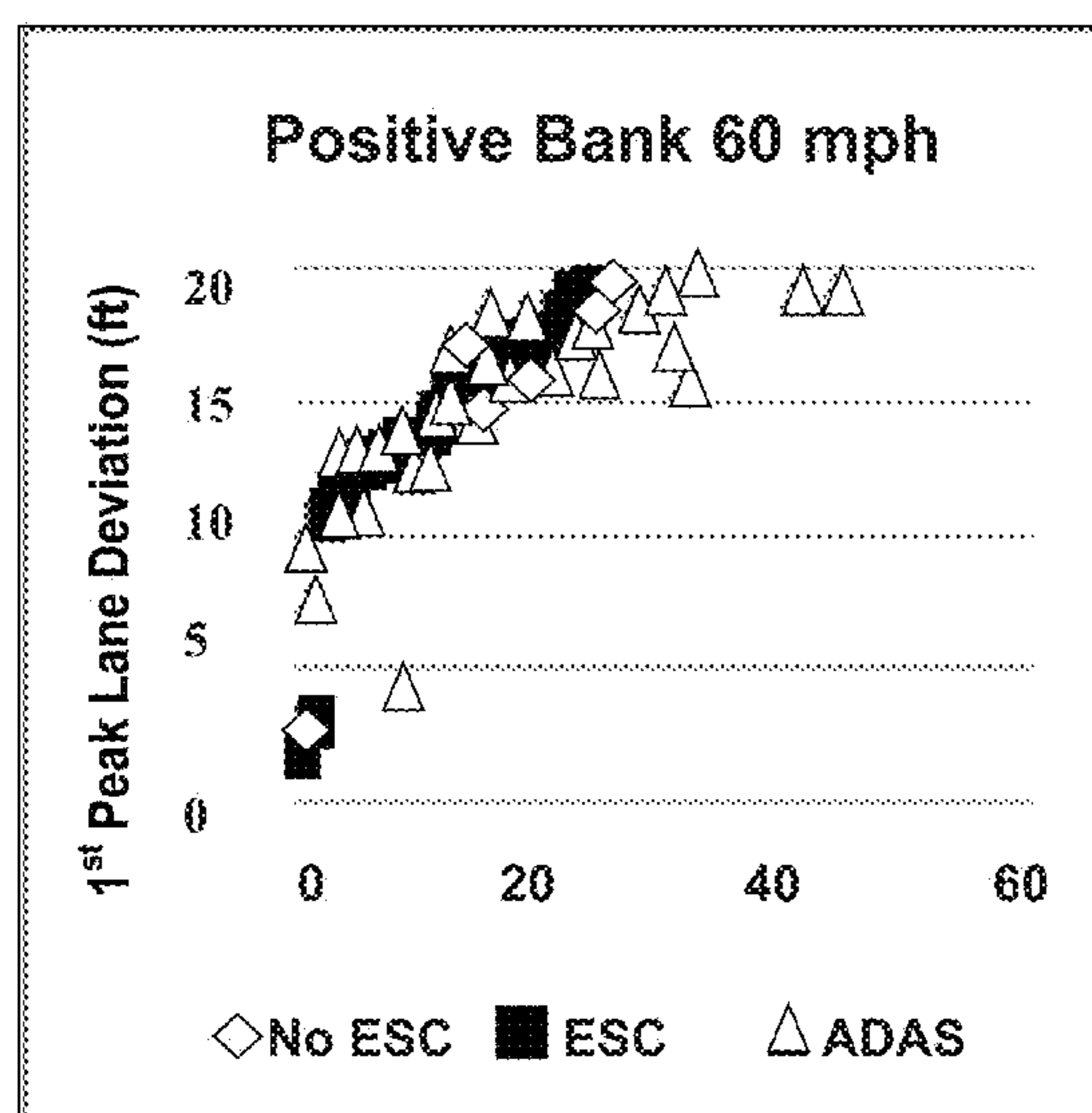
PRIMARY LANE DEVIATION PEAK, POSITIVE BANK, 60 MPH
