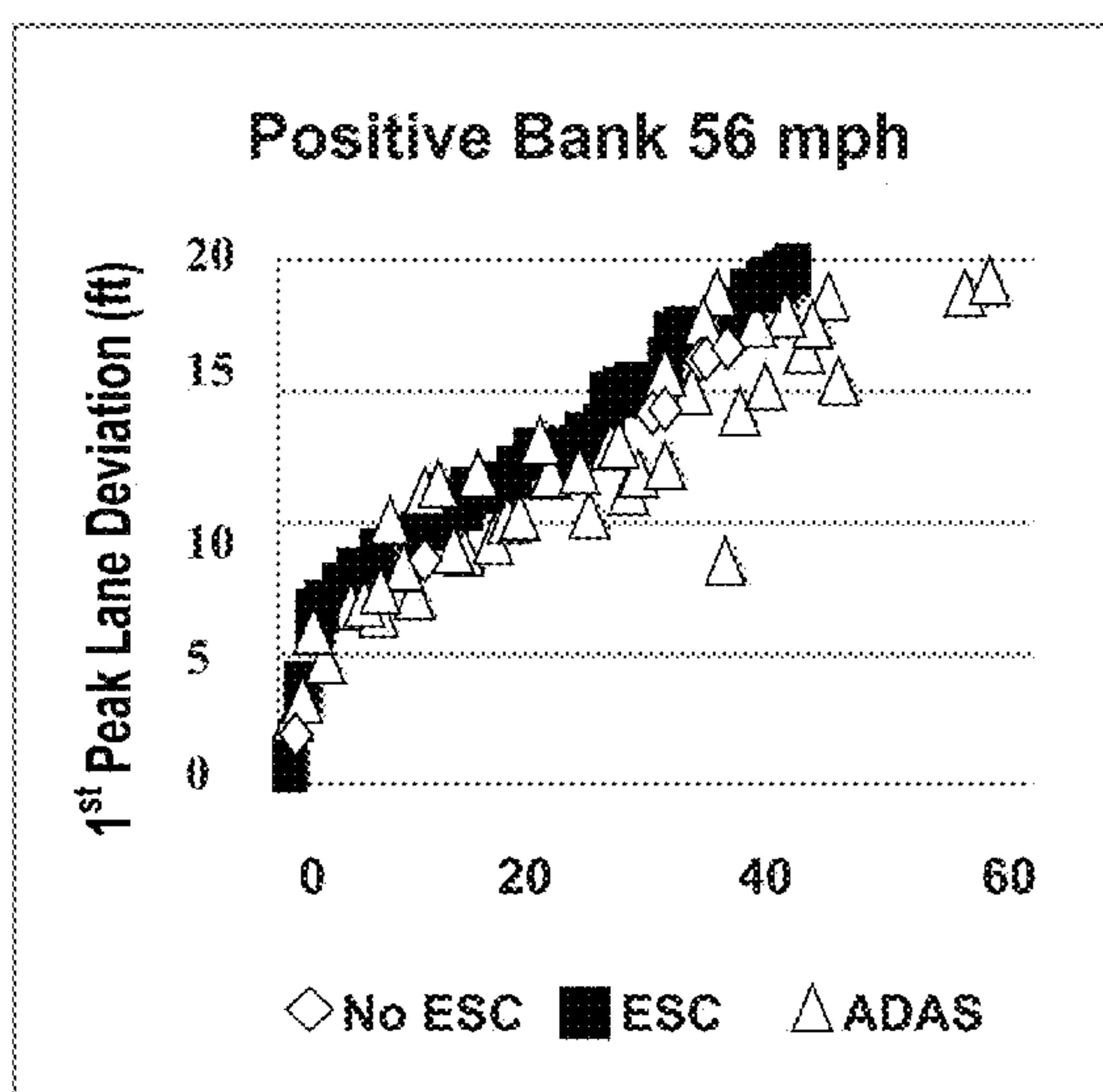
PRIMARY LANE DEVIATION PEAK, POSITIVE BANK, 56 MPH
