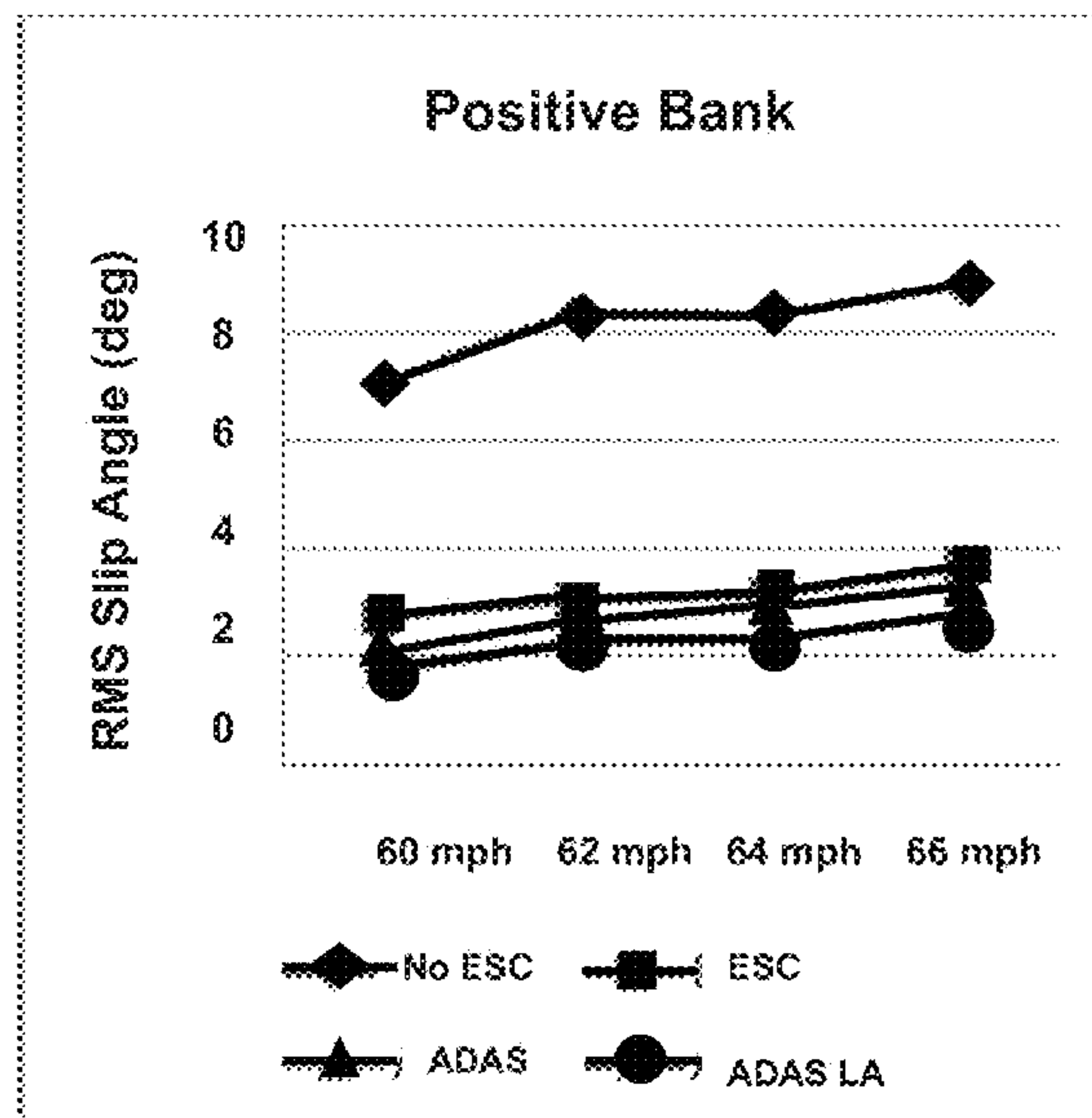
RMS SLIP ANGLE, POSITIVE BANK
