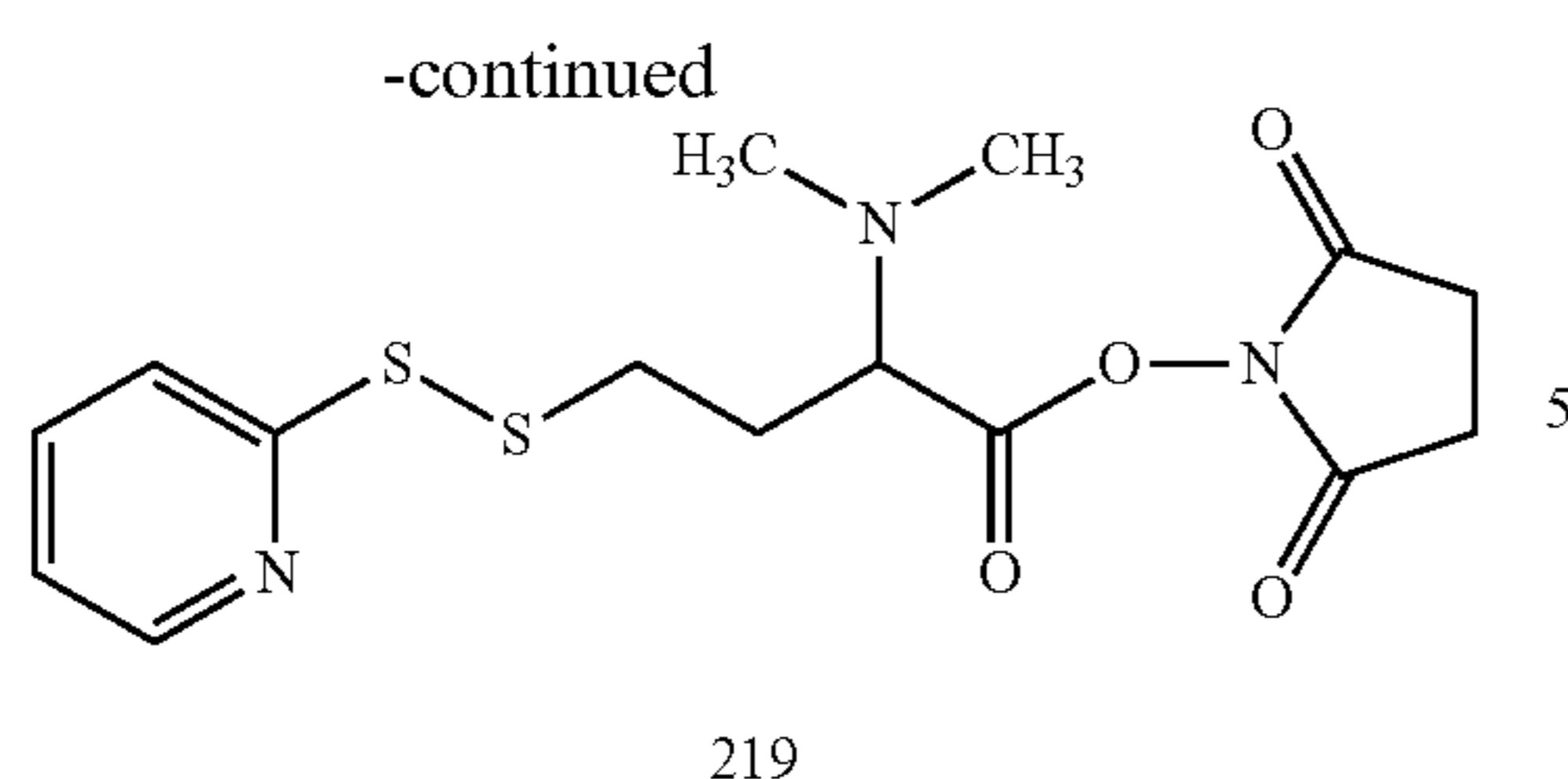
3-(Dimethylamino)dihydrothiophen-2(3H)-one (217)
