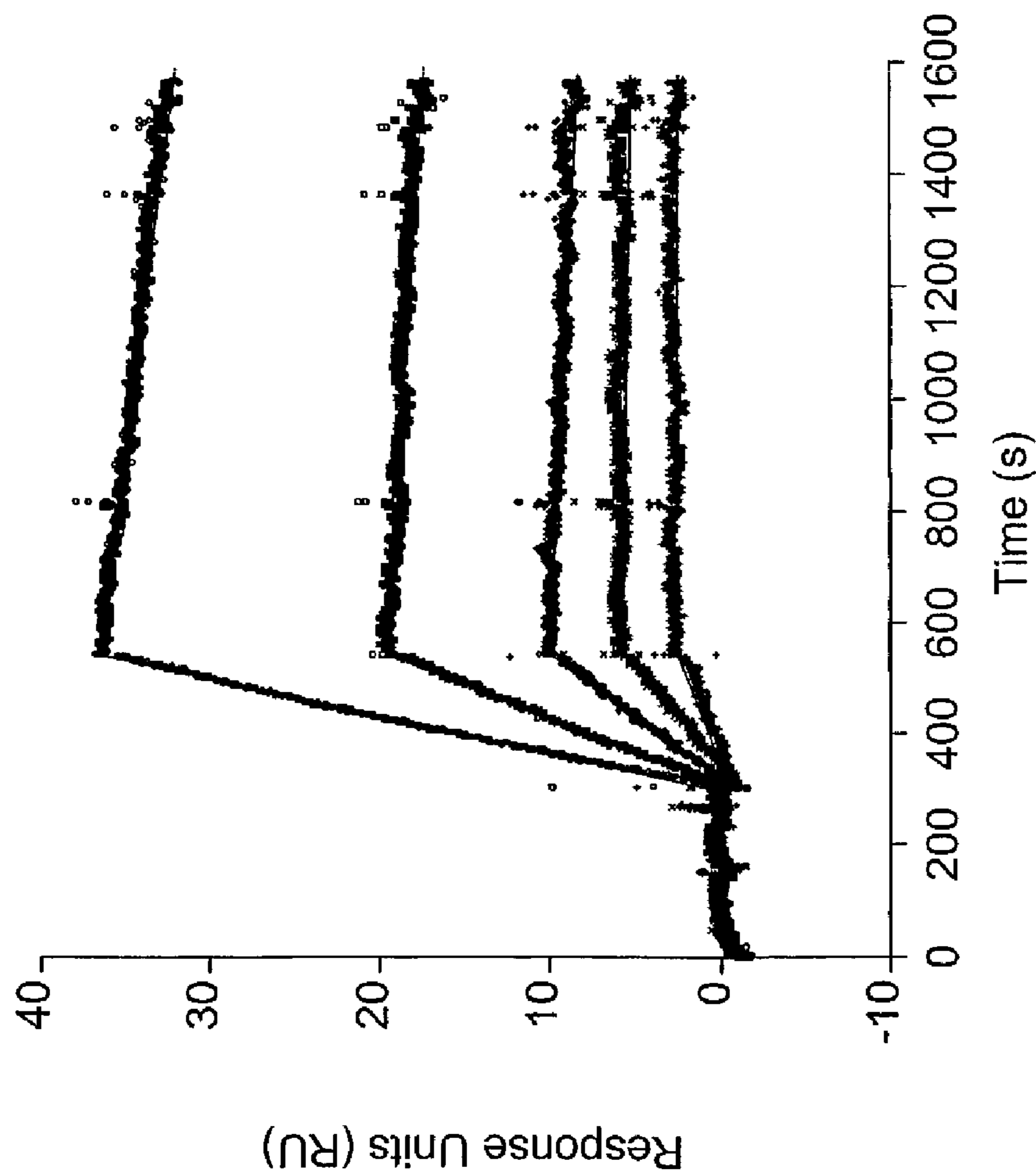
FIGURE 9 Binding kinetics: 911 Fab on NGF CM5 chip
