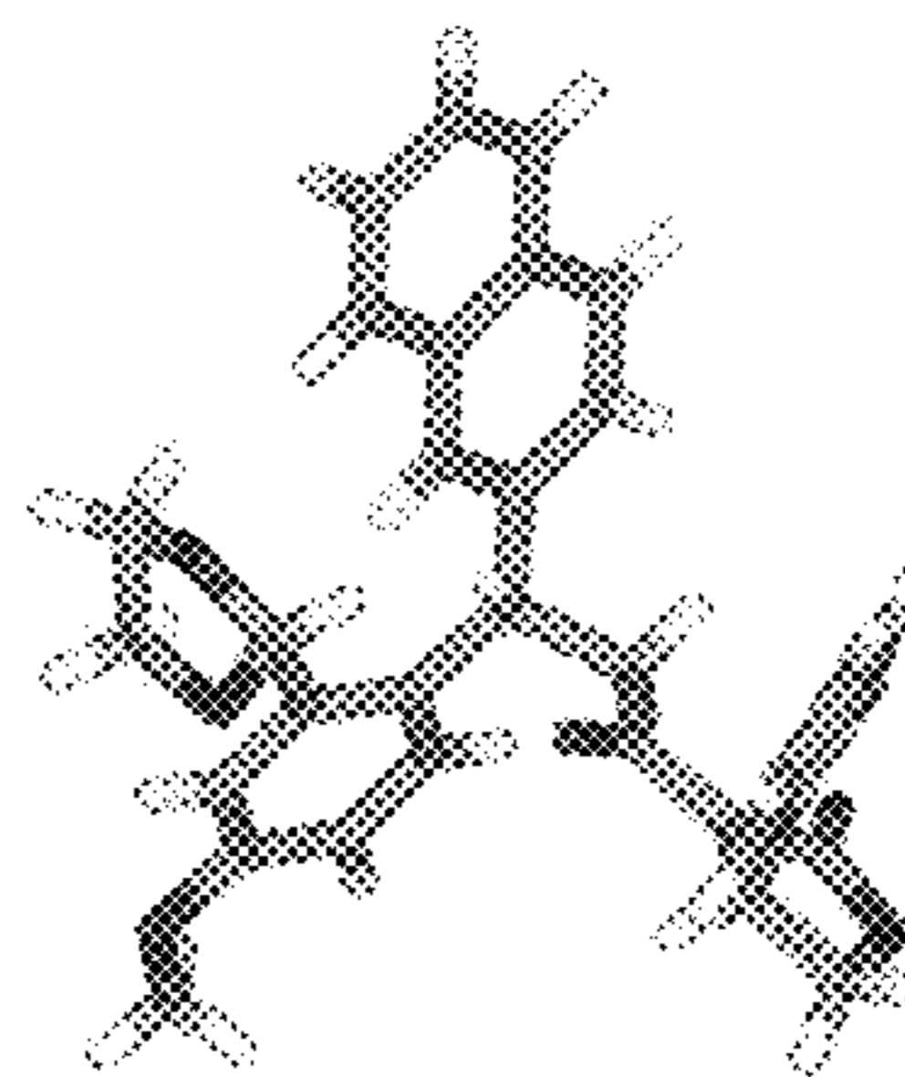
Single Crystal Structure of Compound 22
