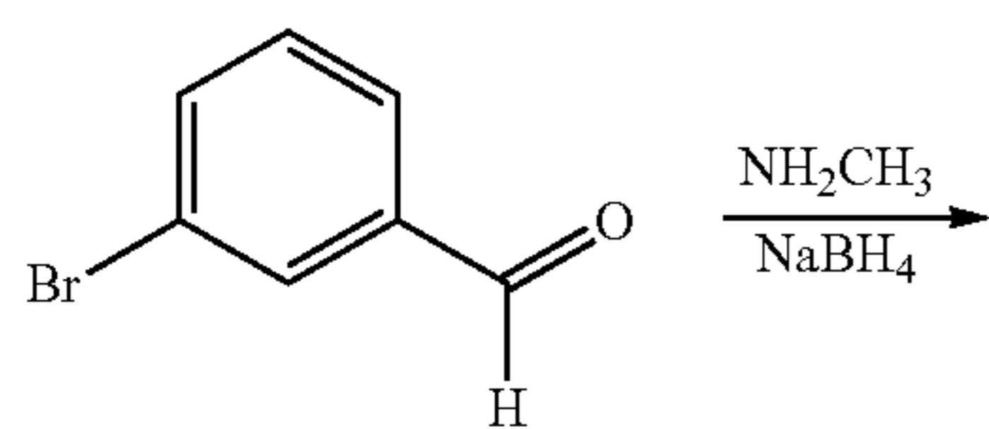
Synthesis Scheme 2
