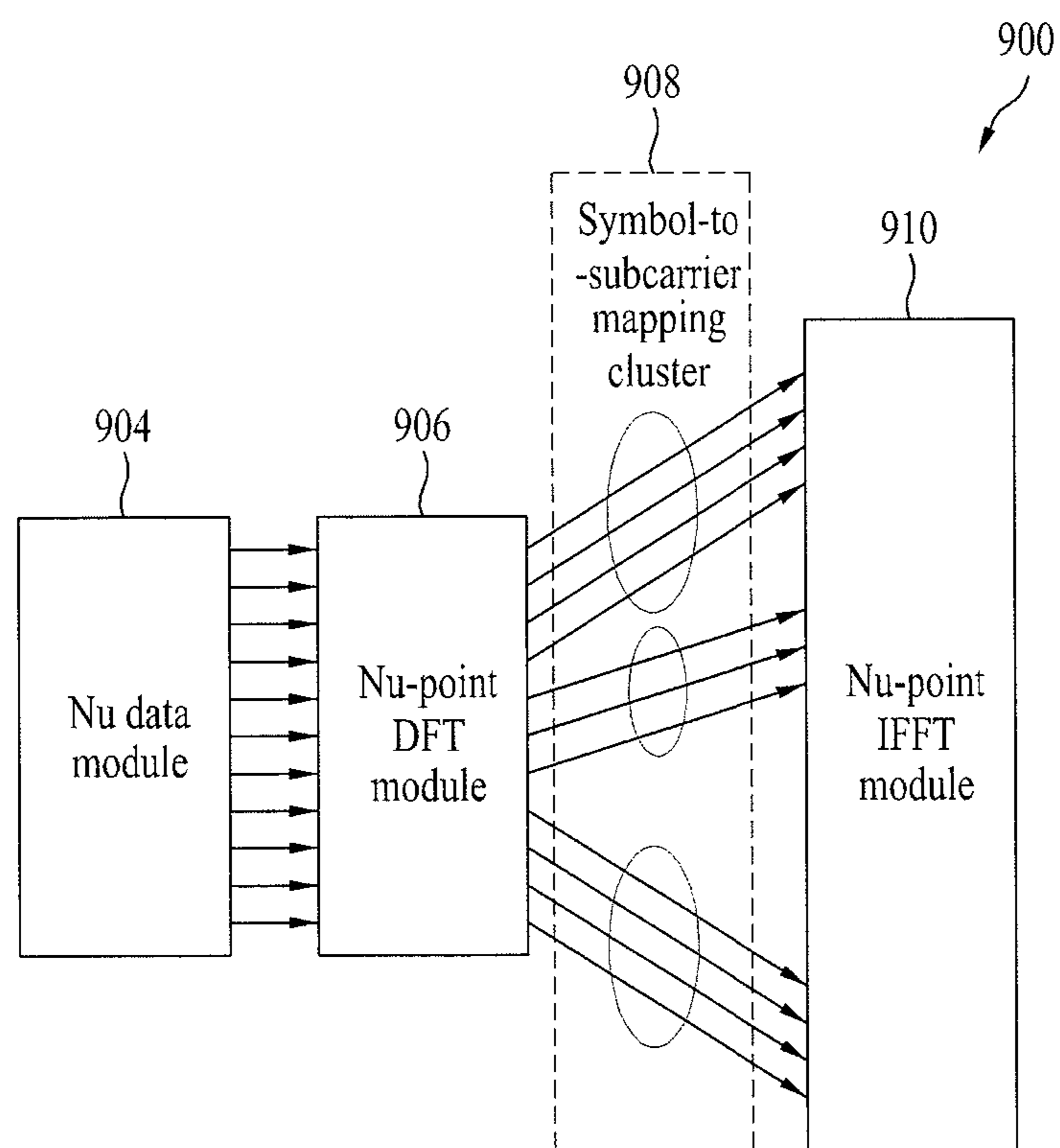
Clustered DFT-s-OFDMA
