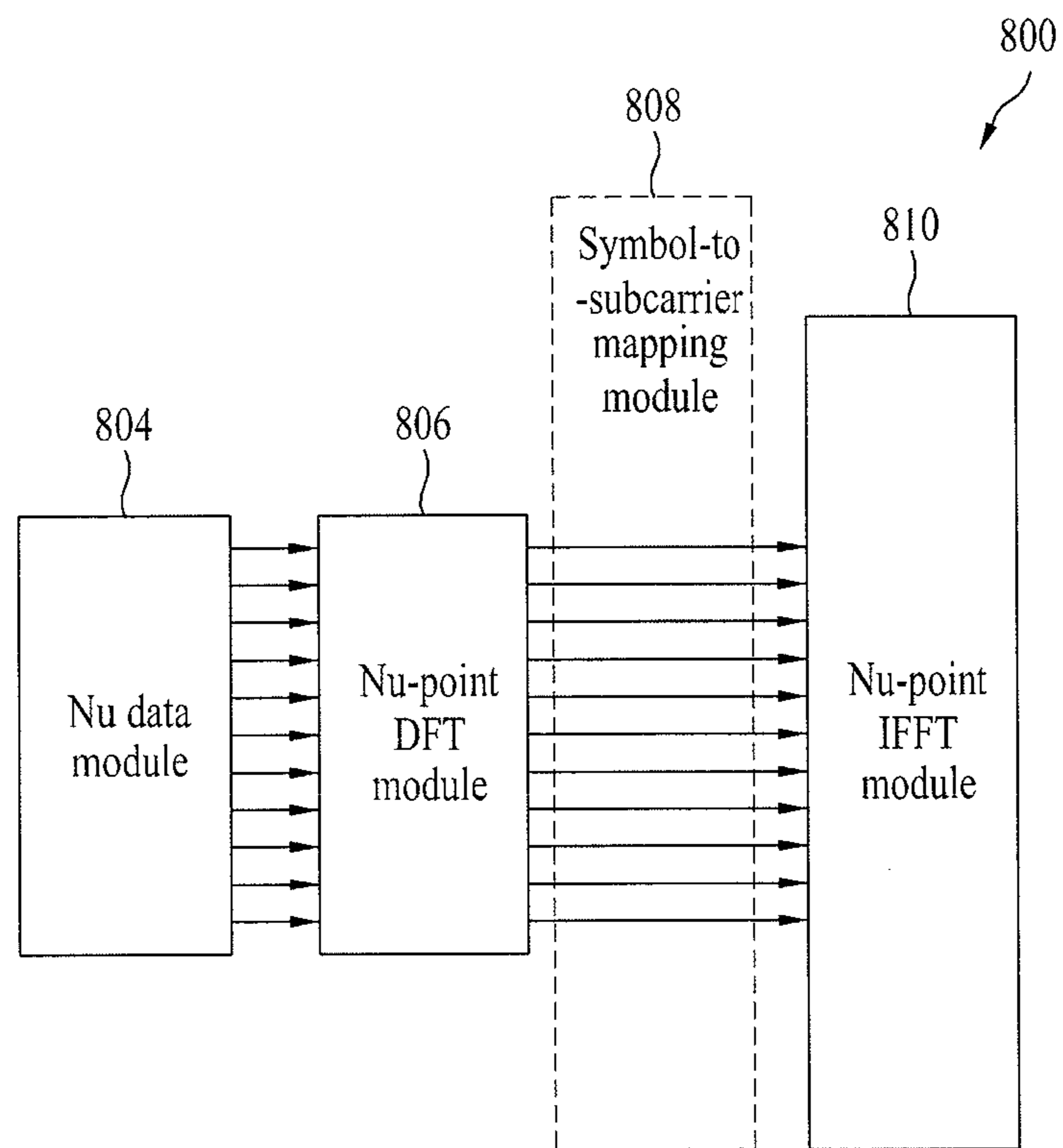
Localized DFT-s-OFDMA
