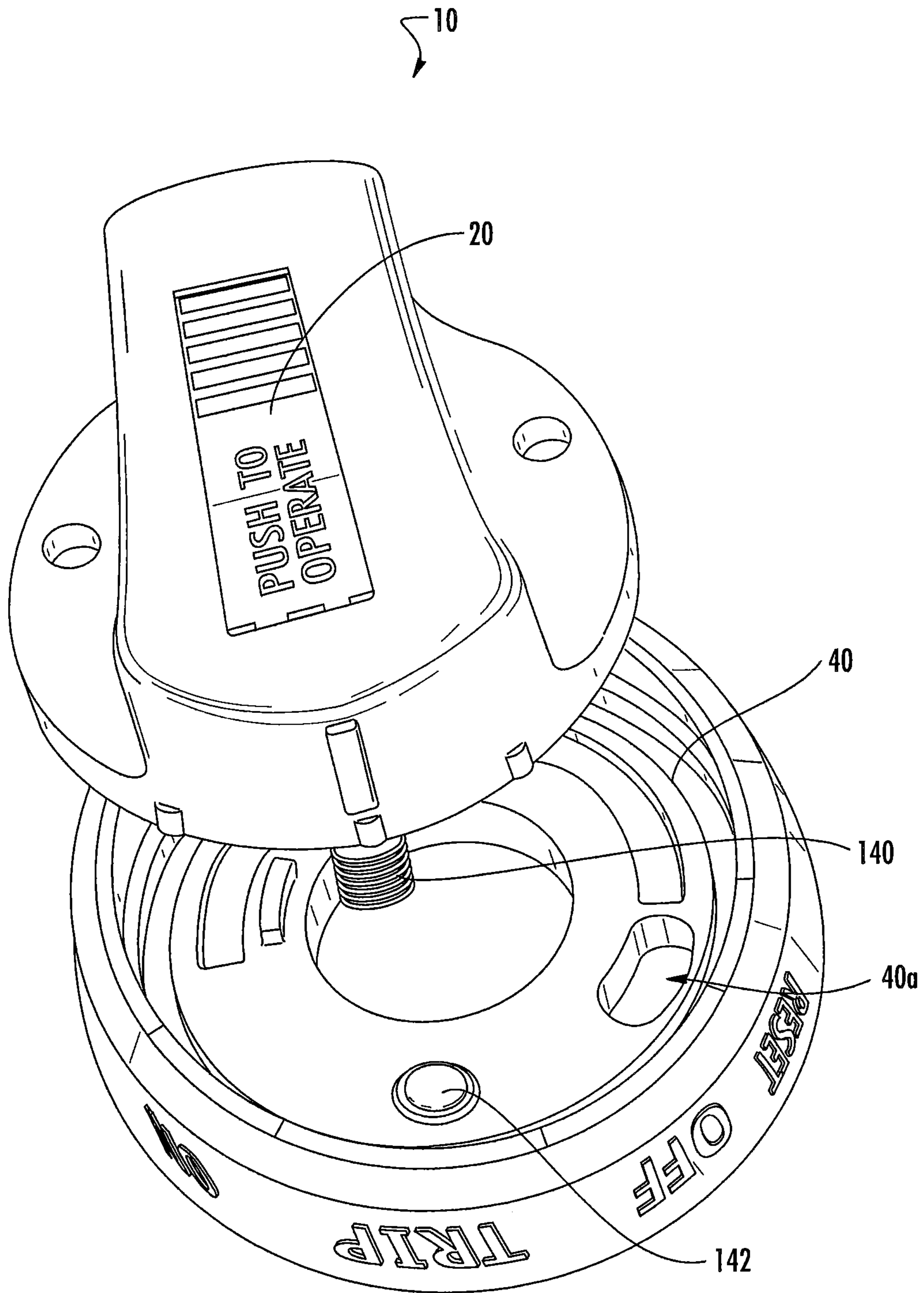
FIG. 12D
