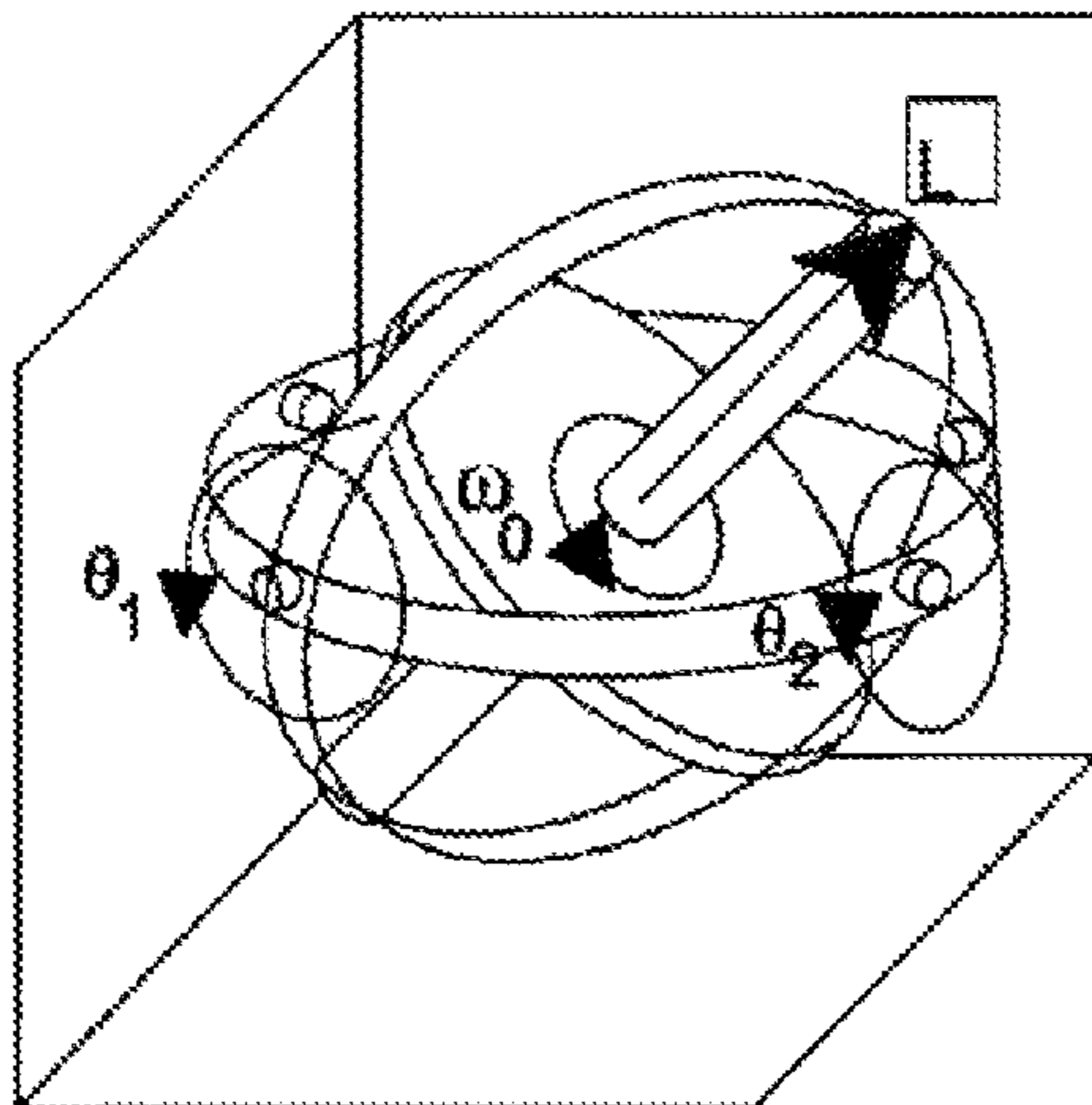
1311 GYROSCOPE TYPE
