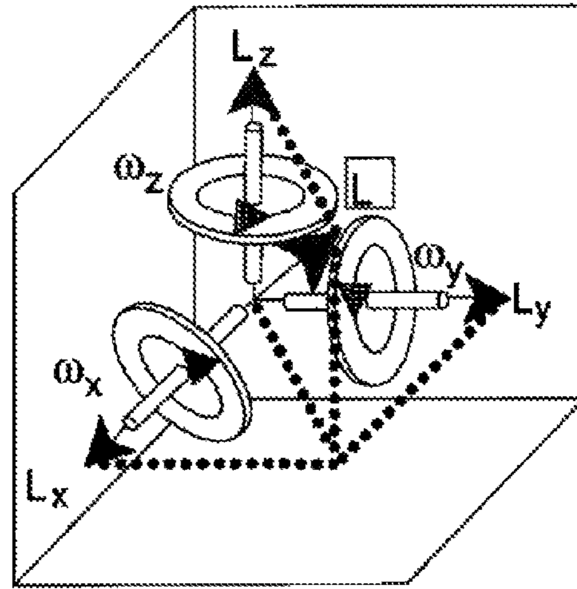
1312 RESULTANT ANGULAR MOMENTUM VECTOR DIFFERENTIAL TYPE
