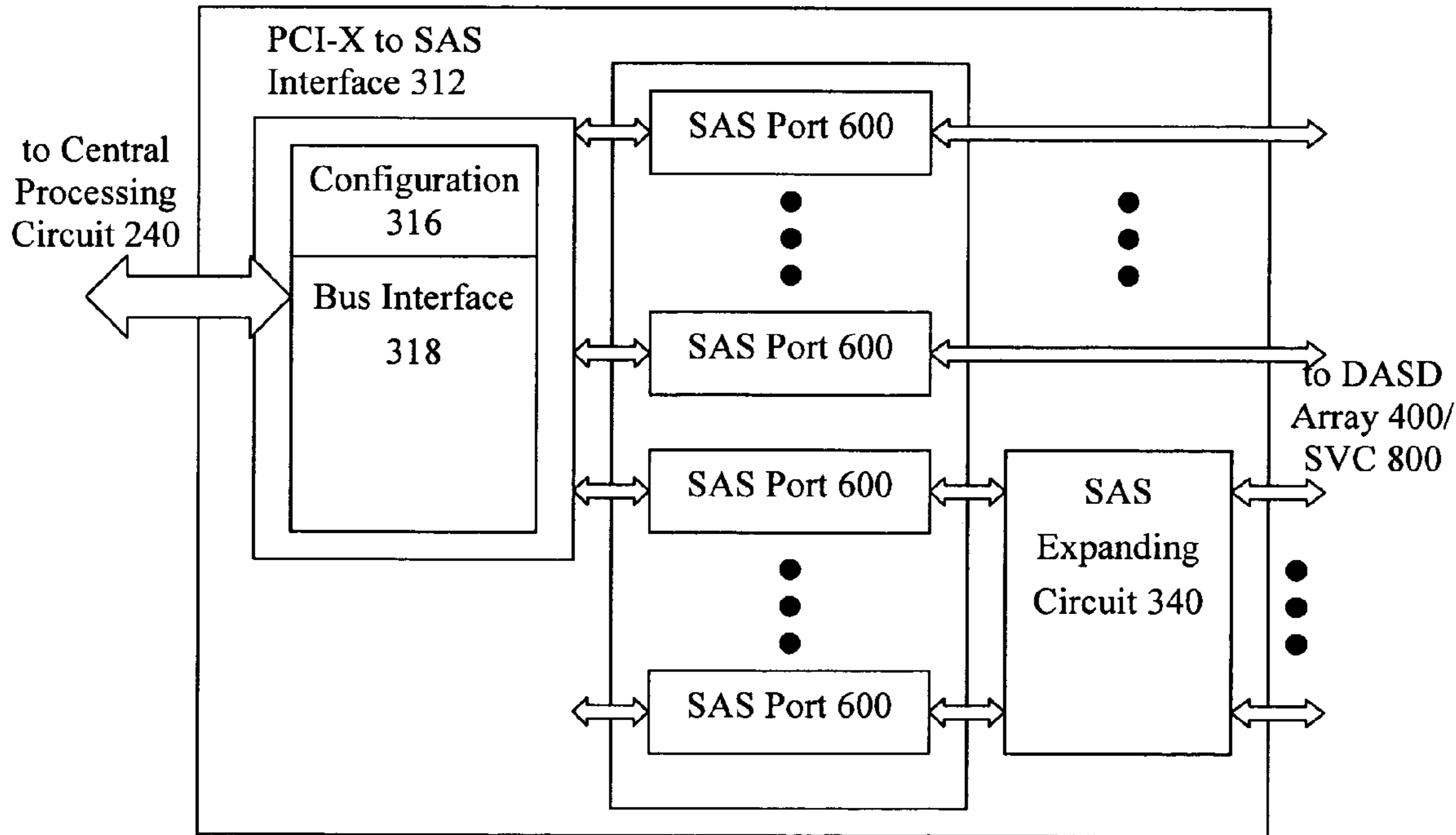
PCI-X to SAS Controller 310
