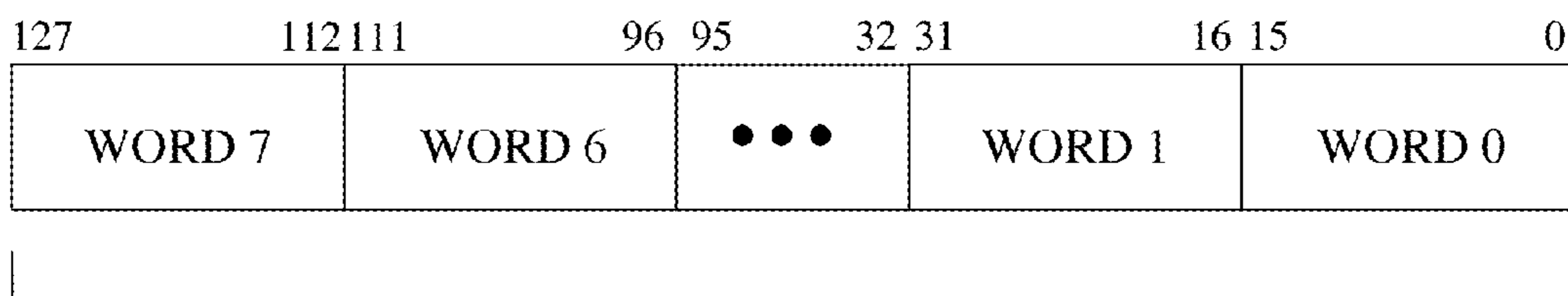
320 PACKED WORD
