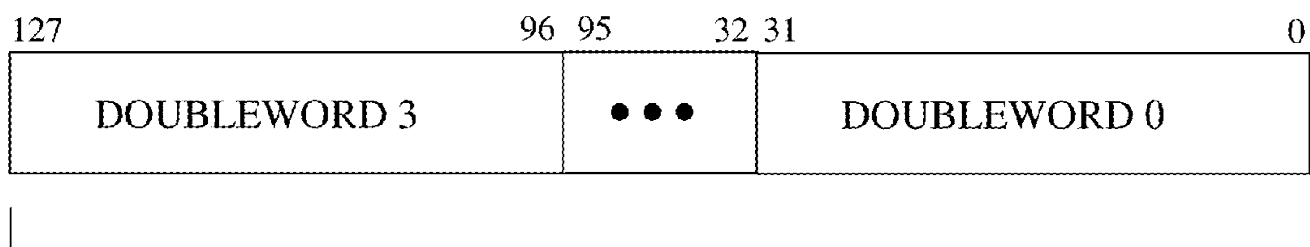
330 PACKED DOUBLEWORD
