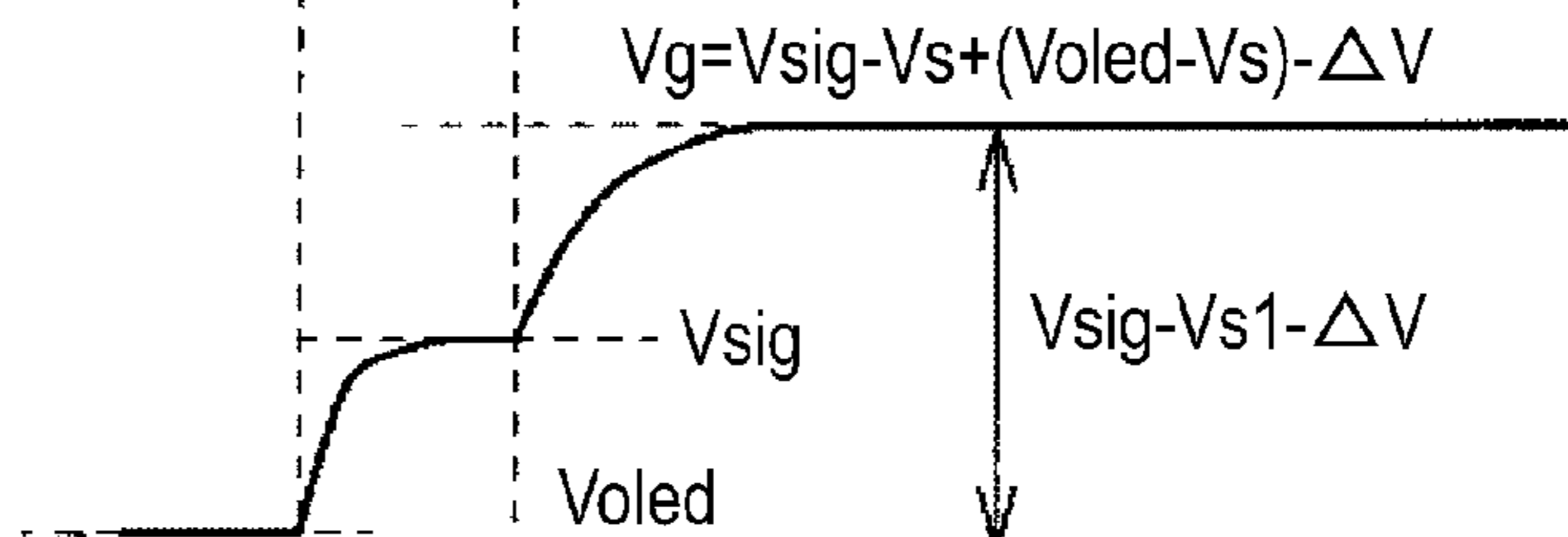
FIG. 12B GATE VOLTAGE Vg
