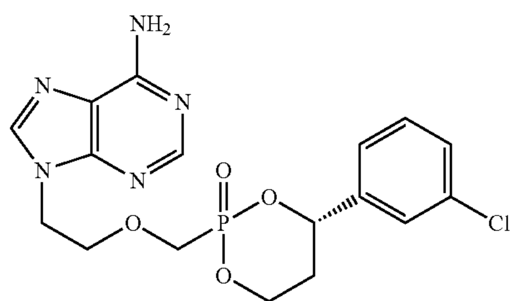
Pradefovir
