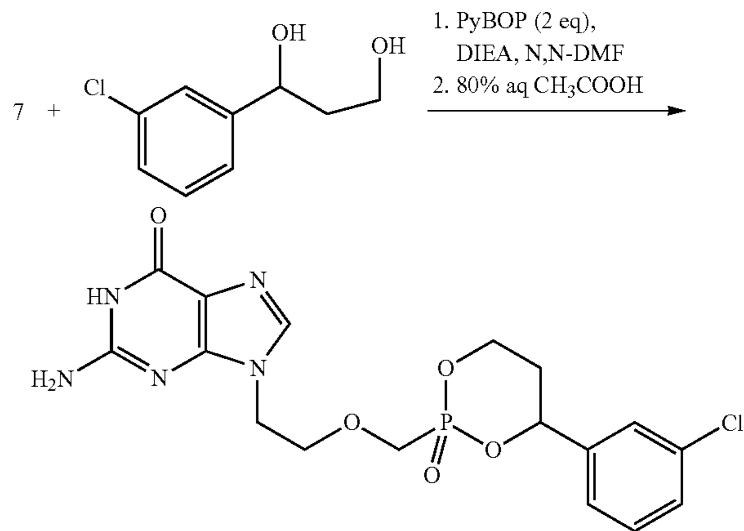
Scheme I
