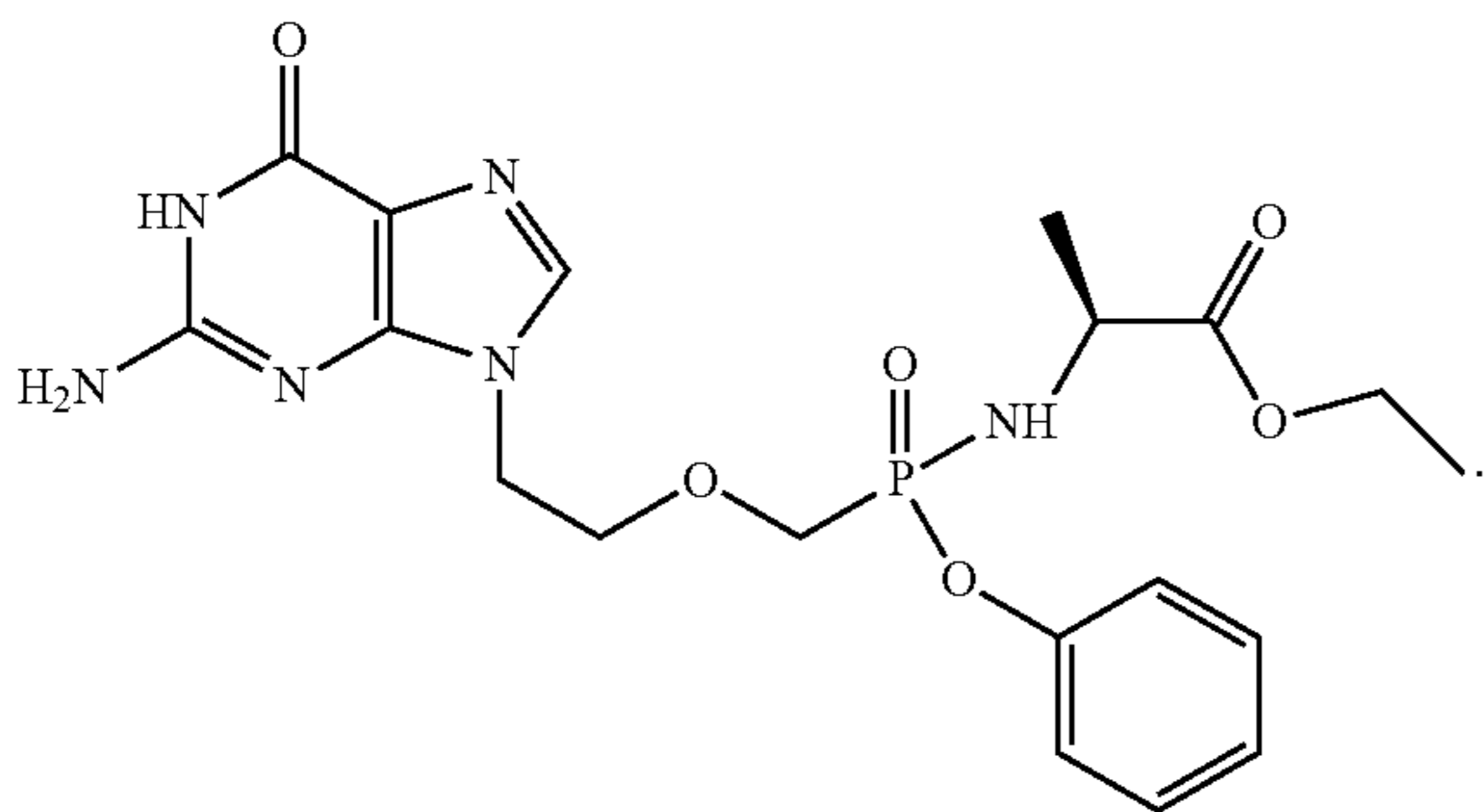
9-[2-phenyloxy-(ethoxy-L-alaninyl)]-phosphonomethoxy ethyl]guanine
