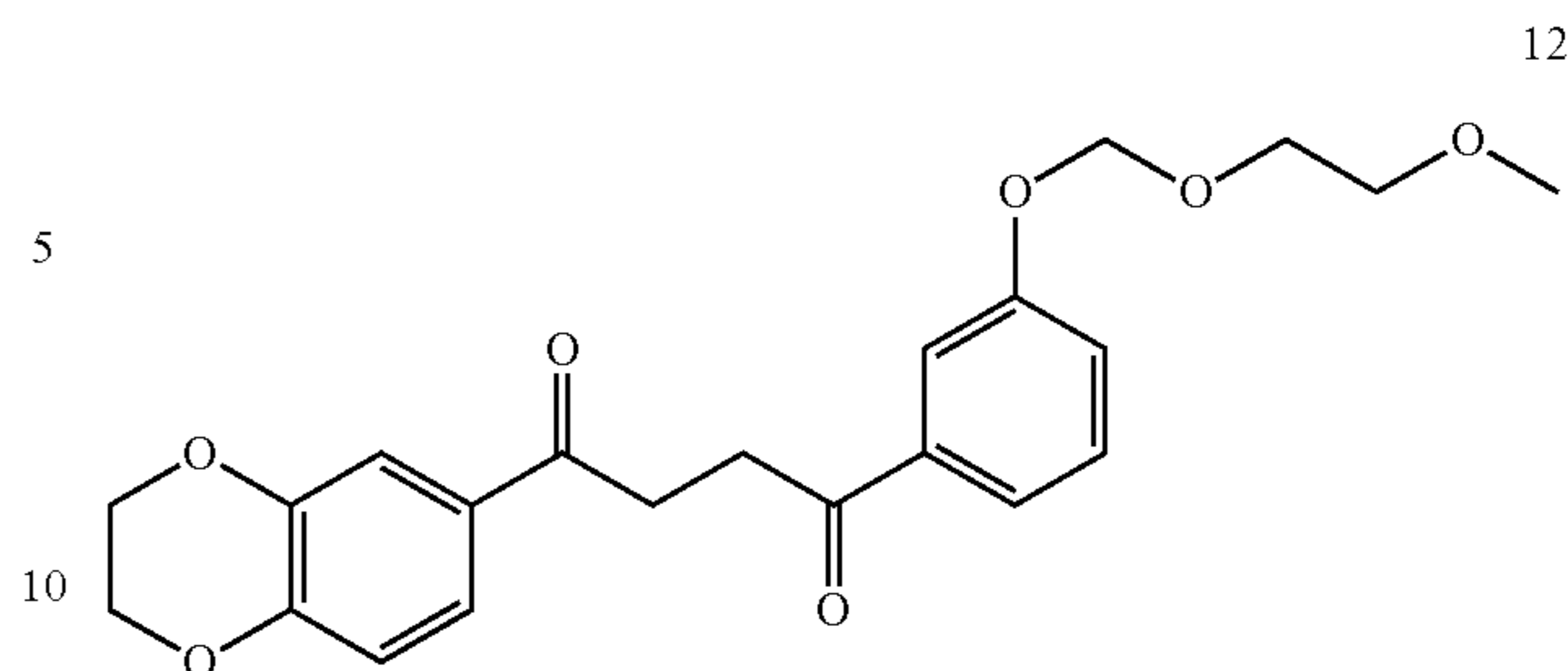
1-(2,3-dihydrobenzo[b][1,4]dioxin-6-yl)-4-(3((2-methoxyethoxy) methoxy)phenyl)butane-1,4-dione 12
