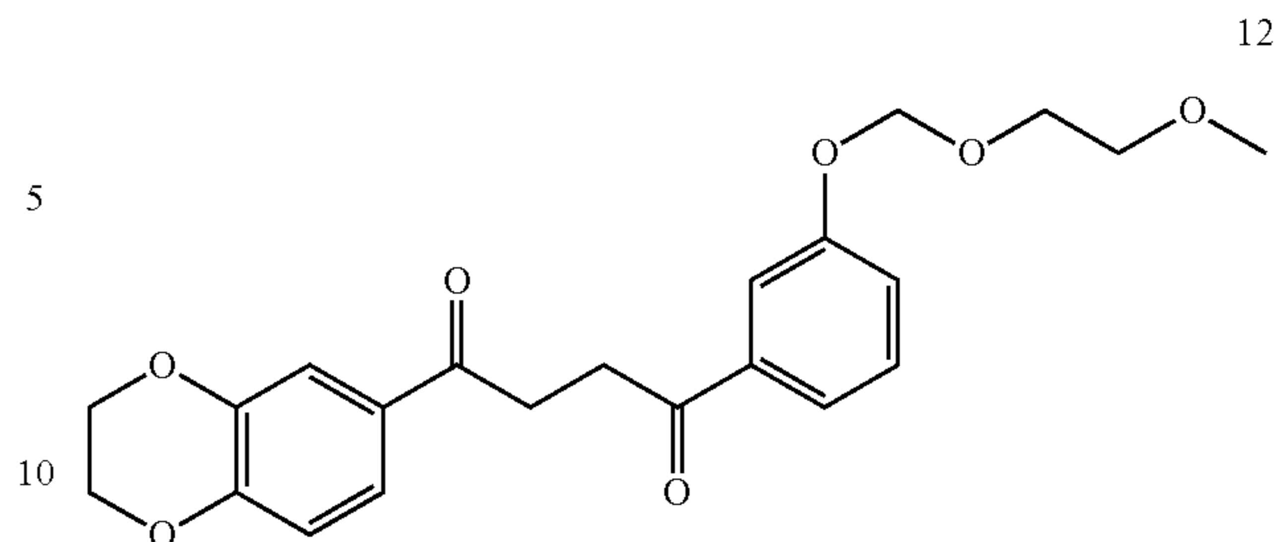
1-(2,3-dihydrobenzo[b][1,4]dioxin-6-yl)-4-(3((2-methoxyethoxy) methoxy)phenyl)butane-1,4-dione 12
