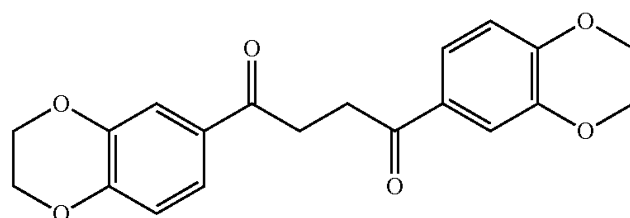
1,4-bis(2,3-dihydrobenzo[b][1,4]dioxin-6-yl)butane-1,4-dione 14
