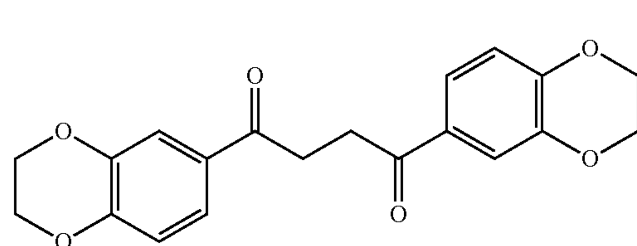
1,4-bis(2,3-dihydrobenzo[b][1,4]dioxin-6-yl)butane-1,4-dione 14
