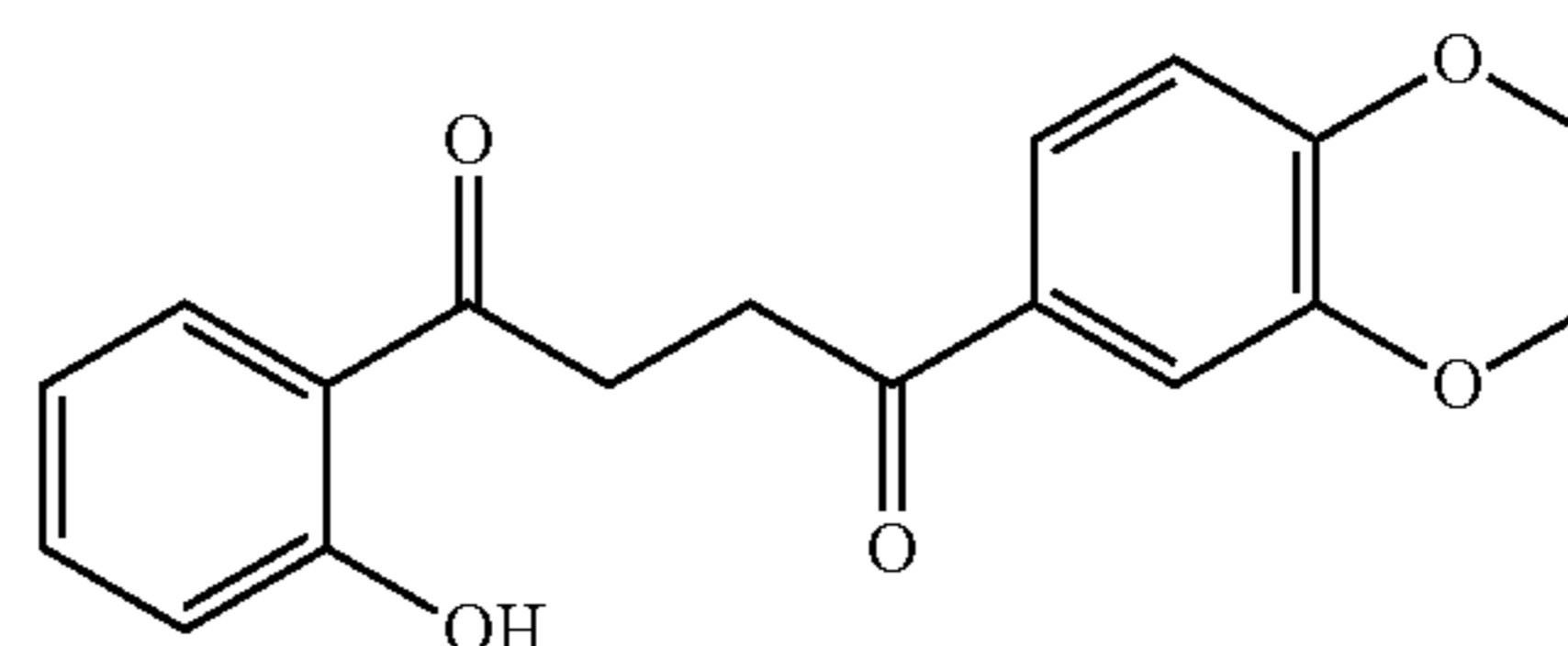
1-(2,3-dihydrobenzo[b][1,4]dioxin-6-yl)-4-(2-hydroxyphenyl)butane-1,4-dione 8
