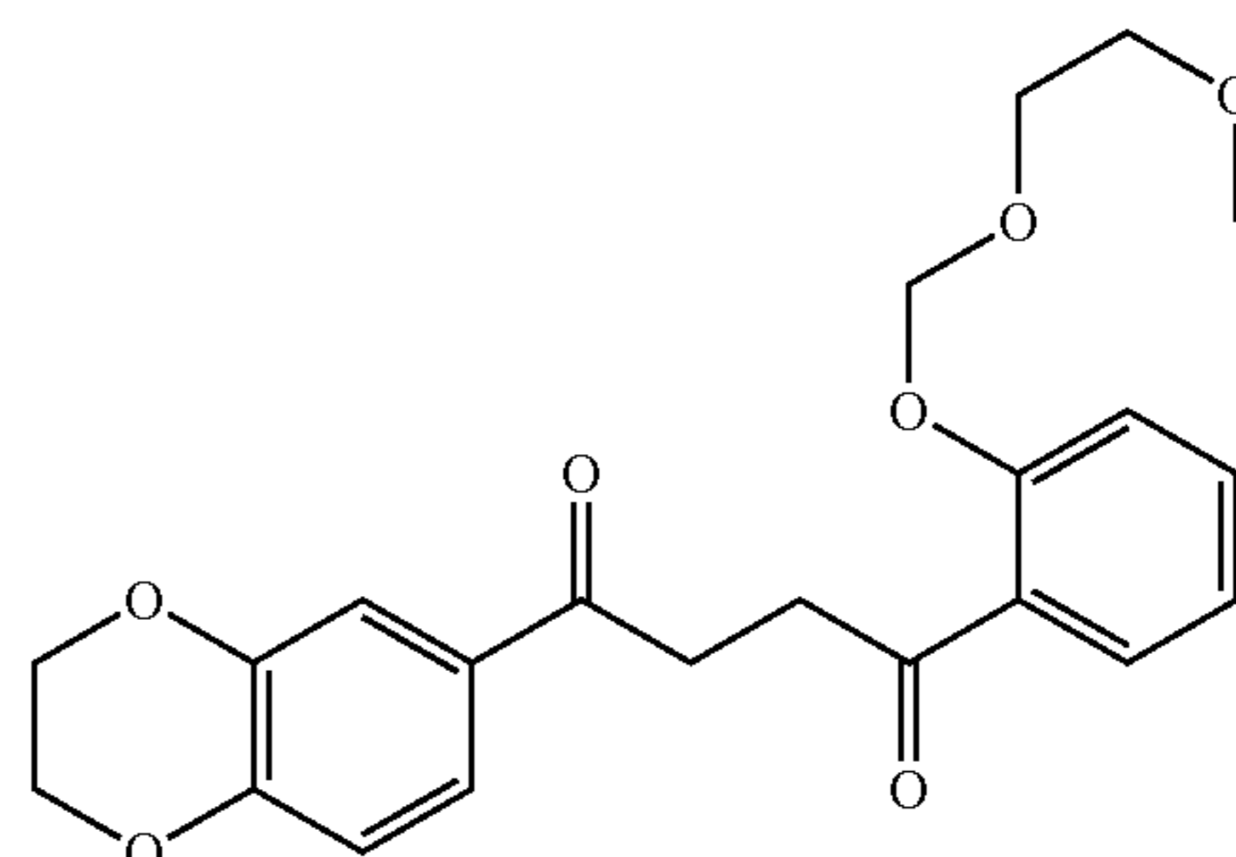
1-(2,3-dihydrobenzo[b][1,4]dioxin-6-yl)-4-(2-((2-methoxyethoxy) methoxy)phenyl)butane-1,4-dione 13
