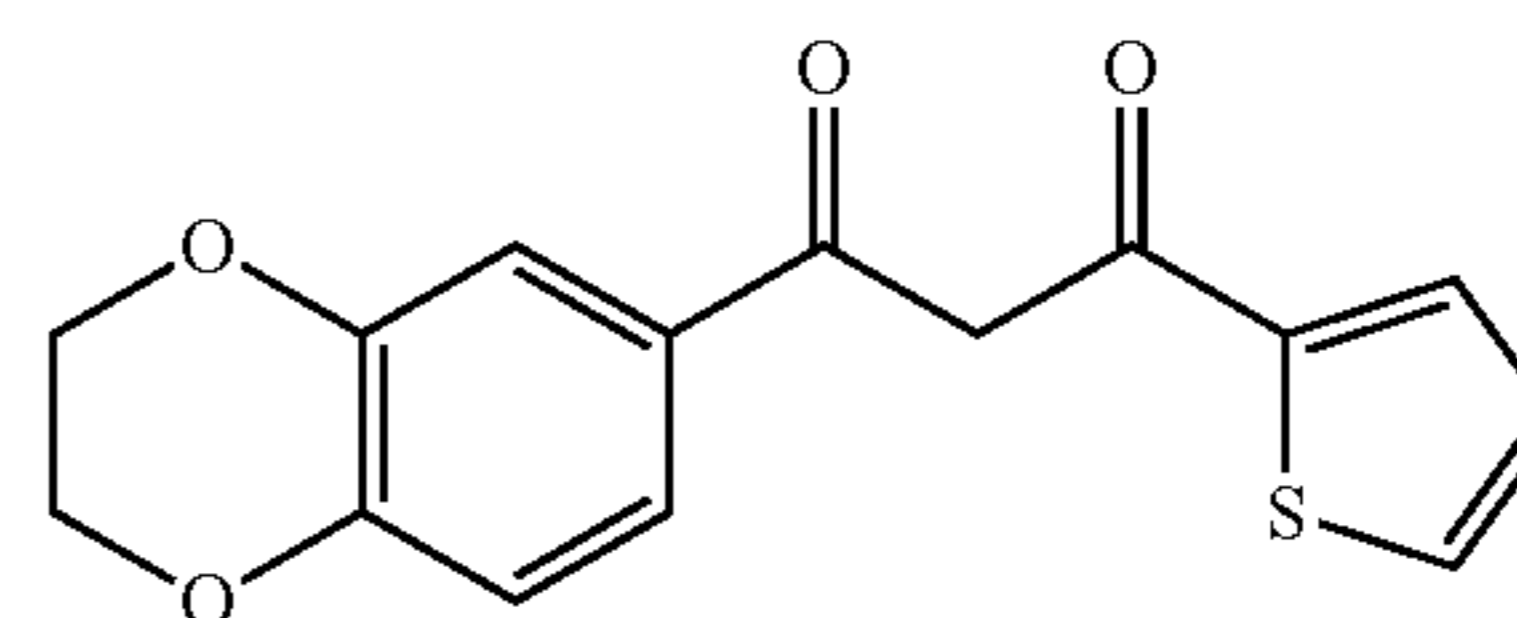
1-(2,3-dihydrobenzo[b][1,4]dioxin-6-yl)-3-(thiophen-2-yl)propane-1,3-dione 16
