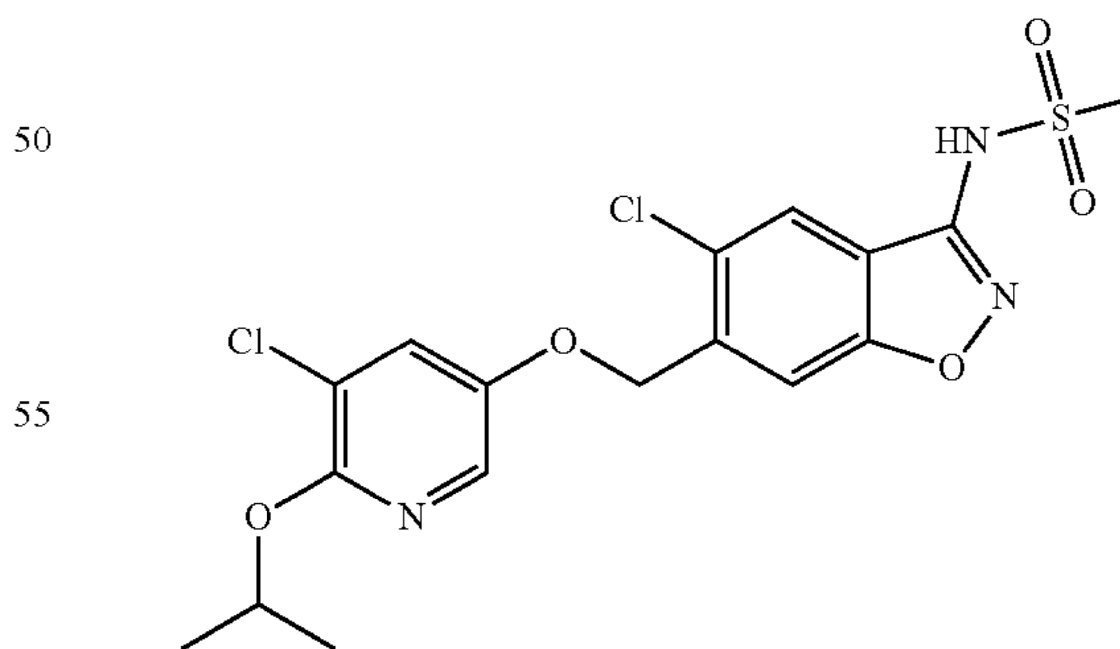
N-(5-chloro-6-((5-chloro-6-isopropoxy-pyridin-3-yl)oxy)methyl)benzo[d]isoxazol-3-yl)-methanesulfonamide
