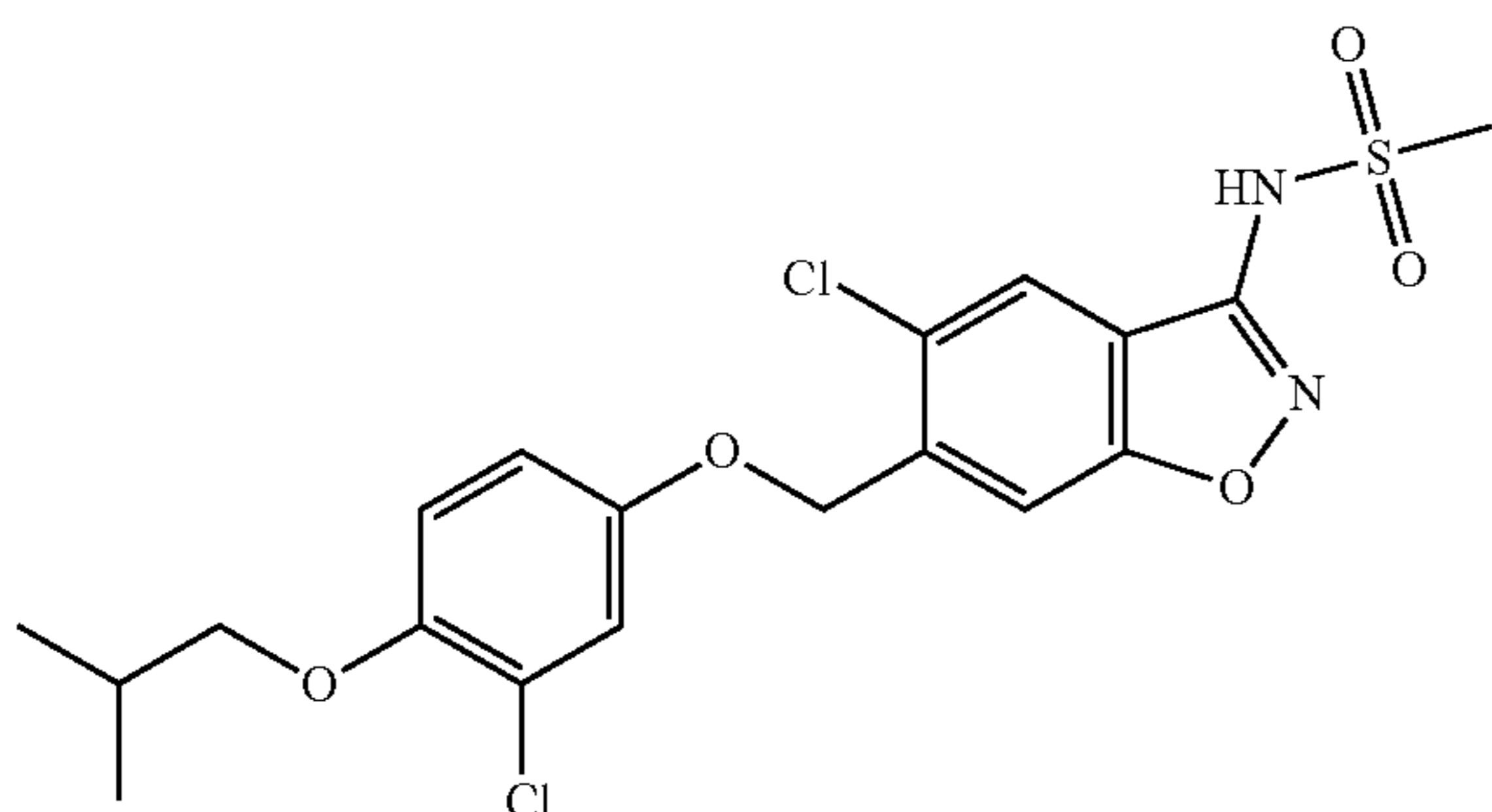
N-(5-chloro-6-((3-chloro-4-isobutoxyphenoxy)methyl)benzo[d]isoxazol-3-yl)methanesulfonamide
