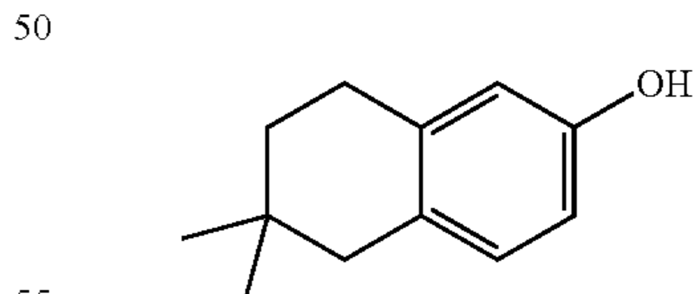
6,6-dimethyl-5,6,7,8-tetrahydronaphthalen-2-ol
