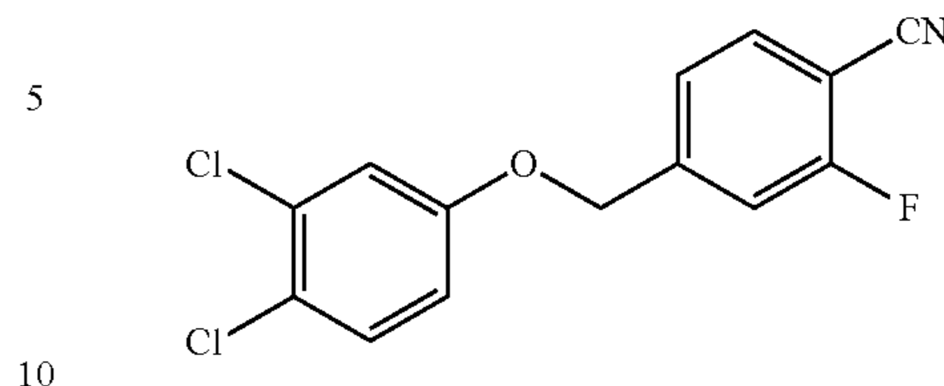
4-((3,4-dichlorophenoxy)methyl)-2-fluorobenzonitrile
