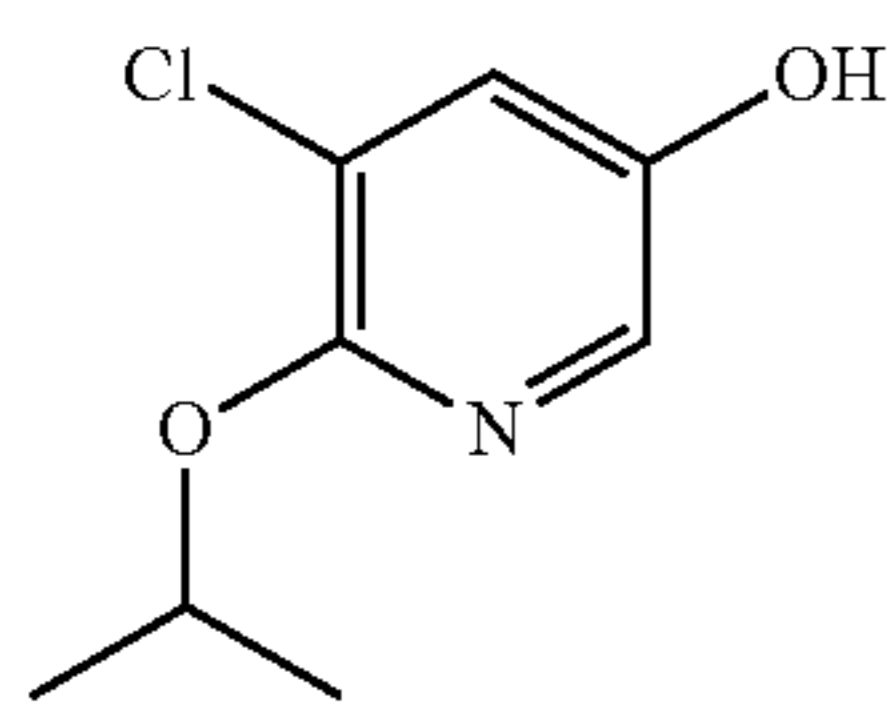
5-chloro-6-isopropoxy-pyridin-3-ol
