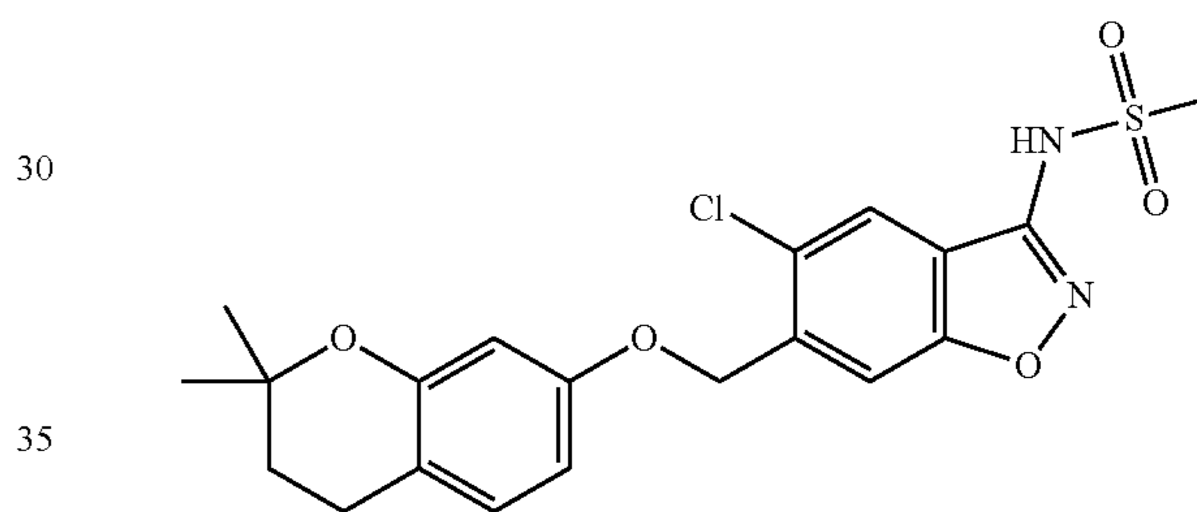
N-(5-chloro-6-((2,2-dimethylchroman-7-yl)oxy)methyl)benzo[d]isoxazol-3-yl)methanesulfonamide
