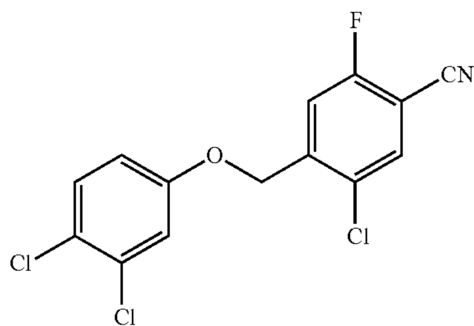
5-chloro-4-((3,4-dichlorophenoxy)methyl)-2-fluorobenzonitrile
