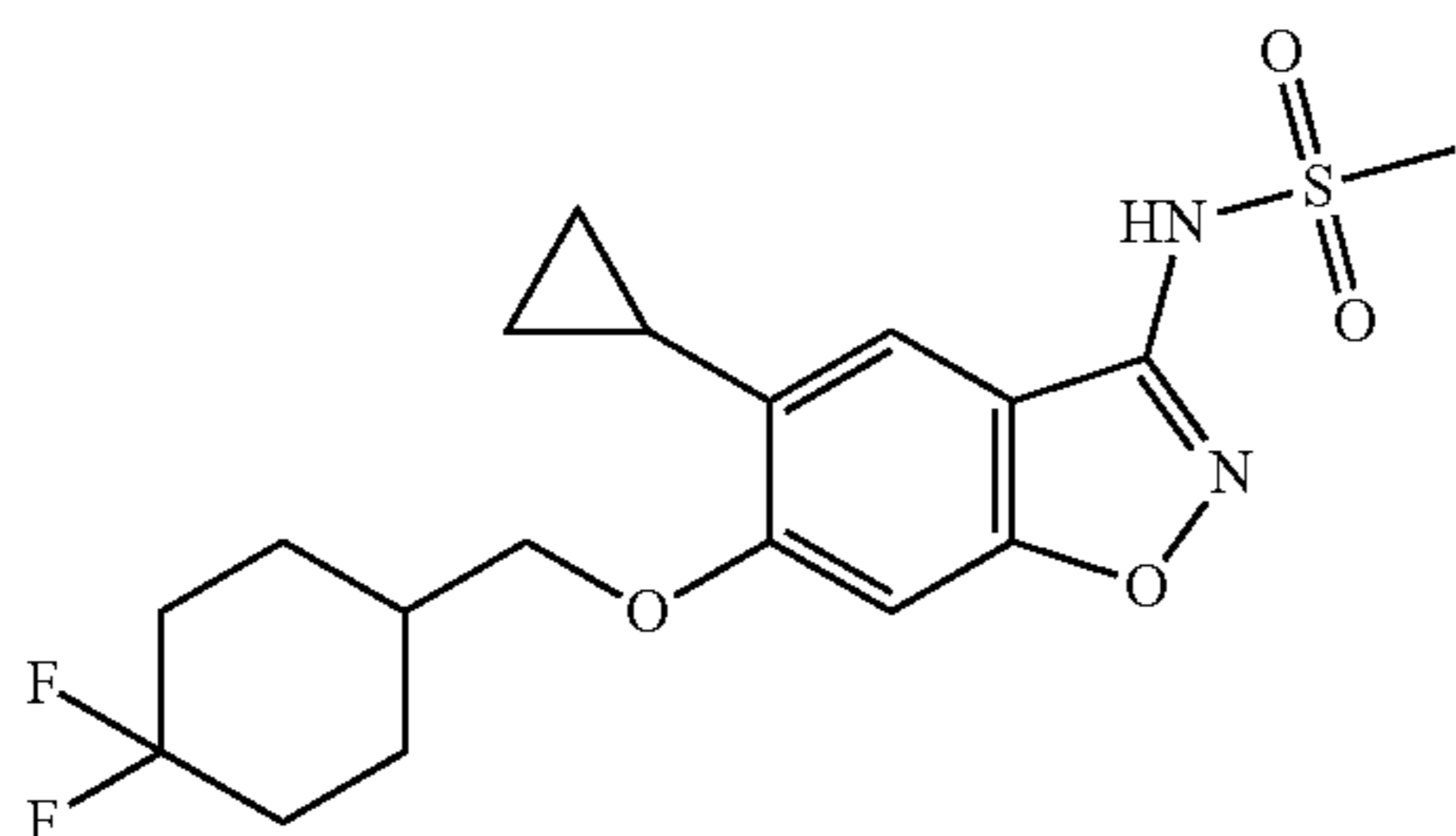
N-(5-cyclopropyl-6-((4,4-difluorocyclohexyl)methoxy)benzo[d]isoxazol-3-yl)-methanesulfonamide
