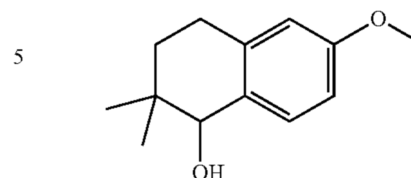
6-methoxy-2,2-dimethyl-1,2,3,4-tetrahydronaphthalen-1-ol
