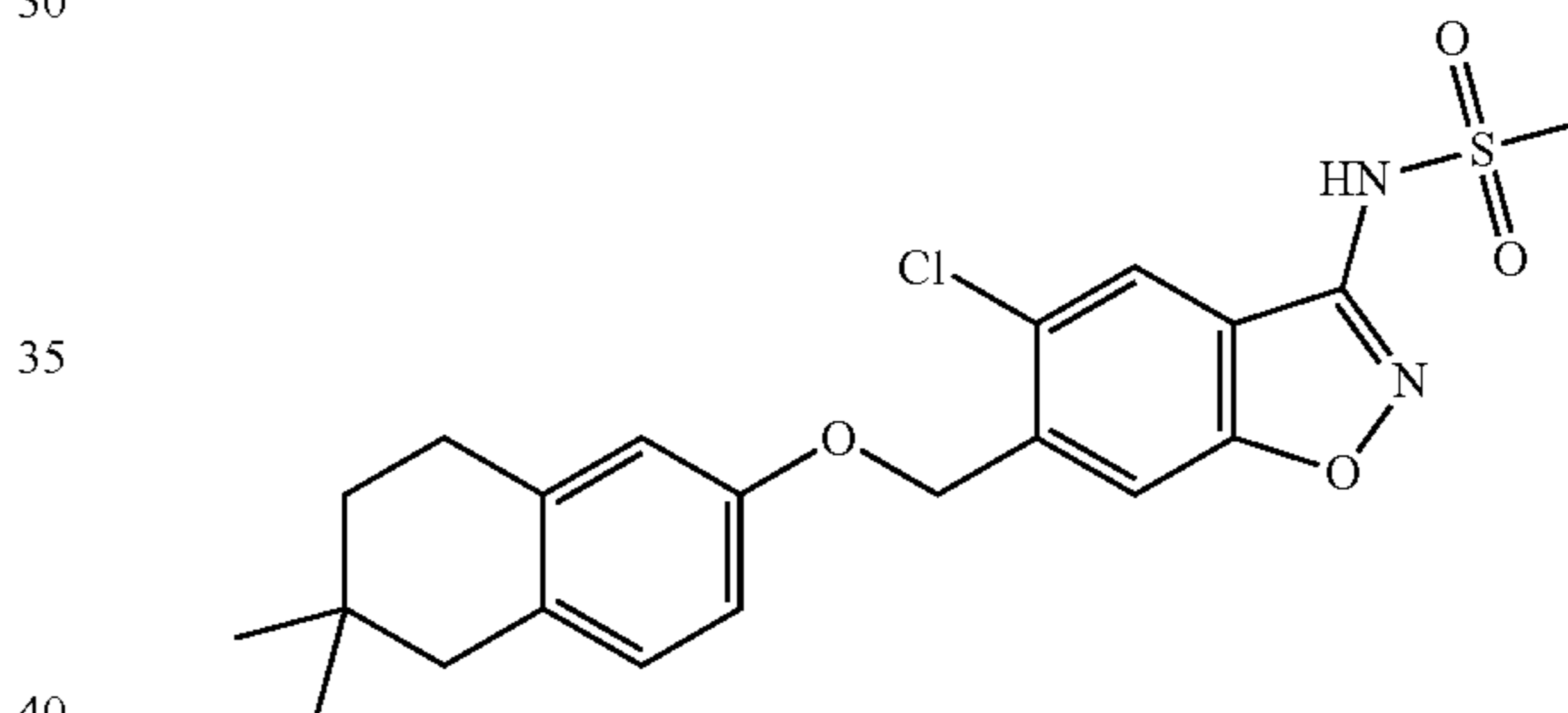
N-(5-chloro-6-((6,6-dimethyl-5,6,7,8-tetrahydronaphthalen-2-yloxy)methyl)benzo[d]-isoxazol-3-yl)methanesulfonamide
