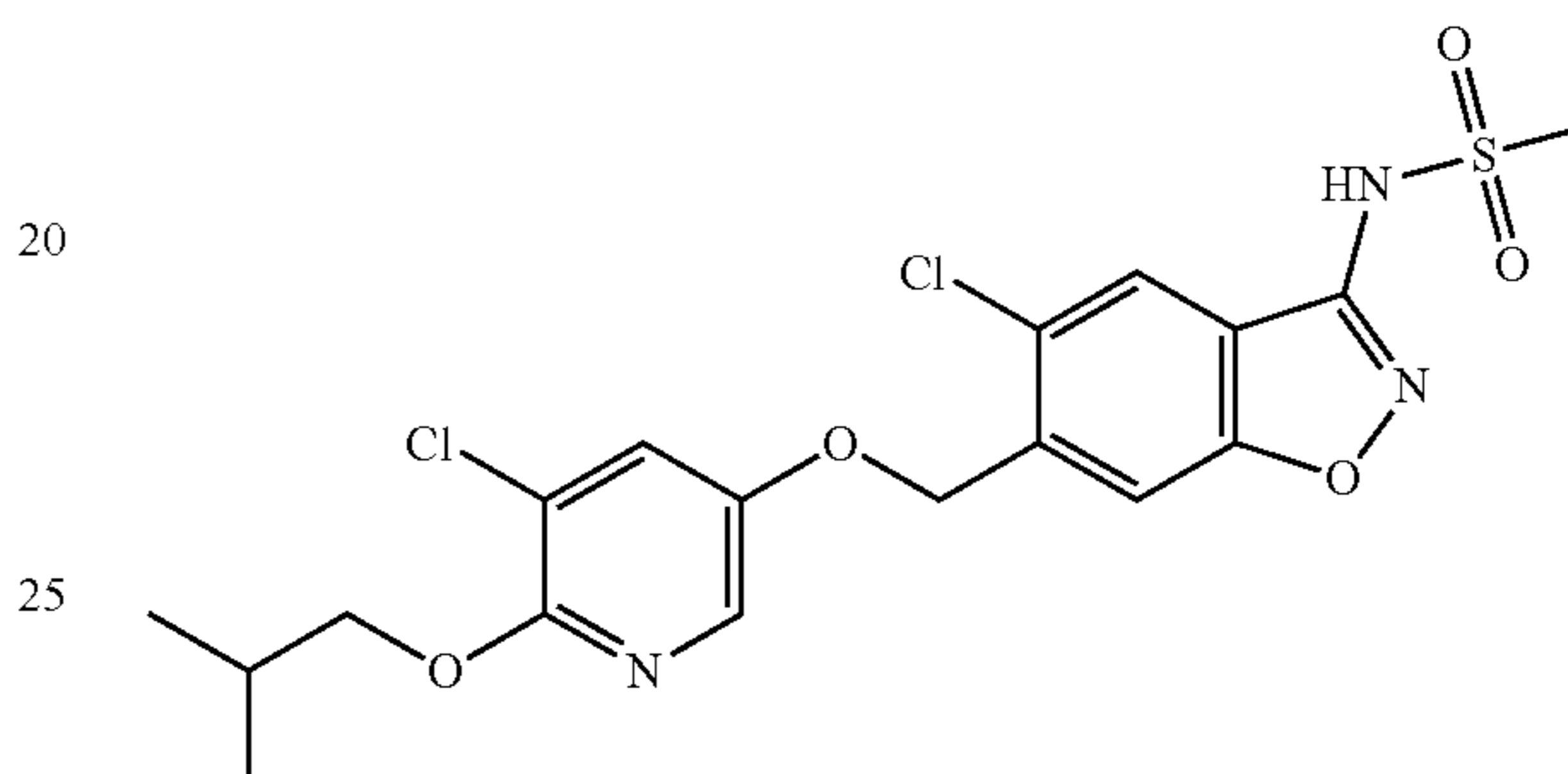
N-(5-chloro-6-((5-chloro-6-isobutoxypyridin-3-yl)oxy)methyl)benzo[d]isoxazol-3-yl)-methanesulfonamide
