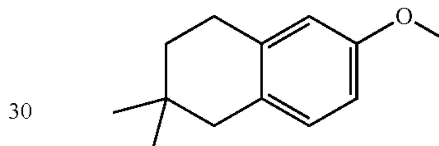
6-methoxy-2,2-dimethyl-1,2,3,4-tetrahydronaphthalene
