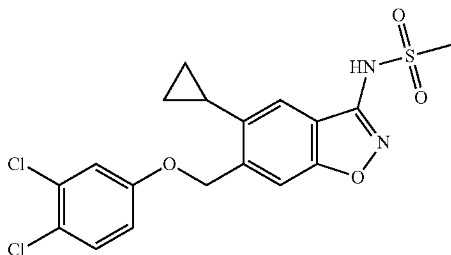
N-(5-cyclopropyl-6-((3,4-dichlorophenoxy)methyl)benzo[d]isoxazol-3-yl)-methanesulfonamide
