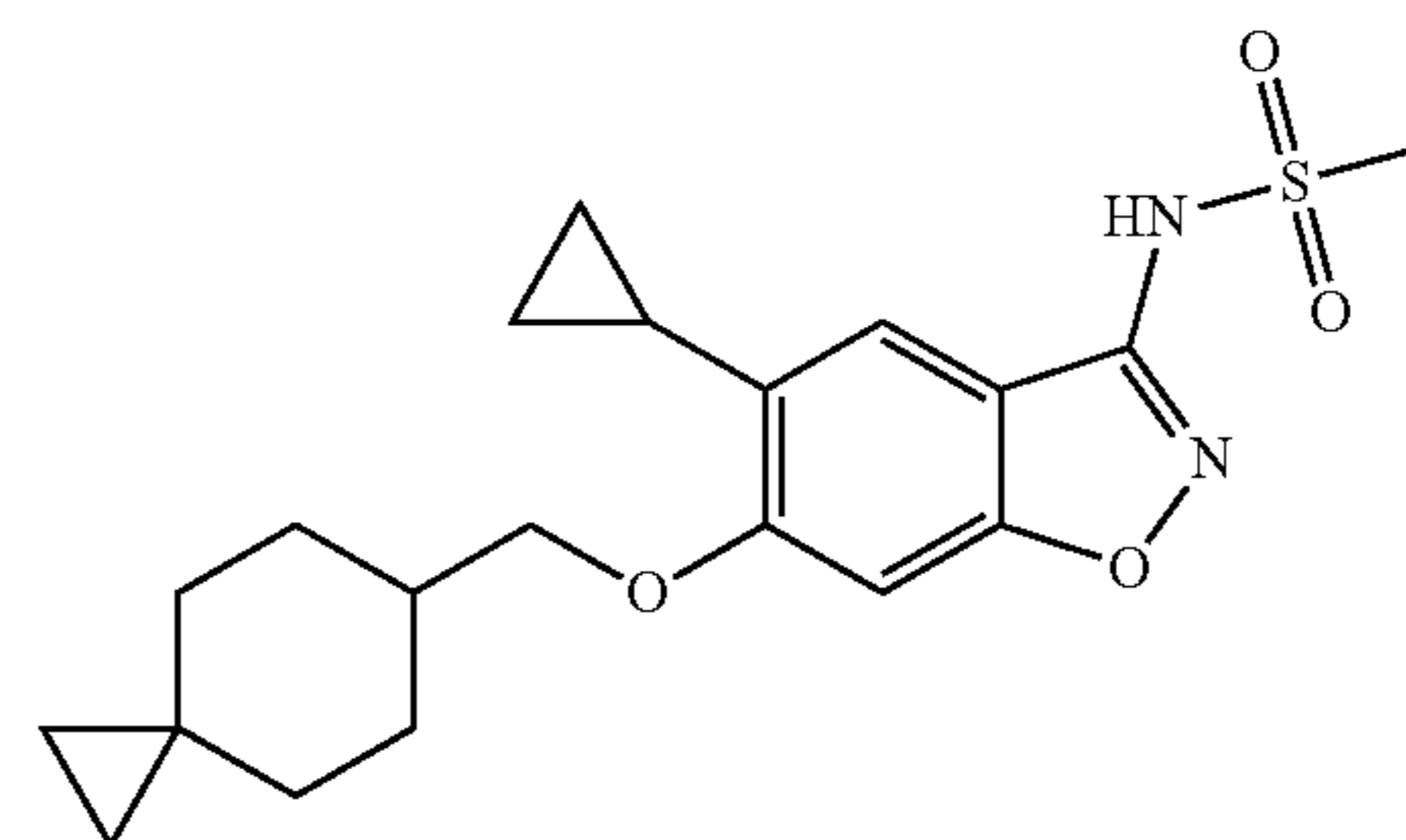
N-(5-cyclopropyl-6-{spiro[2.5]octan-6-ylmethoxy}-1,2-benzoxazol-3-yl)-methanesulfonamide
