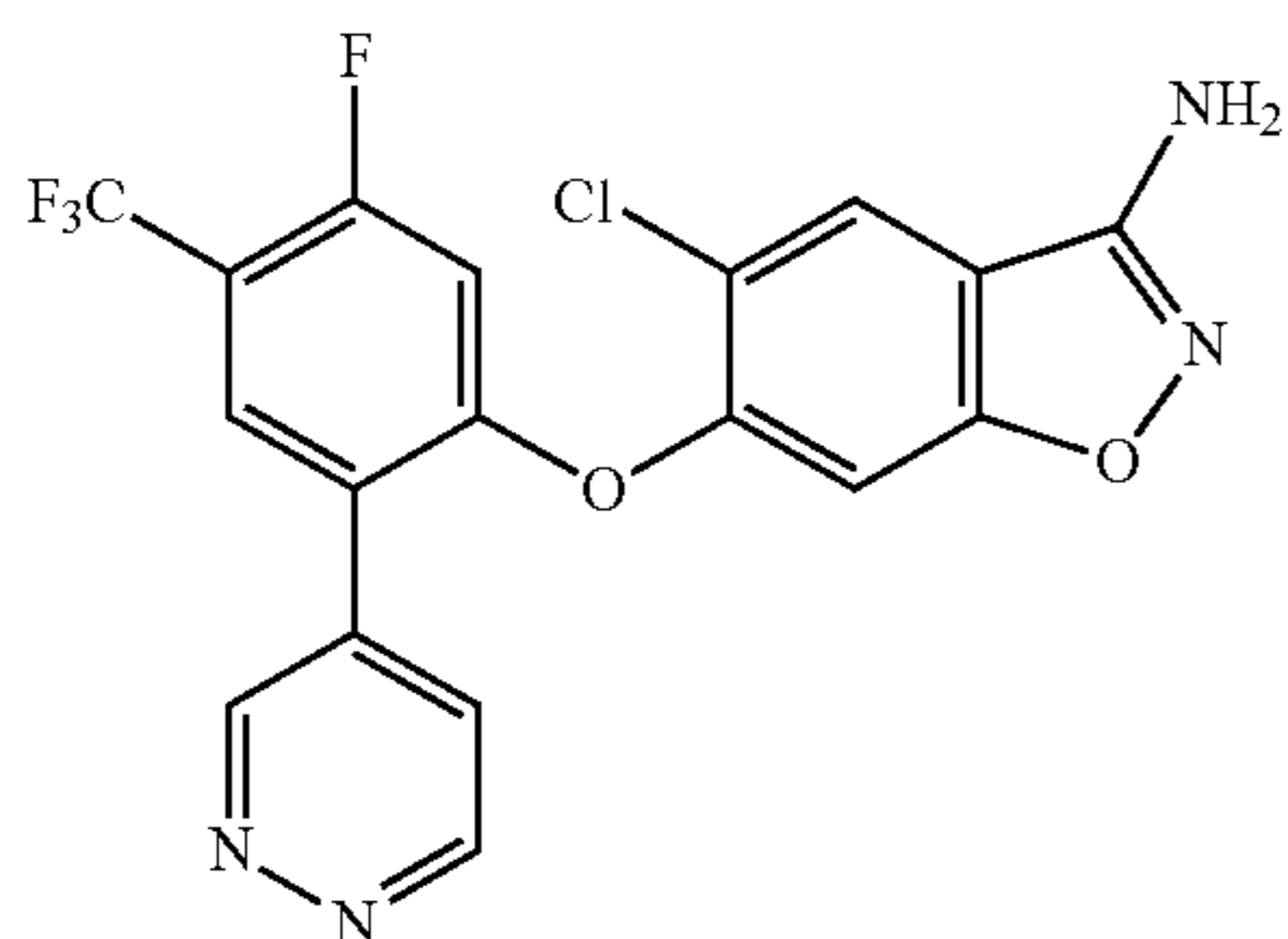
5-chloro-6-(5-fluoro-2-(pyridazin-4-yl)-4-(trifluoromethyl)phenoxy)benzo[d]isoxazol-3-amine
