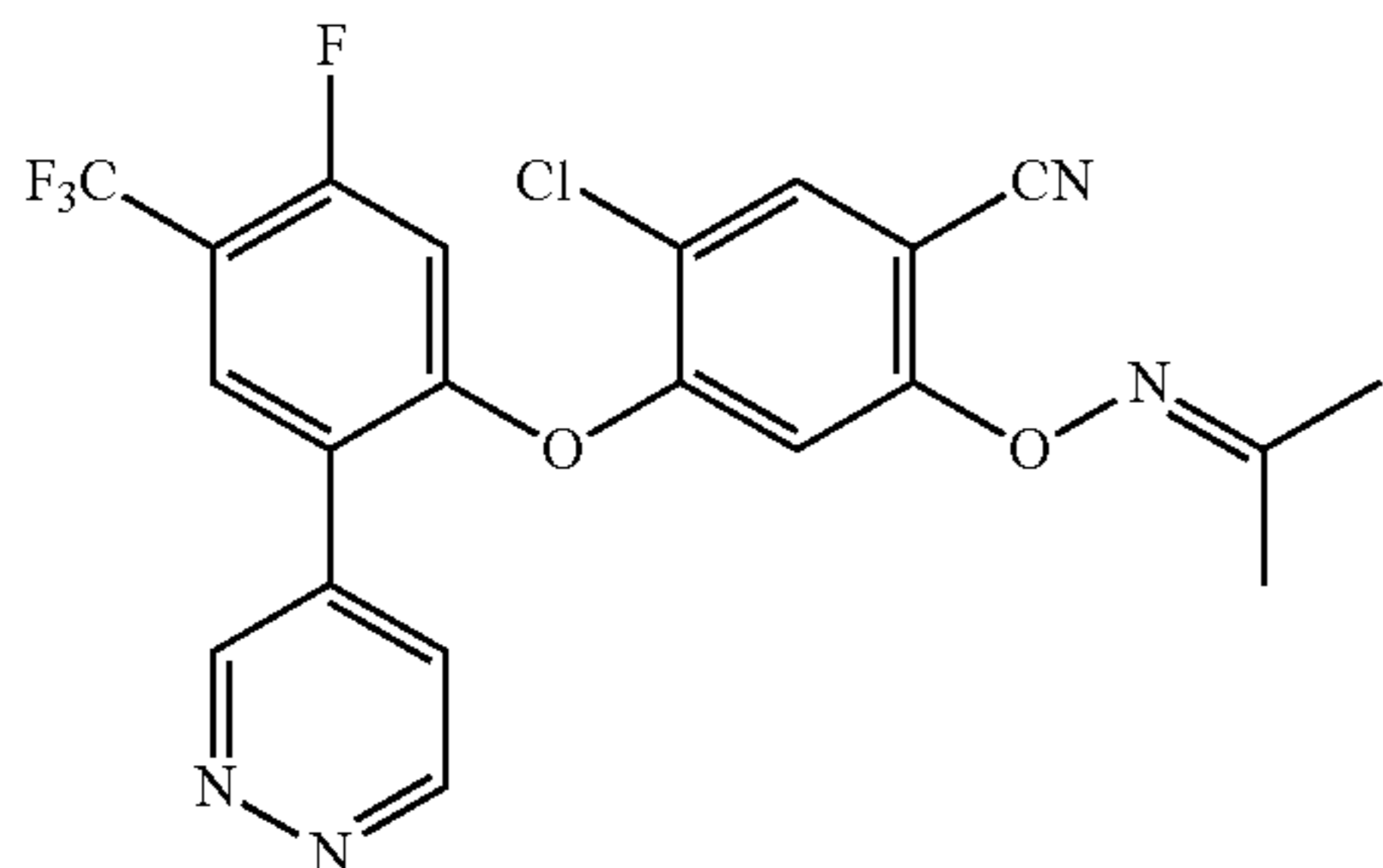
5-chloro-4-(5-fluoro-2-(pyridazin-4-yl)-4-(trifluoromethyl)phenoxy)-2-(propan-2-ylideneaminoxy)benzonitrile
