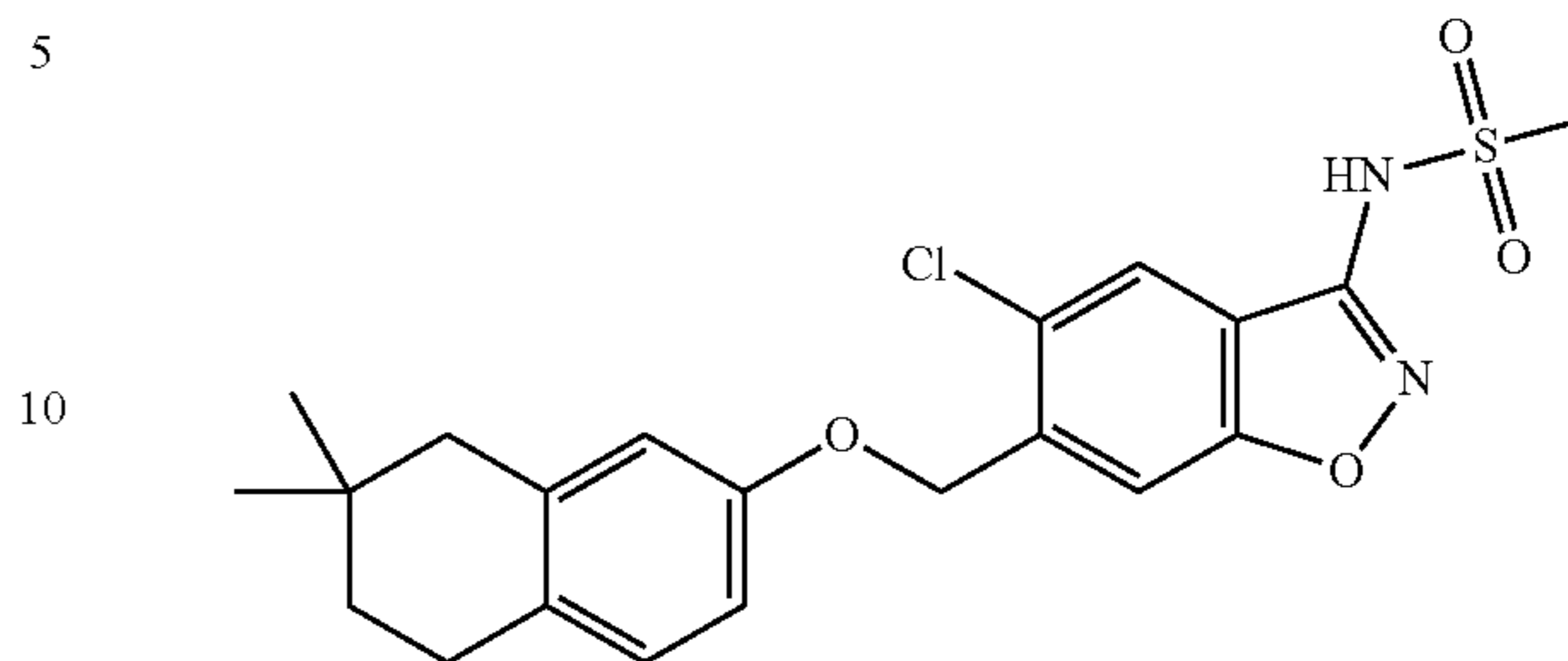
N-(5-chloro-6-((7,7-dimethyl-5,6,7,8-tetrahydronaphthalen-2-yloxy)methyl)benzo[d]-isoxazol-3-yl)methanesulfonamide
