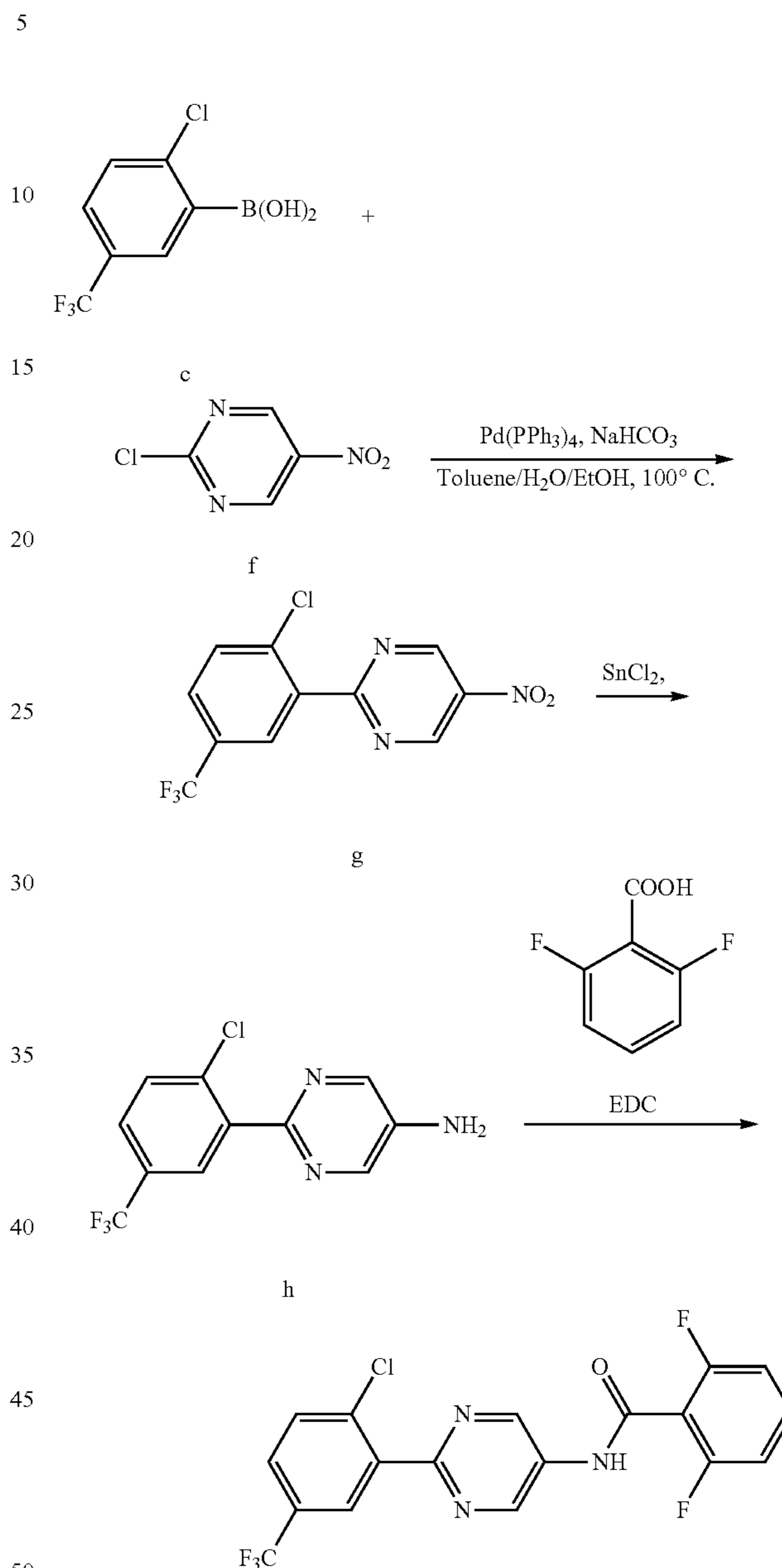
Compound 122
