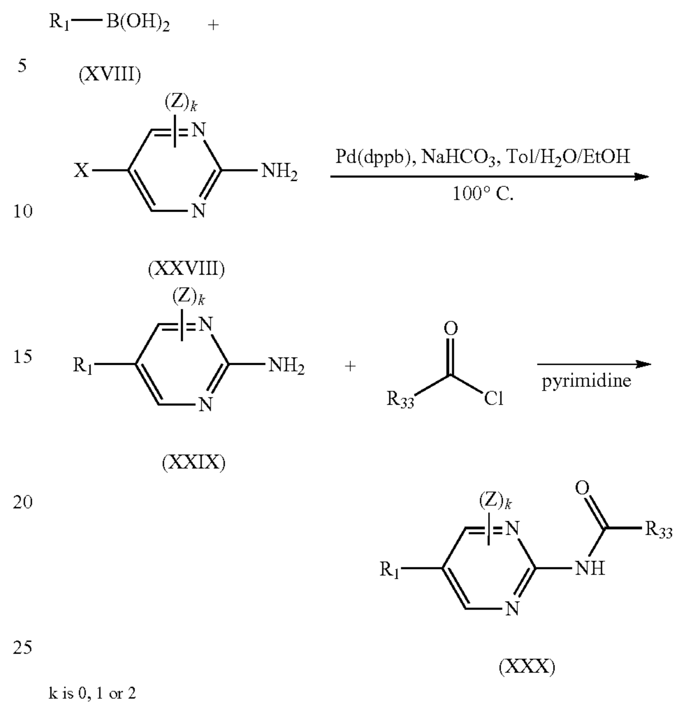
Scheme V
