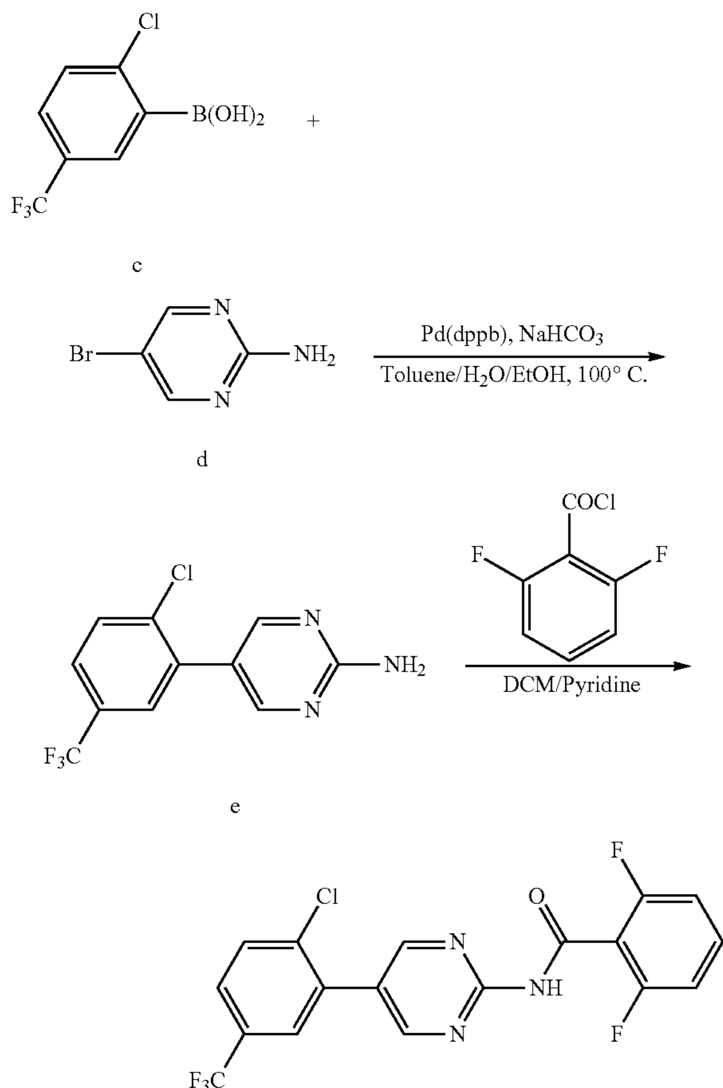
Compound 116
