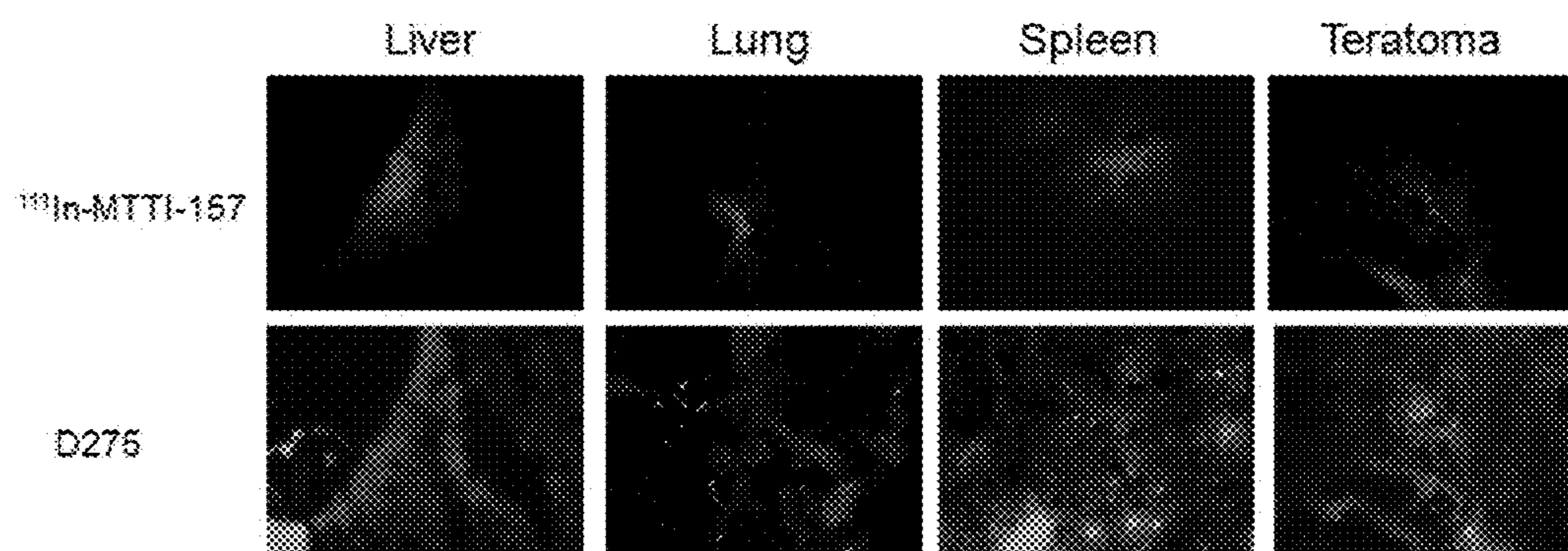
FIG. 8. Fluorescence microscopy of frozen sections from liver, lung, and spleen from a mouse sacrificed on day 10 after injection by tail vein of ^{111}\text{In-MTTI-157} labeled stem cells, and a teratoma from mouse on day 14 with subcutaneous injection on the shoulder. The first row, red fluorescence is ^{111}\text{In-MTTI-157} ; the second row, green fluorescence is dye D275 (Ex: 484 nm, Em: 501 nm) which was used here to stain the field of view. Magnification: 200x.
