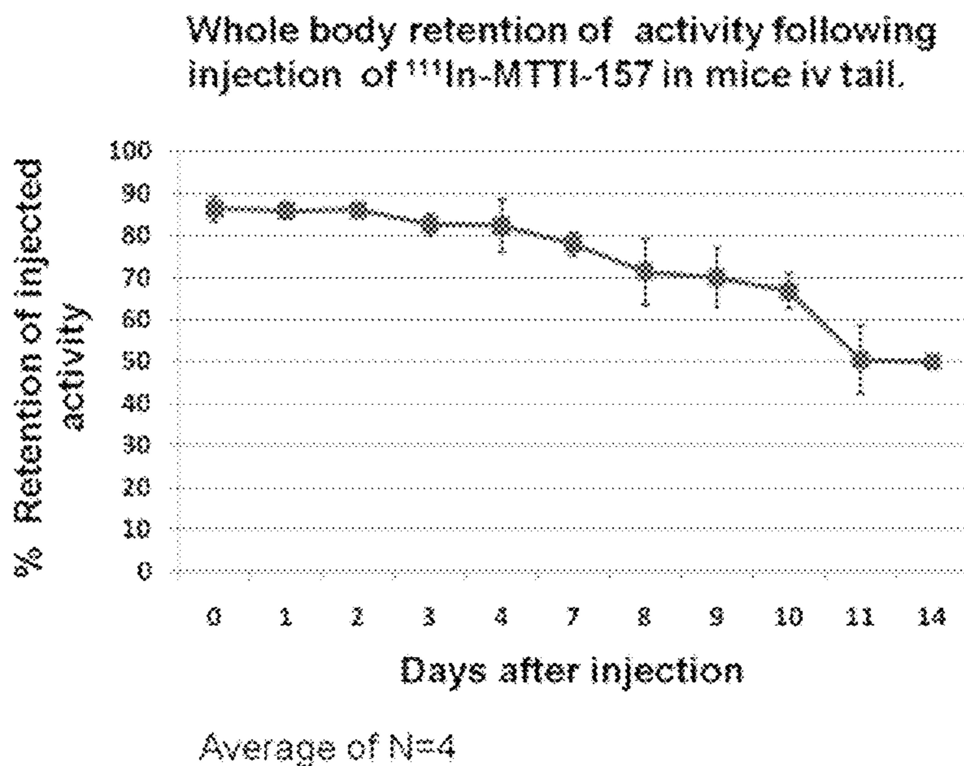
FIG. 21. Whole body 111 In activity through 14 days (corrected for decay).
