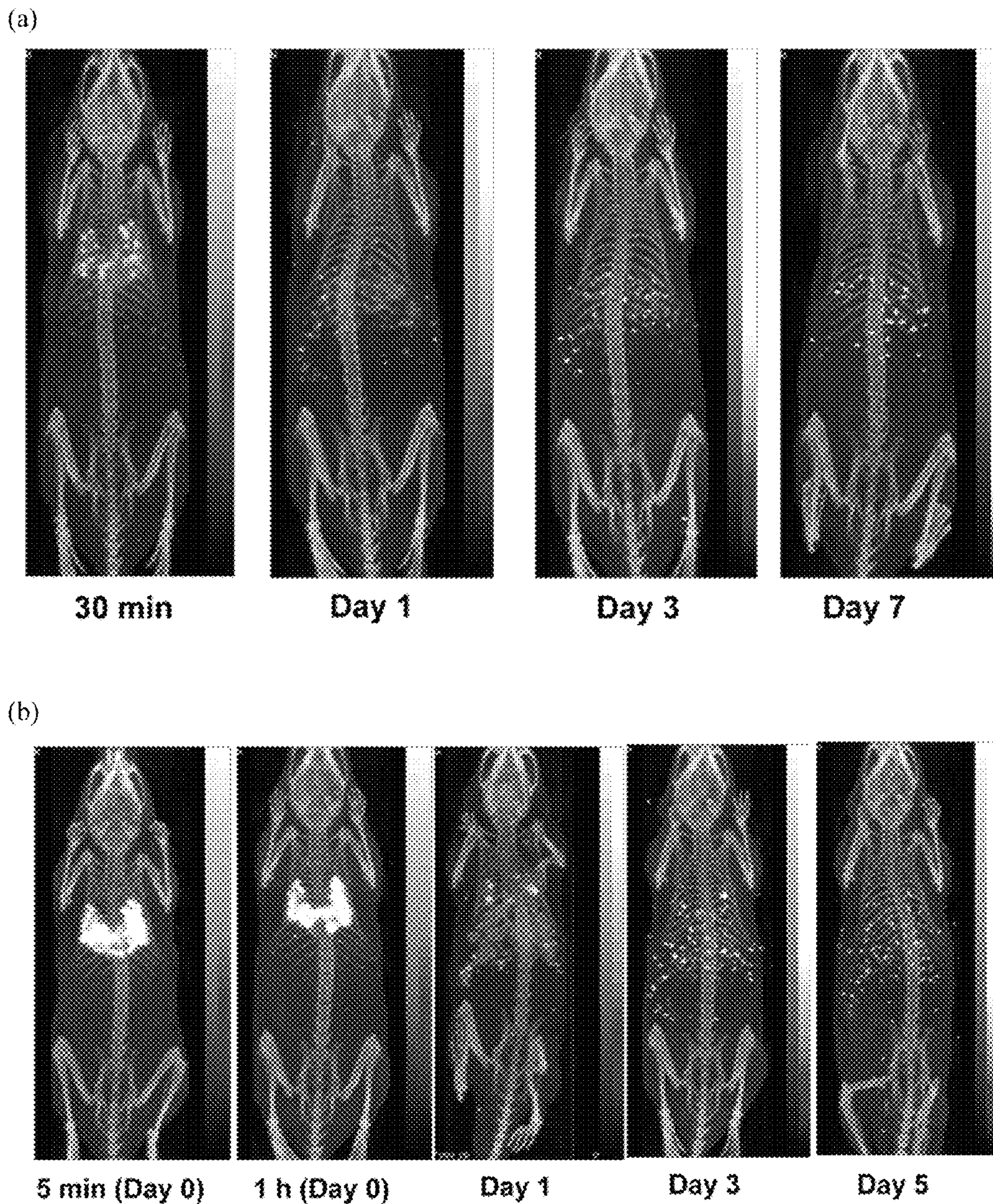
FIG. 20. ^{111}\text{In} -MTTI-157 labeled cells (12-14 \mu\text{Ci} on 2 \times 10^6 cells) were injected IV into SKH-1 mice. Radioactivity was observed by SPECT/CT through day 7 in (a) and through day 5 (b). Activity is in the lungs in the early images and then distributes to the liver and spleen.
