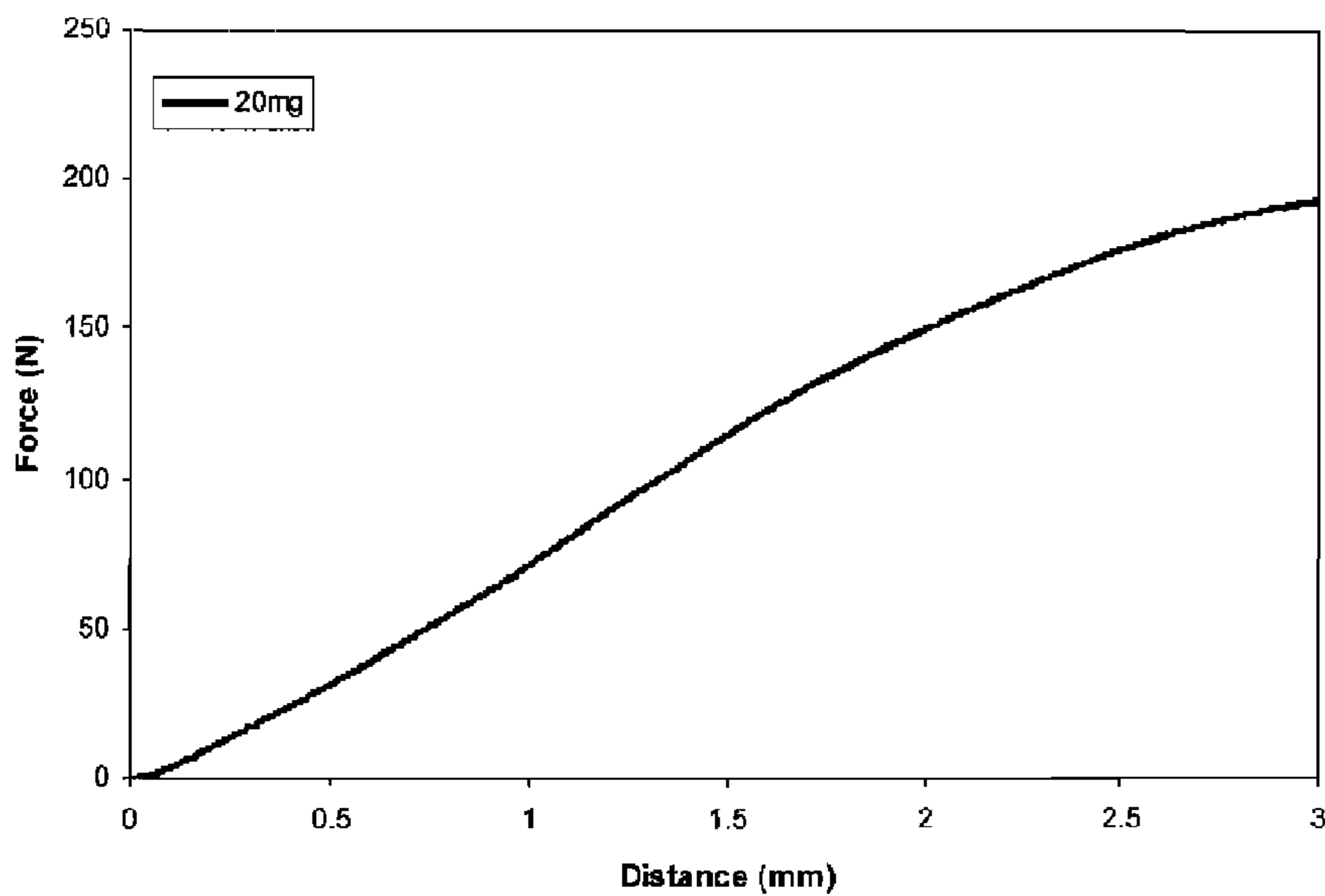
Example 20 Indentation Test of Example 13.3 tablet
