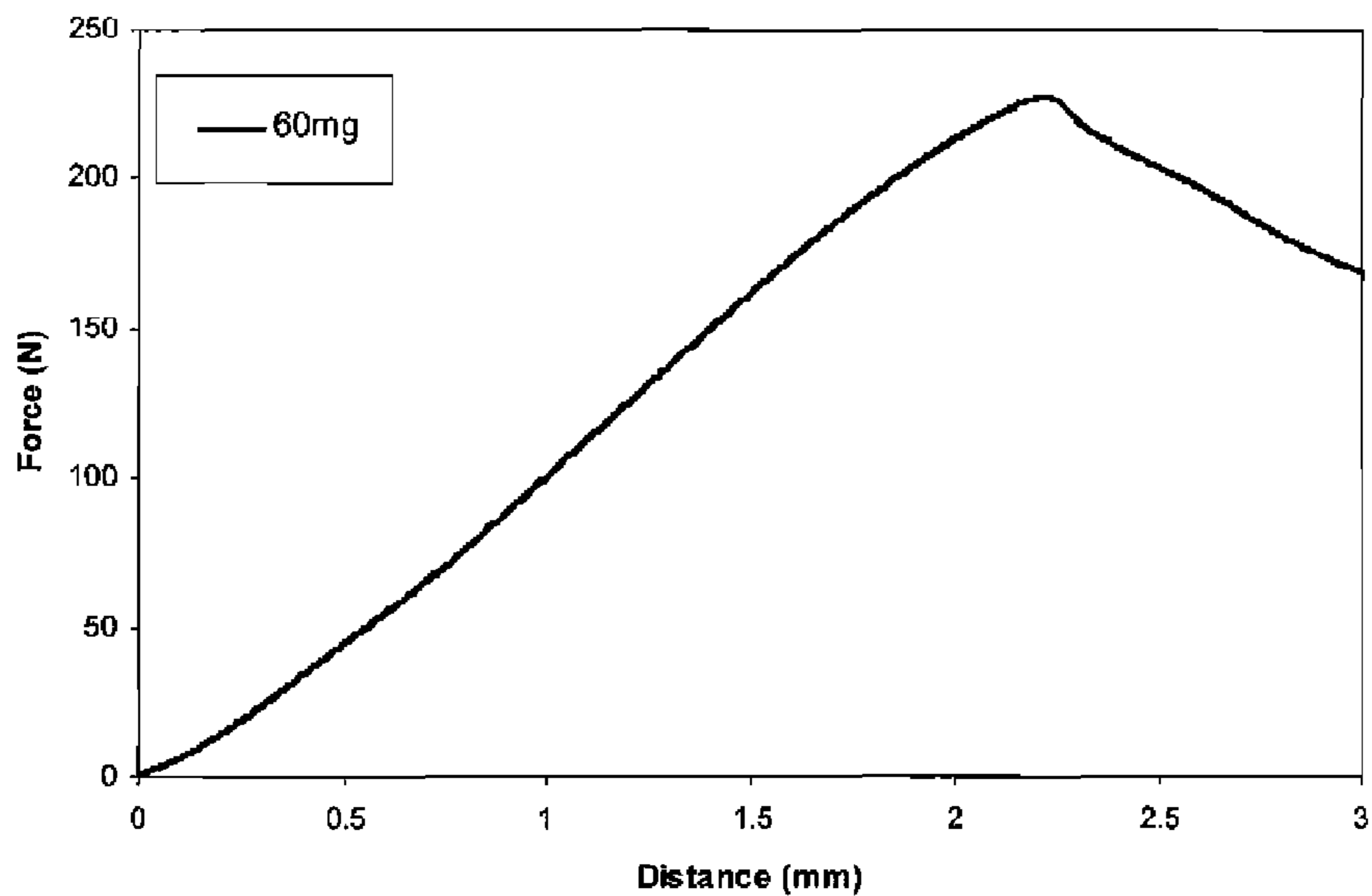
Example 20 Indentation Test of Example 16.1 tablet
