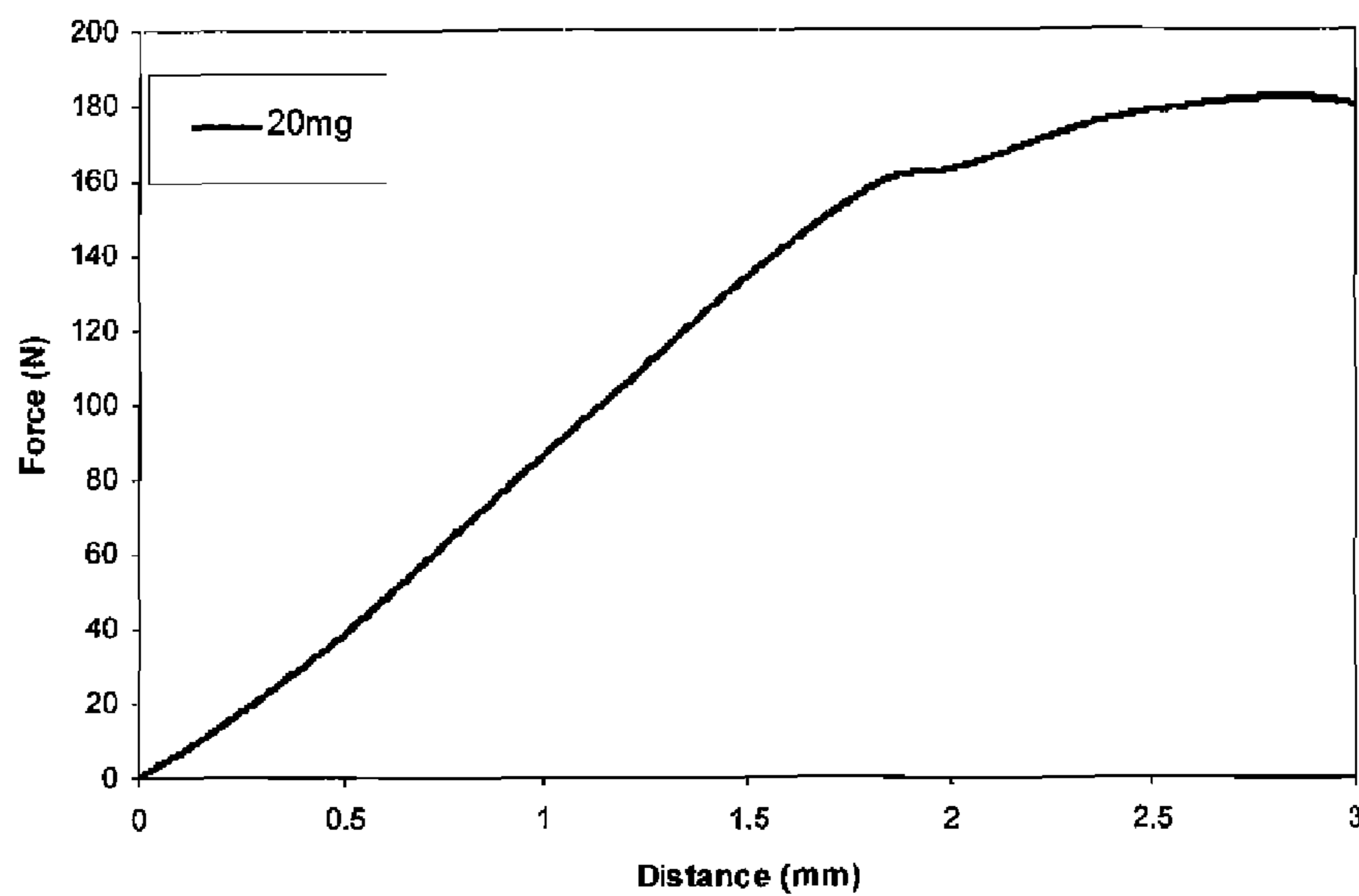
Example 20 Indentation Test of Example 14.3 tablet
