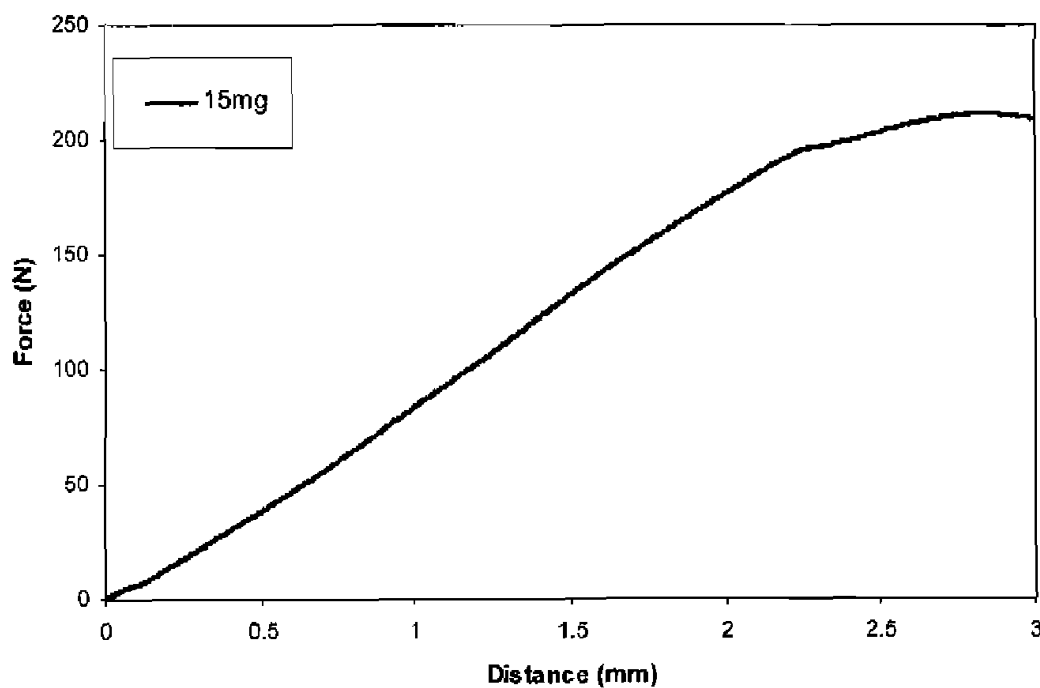
Example 20 Indentation Test of Example 14.2 tablet
