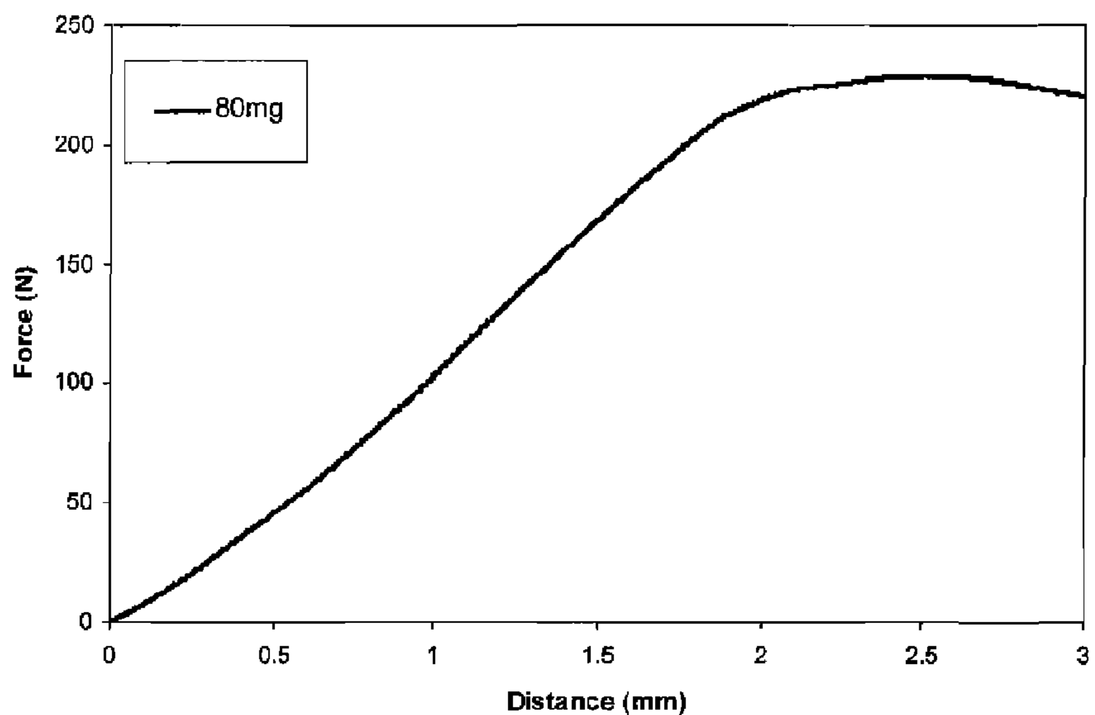
Example 20 Indentation Test of Example 16.2 tablet
