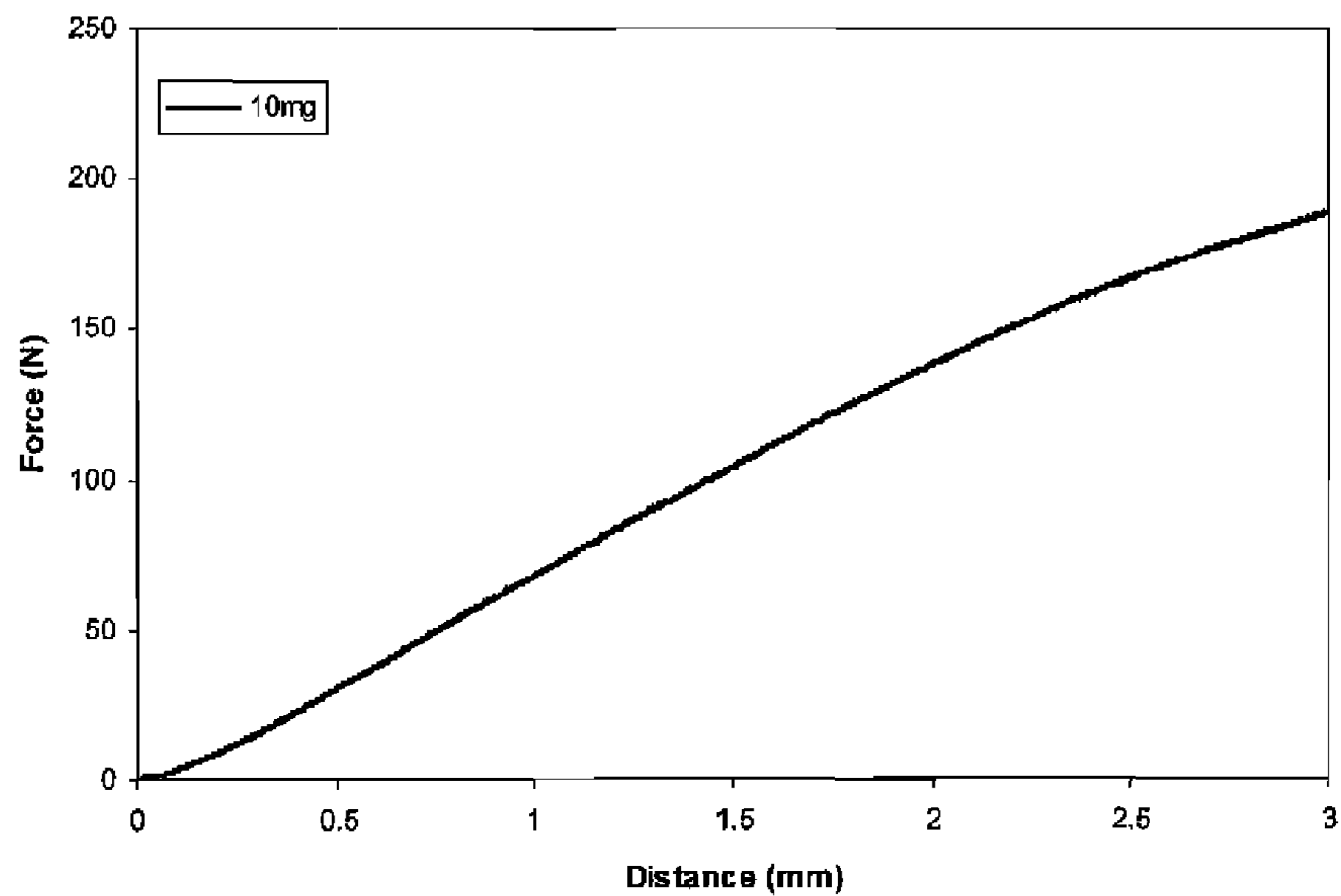
Example 20 Indentation Test of Example 13.1 tablet
