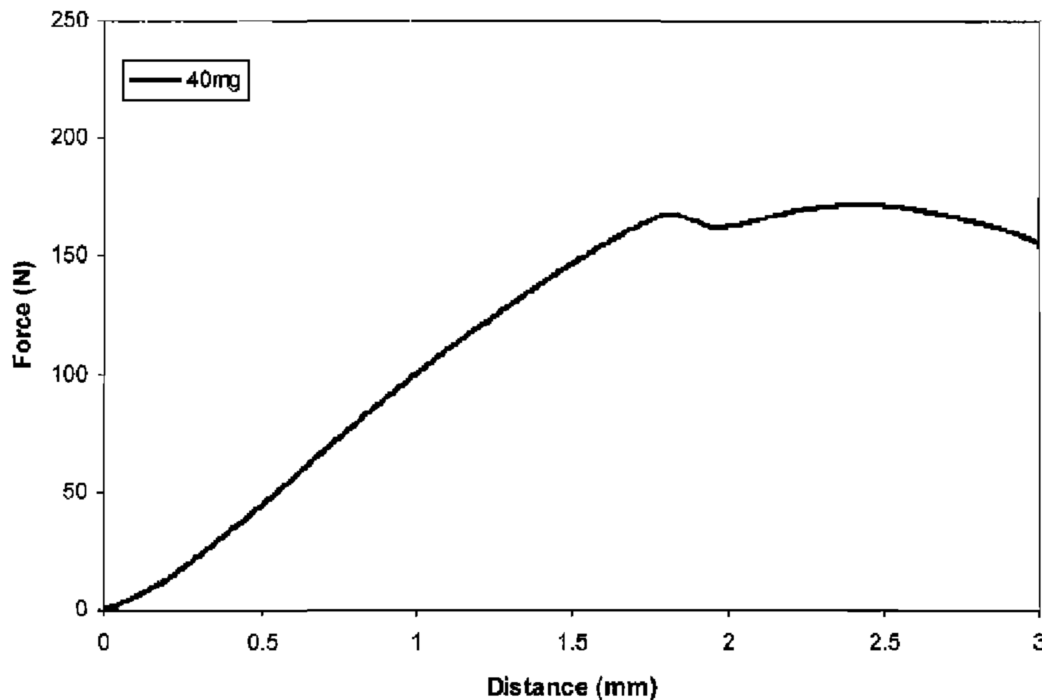
Example 20 Indentation Test of Example 13.5 tablet
