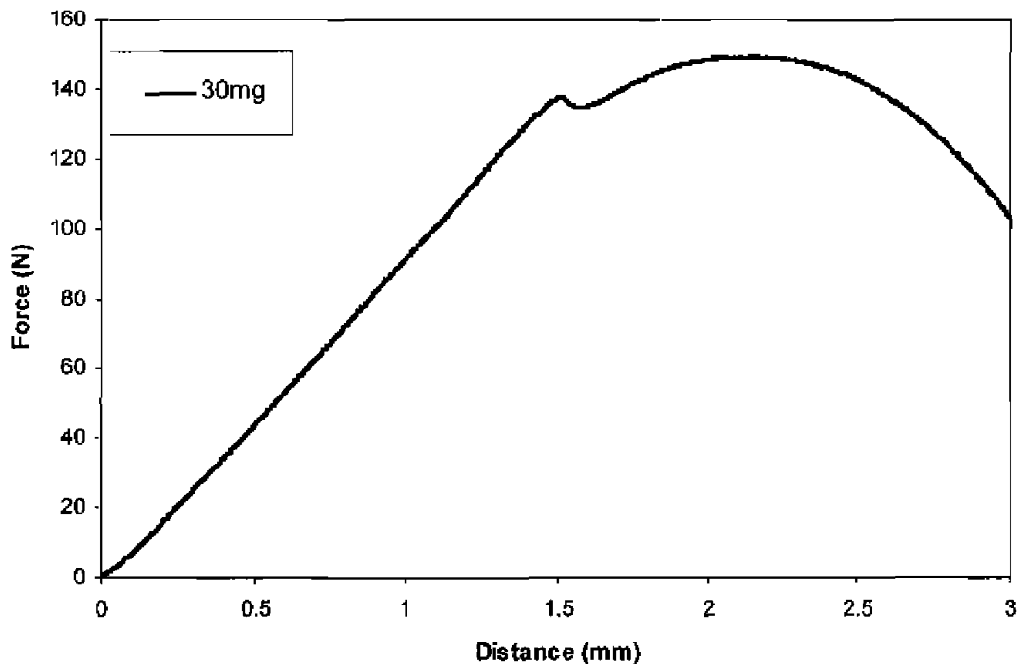
Example 20 Indentation Test of Example 14.4 tablet
