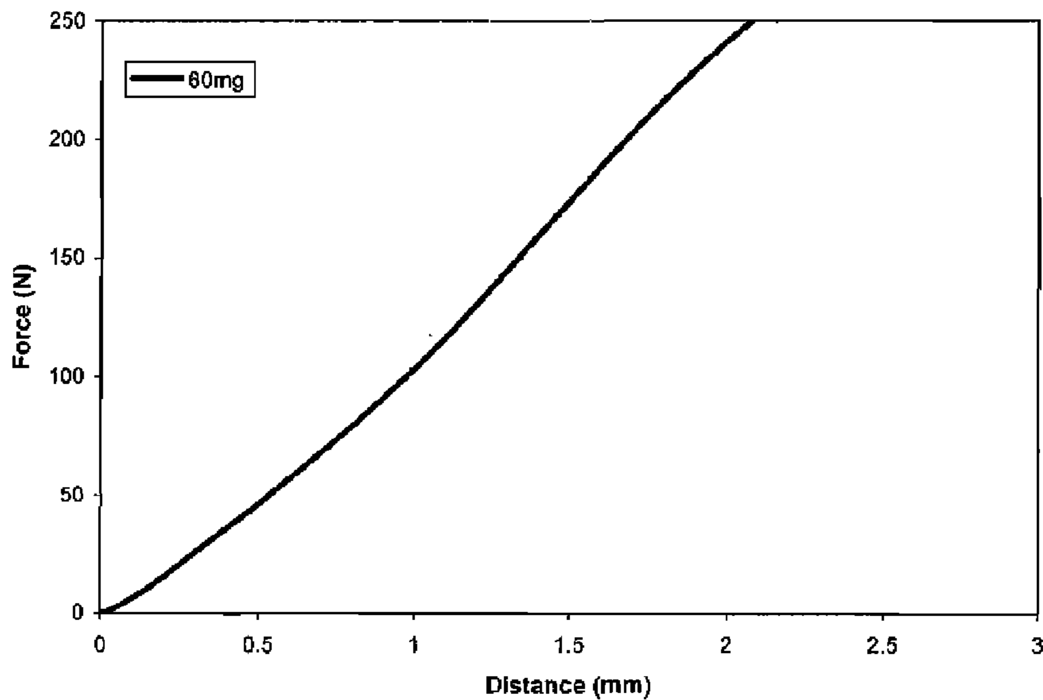
Example 20 Indentation Test of Example 17.1 tablet
