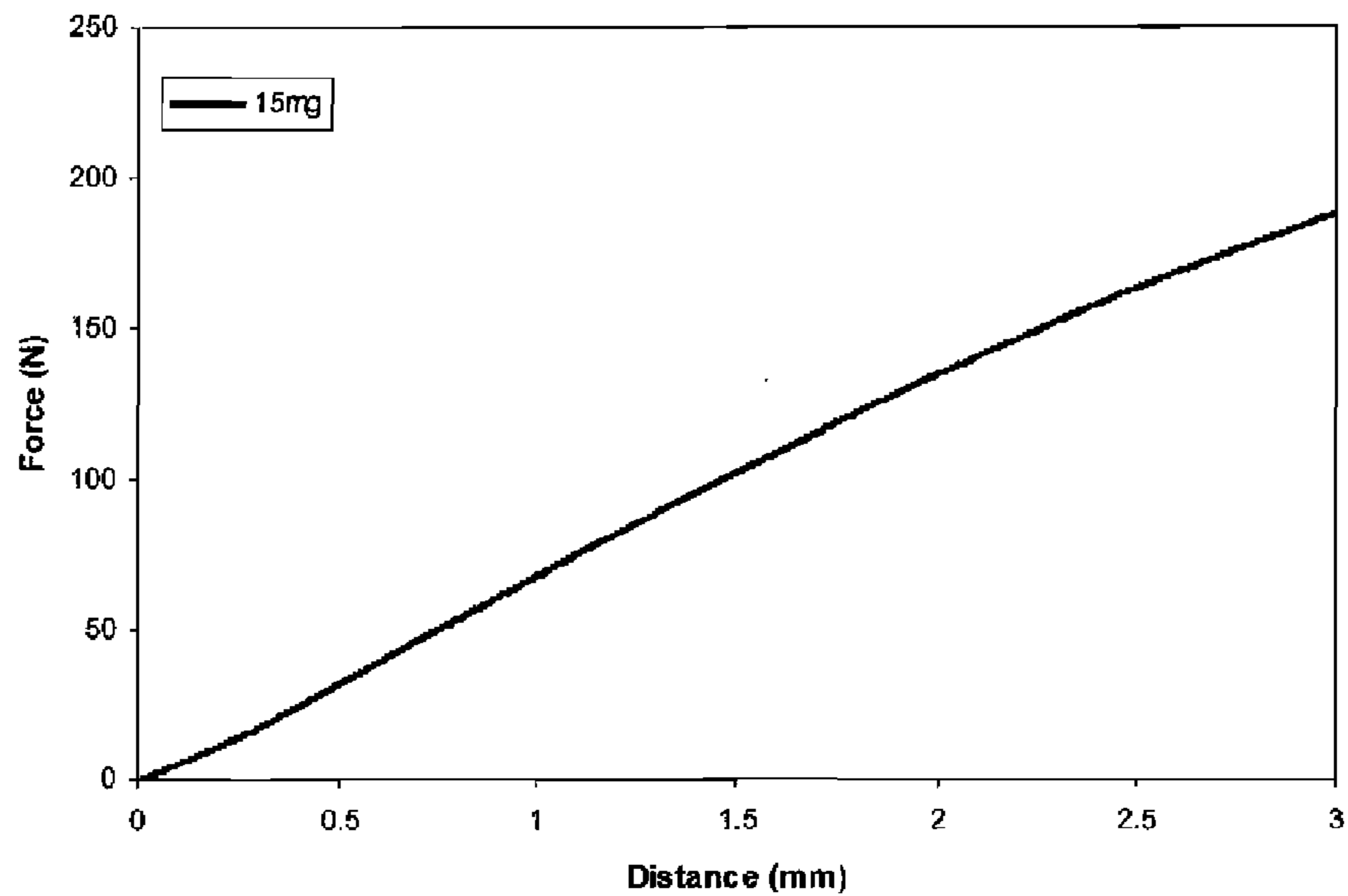
Example 20 Indentation Test of Example 13.2 tablet
