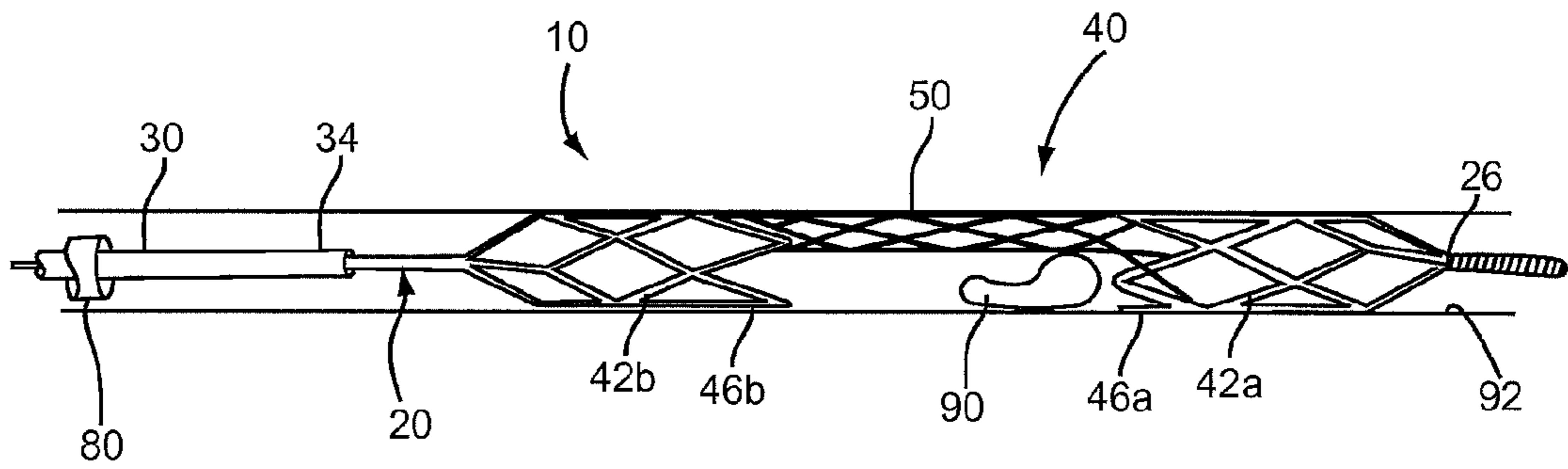
FIG. 2D
