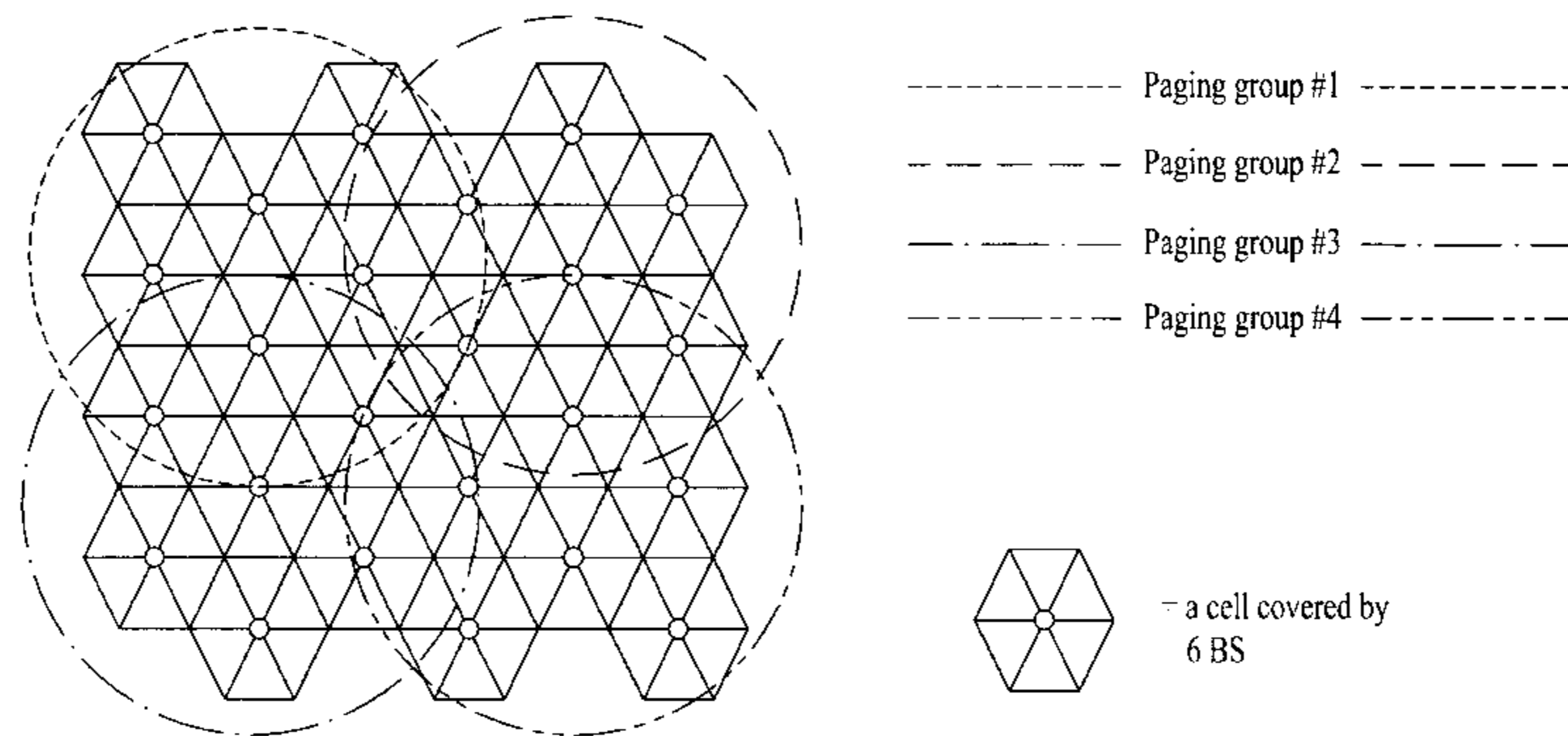
Figure 166-Paging groups example
