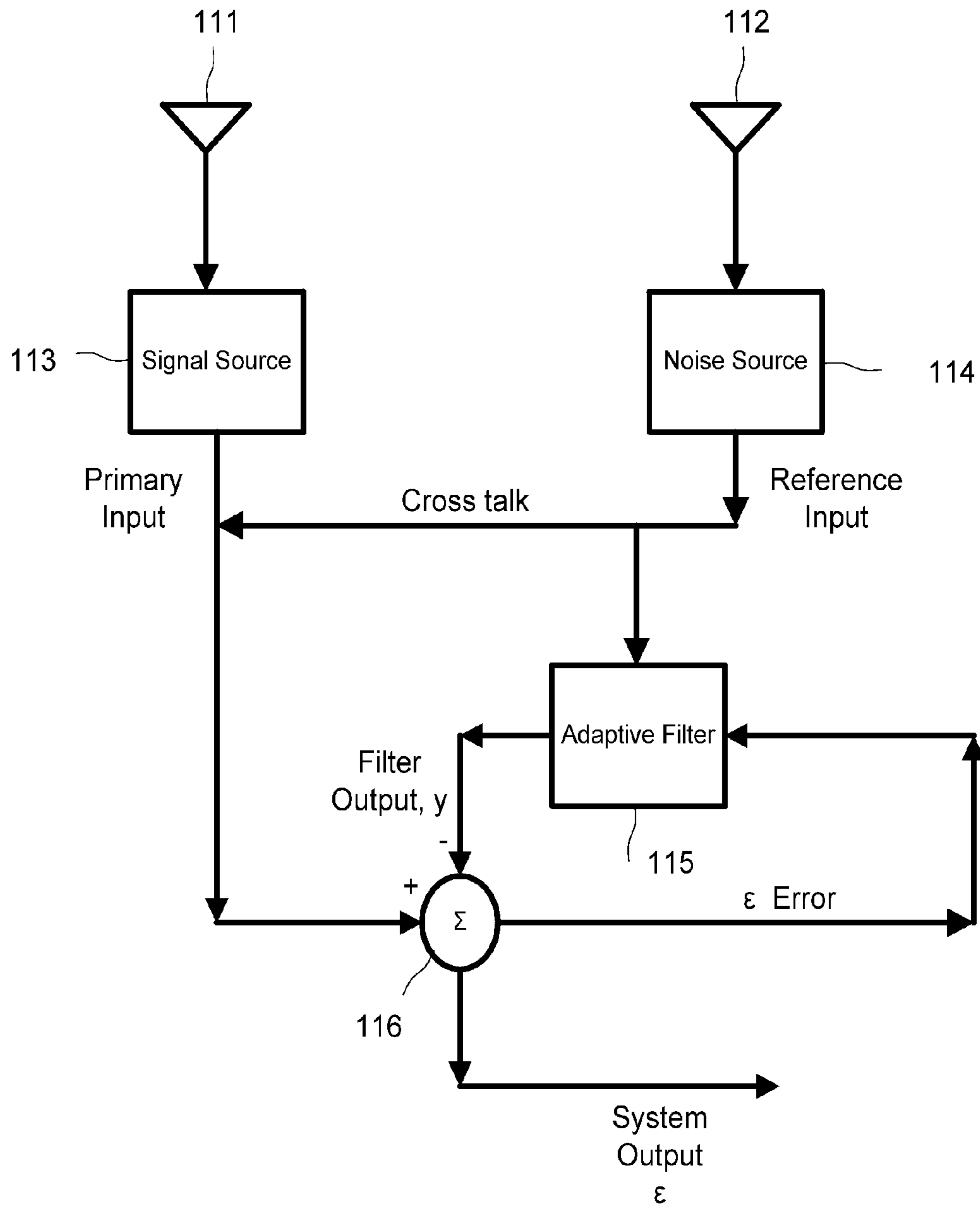
FIG. 1 PRIOR ART
