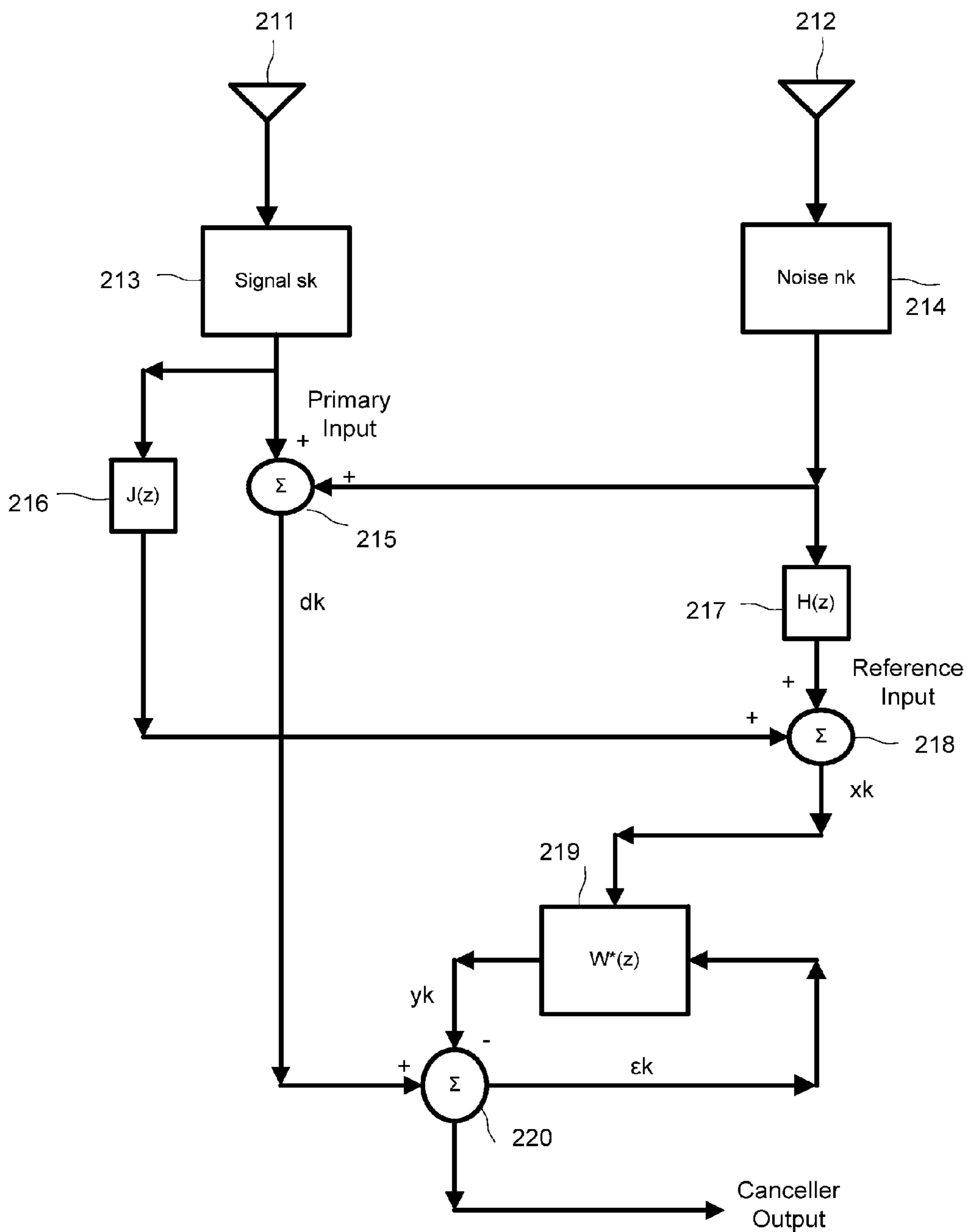
FIG. 2 PRIOR ART
