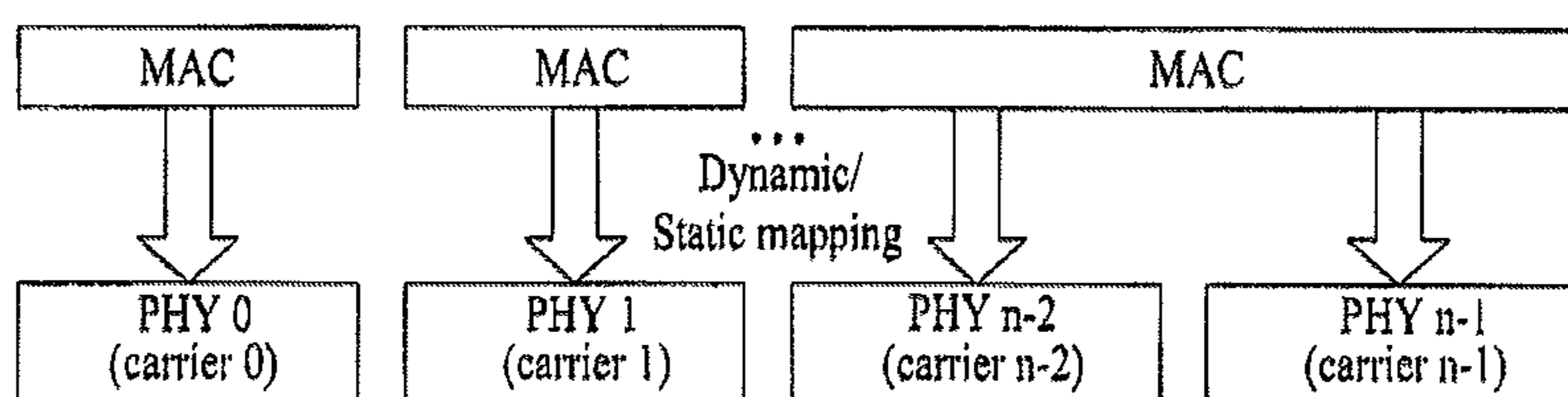
(a) Transmitter
