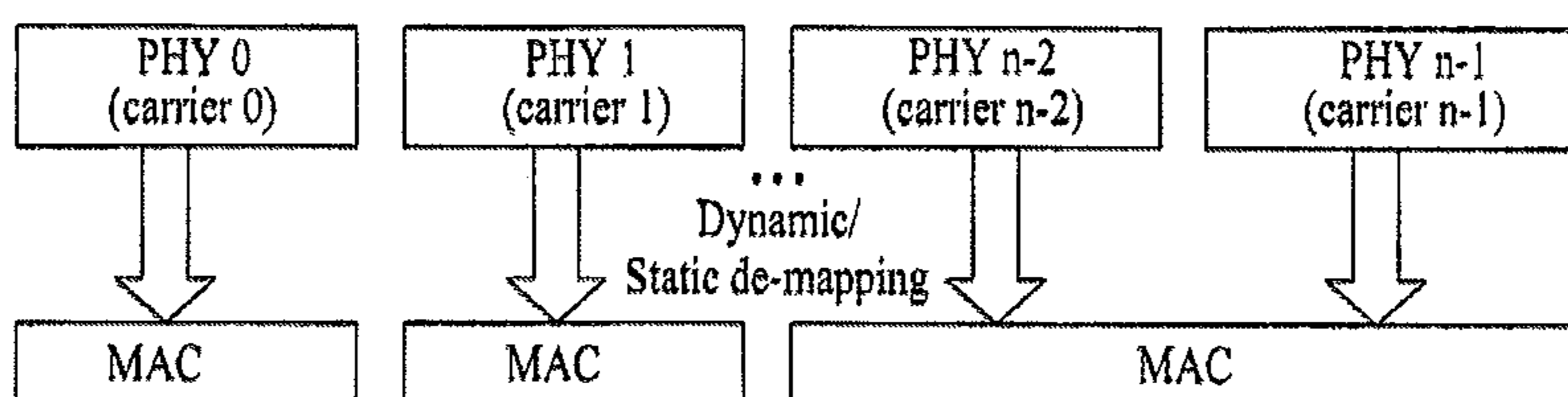
(b) Receiver
