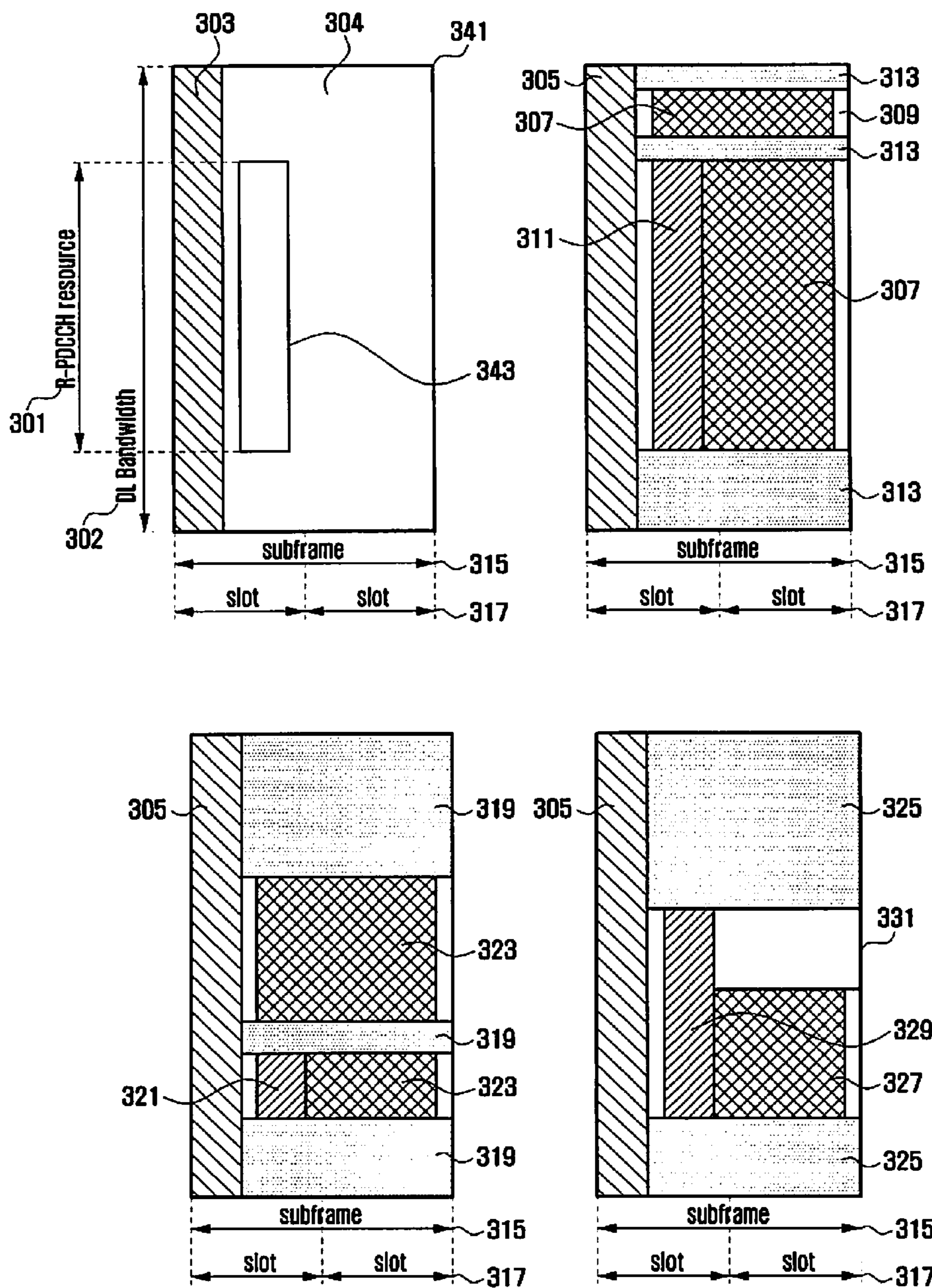
FIG. 1 (PRIOR ART)
