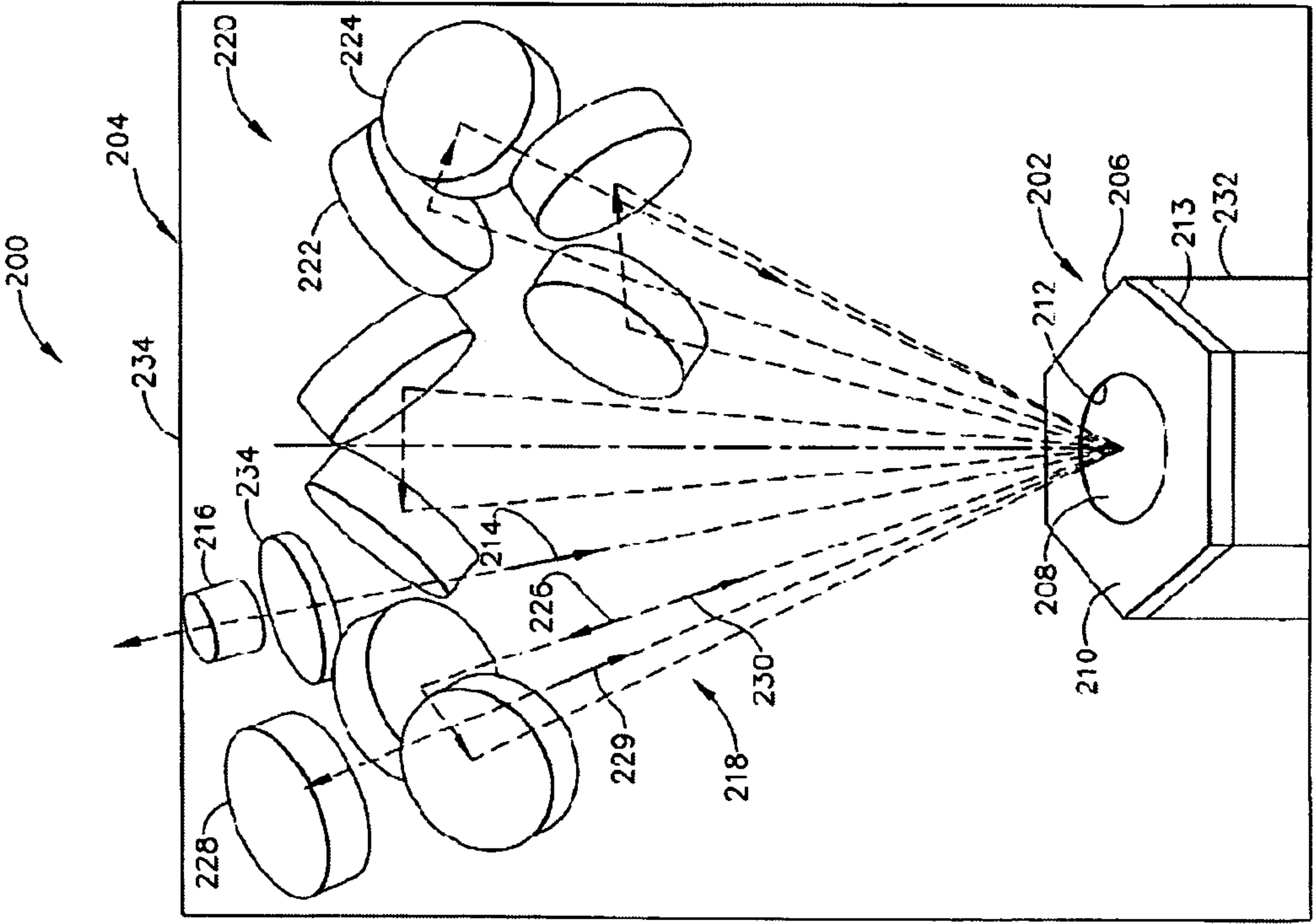
FIG. 2 (PRIOR ART)
