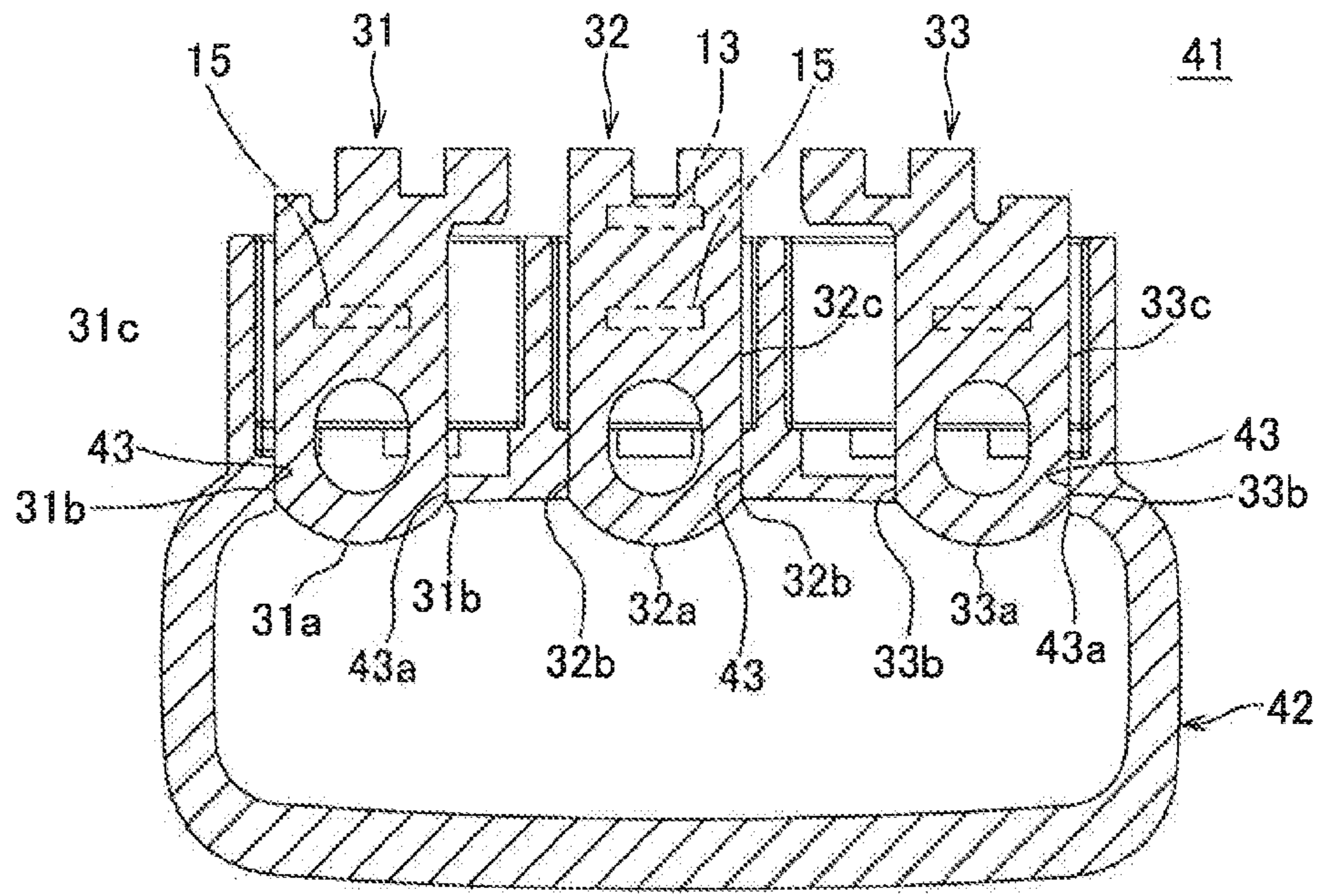
FIG. 6 PRIOR ART
