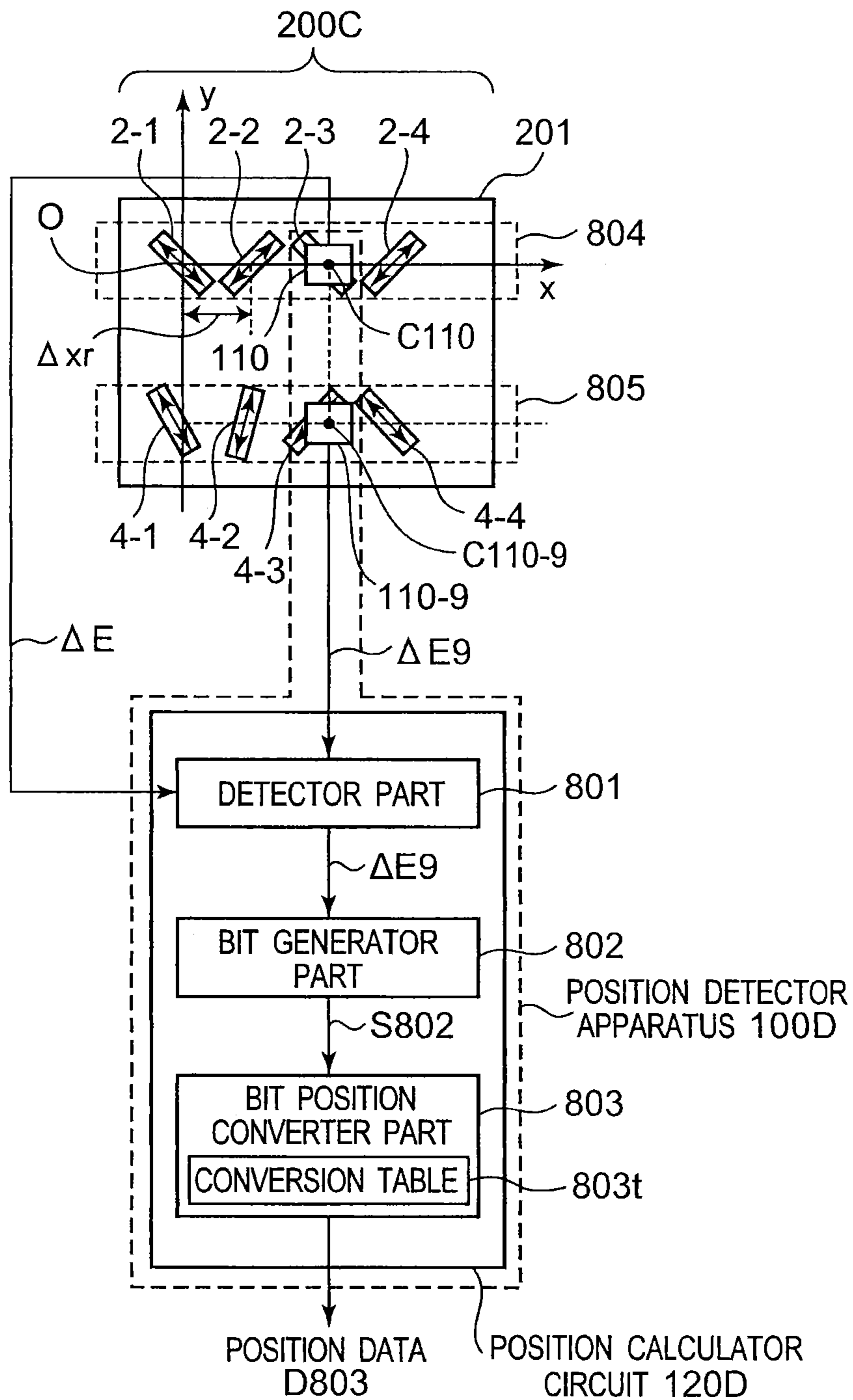
Fig. 14 POSITION MEASUREMENT APPARATUS 1D
