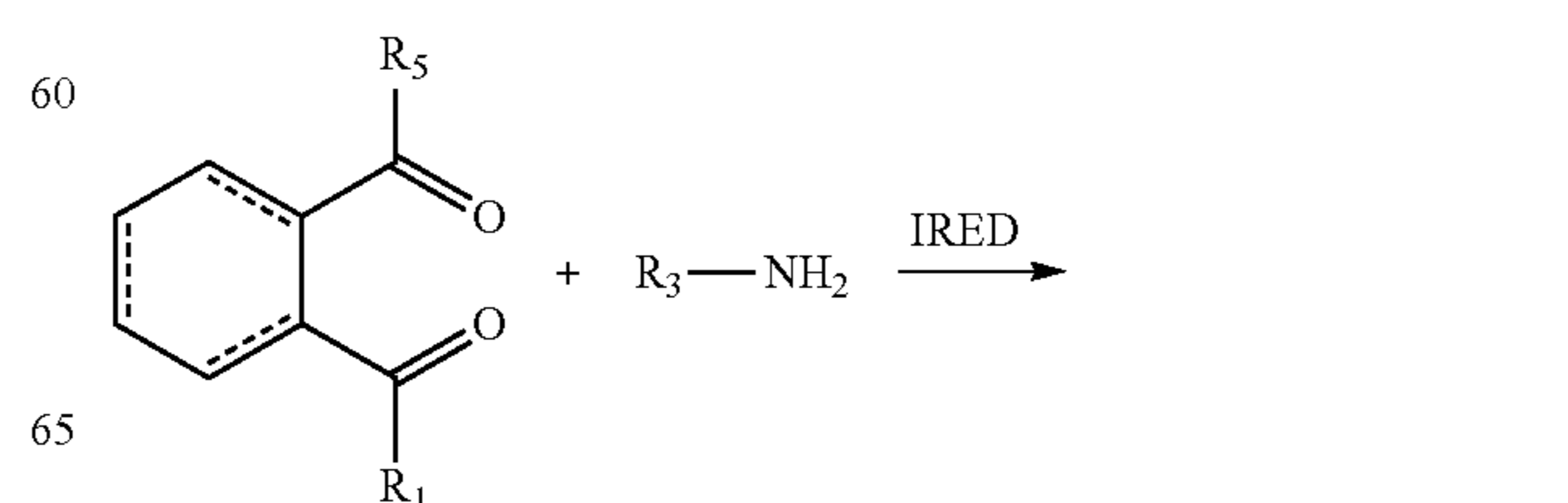
Scheme 9
