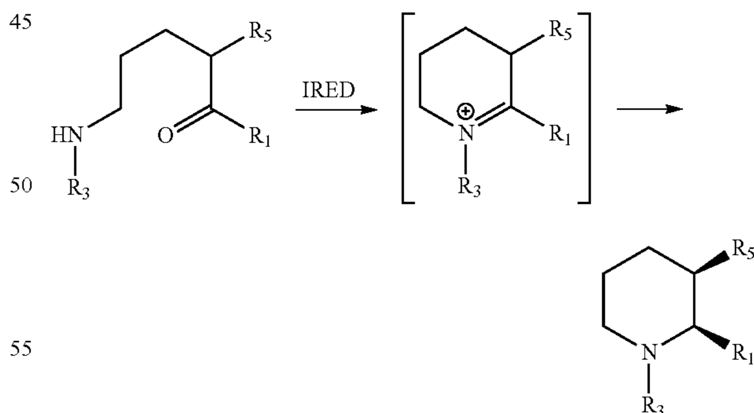
Scheme 3
