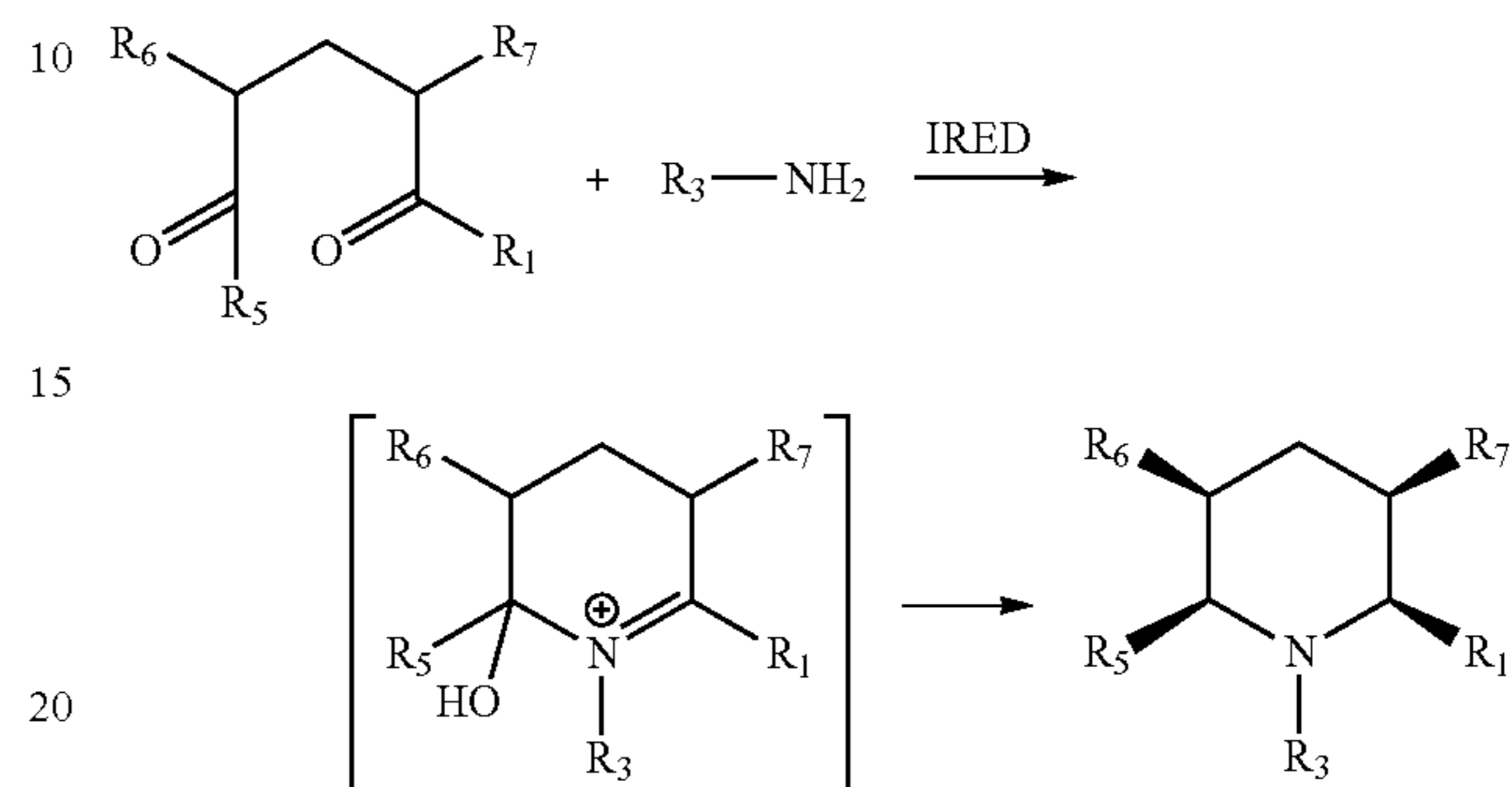
Scheme 7
