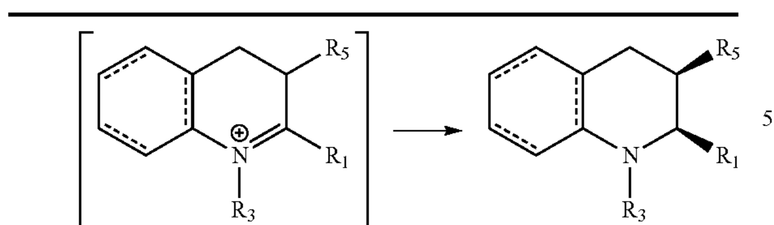
Scheme 4
