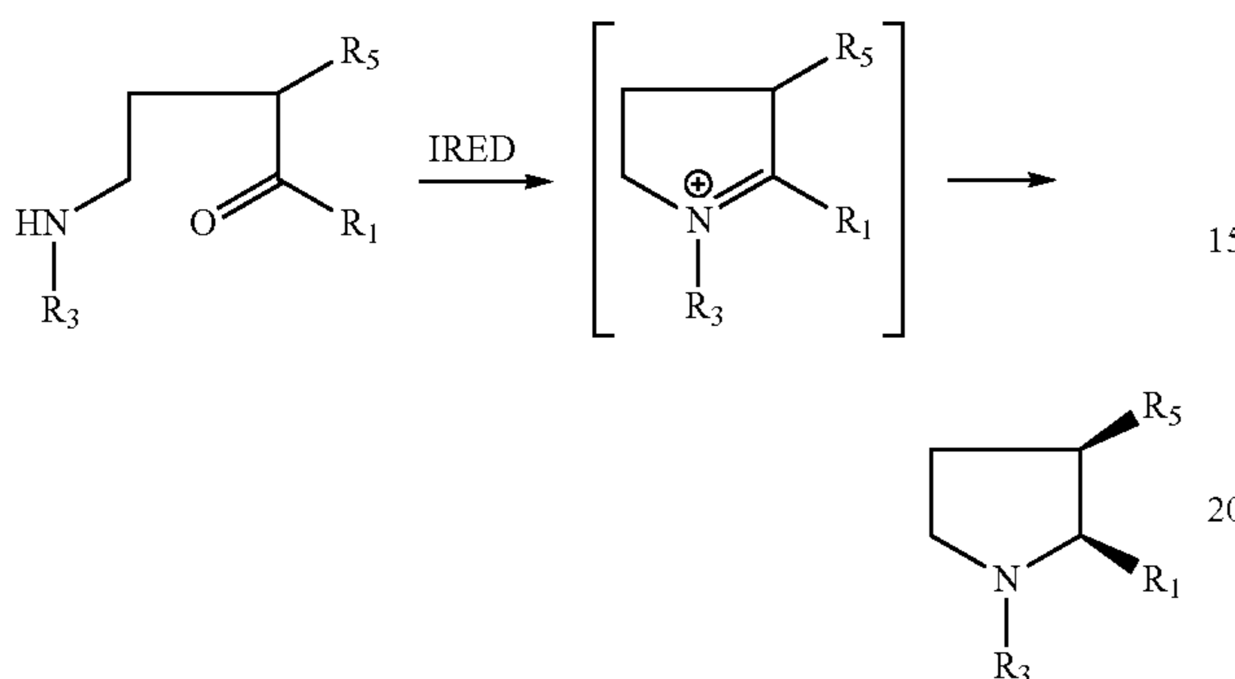
Scheme 5
