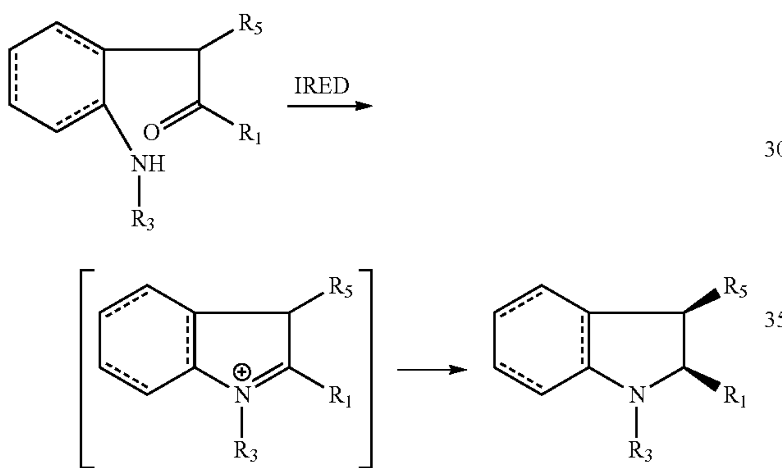
Scheme 5
