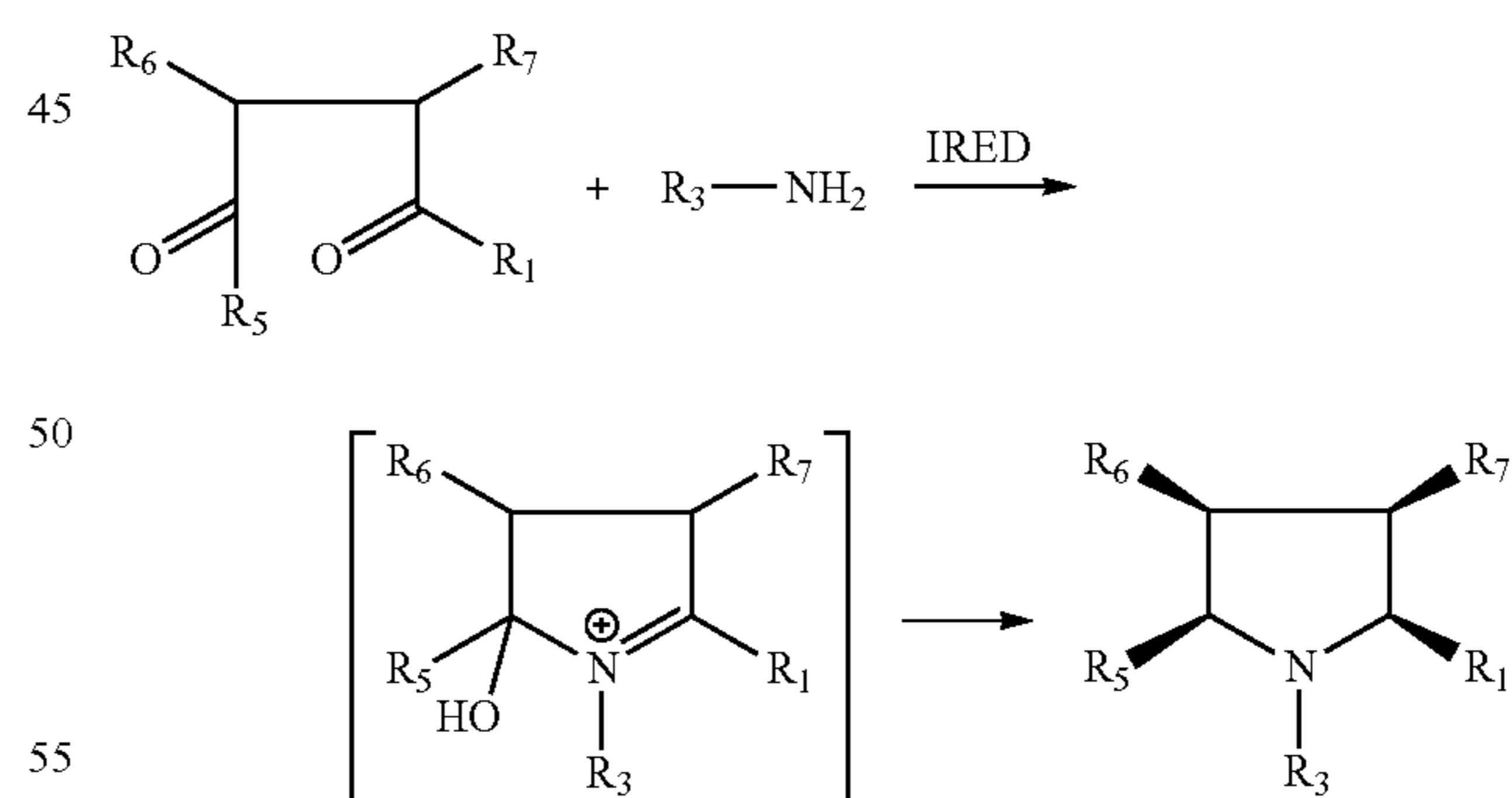
Scheme 9
