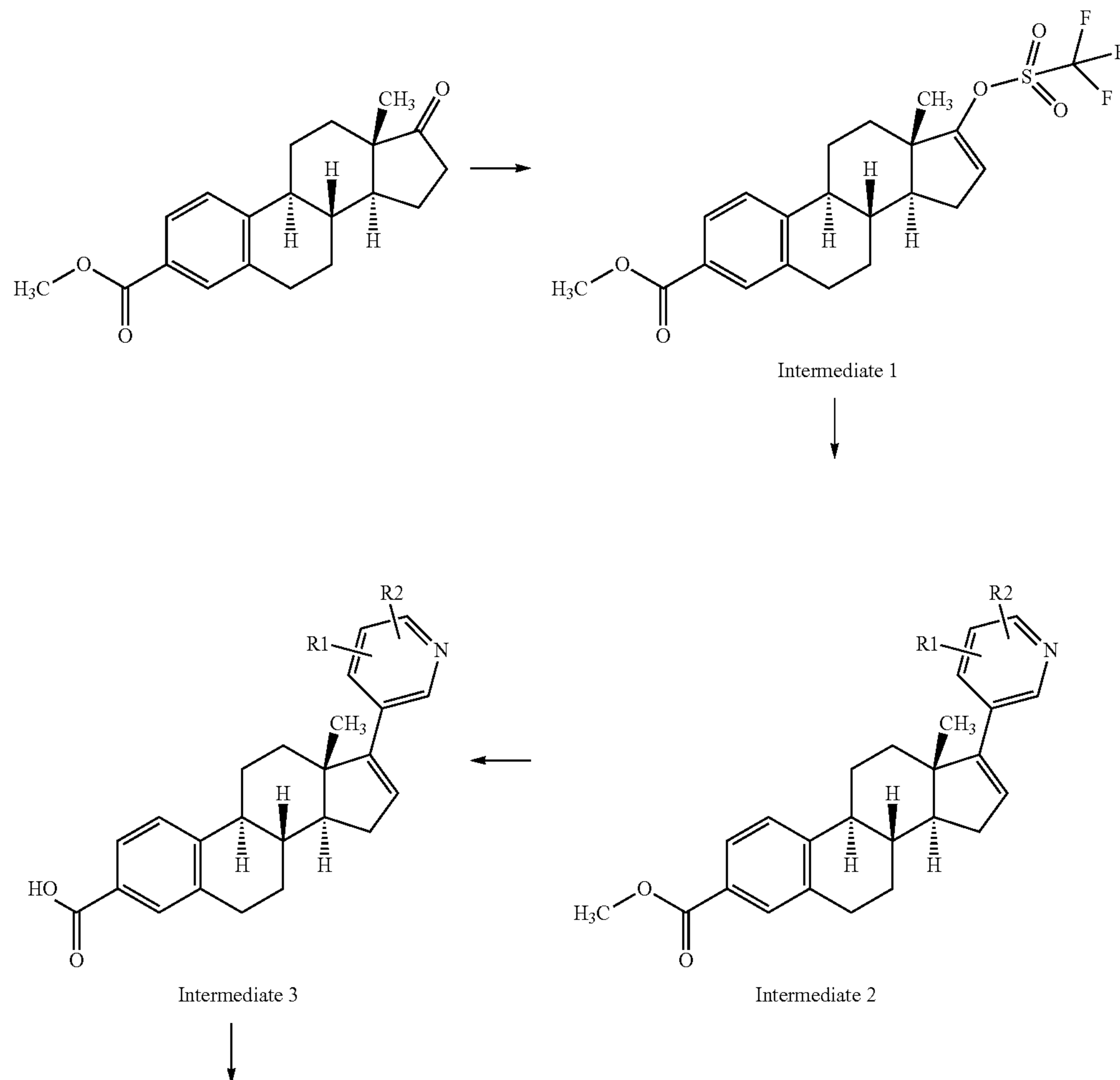
Synthesis scheme 1
