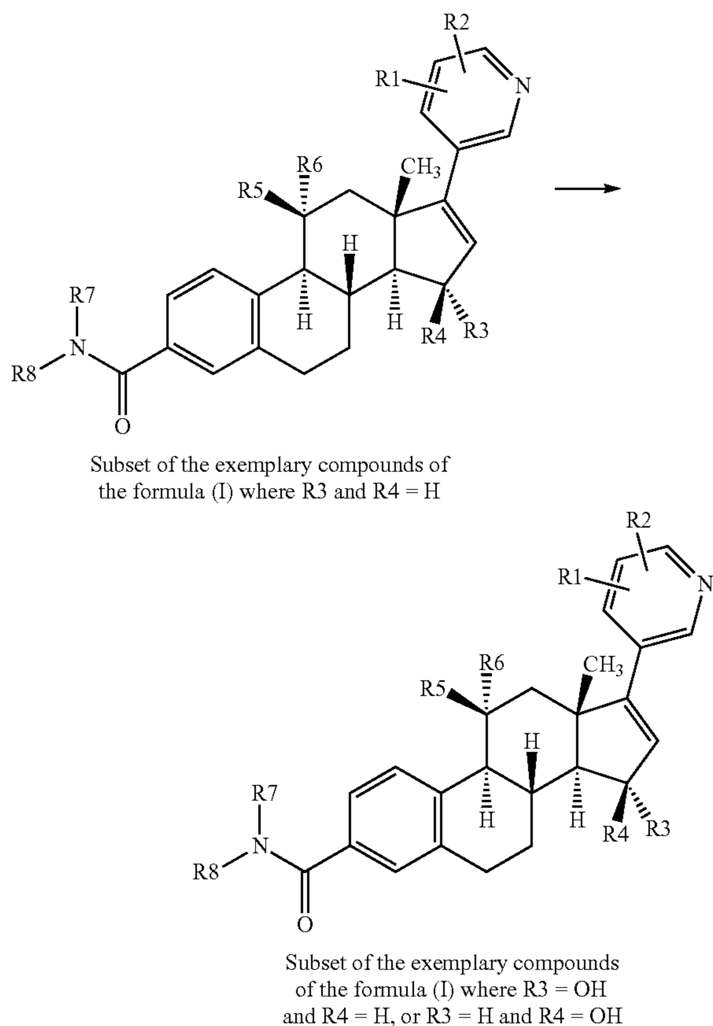
Synthesis scheme 3
