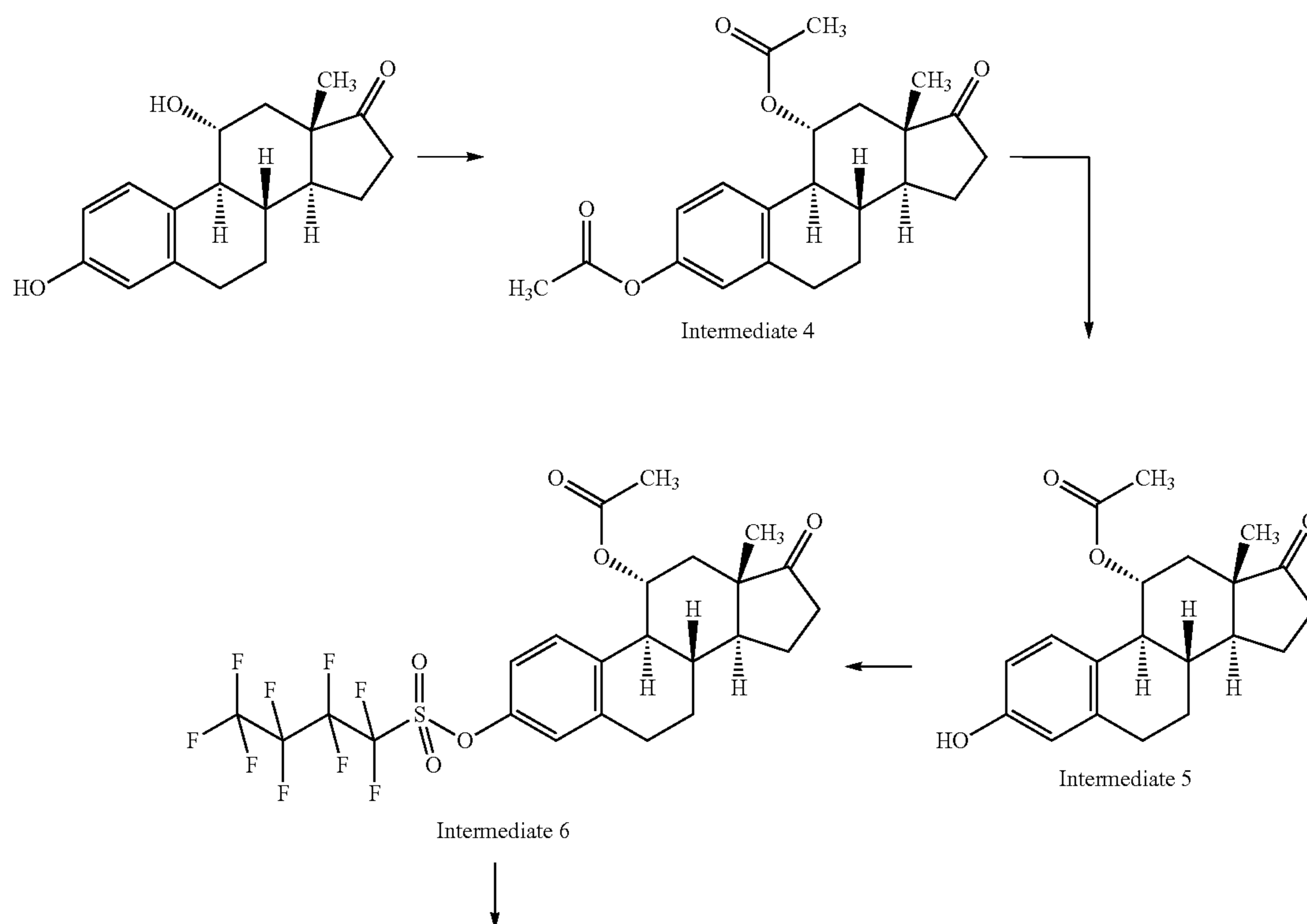
Synthesis scheme 2
