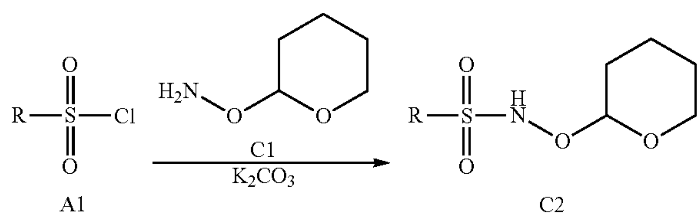
Scheme C. General Synthesis of Intermediate N-(tetrahydro-pyran-2-yloxy)sulfonamides.
