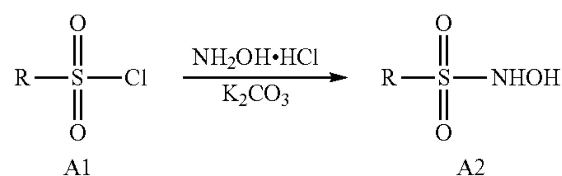
Scheme A. General Synthesis of N-Hydroxysulfonamides.
