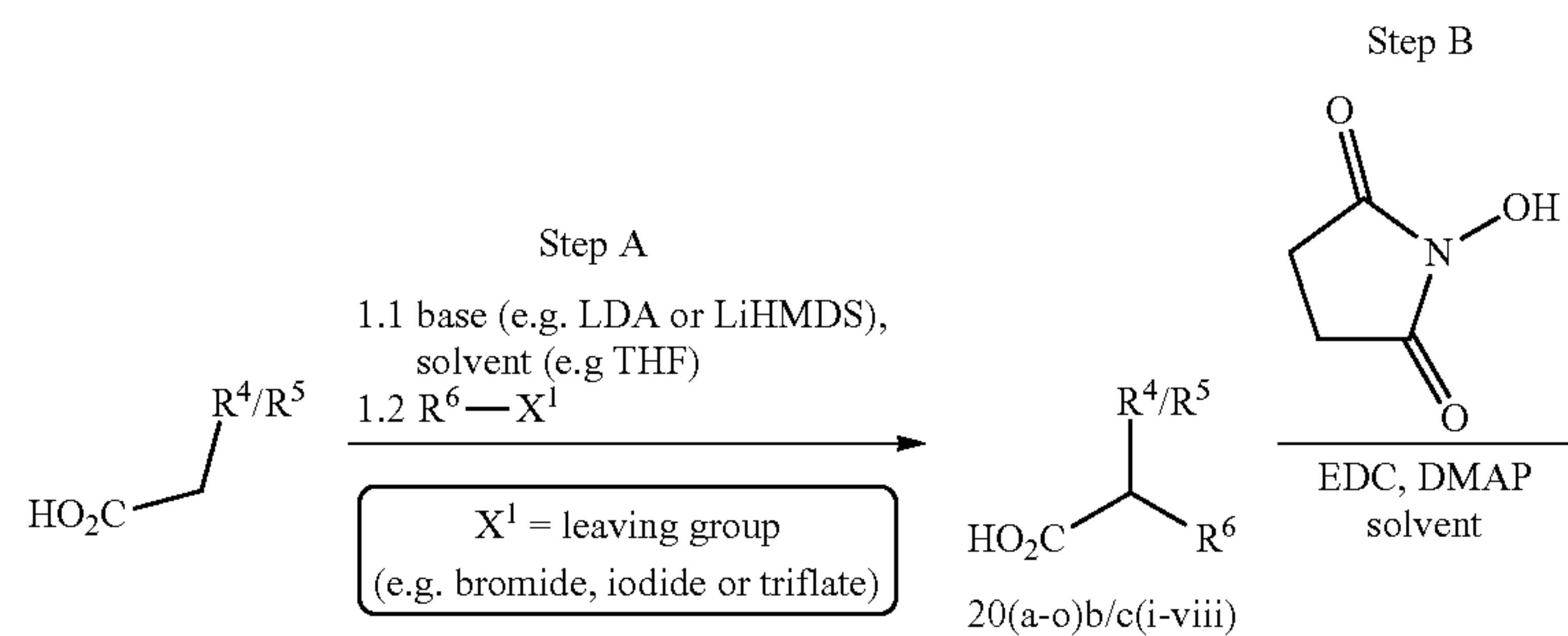
Scheme 7f
