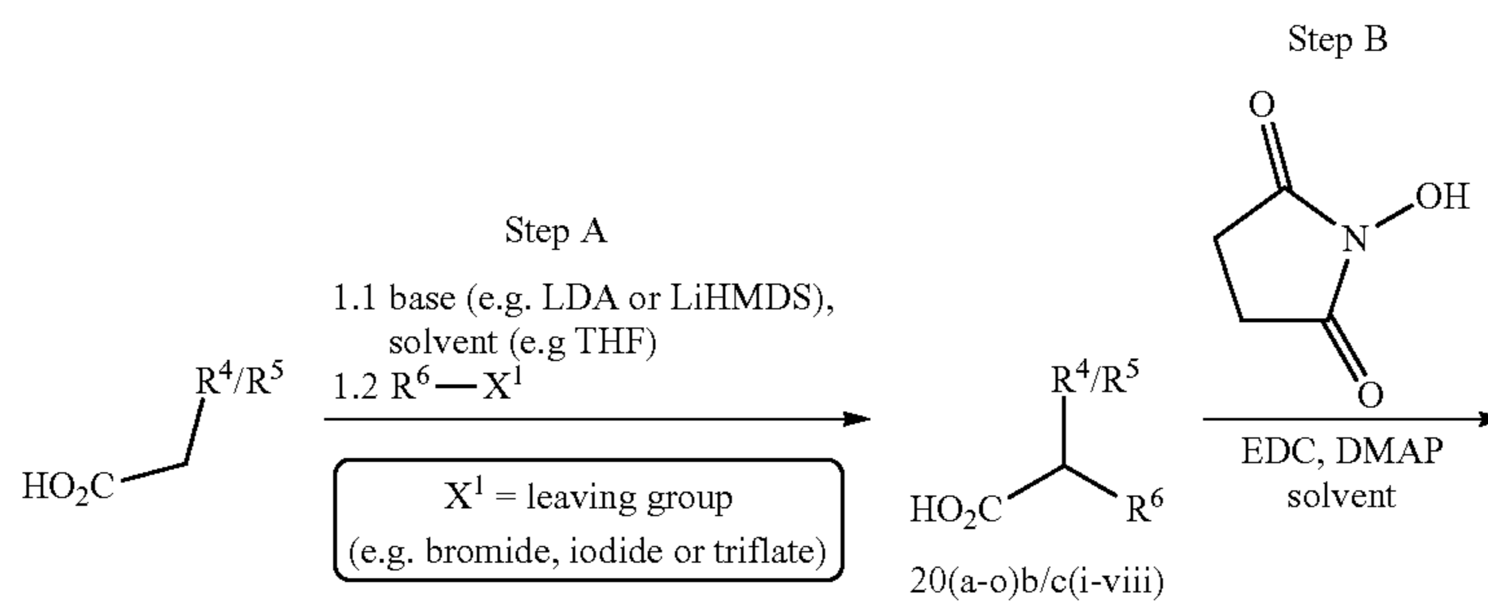
Scheme 7f
