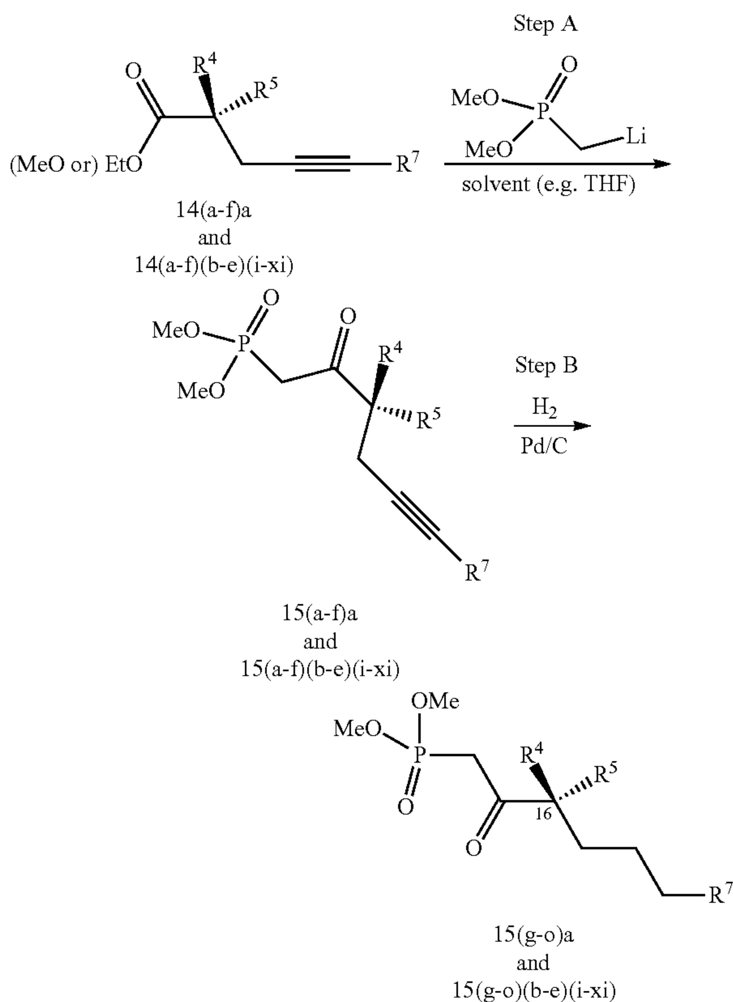
Scheme 8
