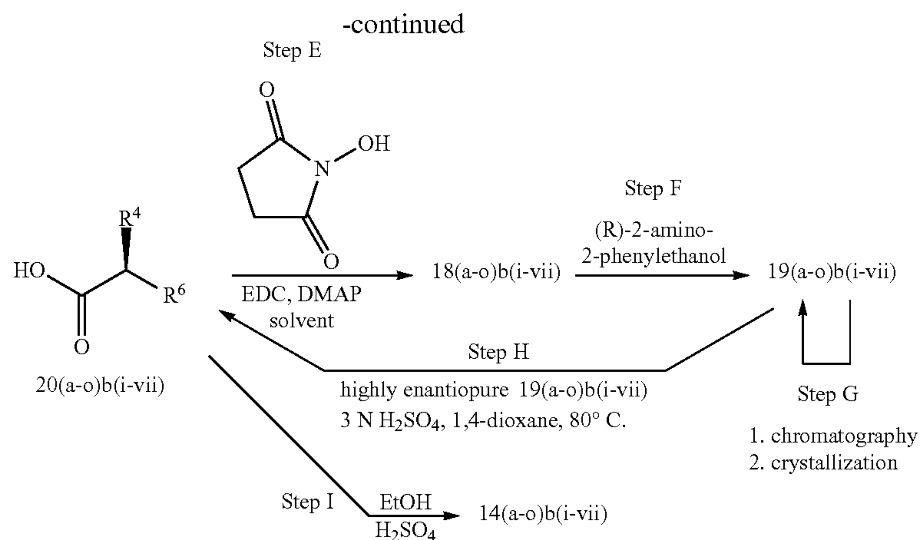
20 Scheme 7a, Step A: Preparation of diethyl 2-(but-2-yn-1-yl)-2-methylmalonate (16a(i))
