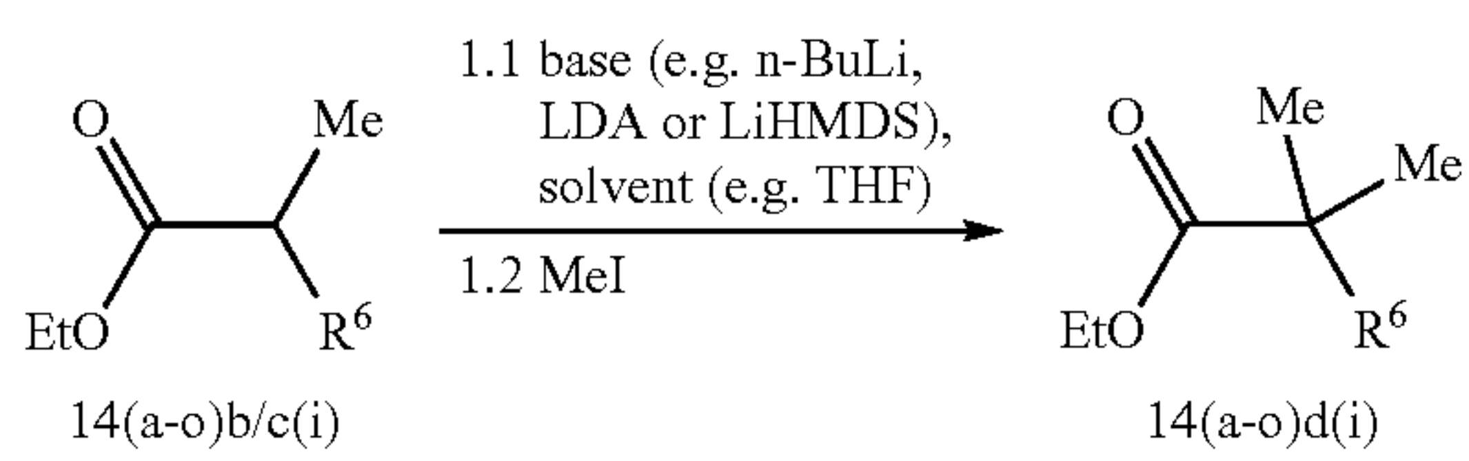
Scheme 7b
