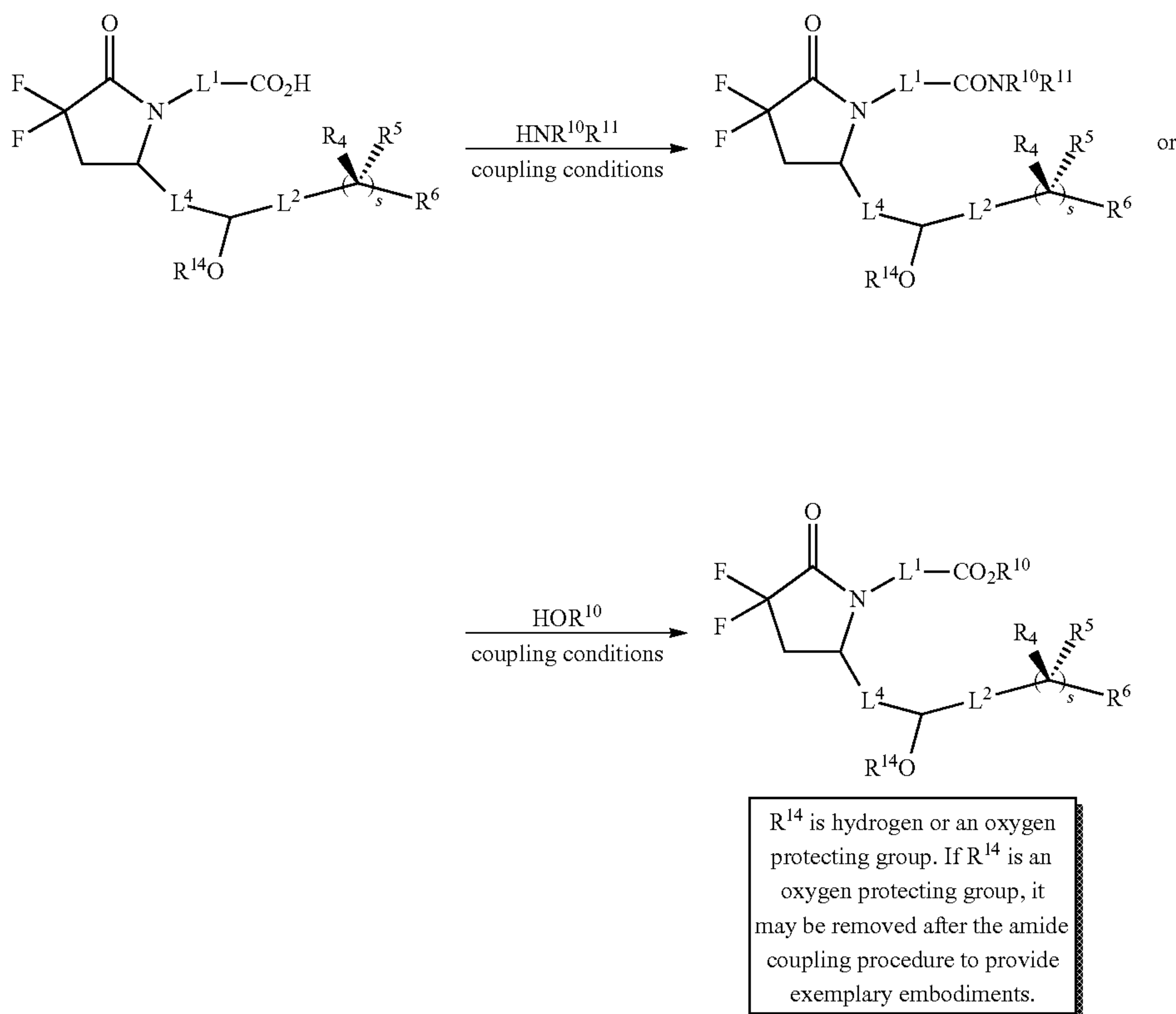
Scheme 11
