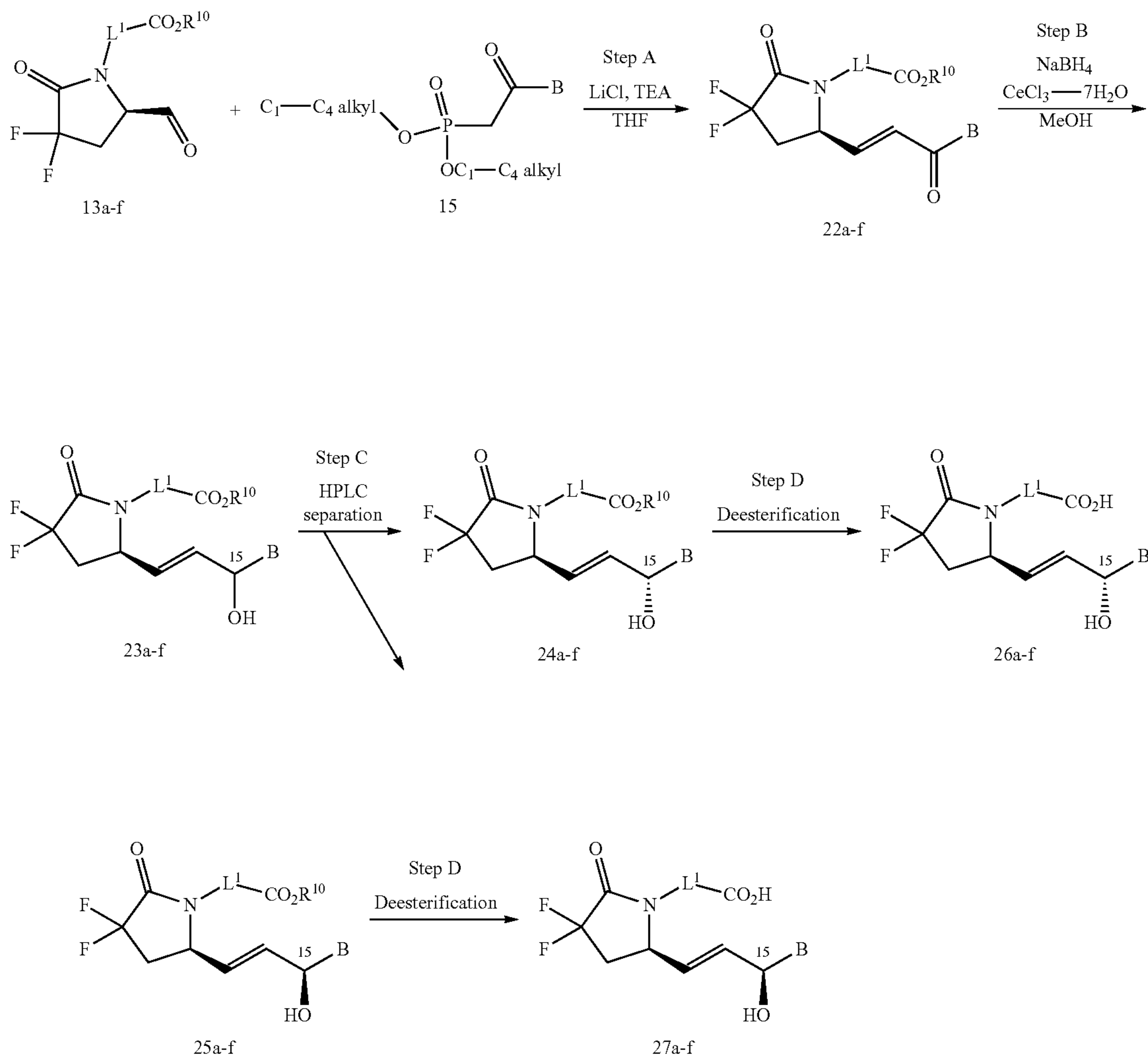
Scheme 9
