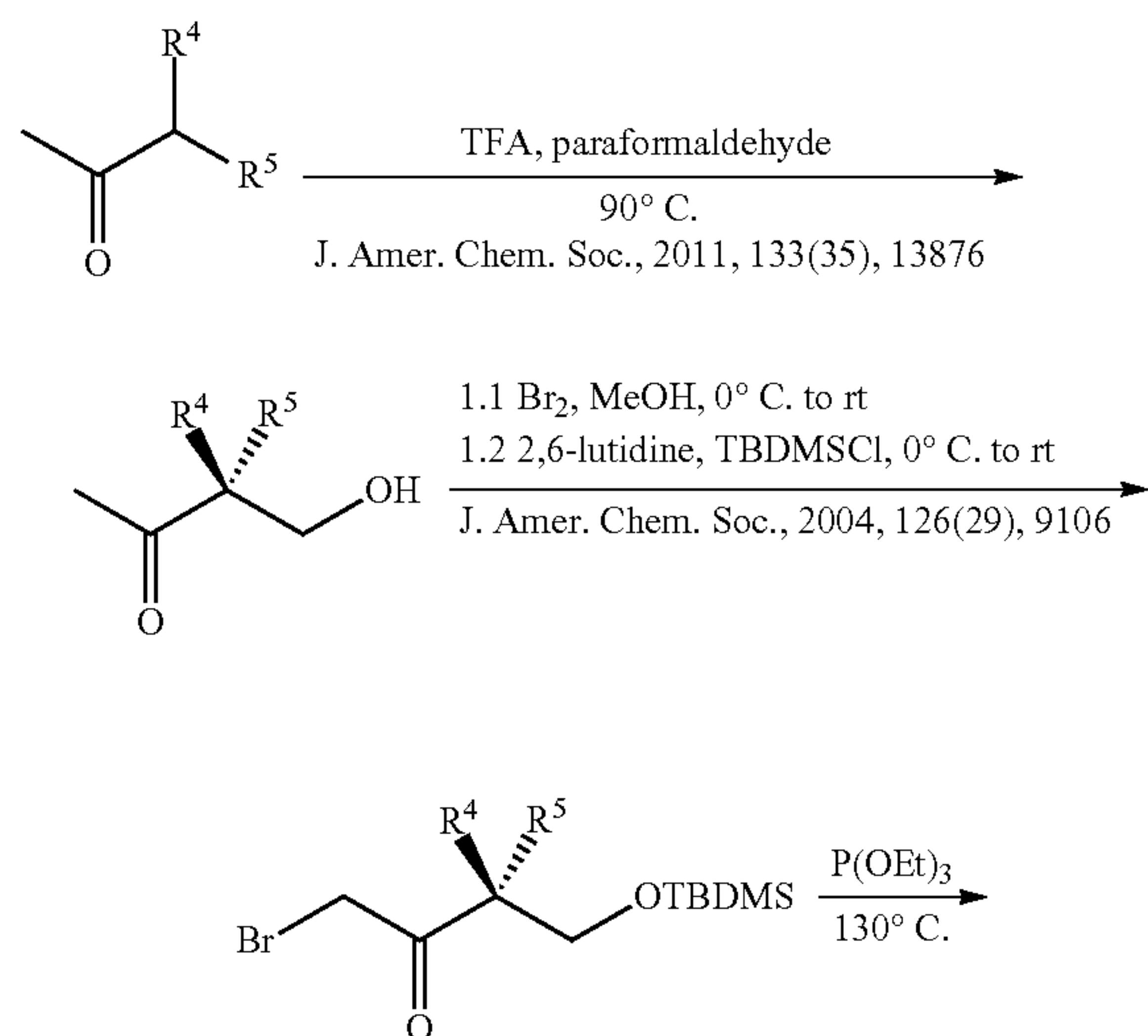
Scheme 2C
