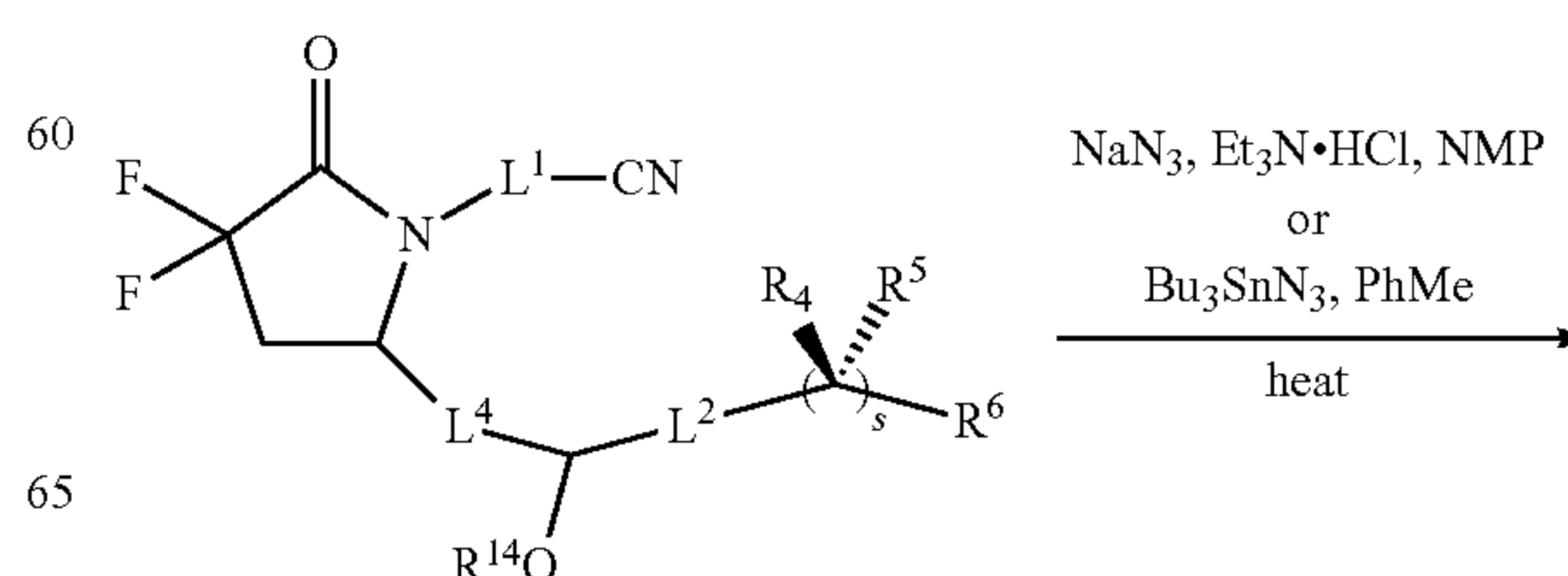
Scheme 12
