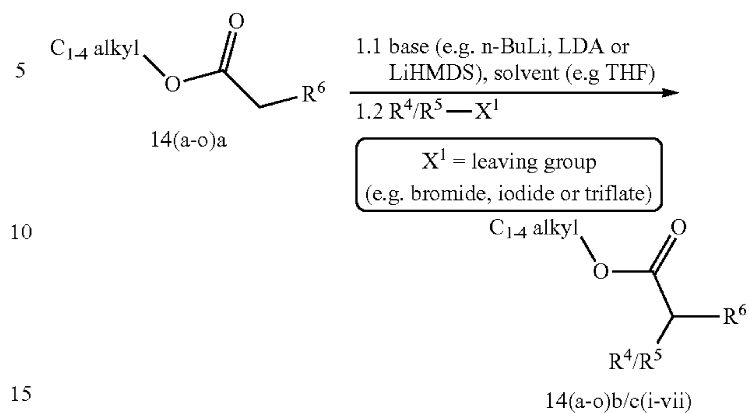
Scheme 7c
