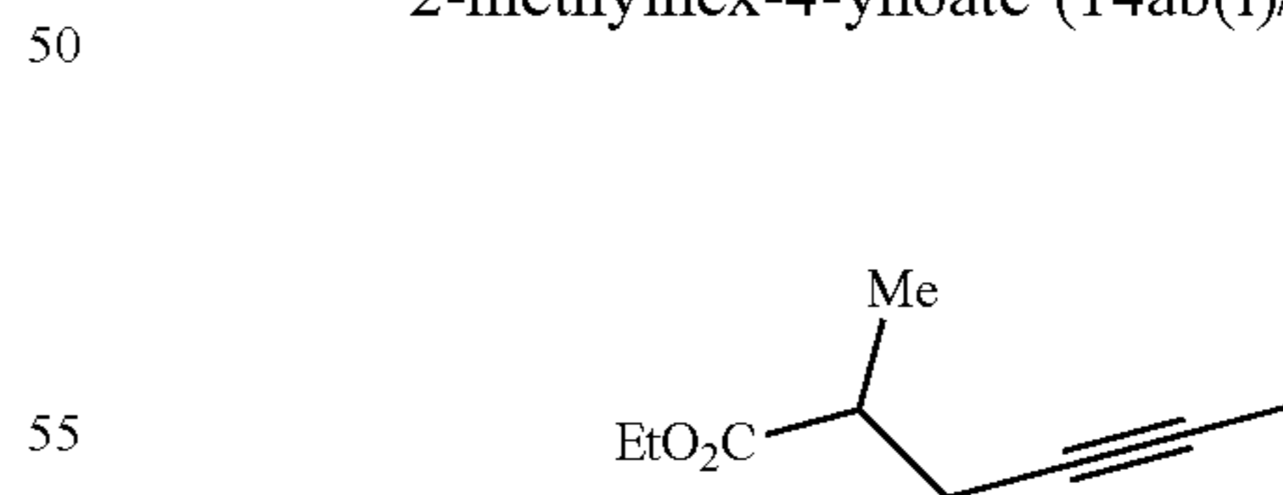
45 Scheme 7a, Step B: Preparation of (±)-ethyl 2-methylhex-4-ynoate (14ab(i)/14ac(i))
