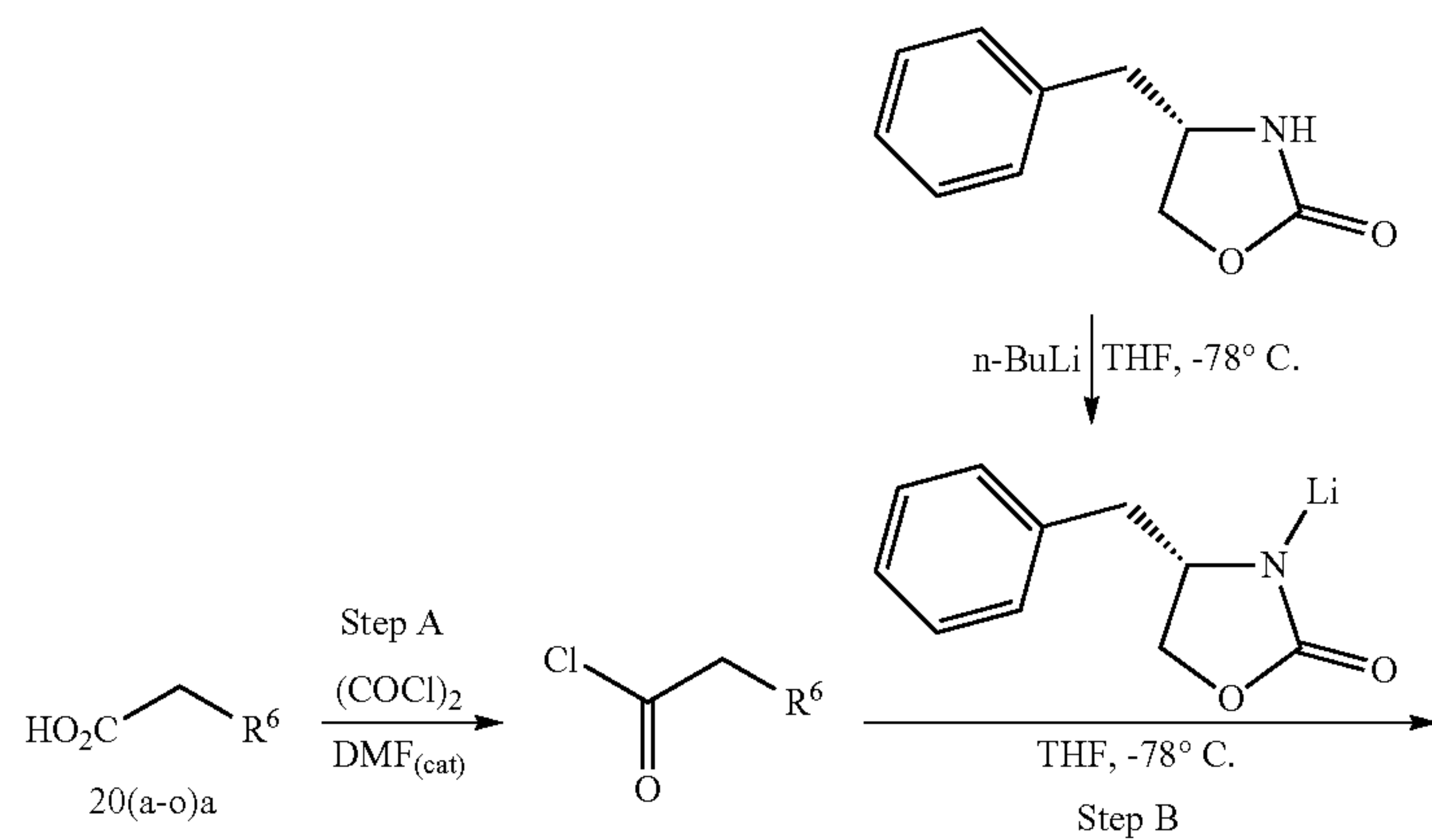
Scheme 7g
