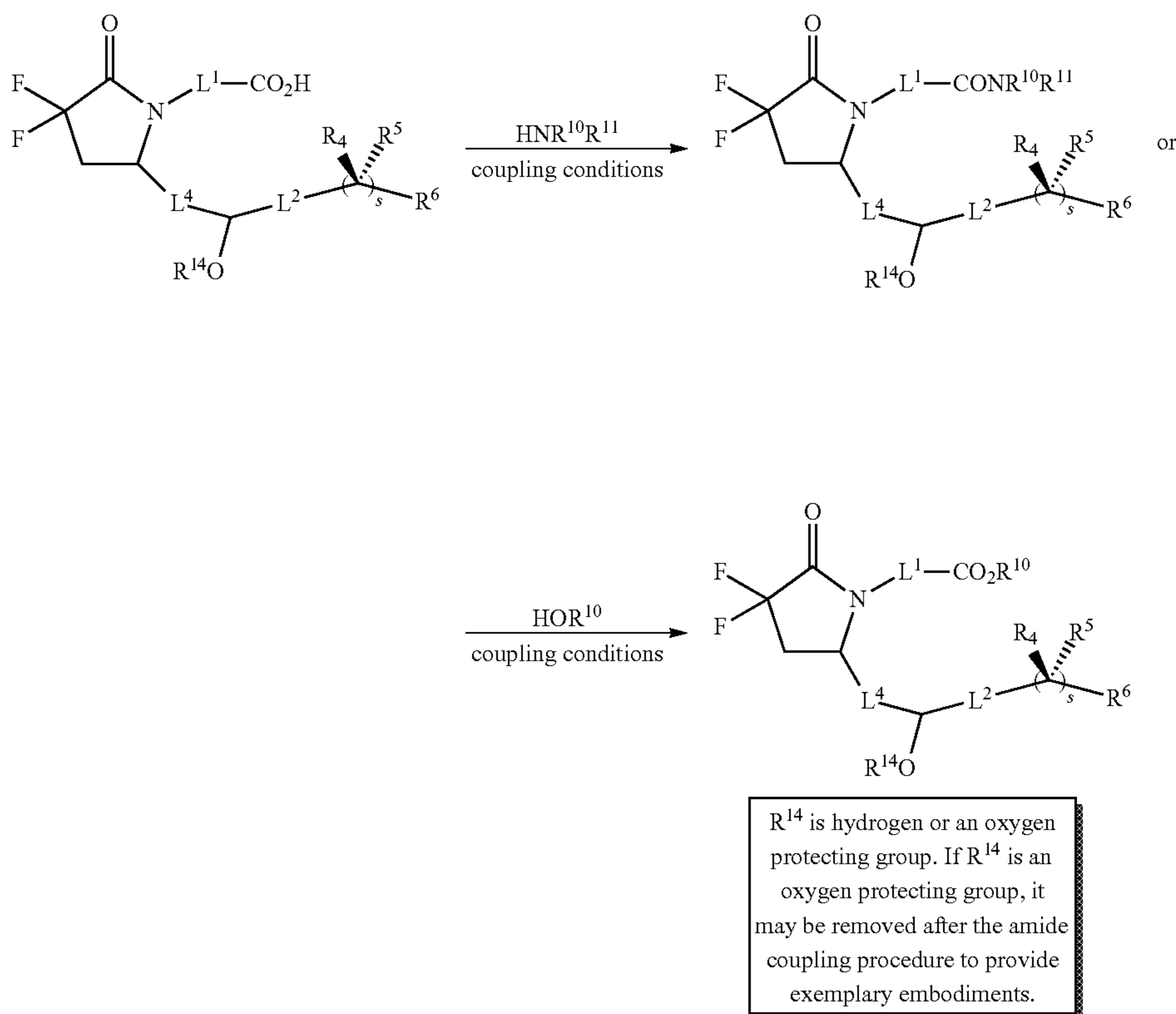
Scheme 11
