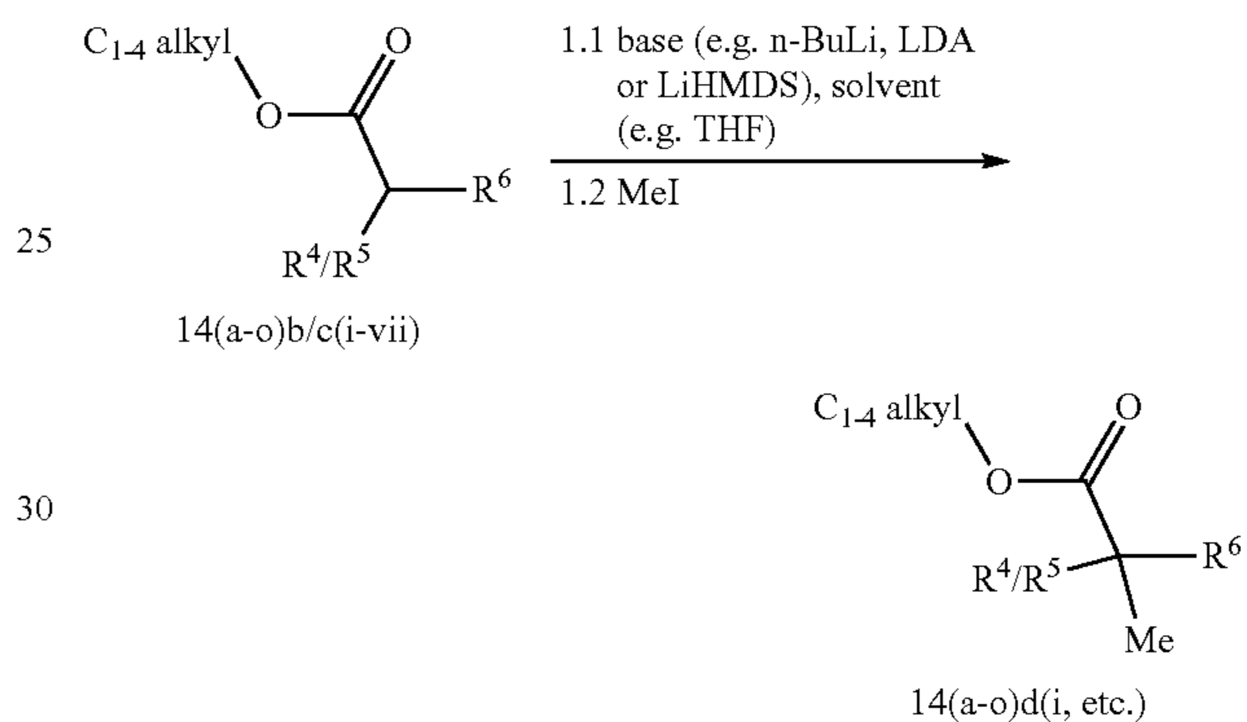
Scheme 7d
