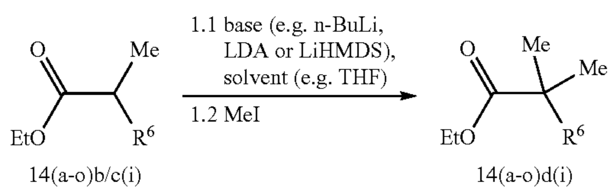
Scheme 7b
