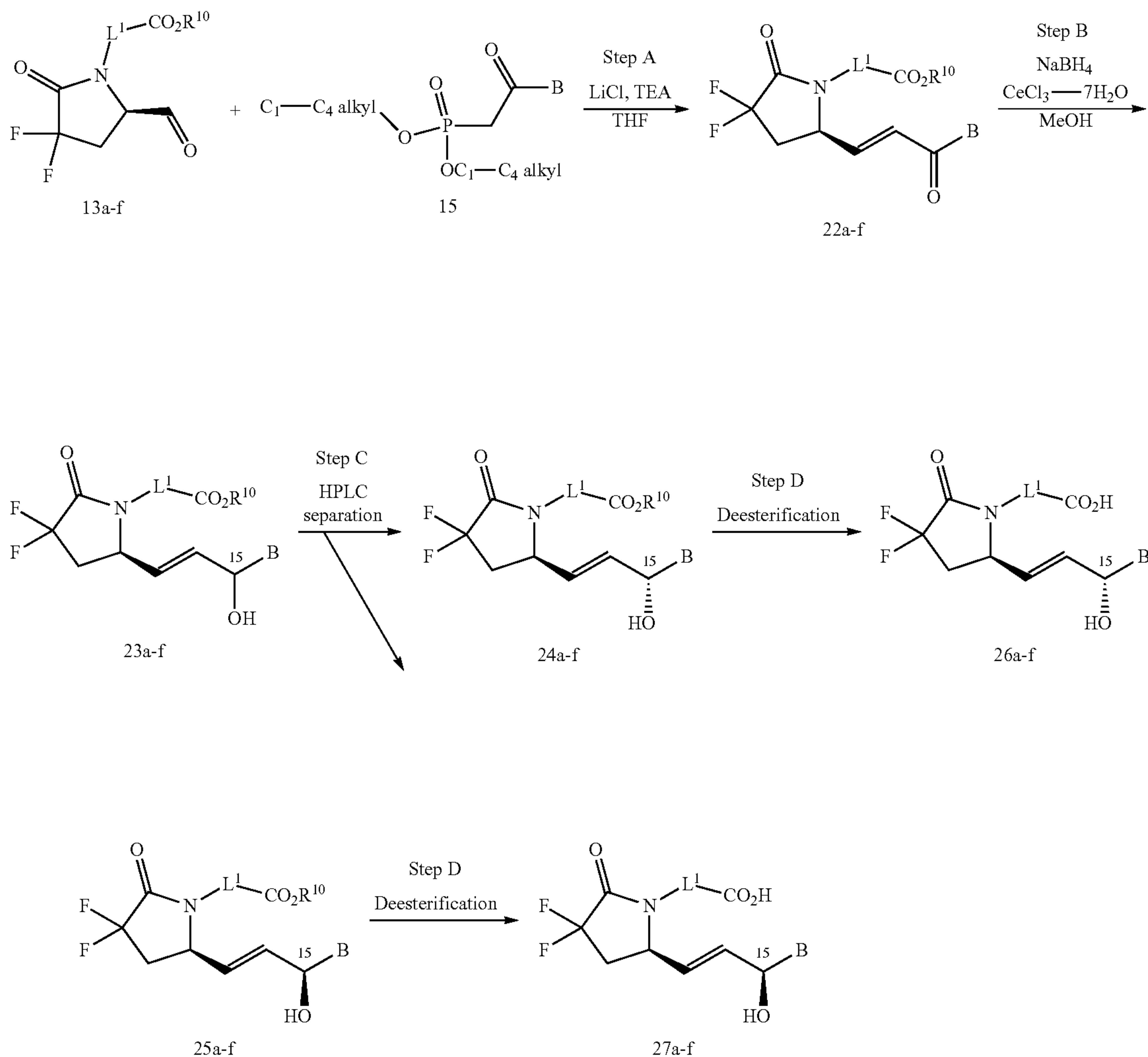
Scheme 9
