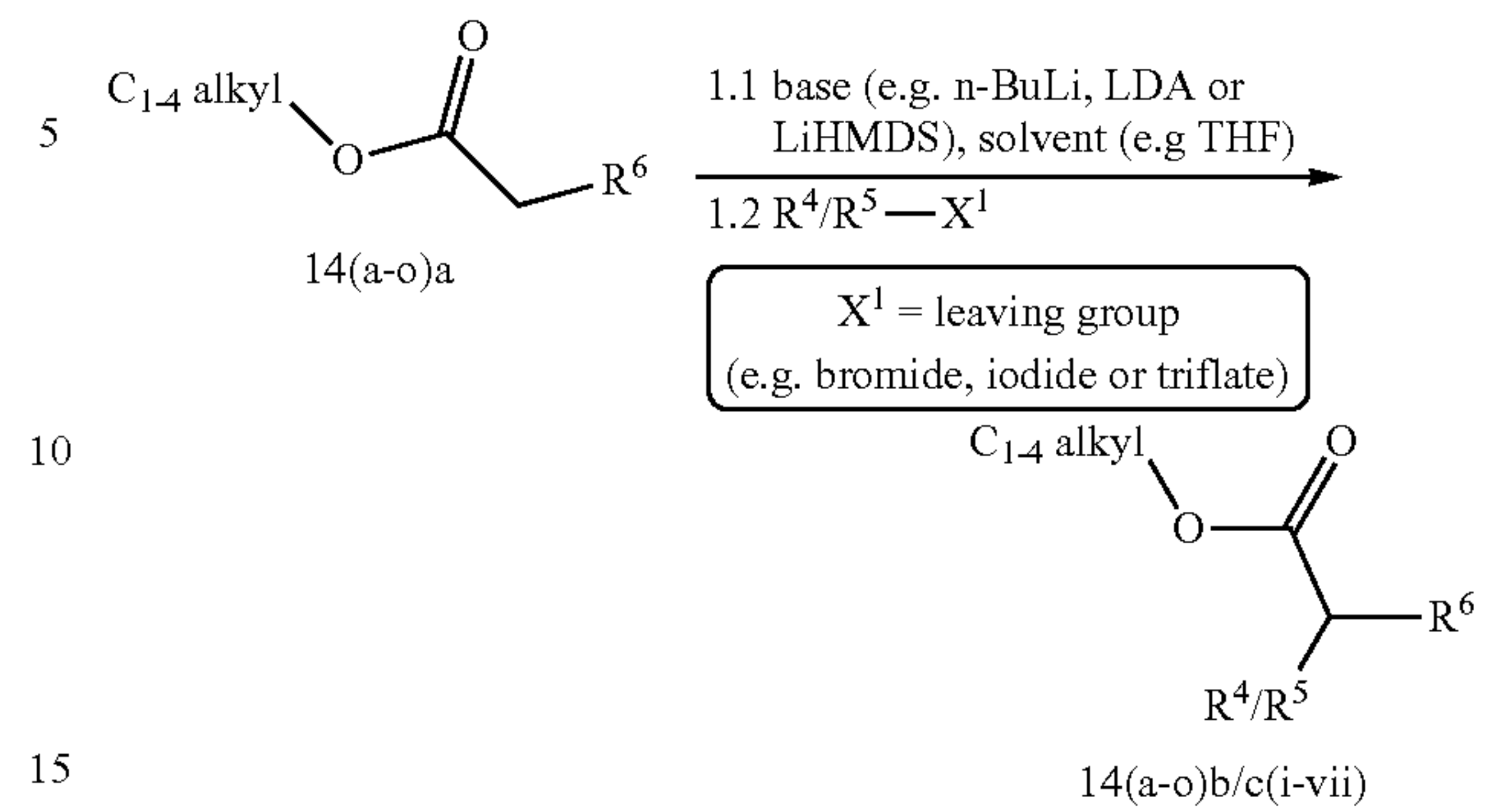
Scheme 7c
