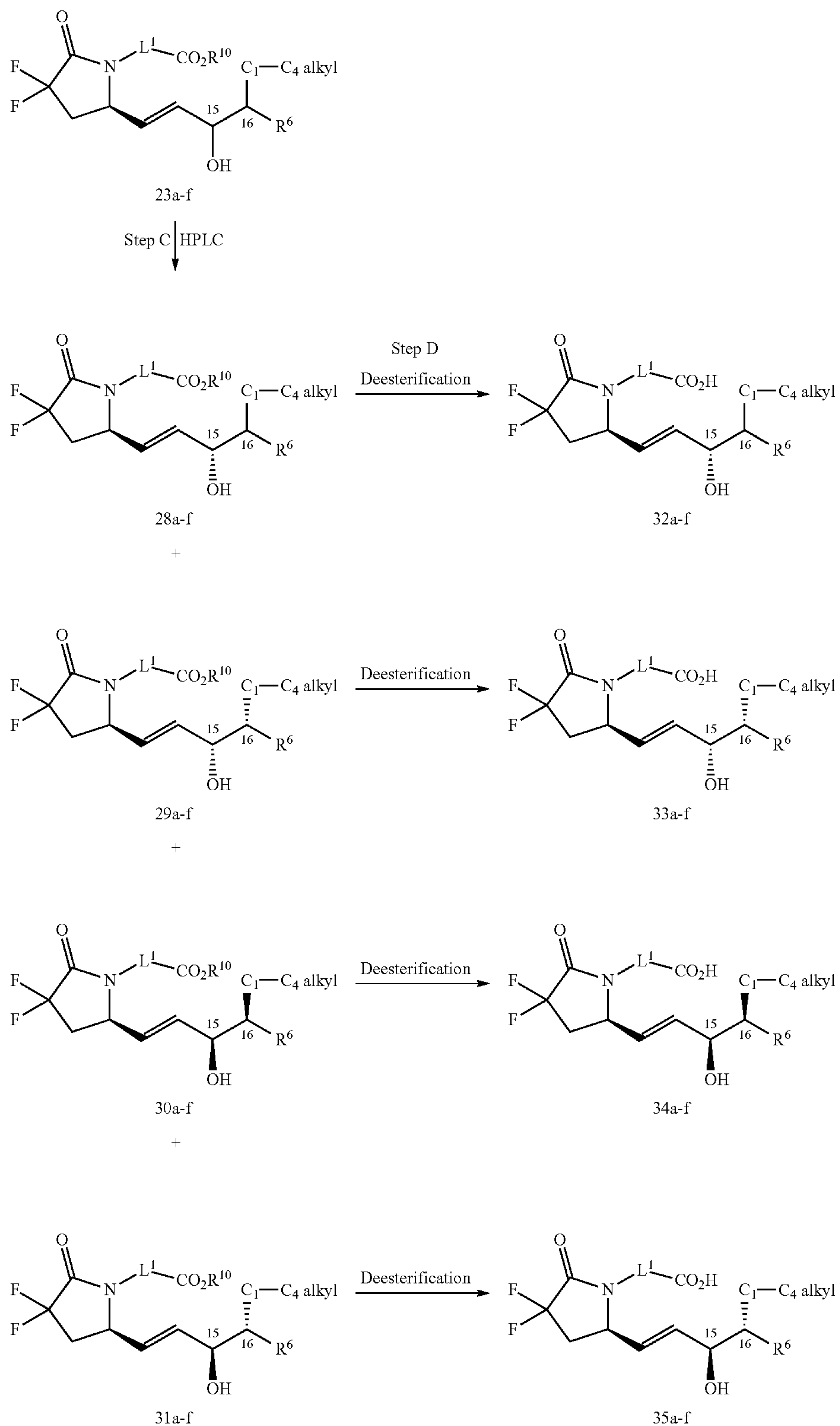
Scheme 10
