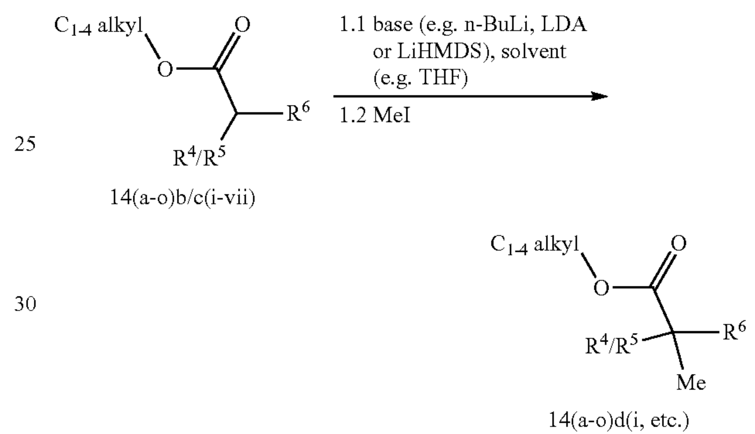
Scheme 7d
