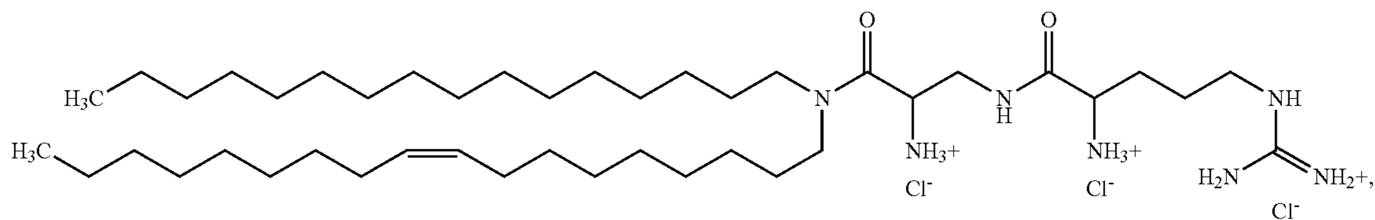
\beta -arginyl-2,3-diamino propionic acid-N-palmityl-N-oleyl-amide trihydrochloride
