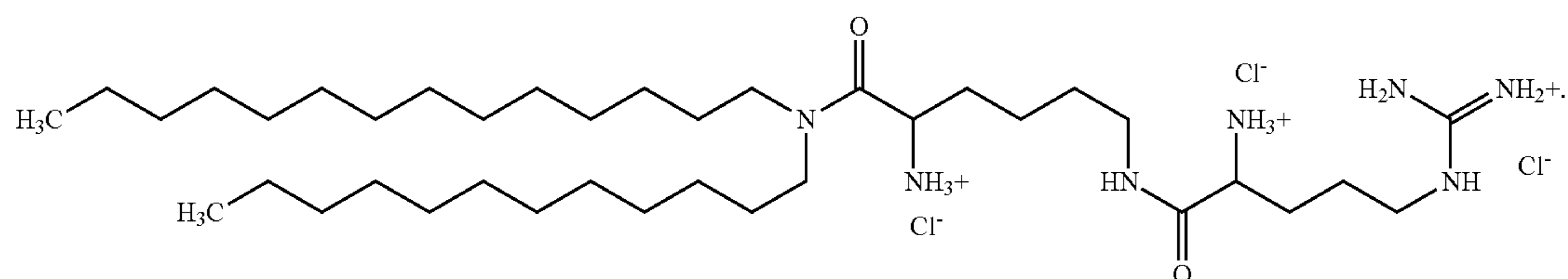
\epsilon -arginyl-lysine-N-lauryl-N-myristyl-amide trihydrochloride
