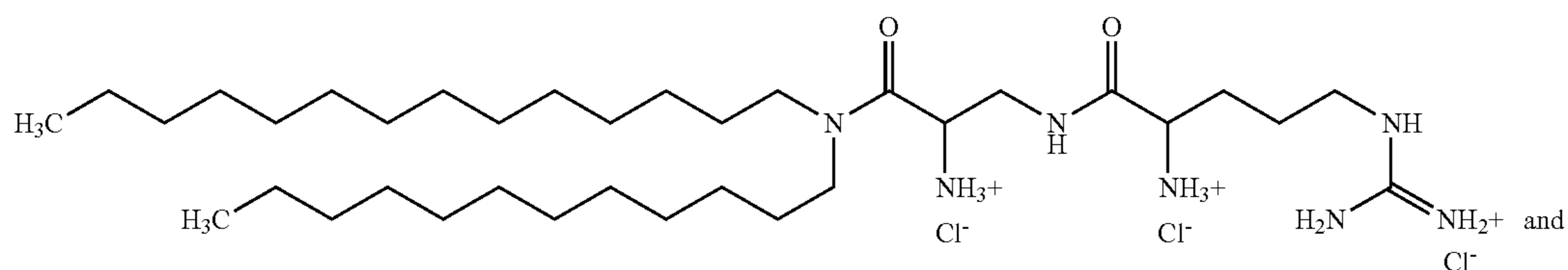
\beta -arginyl-2,3-diamino propionic acid-N-lauryl-N-myristyl-amide trihydrochloride
