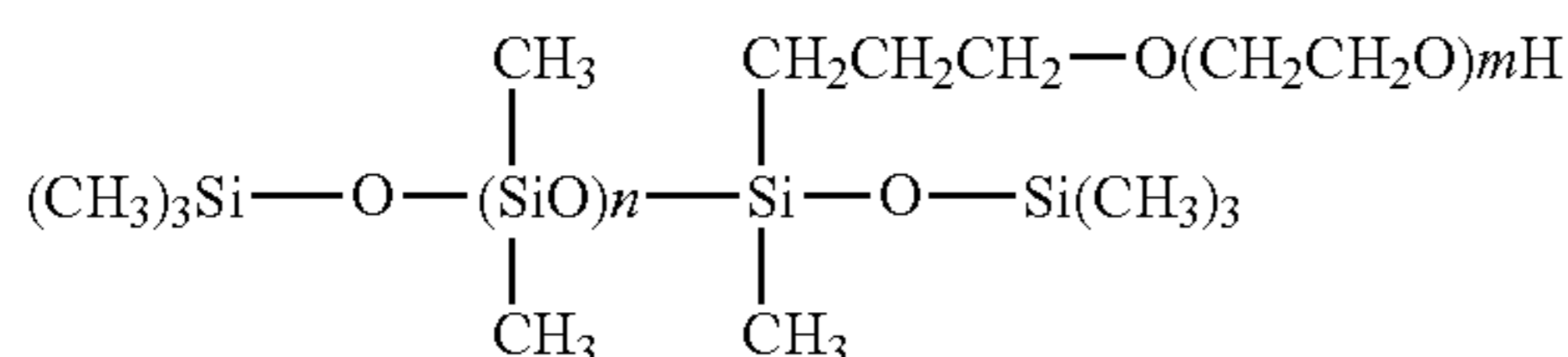
Formula (II)
