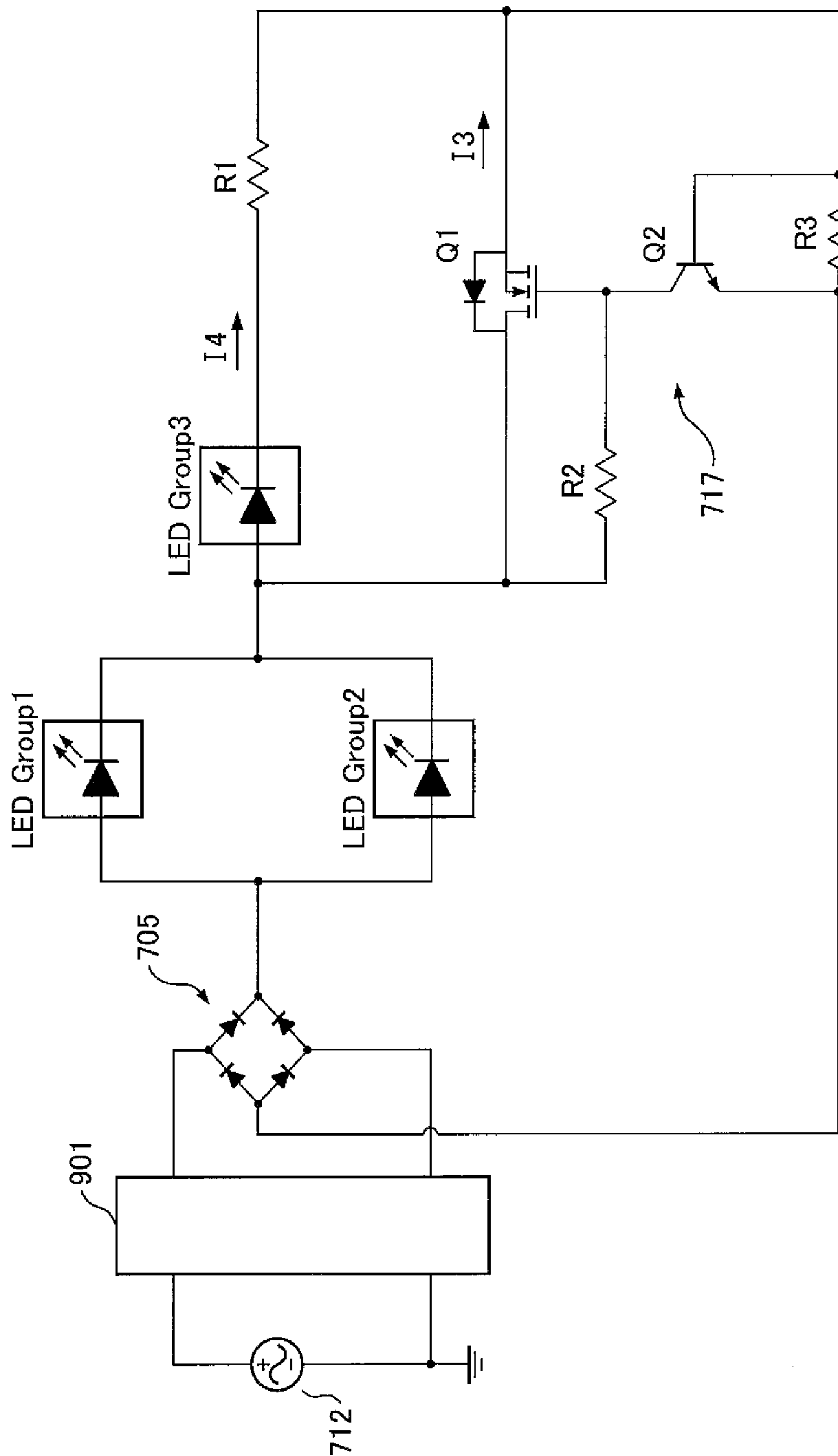
Fig. 9 PRIOR ART
