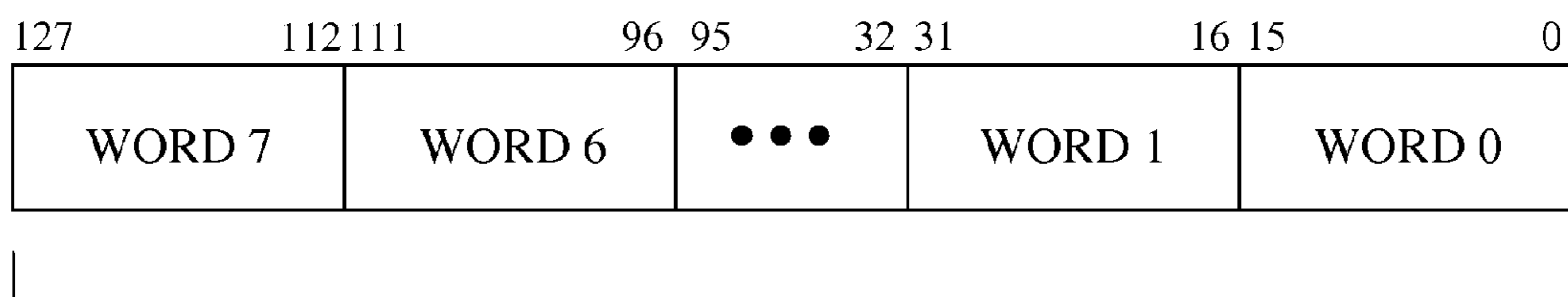
320 Packed Word
