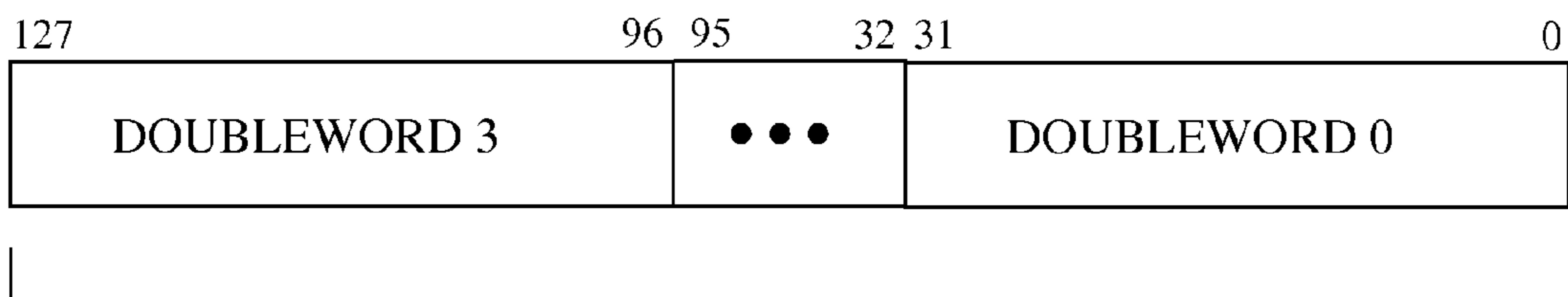
330 Packed Doubleword
