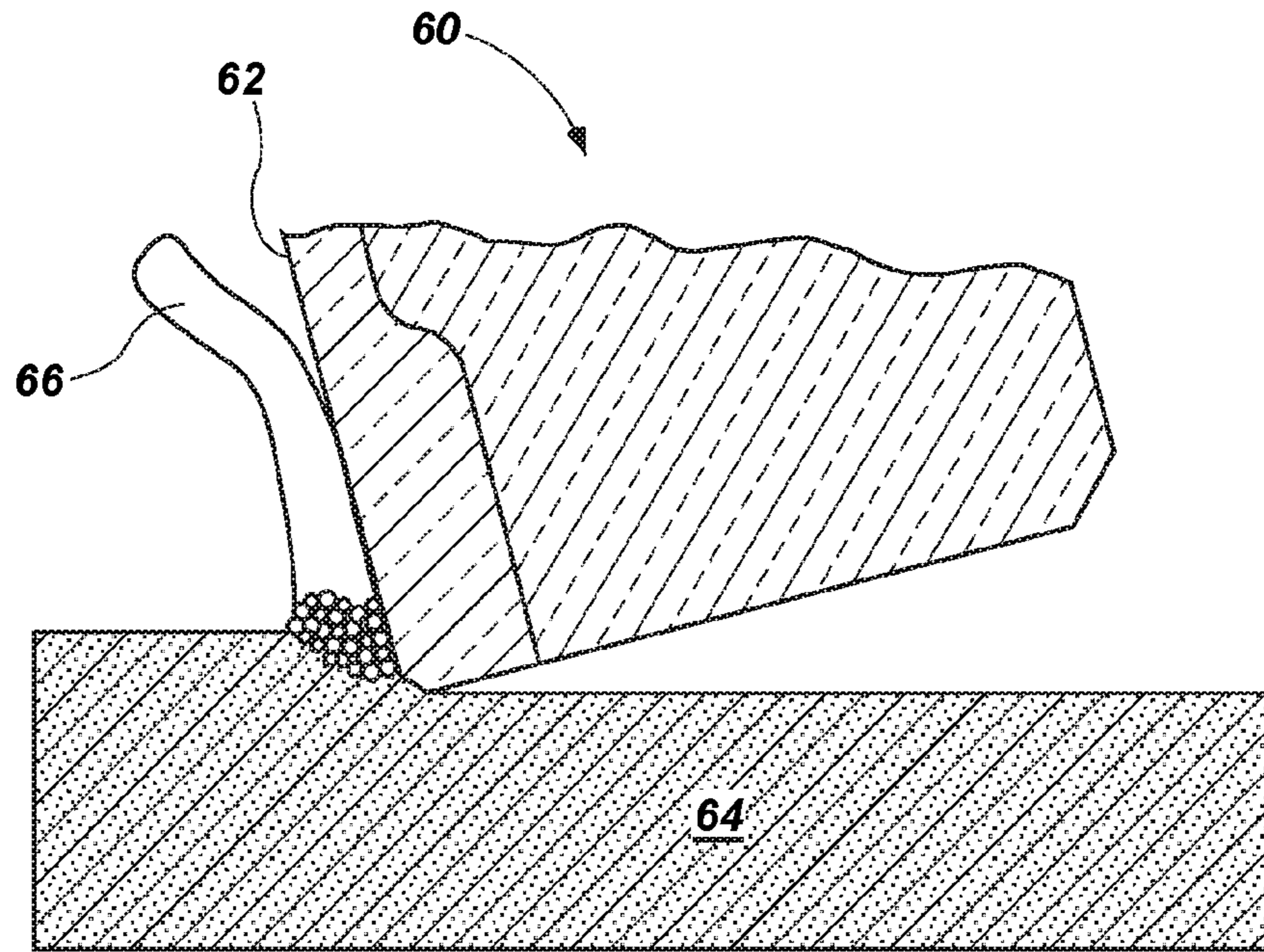
FIG. 29 (PRIOR ART)
