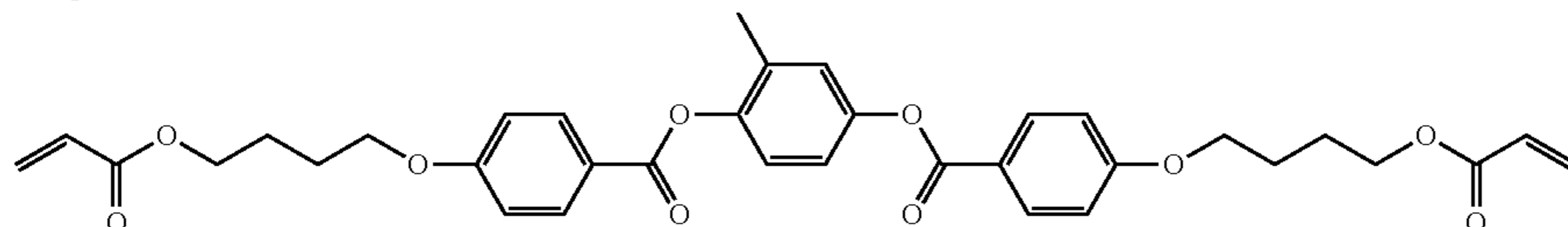
(Compound B) Compound 2
