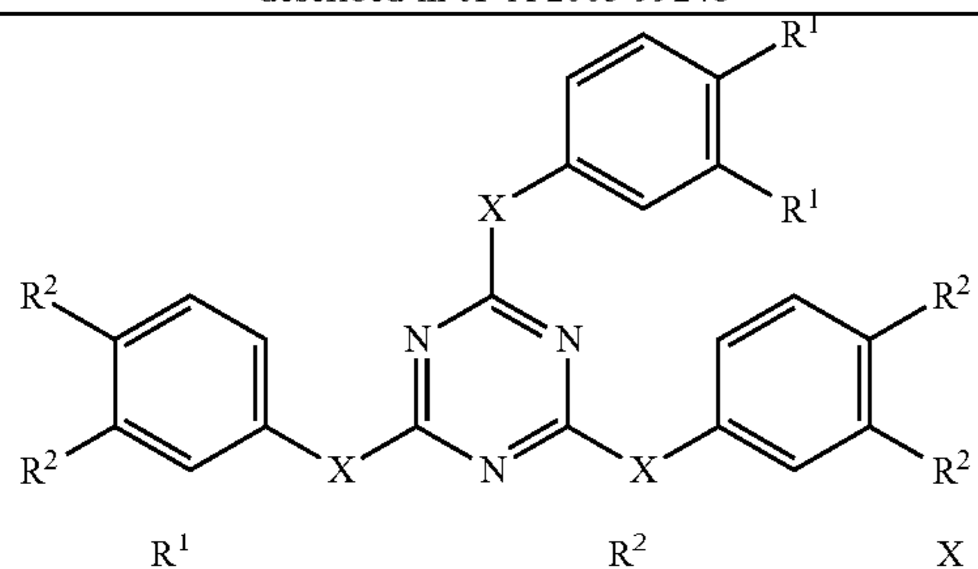
Chiral agent (A)
