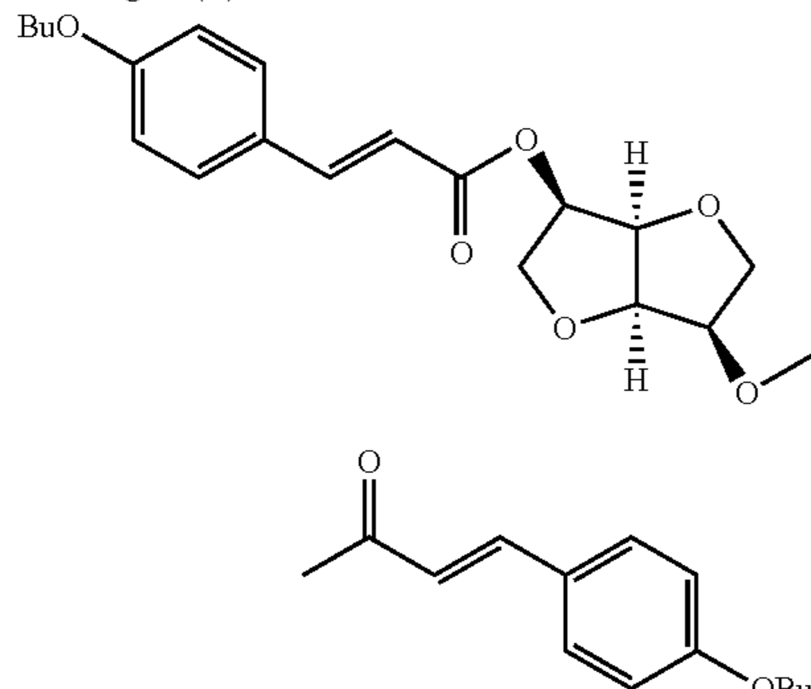
Chiral agent (A)
