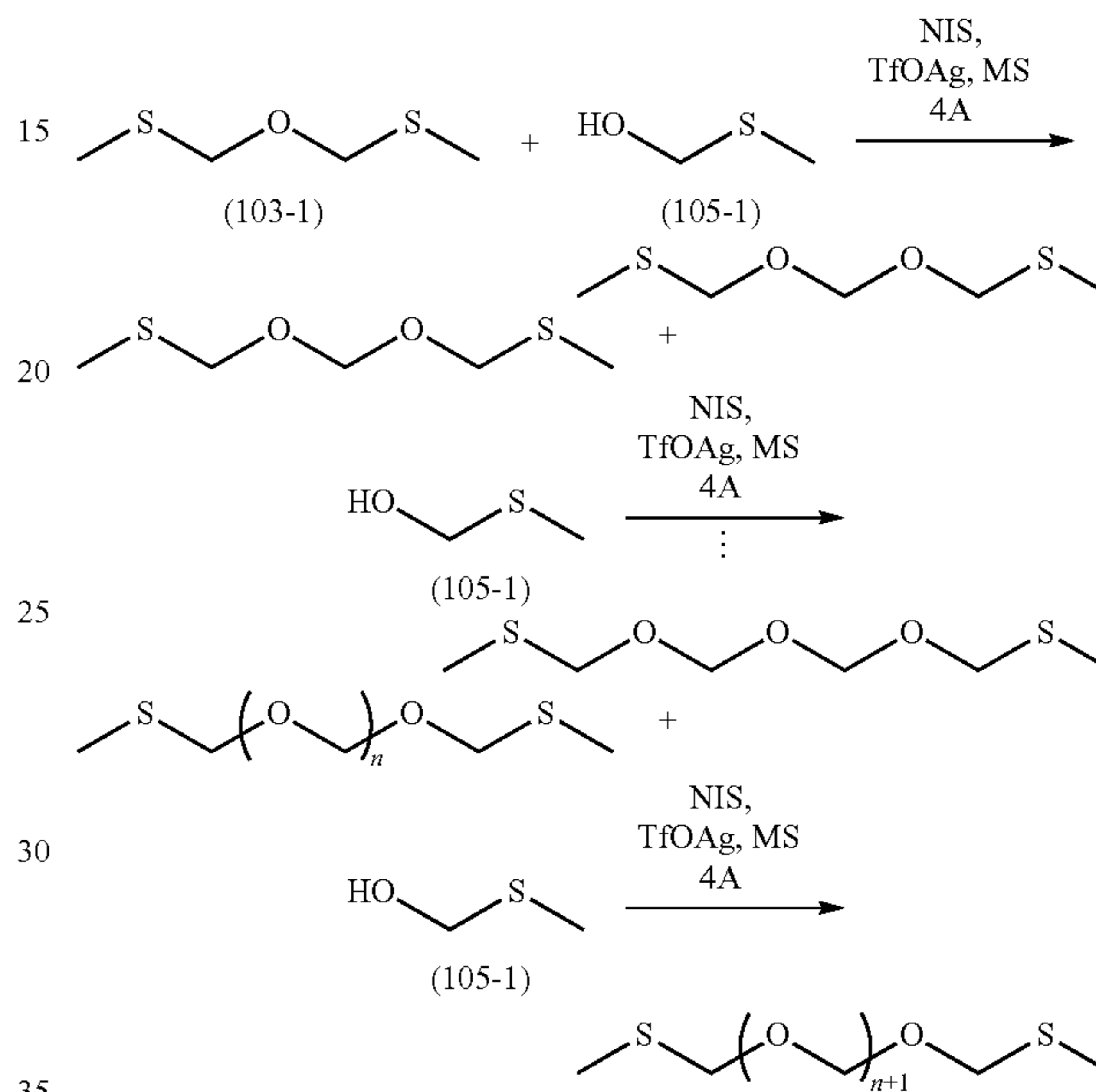
Scheme 2-2
