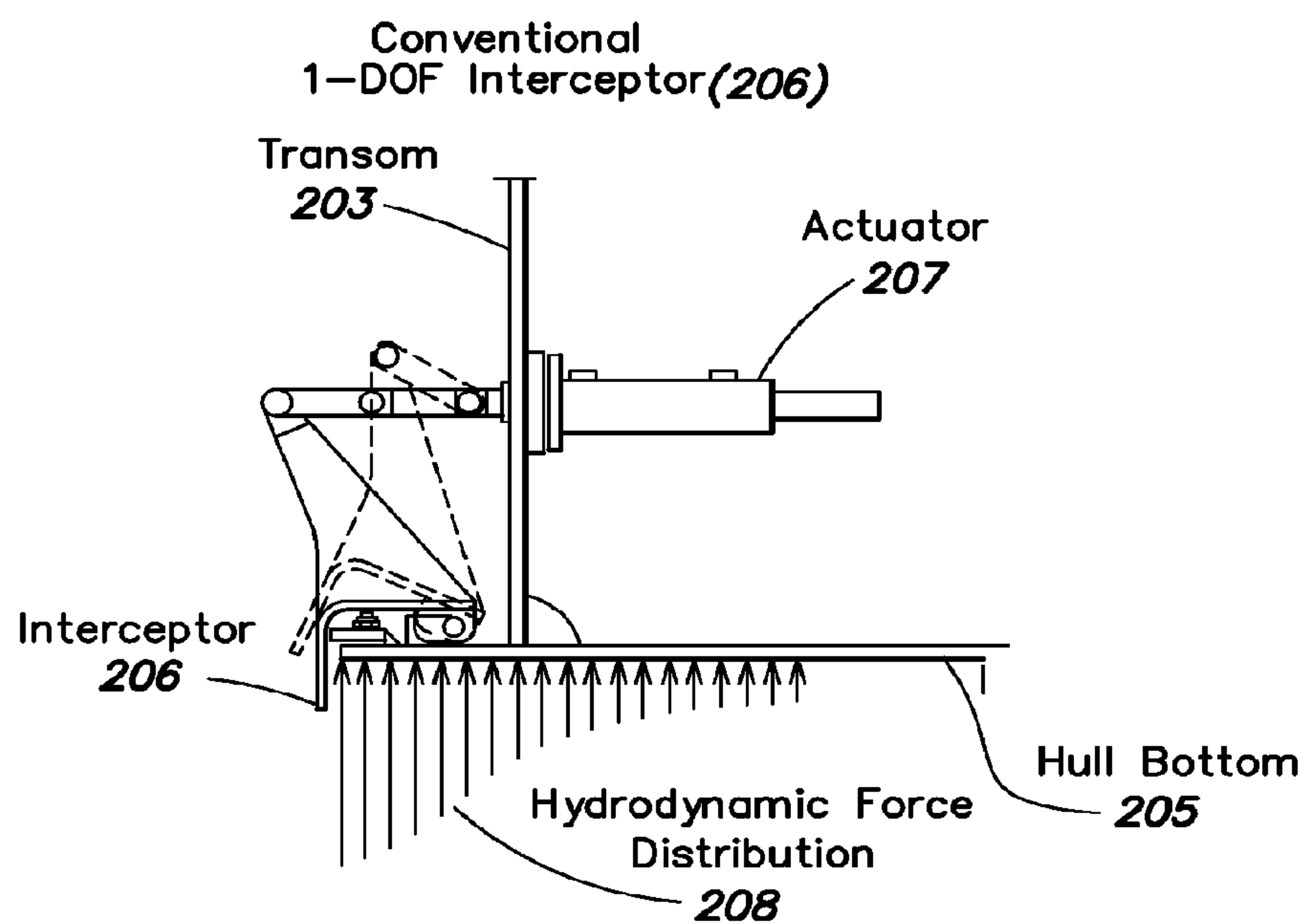
FIG. 2 (Prior Art)
