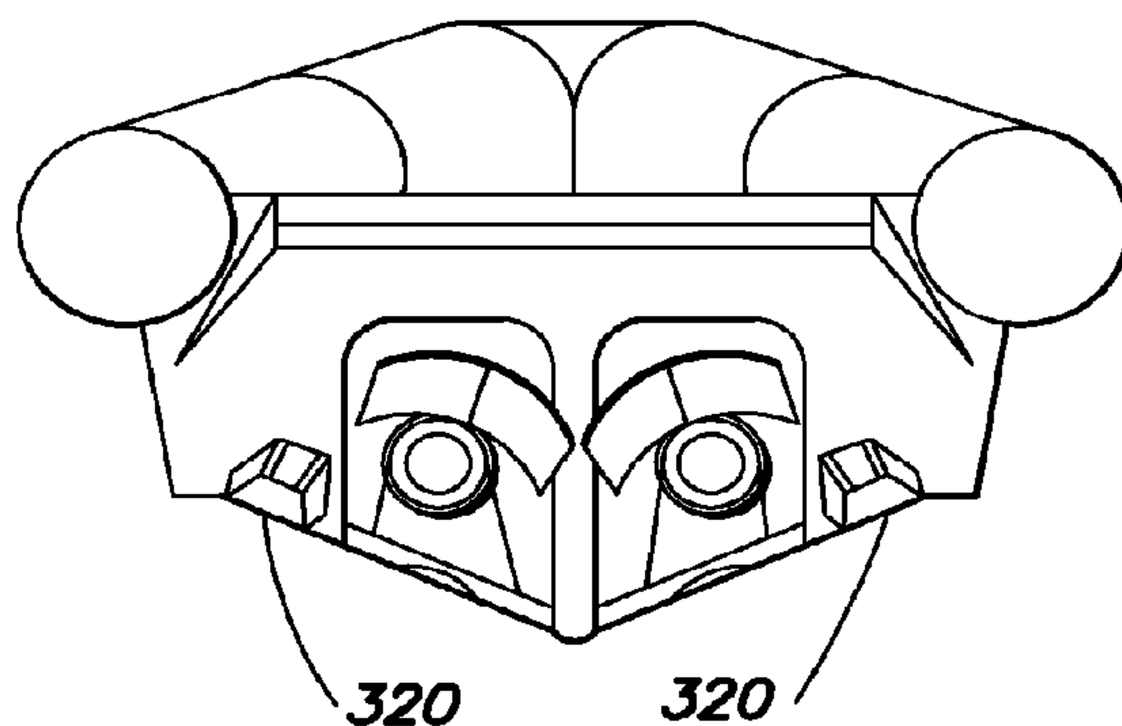
Conventional 1DOF Trim-Tabs - Up
