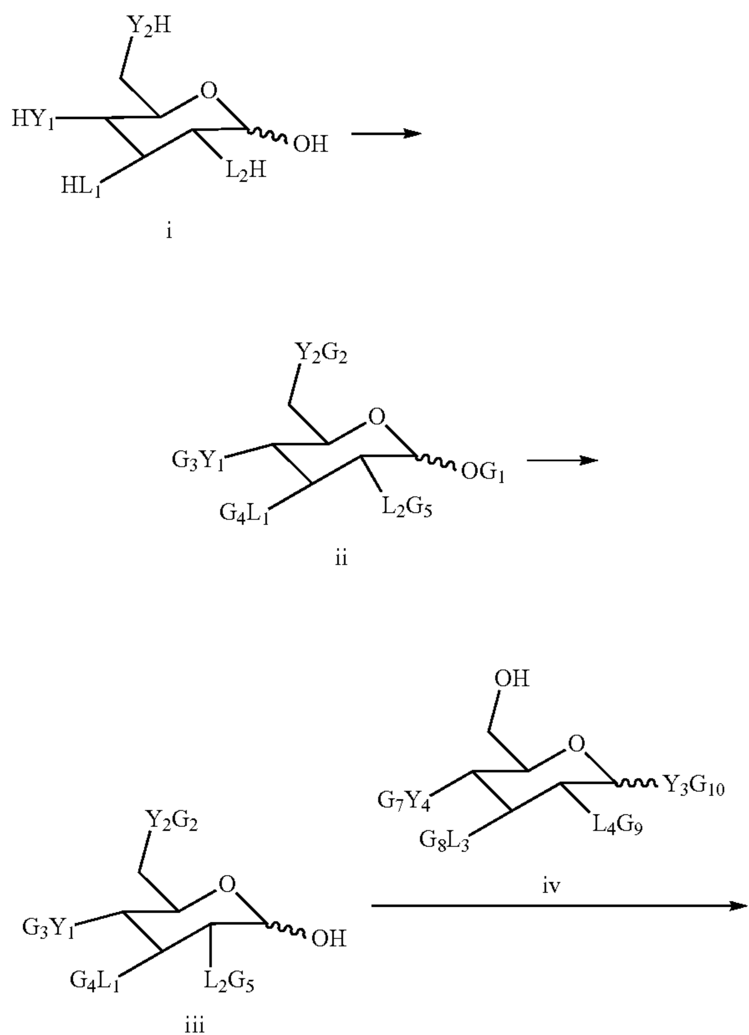
Reaction Scheme 1
