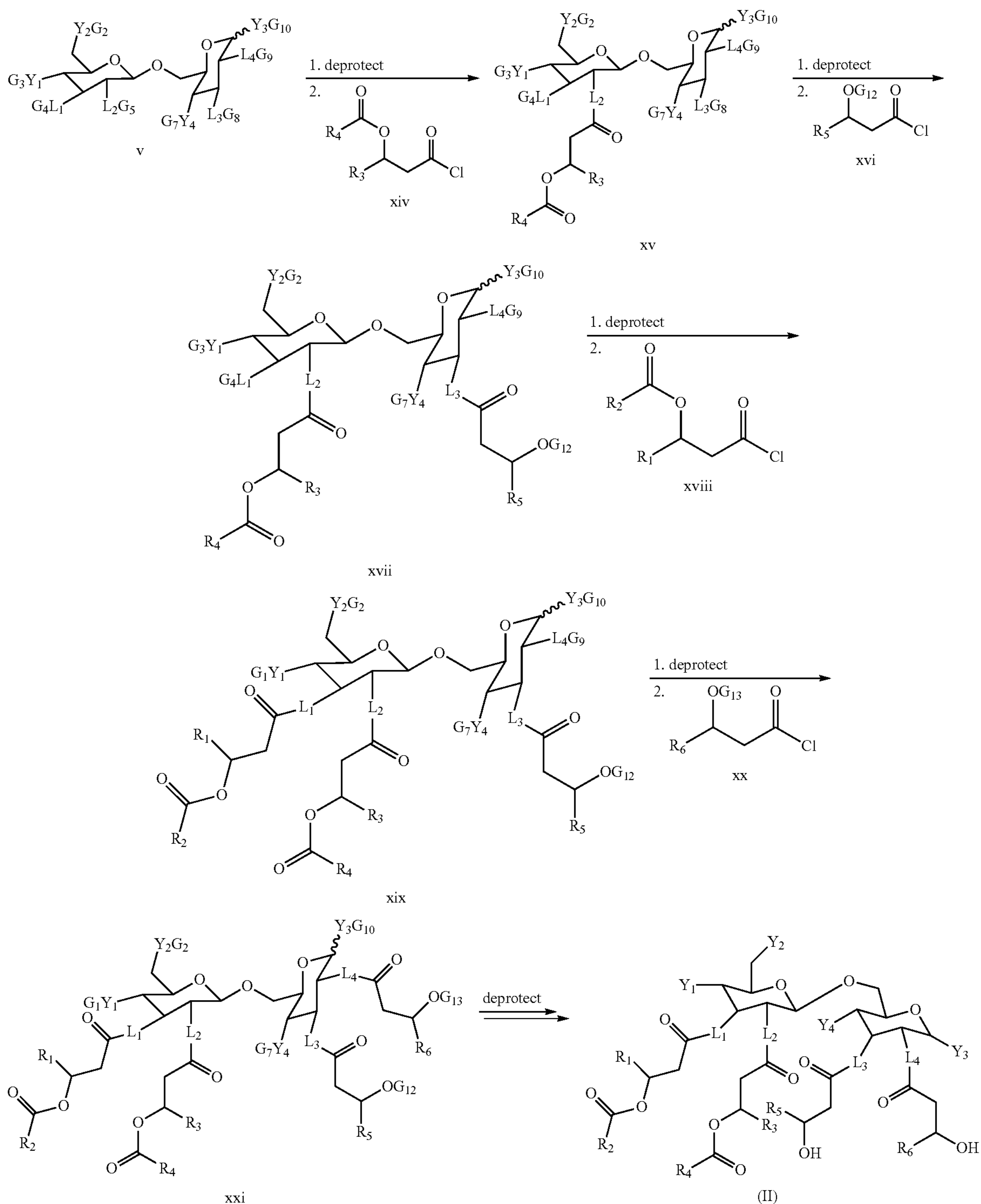
Reaction Scheme 3
