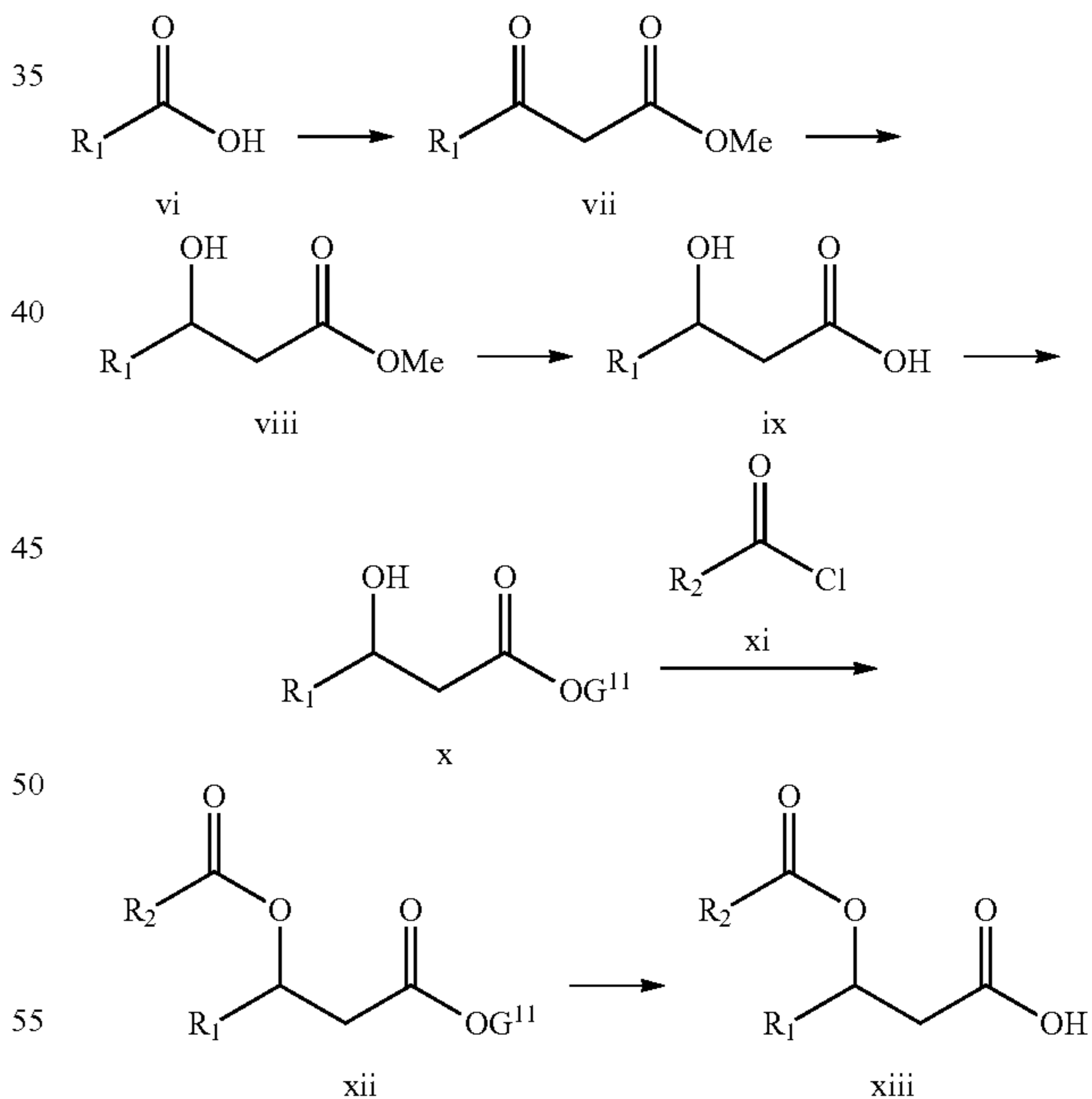
Reaction Scheme 2
