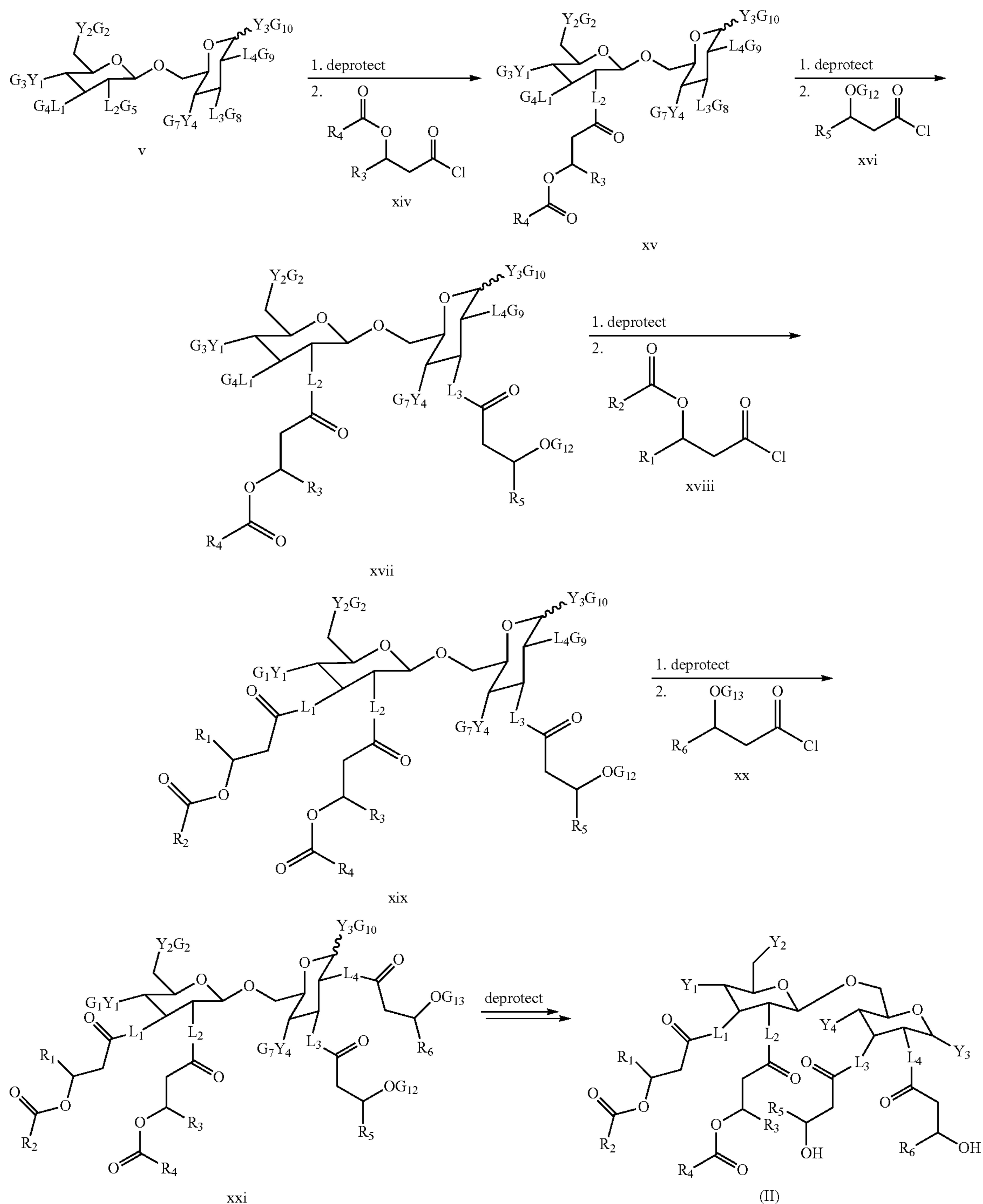
Reaction Scheme 3
