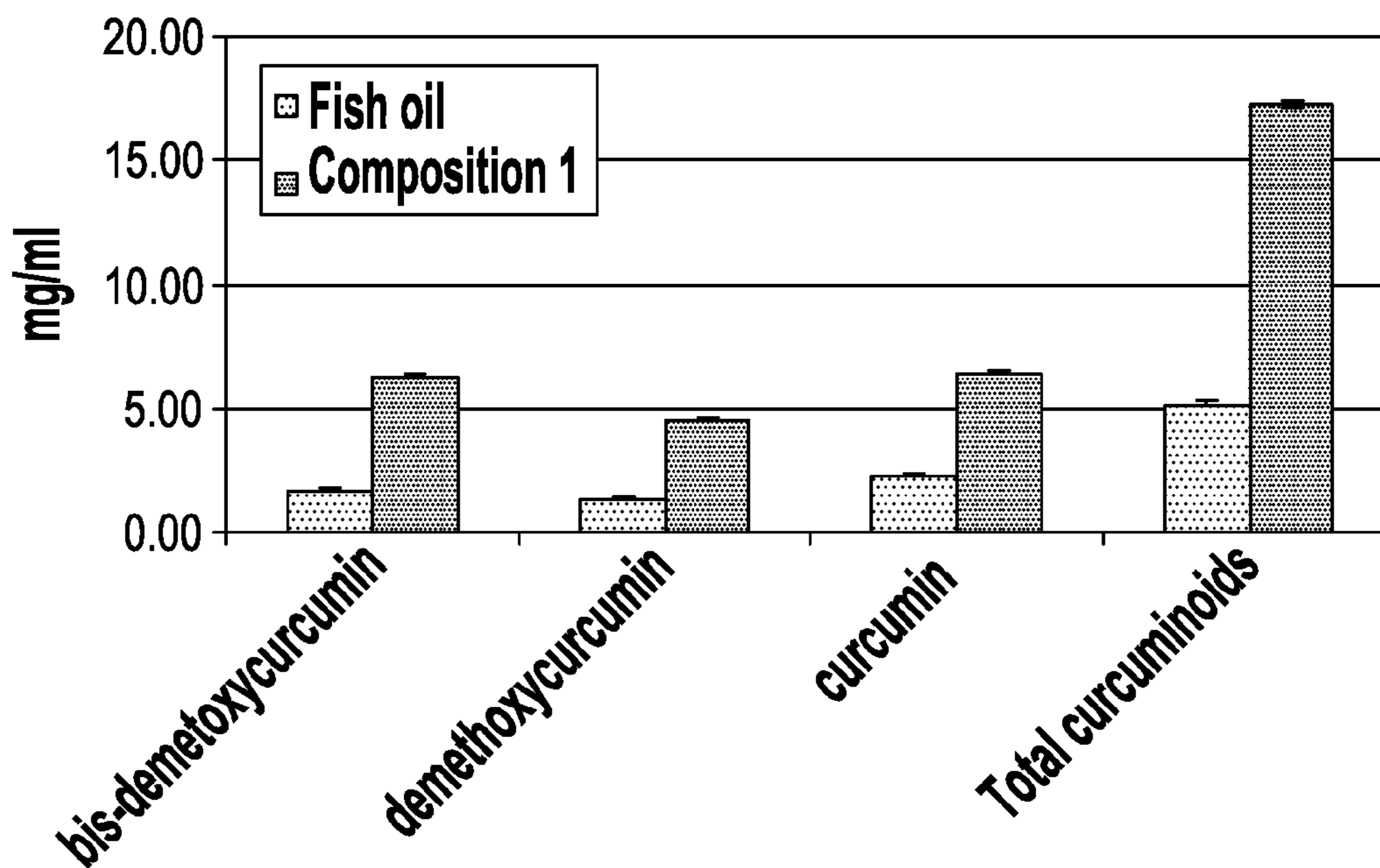
Curcuminoids solubility
