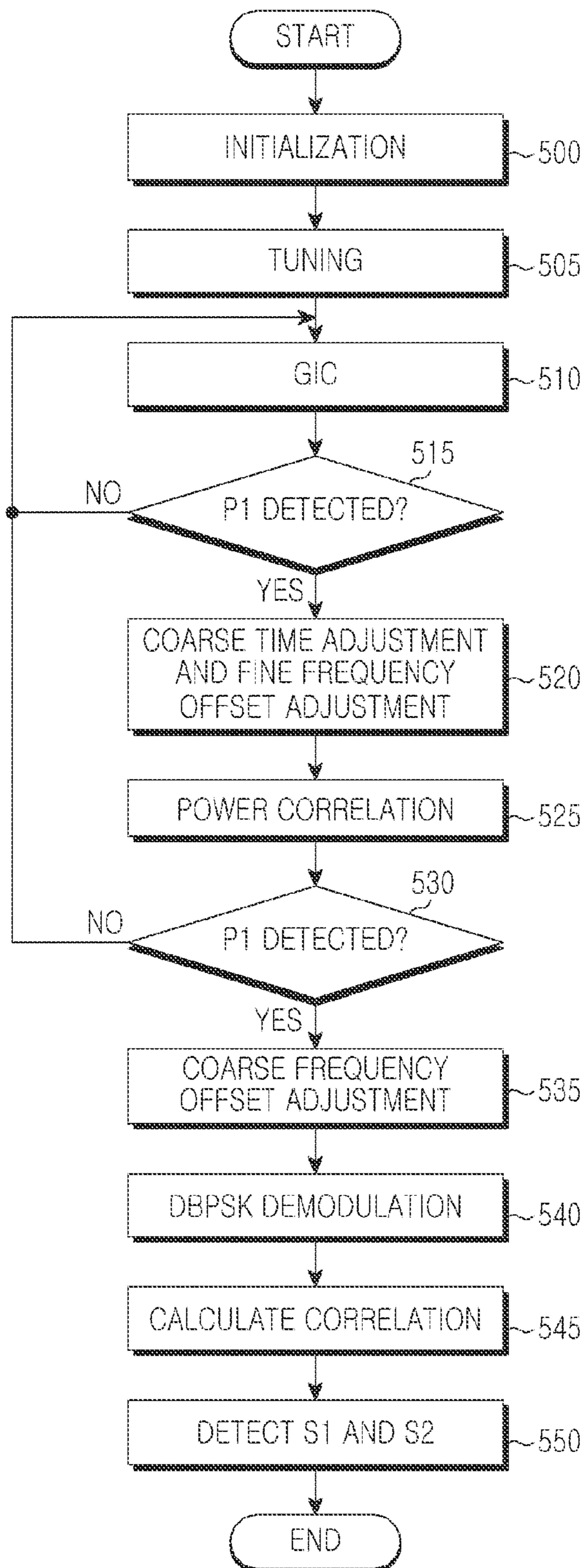
FIG. 5 (PRIOR ART)
