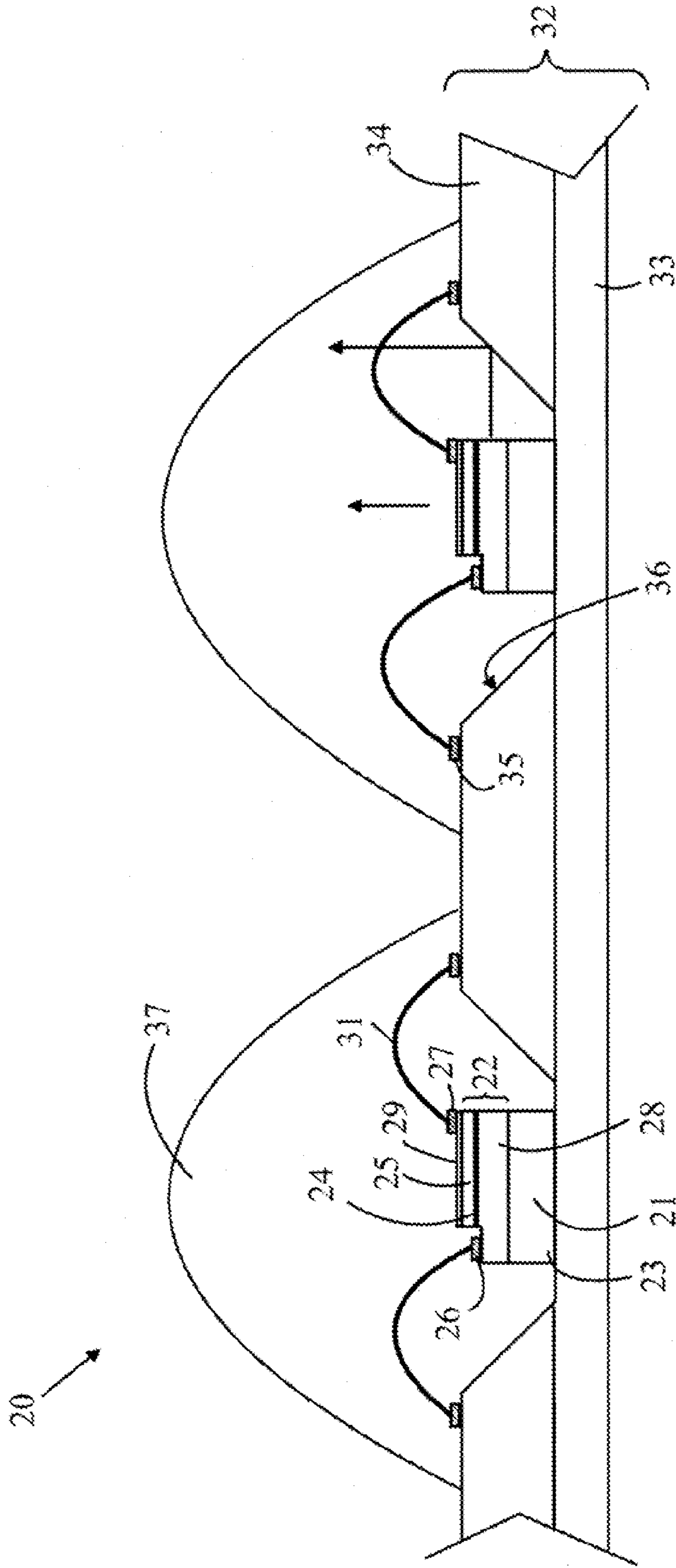
FIG. 1 (PRIOR ART)
