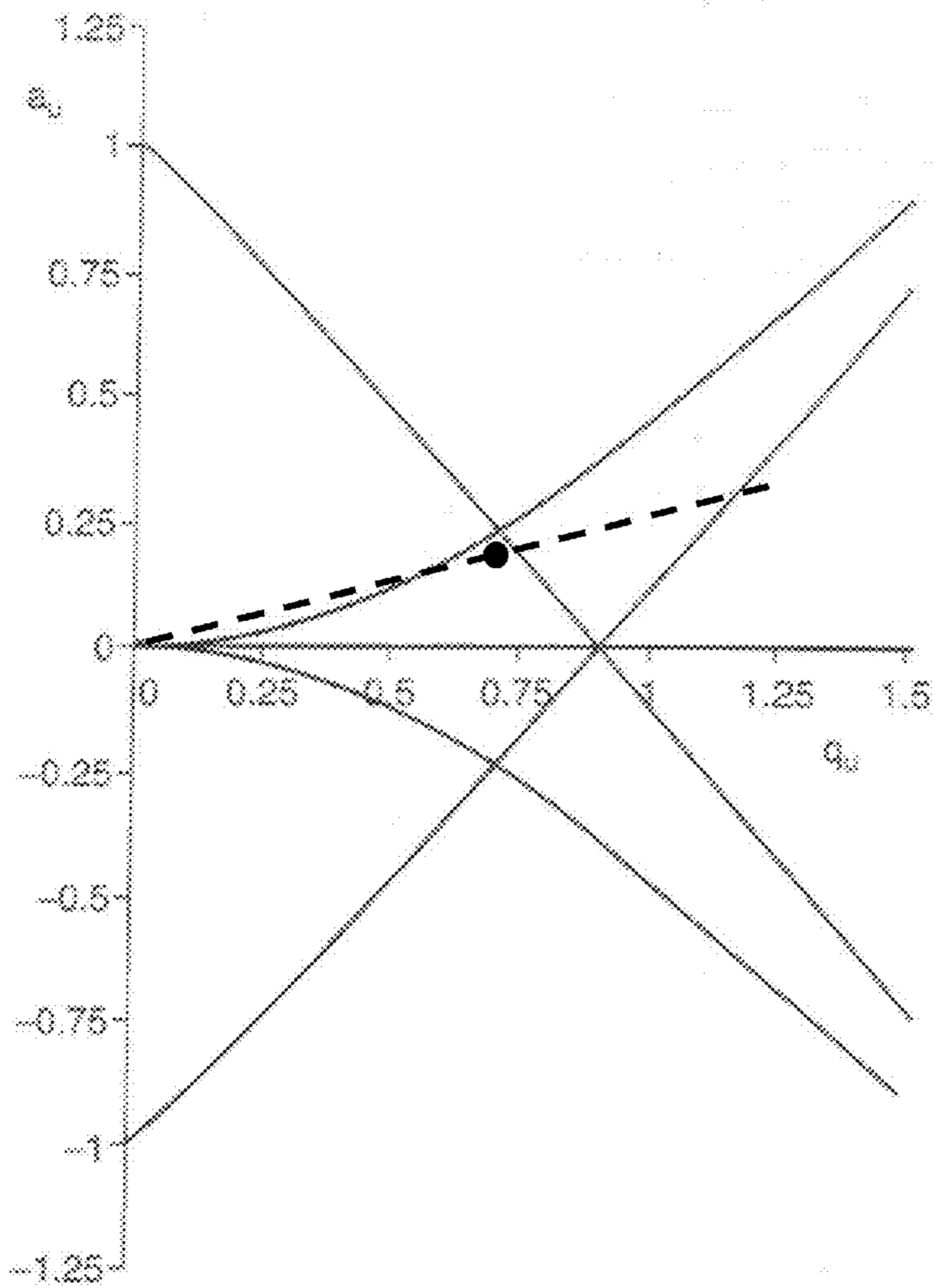
Precursor isolation in a quadrupole mass filter
