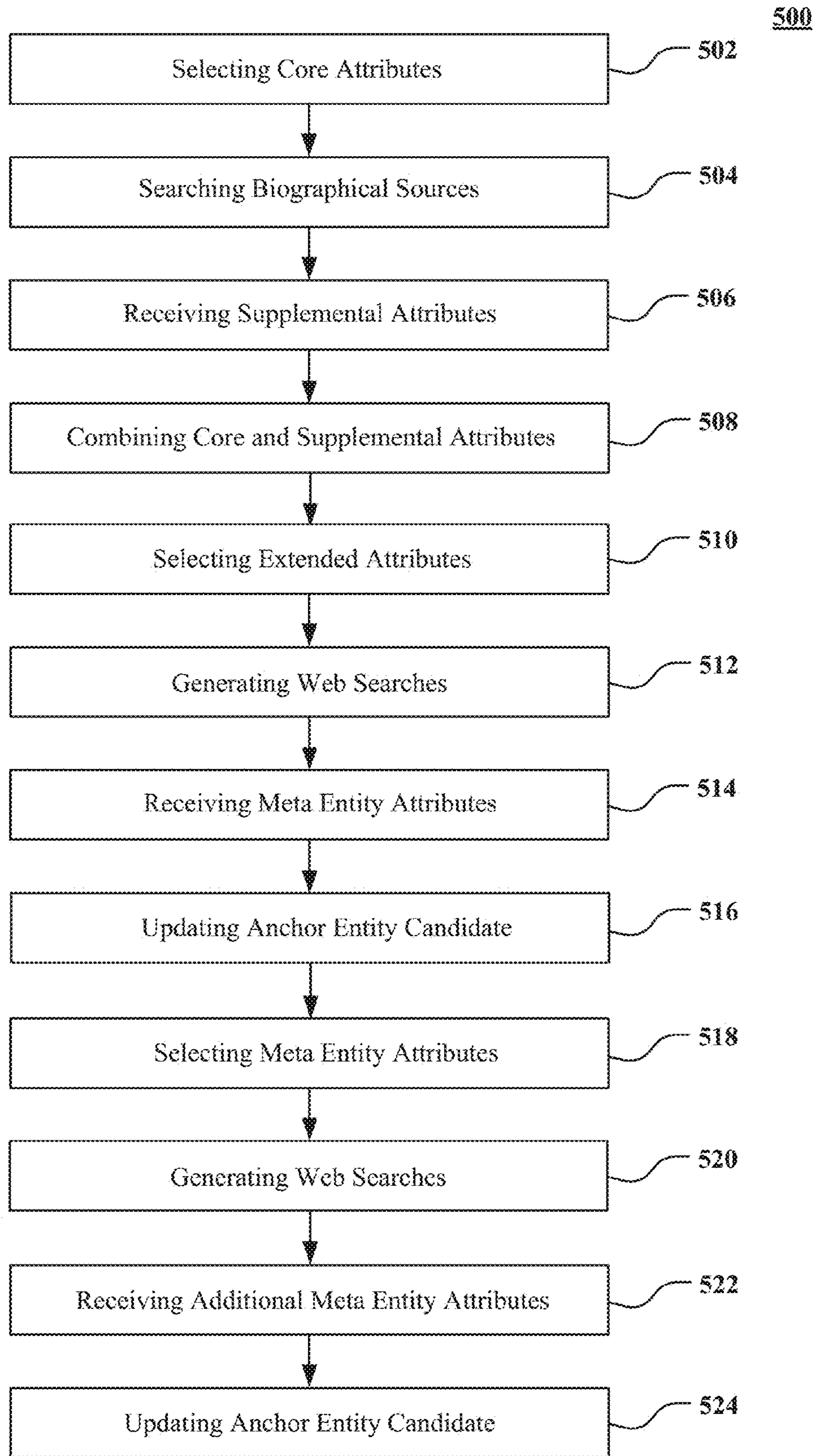
Fig. 5 – Entity Identification
