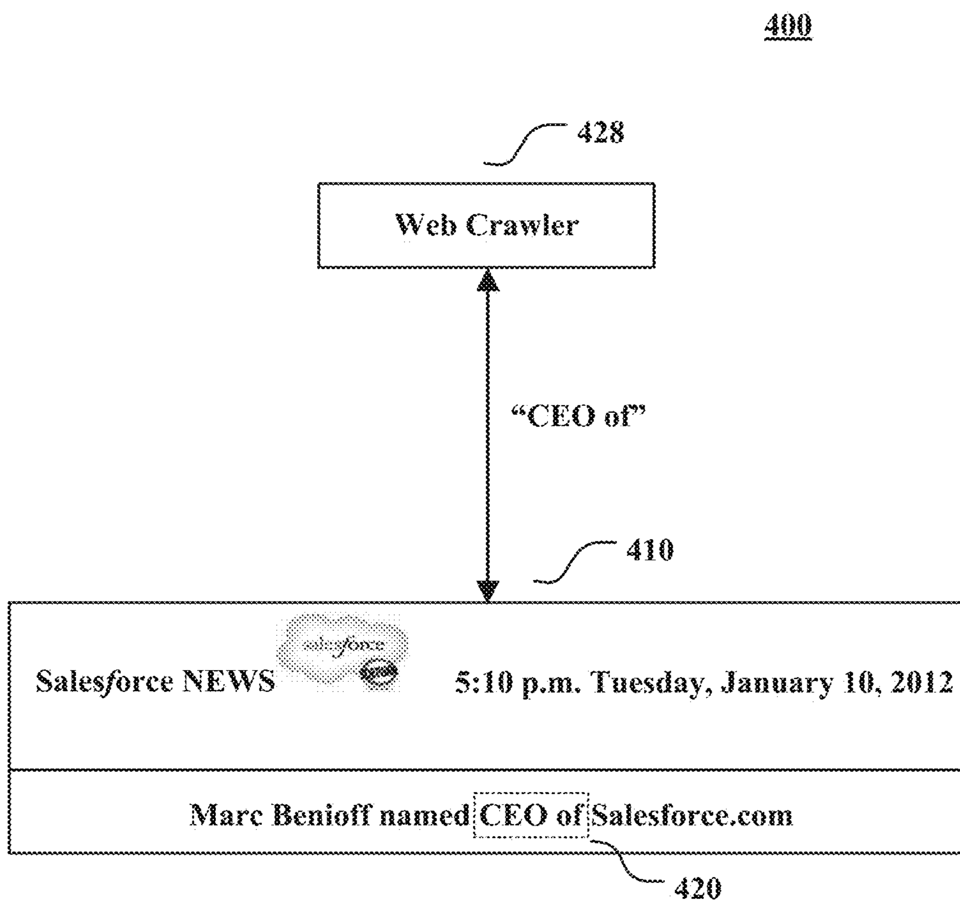
Fig. 4 – Predicate Analysis
