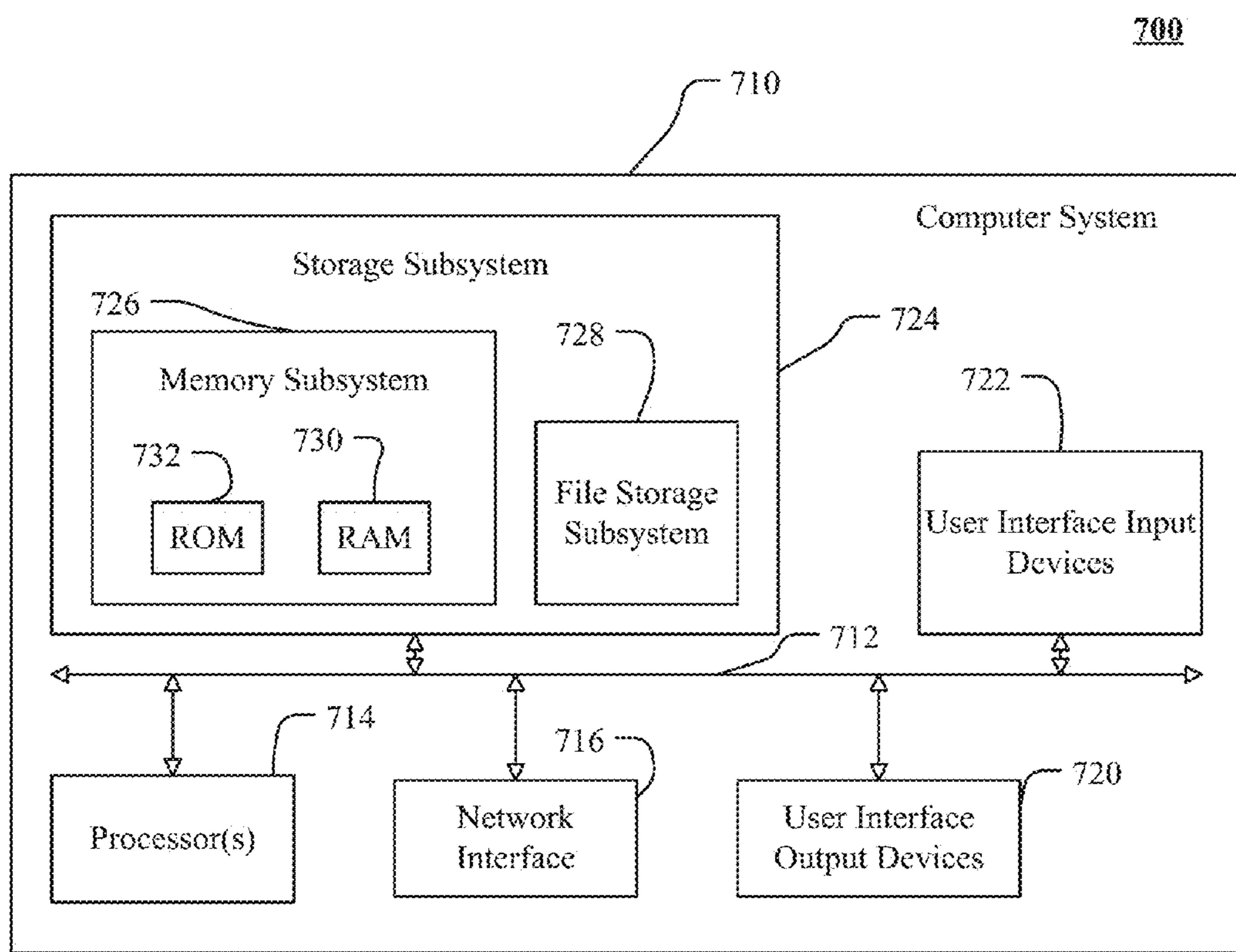
Fig. 7 – Computer System
